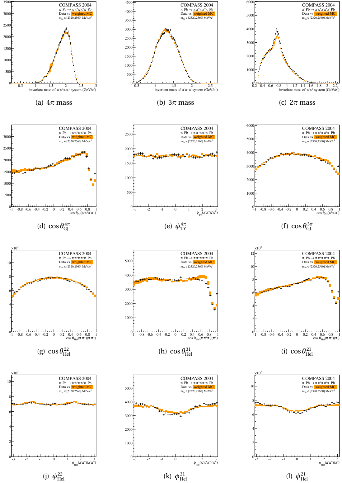
Figure 5.5: Comparison of the model (orange) with the data (black). For a detailed description of the kinematic variables shown, see text. m_{5\pi} \in [2.32, 2.56] \text{ GeV}/c^2
