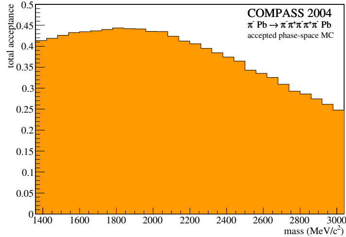
Figure 3.14: Total acceptance for low- t' events ( t' < 0.005 \text{ GeV}^2/c^2 ) as determined by phase-space Monte Carlo simulation.
