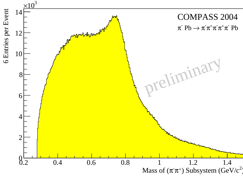
Figure 3.7: Invariant mass of \pi^+\pi^- pairs out of the 5 charged pions in the final state. There are 6 entries per event in this plot. The \rho(770) is clearly visible on top of a large (combinatorial) background.
