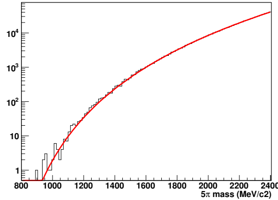
Figure 6.1: 5 pion phase space. The histogram shows the distribution predicted by the GENBOD Monte Carlo generator. The red line is the fit according to equation 6.5.
