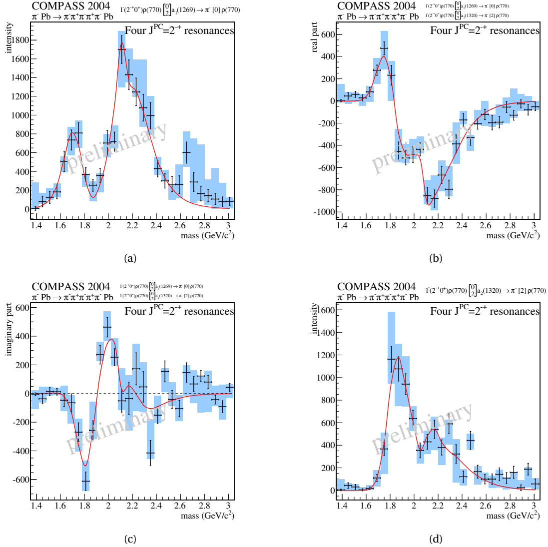
Figure 6.16: The 2^{-+}\rho a_1 (a) and 2^{-+}\rho a_2 (d) amplitudes and their interference (c,b) as described by the fit with four \pi_2 resonances. Note that the this fit is unstable if the allowed parameter ranges are changed.
