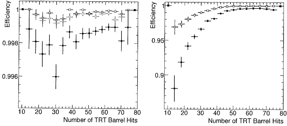
Figure 3.26: Pixel detection efficiency as a function of the number of TRT barrel hits on track with the solenoid magnet on (left) and off (right). The estimated efficiency is shown after the basic selection (cf. 3.4.1) in black solid circles, after the cluster association correction (cf. 3.4.3) in open red circles, and after an additional correction to avoid problematic pixels (cf. 3.4.4) in open blue squares. Note the different y-axis scales used for the two plots.
