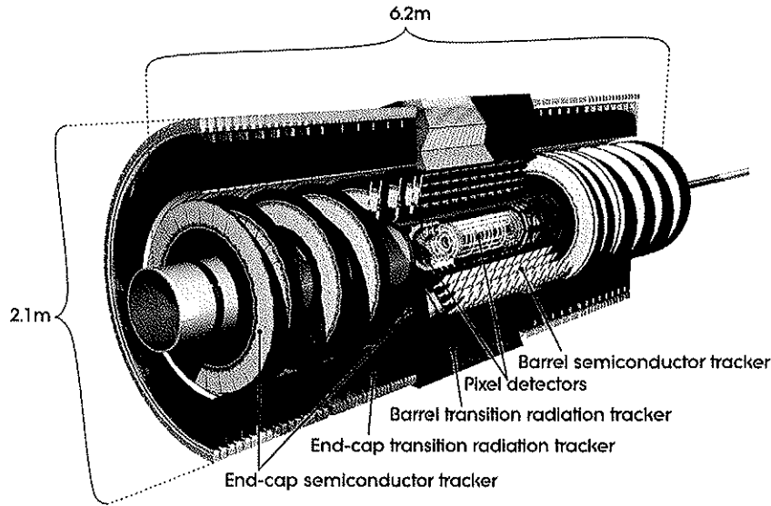
Figure 2.4: General layout of the ATLAS inner detector [32].
