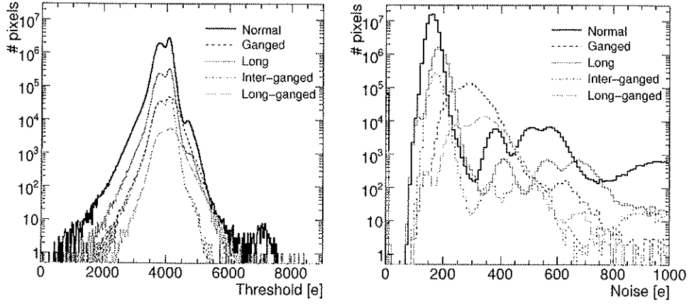
Figure 3.10: Threshold (left) and noise (right) distributions per pixel using an old tuning of the TDACs. The threshold scan used to extract these data is done in-situ. The two peaks present in the threshold distribution correspond to the two sets of modules that were produced in two different sites. The peak at zero in both distributions represents the modules, chips or individual pixels that failed the scan.
