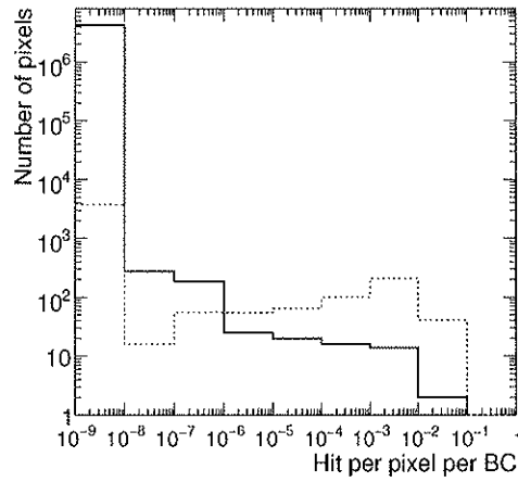
Figure 3.14: Pixel occupancy measured on surface with endcap A. Special pixels from the production SPM are shown as a red dashed line, other pixels as a solid black line.
