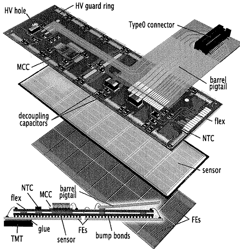
Figure 3.2: Layout of an ATLAS pixel module [34].
