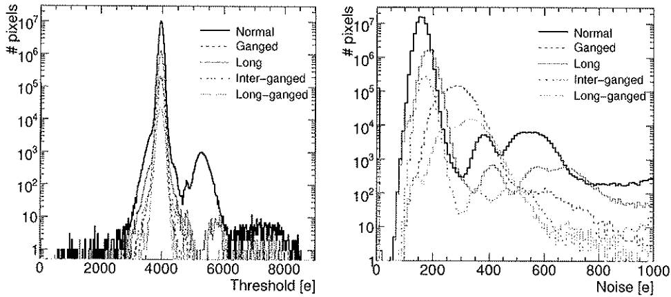
Figure 3.11: Threshold (left) and noise (right) distribution per pixel using an in-situ tuning of the TDACs. The threshold scan used to extract the data is done in-situ. The second peak in the threshold distribution, at about 5300 e, represents one bad module. The peak at zero in both distributions represents the modules, chips or individual pixels that failed the scan.
