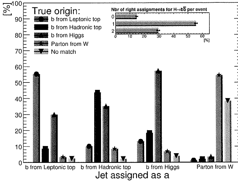
Figure 4.40: Truth origin for jets as assigned by the likelihood reconstruction method.
