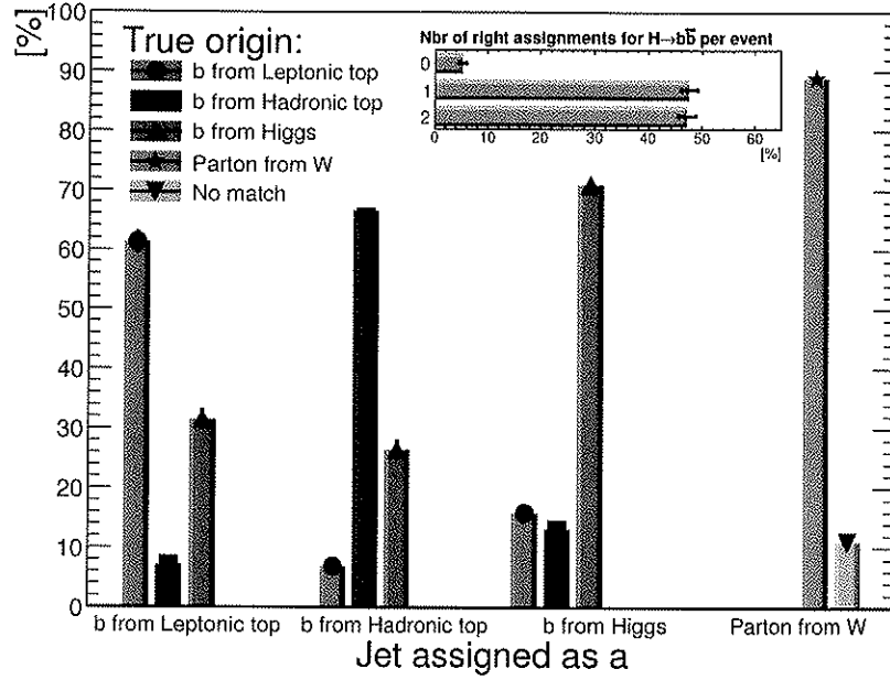
Figure 4.41: Truth origin for jets as assigned by the likelihood reconstruction method. Only event with a perfect preselection are kept.
