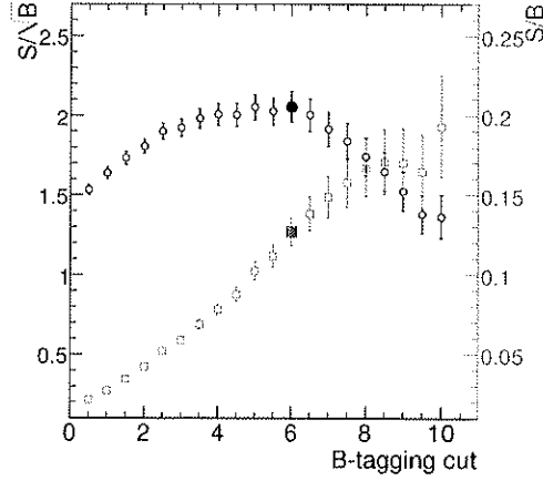
Figure 4.20: S/\sqrt{B} and S/B versus the b-tagging cut. S and B are computed for the cut-based analysis for 30 \text{ fb}^{-1} of data. Solid symbols indicate the chosen cut.
