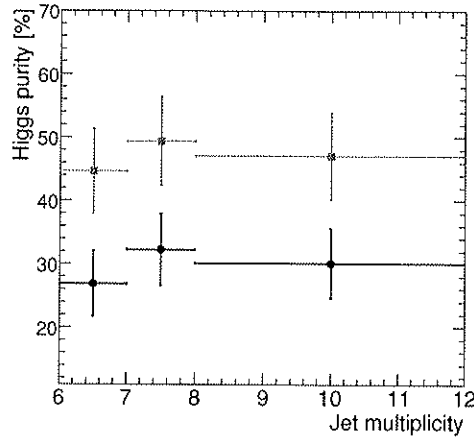
Figure 4.39: Higgs boson purity as a function of the number of jets per event for all events (black solid lines) and for events with perfect preselection (red dashed lines).
