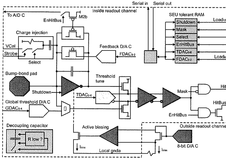
Figure 3.4: Diagram showing the pixel cell electronics [34].
