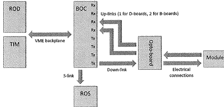
Figure 3.5: Schematic view of the pixel DAQ system showing its main components.
