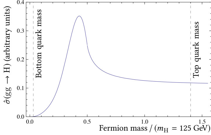
Figure 62: LO partonic gg \rightarrow H cross section as a function of the loop fermion mass. The dashed vertical lines indicate the mass of the bottom and top quark, m_b = 4.5 \text{ GeV} and m_t = 175 \text{ GeV} .
