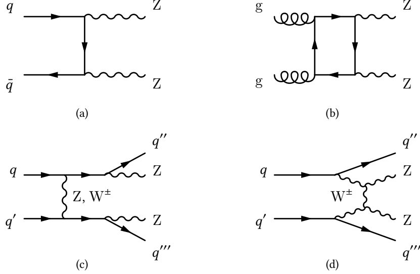
Figure 20: Examples of leading-order SM Feynman diagrams for ZZ (and ZZjj ) production in proton-proton collisions: (a) q\bar{q} -initiated, (b) gg -initiated, (c) electroweak ZZjj production, (d) electroweak ZZjj production via weak-boson scattering. The decays to leptons are omitted for readability.
