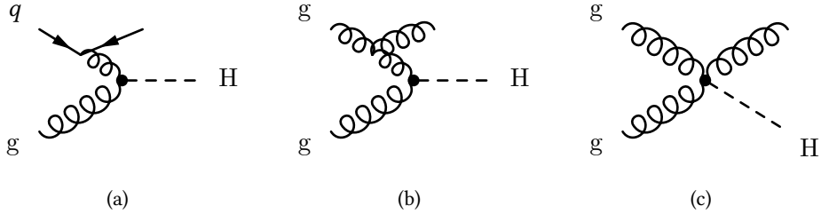
Figure 66: Example LO Feynman diagram for Higgs boson plus jet production via gluon fusion in the m_t \rightarrow \infty approximation.
