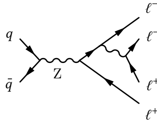
Figure 59: Z-boson production with subsequent decay to four leptons via Z^*/\gamma^* radiation off a lepton.
