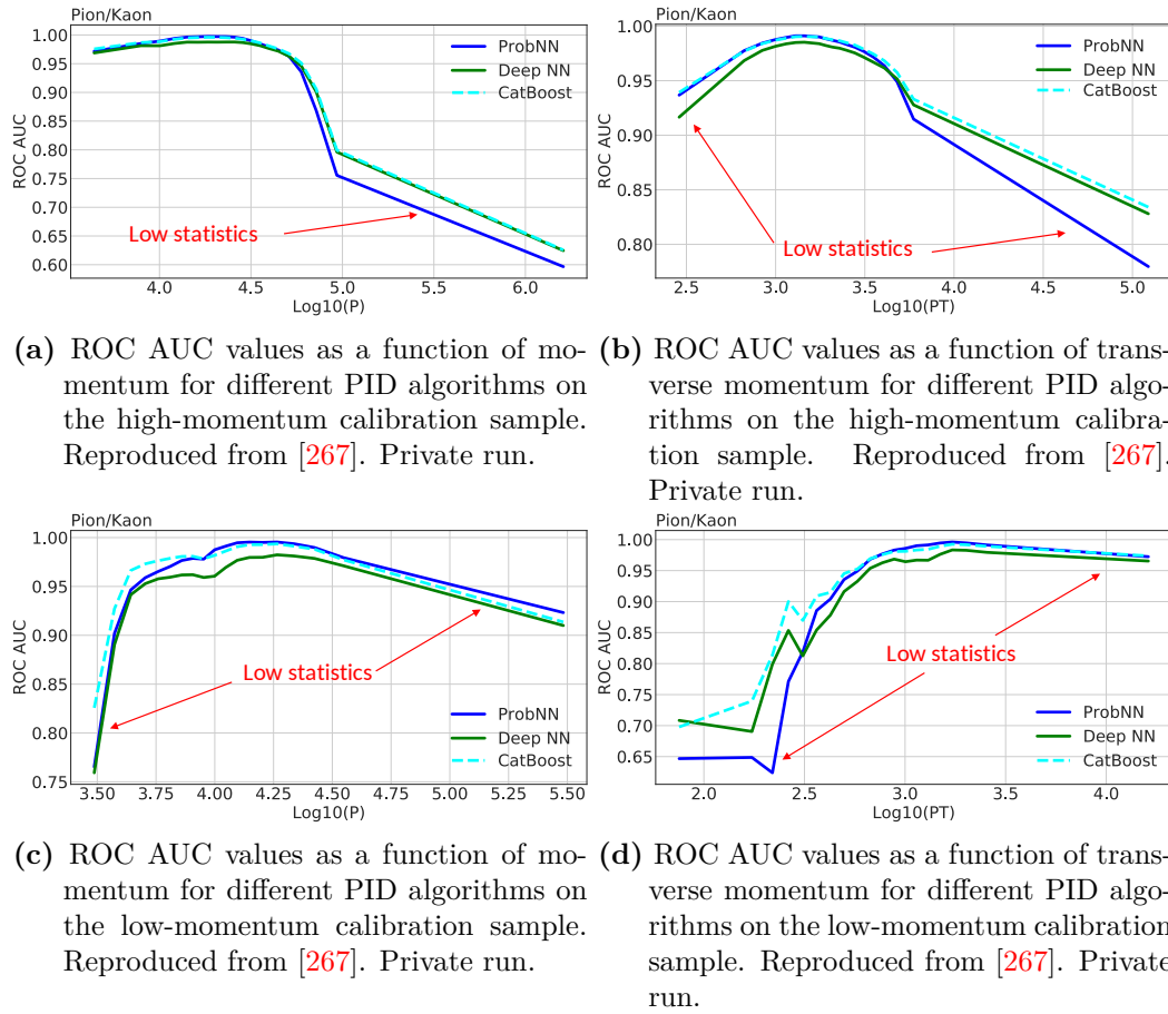
Figure 7.10. ROC AUC values as a function of momentum and transverse momentum.
