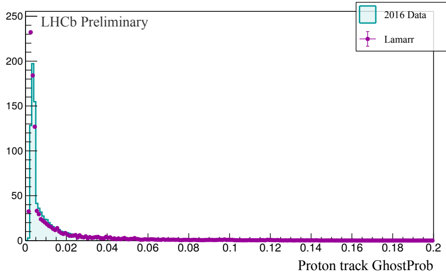
Figure 8.16. Response of a neural network trained to identify ghost tracks, i.e. random combinations of hits not associated to any charged particle. On data, the neural network is evaluated on a calibration sample of protons tagged through the decay \Lambda_b^0 \rightarrow \Lambda_c^+ \mu^- \bar{\nu}_\mu with \Lambda_c^+ \rightarrow p K^- \pi^+ . In the simulated sample the ghost probability is the response of the neural network inside Lamarr. The overall distribution shape is well-reproduce. The difference in the peak height is around 15% and is compounded by the binning effects. First published in [302].
