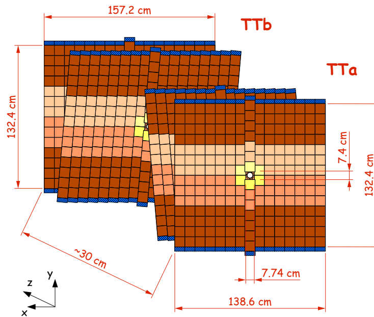
Figure 4.5. Layout of TT layers. Reproduced from [191]
