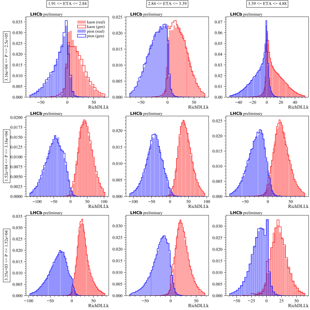
Figure 8.12. Weighted real data and generated distributions of RichDLLk for kaon and pion track candidates in bins of pseudorapidity ( \eta ) and momentum ( P , MeV) over the full phase-space. First published in [300].
