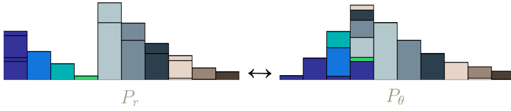
Figure 2.18. An illustration of the optimal transport for a single-dimensional case. The distribution on the left is the source distribution, distribution to the right is the target distribution. The source distribution is broken into chunks which are rearranged to match the target distribution. Reproduced from [136].
