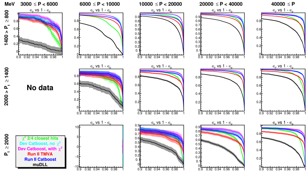
Figure 5.10. Muon efficiency versus proton rejection after applying IsMuon selection using 2016 calibration data that is weighted in momentum and nPVs. “ \chi^2 2/4 closest hits” is described in section 5.3. “Run II Catboost” and “Run II TMVA” are described in section 5.4. “Dev Catboost” are the models trained on data weighted to emphasize the high nPVs events as described in section 5.5. “Dev Catboost, with \chi^2 ” uses \chi^2_{\text{CORR}} as a feature, “Dev Catboost, no \chi^2 ” does not. 2
