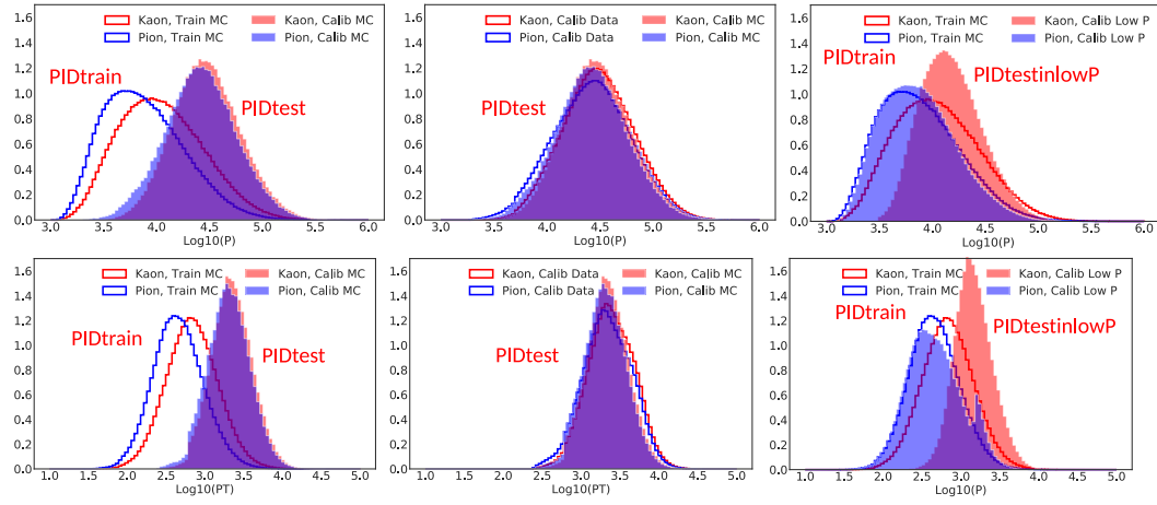
Figure 7.7. Momentum (upper panels) and transverse momentum (lower panels) distributions. Train MC is the simulated dataset used for PID training; Calib Data dataset is the high-momentum calibration dataset; Calib MC is the simulated high-momentum calibration dataset; Calib Low P is the low-momentum calibration dataset
