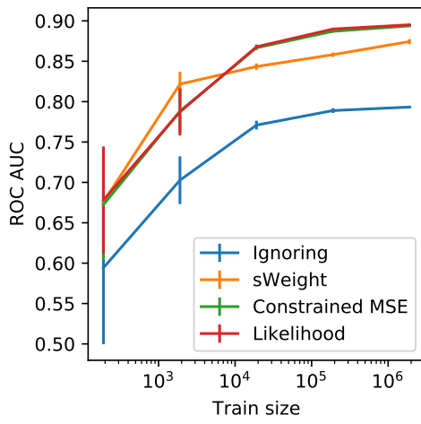
(a) Catboost
