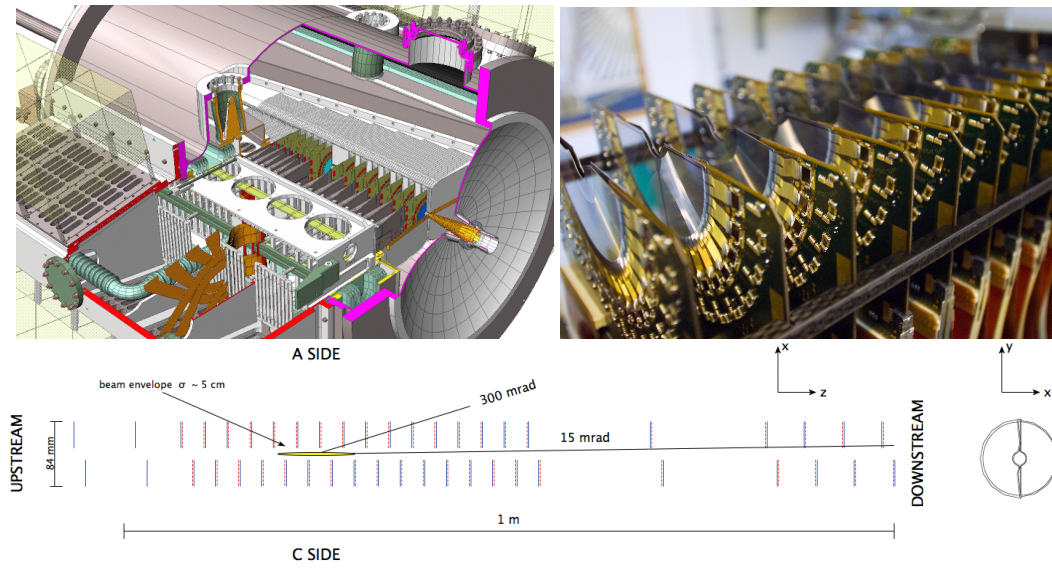
Figure 4.4. (top left) The LHCb VELO vacuum tank. (top right) A photograph of one side of the VELO during assembly showing the silicon sensors and the readout hybrids. (bottom) Cross-section of the detector in the closed position in the xz plane at y = 0 of the sensors; and a view of the sensors in the xy plane. Reproduced from [189].
