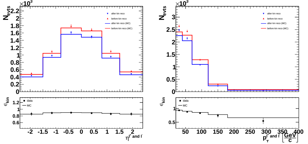
Figure 8.5: Differences between the number of events before (red) and after (blue) the kinematic reconstruction. The left plot shows the behaviour in the pseudorapidity and the right plot in the transverse momentum of the leptons.
