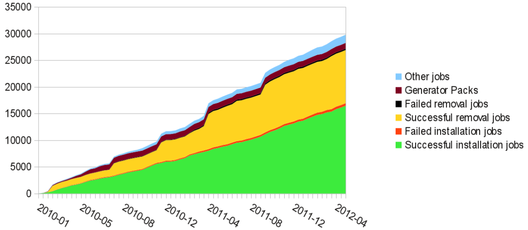
Figure 4.7: Overview of all grid jobs sent with the deployment tools since 2010. Jobs which have installed or removed more multiple releases are counted multiple times.
