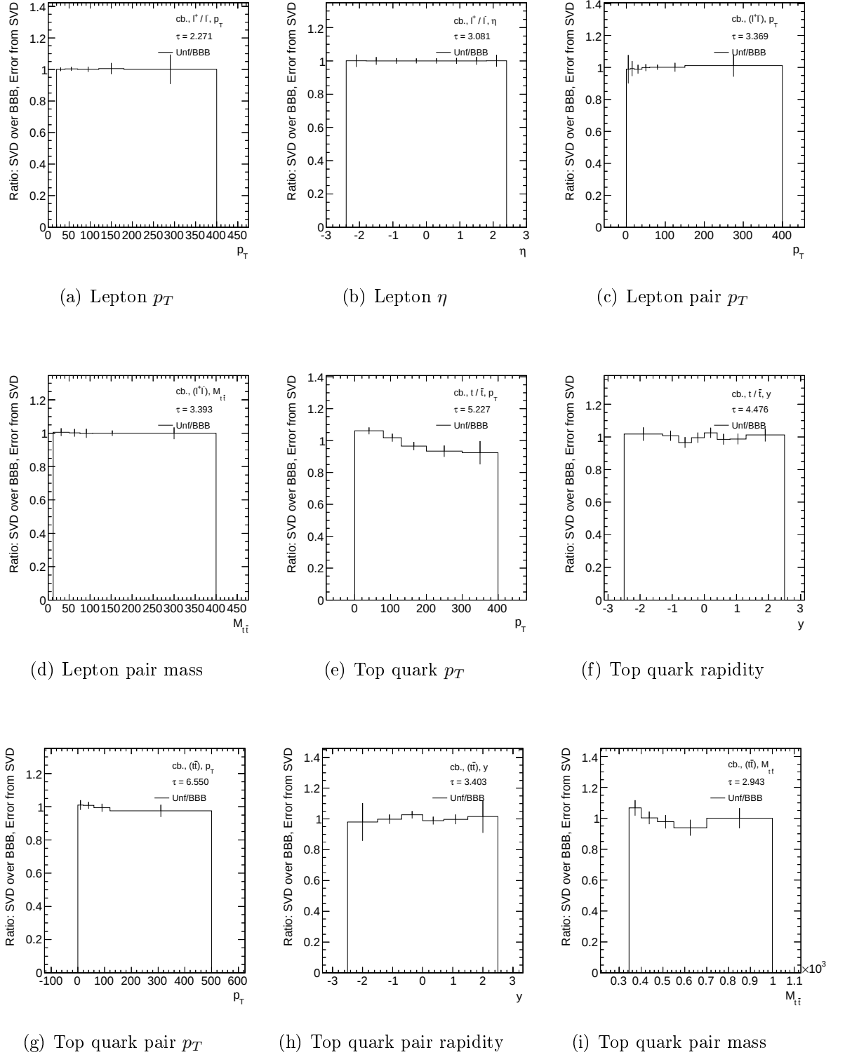
Figure D.6: Comparison between full unfolding and binwise cross section calculations [153].
