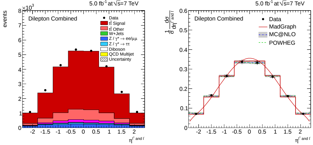
Figure 10.4: Event yield and normalised lepton \eta^{\ell^+} and \eta^{\ell^-} cross section for 5 \text{ fb}^{-1} [140, 150].
