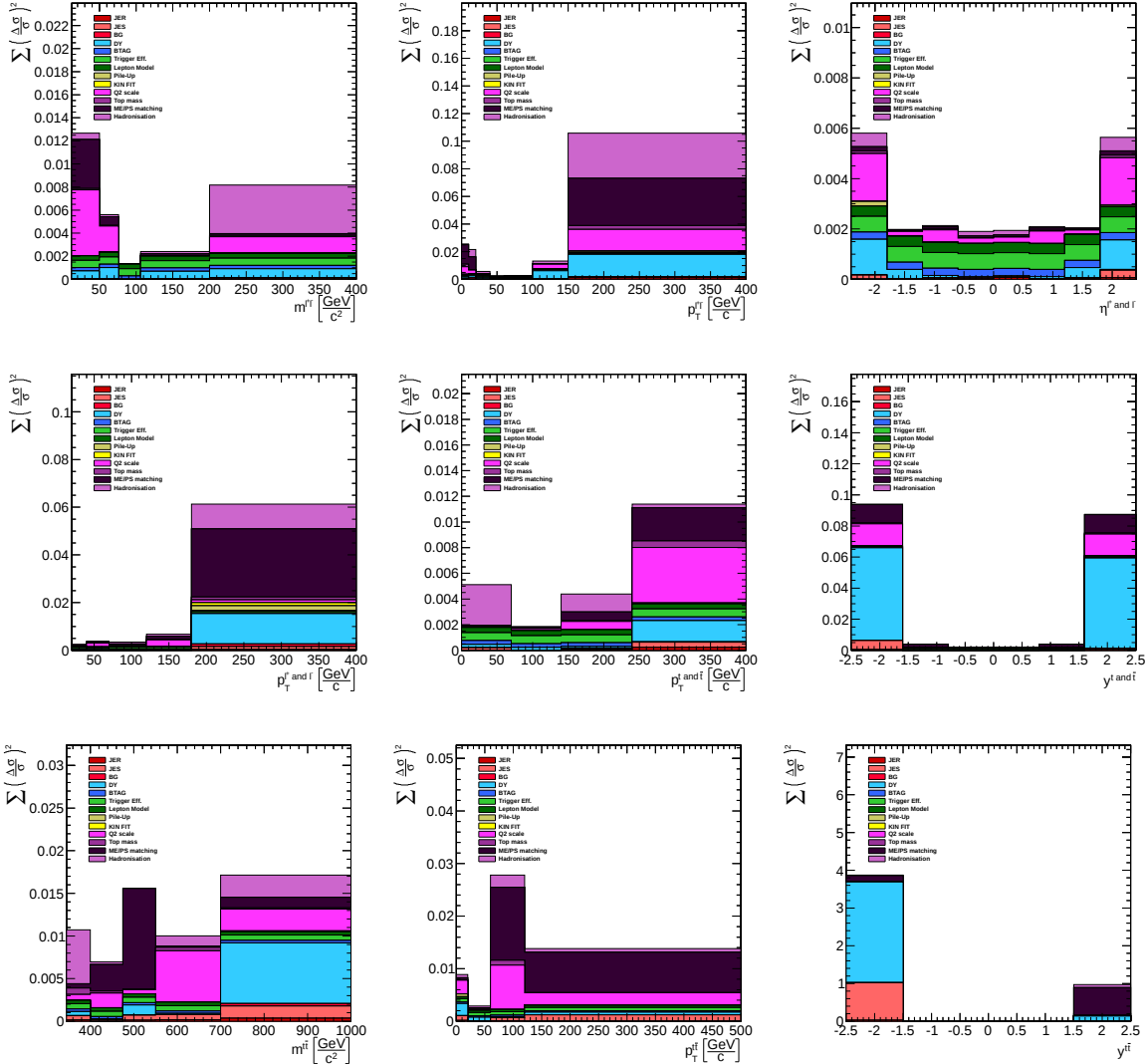
Figure B.1: The plots show the squares of the systematic uncertainties in all bins of all measured cross section quantities for the ee channel.
