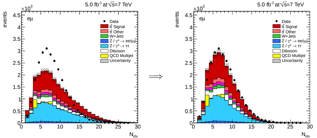
Figure 10.1: Vertex multiplicity in the e\mu channel after dilepton selection before (left) and after (right) reweighting in 5 fb -1 [150].
