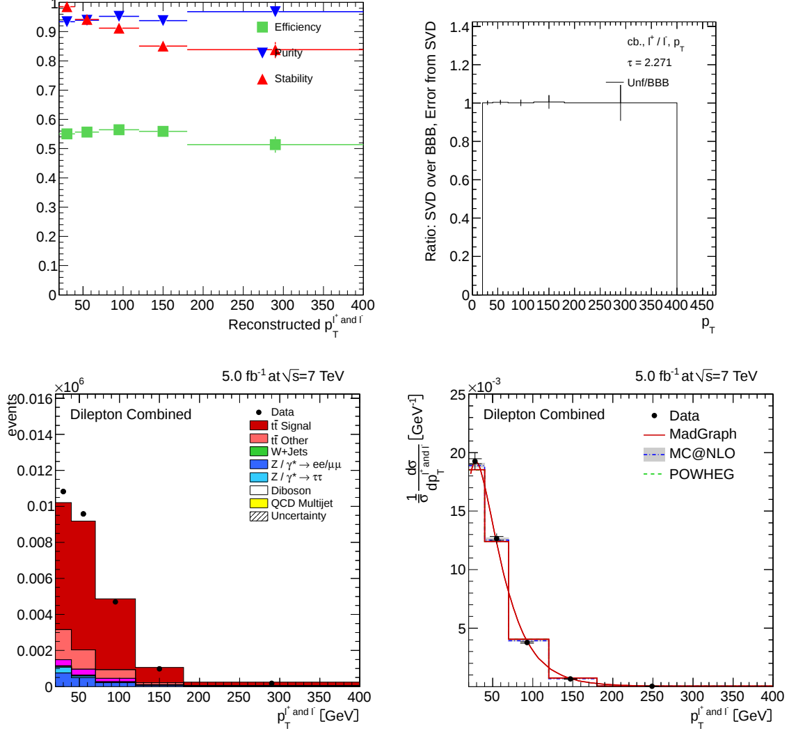
Figure 10.3: Normalised lepton p_T^{\ell^+ and \ell^-} cross section for 5 \text{ fb}^{-1} [140, 150]. The first row shows the purities, stabilities and efficiencies and the ratio between the results from SVD and binwise unfolding [153]. The second row shows the event yield and the normalised differential cross section.
