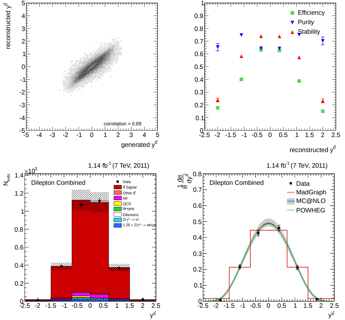
Figure 9.10: Top row: correlation between generated and reconstructed y^{t\bar{t}} and calculated purity, stability and efficiency. Bottom row: event yield on the left and the normalised differential cross section on the right.
