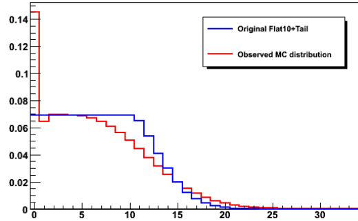
Figure 8.1: Ideal (blue curve) and observed (red curve) primary vertex distribution for simulated samples [126], including the unintended large one vertex bin.
