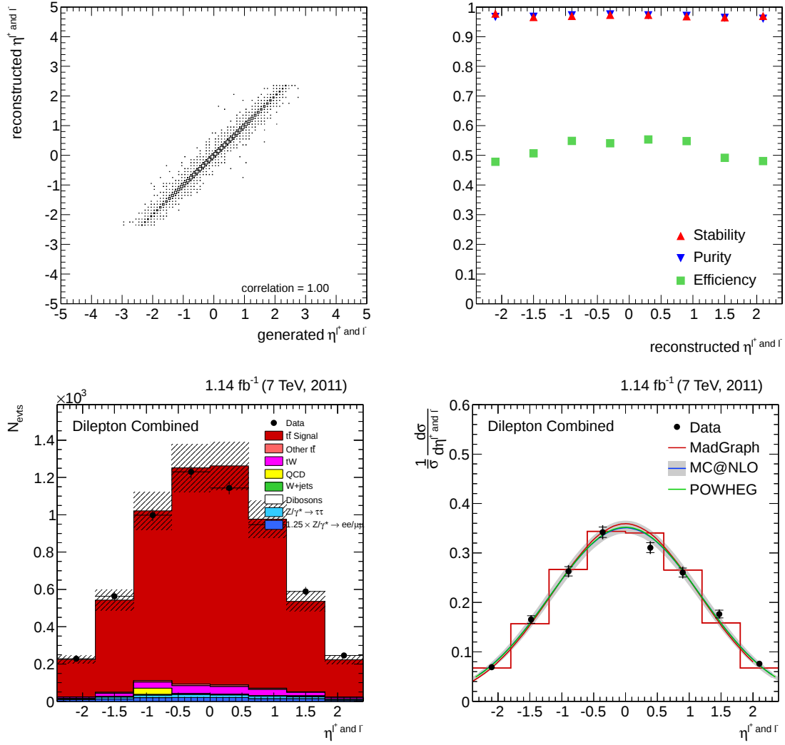
Figure 9.3: Top row: correlation between generated and reconstructed \eta^{\ell^+} and \eta^{\ell^-} and calculated purity, stability and efficiency. Bottom row: event yield on the left and the normalised differential cross section on the right.
