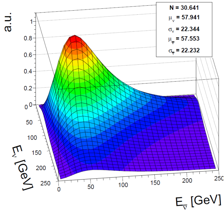
Figure 7.6: Fit to a simulated neutrino spectrum generated with PYTHIA [91]. The most probable neutrino energies, \mu_\nu/\bar{\nu} , are \sim 58 GeV for both neutrinos; the width \sigma is \sim 22 GeV, and N is a normalisation factor irrelevant for this study.
