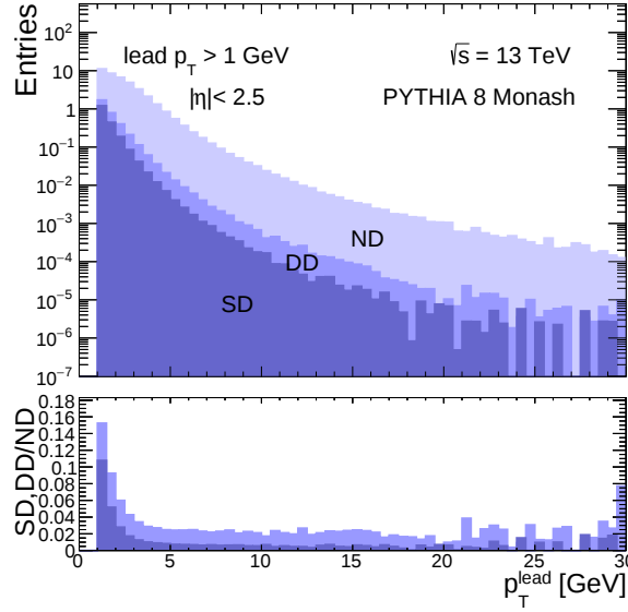
Fig. 8.2: Comparison of Monash non-diffractive, double diffractive and single diffractive p_T^{lead} components
