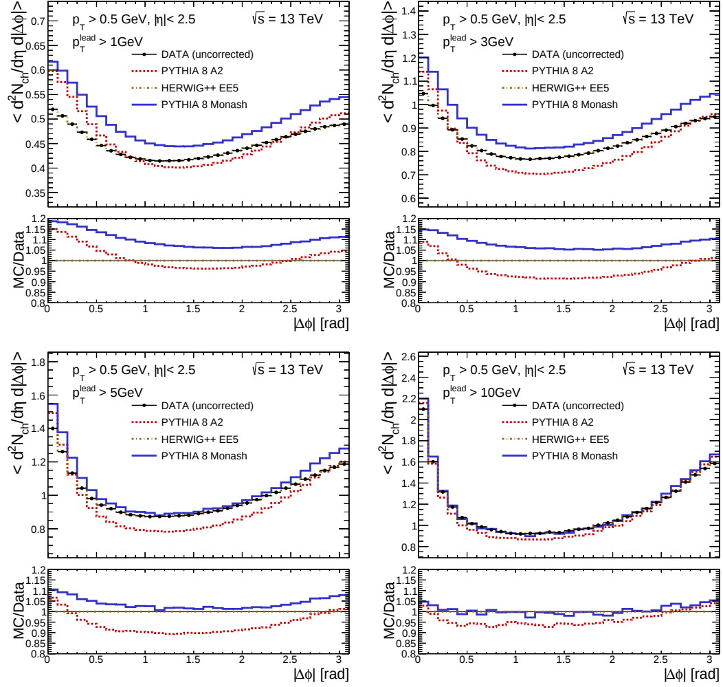
Fig. 8.3: Mean number of tracks per unit \eta - \phi vs |\Delta\phi| for p_T^{\text{lead}} > 1, 3, 5 and 10 GeV, leading track excluded.
