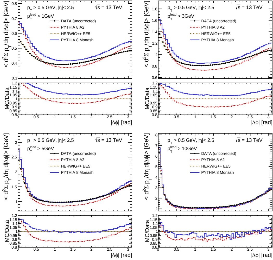
Fig. 8.5: Mean scalar p_T sum of track per unit \eta - \phi with respect to \Delta\phi for p_T^{\text{lead}} > 1, 3, 5 and 10 GeV, leading track excluded.
