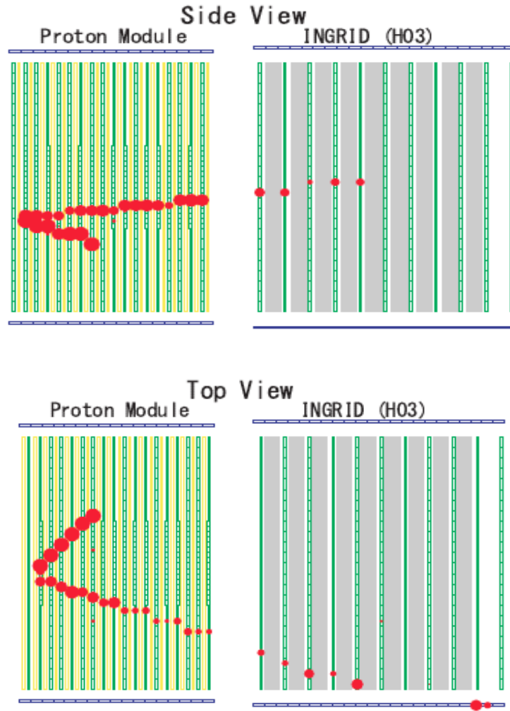
Figure 2.15: Typical neutrino event in the INGRID detector: the neutrino enters from the left, the interaction happens in the Proton Module (left module), producing charged particles whose energy deposition is shown as red circles.
