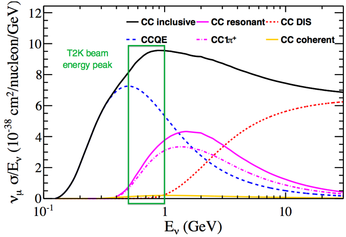
Figure 2.9: NEUT cross sections per nucleon for charged-current interactions of \nu_\mu on carbon as a function of neutrino energy, with the T2K energy band overlaid: the CCQE channel is enhanced and the backgrounds are reduced.
