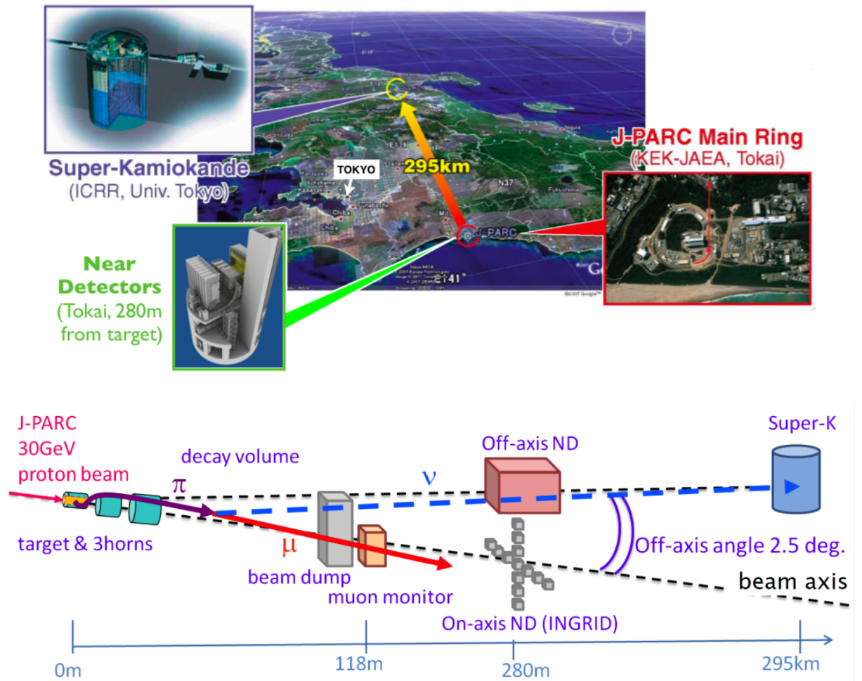
Figure 2.1: Layout of the T2K experiment, showing the position of the J-PARC accelerator facility where the \nu_\mu beam is produced, the near detectors located at 280 meters from the target and the far detector Super-Kamiokande 295 km away.
