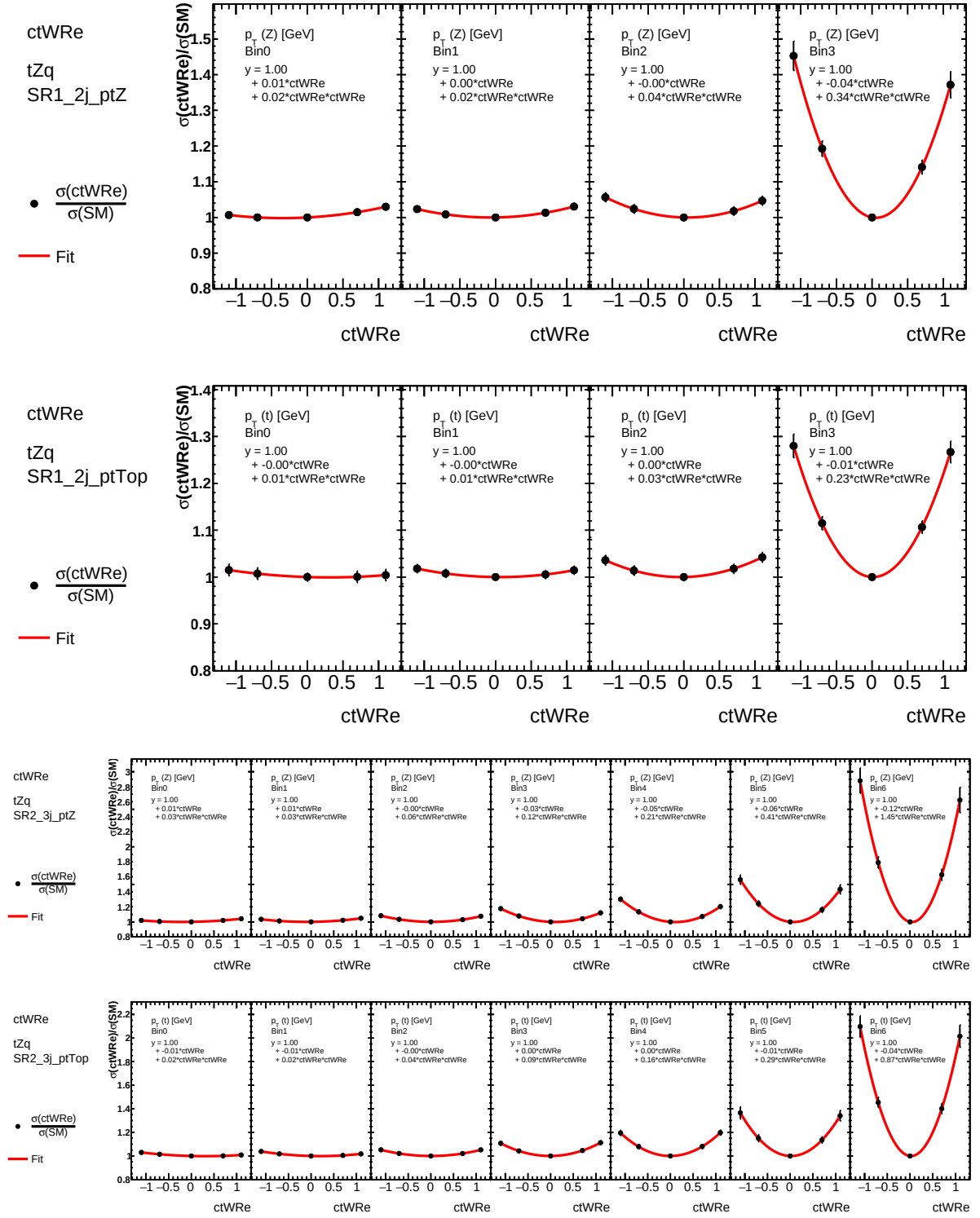
Figure 6.4.: Fits for the p_T in both SRs for the \mathcal{O}_{tW} operator.
