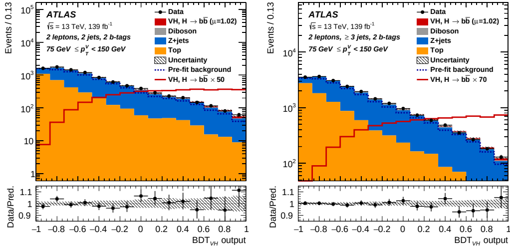
Figure I.1: Distributions of the \text{BDT}_{VH} scores in the categories with 2, \geq 3 jets and 75 \leq p_T^V < 150 GeV of the 2-lepton channel. The stacked histograms show the prediction after the fitting. The red unstacked and unfilled histograms show the VH signals with the scale factors indicated in the legend. The lower panels show the ratio of the data and the prediction of the signals and the backgrounds. The hatched bands in the lower and upper panels show the total uncertainty that includes both the statistical and systematic uncertainties.
