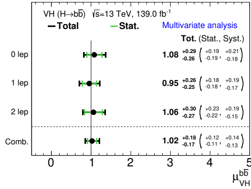
Figure 10.3: Observed signal strengths \mu_{VH}^{bb} of the VH processes in the 0-, 1- and 2-lepton channels and the combination. The \mu_{VH}^{bb} values for the channels are obtained from the simultaneous fits with the individual signal strengths for these channels. The combined \mu_{VH}^{bb} is obtained from the fit with the single signal strength for three channels.
