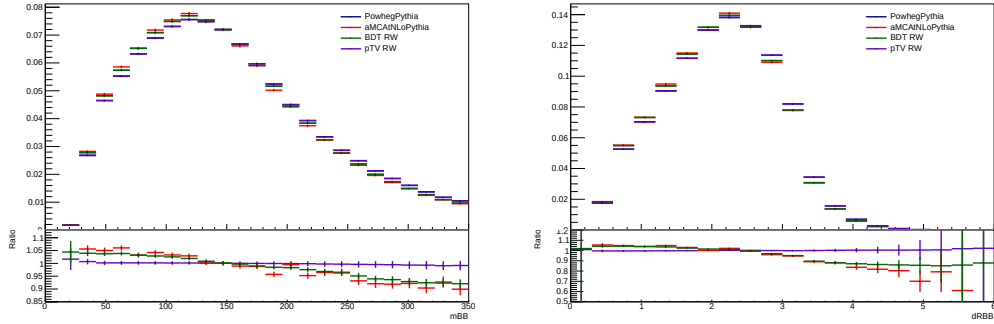
Figure G.3: The m_{b\bar{b}} and \Delta R_{b\bar{b}} distributions of the nominal POWHEG+PYTHIA8 and re-weighted samples are compared to those of the MADGRAPH5_AMC@NLO+PYTHIA8 sample in the 0-lepton channel. The p_T^V distribution is shown in blue for POWHEG+PYTHIA8 and in red for MADGRAPH5_AMC@NLO+PYTHIA8. The green graph shows POWHEG+PYTHIA8 re-weighted by the systematic variation with the multidimensional parametrization. The purple graph shows POWHEG+PYTHIA8 re-weighted by the systematic variation for p_T^V . The green graph shows agreement with MADGRAPH5_AMC@NLO+PYTHIA8.
