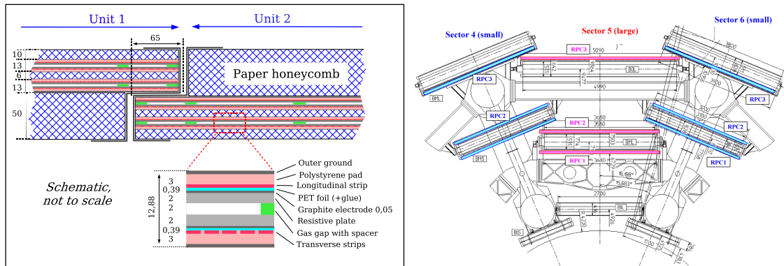
Figure 3.11: Left: Structure of an RPC layer. Right: Layout of the RPC system. The RPC is indicated with color. The middle station has two layers and the outer station has one.
