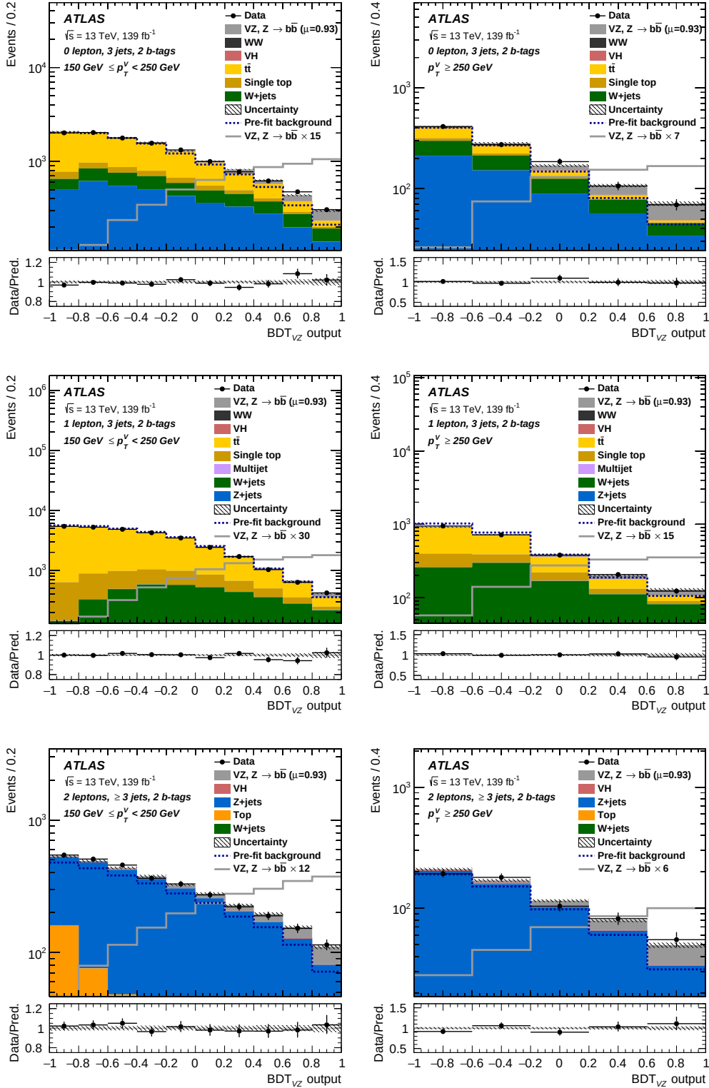
Figure I.9: The distributions of the BDT_{VZ} scores in the categories with 3 or \geq 3 jets and 150 \leq p_T^V < 250 GeV, p_T^V \geq 250 GeV of the 0-, 1- and 2-lepton channels. The stacked histograms show the prediction after the fitting. The gray unstaked and unfilled histograms show the diboson signals with the scale factors indicated in the legend. The lower panels show the ratio of the data and the prediction of the signals and the backgrounds. The hatched bands in the lower and upper panels show the total uncertainty that includes both the statistical and systematic uncertainties.
