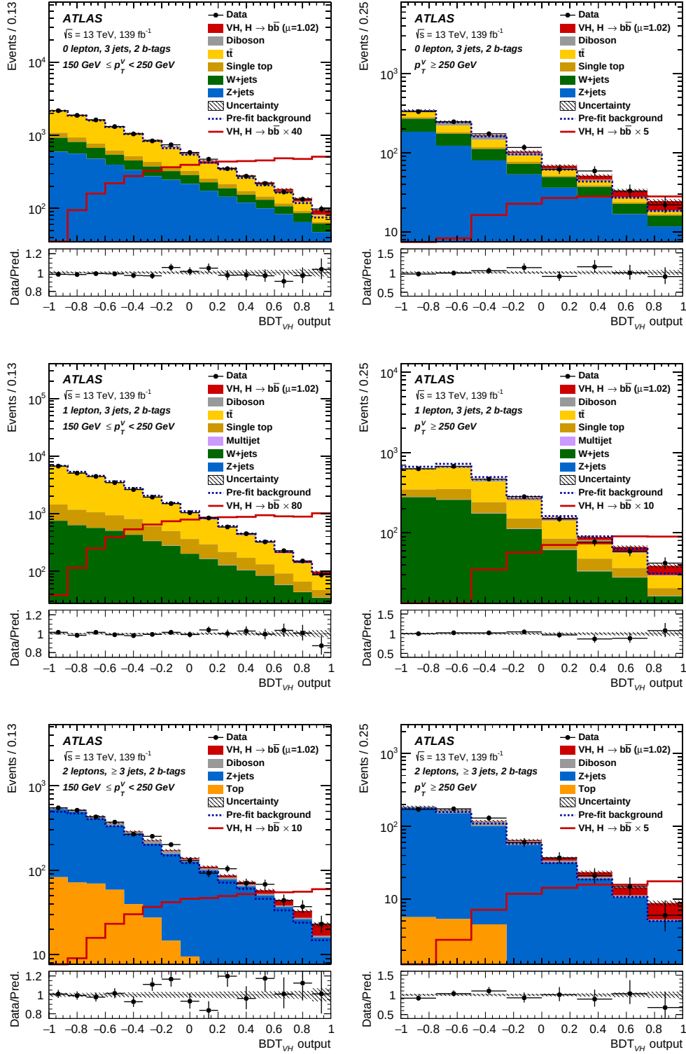
Figure I.2: The distributions of the BDT_{VH} scores in the categories with 3 or \geq 3 jets and 150 \leq p_T^V < 250 GeV, p_T^V \geq 250 GeV of the 0-, 1- and 2-lepton channels. The stacked histograms show the prediction after the fitting. The red unstacked and unfilled histograms show the VH signals with the scale factors indicated in the legend. The lower panels show the ratio of the data and the prediction of the signals and the backgrounds. The hatched bands in the lower and upper panels show the total uncertainty that includes both the statistical and systematic uncertainties.
