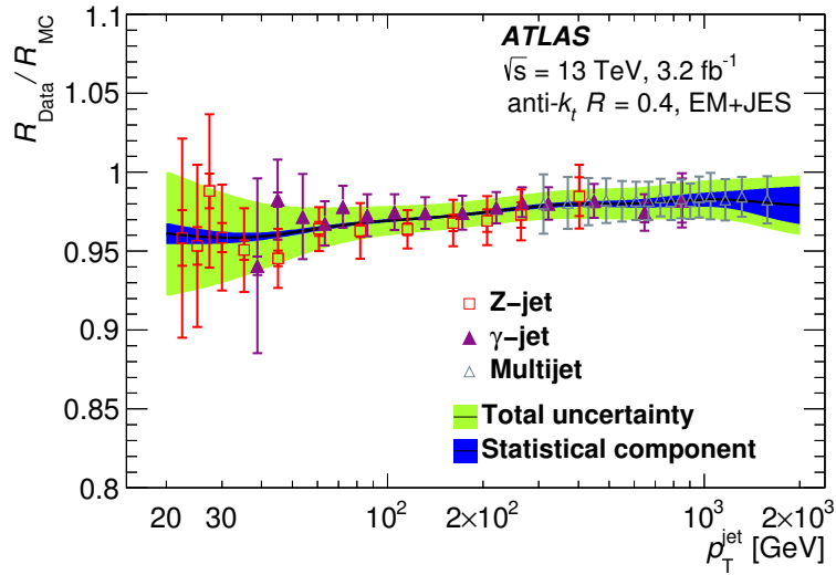
Figure 8.2: Ratio of response of the jet energy as a function of jet p_T [131]. The response is defined as R = \langle p_T^j / p_T^{\text{reference}} \rangle , where the bracket represents the statistical average. The responses derived in the in situ measurements are shown by the red ( Z +jet balance), purple ( \gamma +jet balance) and light blue (multi-jet balance) points. The combined results of the measurement is shown in the black curve, and the statistical and total uncertainties are shown as the dark blue and green area.
