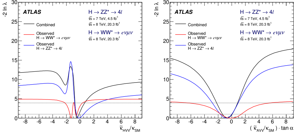
Figure 2.15: Observed scanned values of the log likelihood ratio as functions of \tilde{\kappa}_{HVV}/\kappa_{\text{SM}} and (\tilde{\kappa}_{AVV}/\kappa_{\text{SM}}) \cdot \tan \alpha derived from the analysis of the Higgs decays. The red and blue curves represent the H \rightarrow WW^* \rightarrow e\nu\mu\nu and H \rightarrow ZZ^* \rightarrow 4\ell decays, respectively. The black curve corresponds to the combination of the two decay channels assuming \tilde{\kappa}_{HZZ} = \tilde{\kappa}_{HWW} = \tilde{\kappa}_{HVV} and \tilde{\kappa}_{AZZ} = \tilde{\kappa}_{AWW} = \tilde{\kappa}_{AVV} . The 68% and 95% confidence intervals are indicated by the dotted and dotted-dashed lines indicated in the plots. The plots are taken from Ref. [22].
