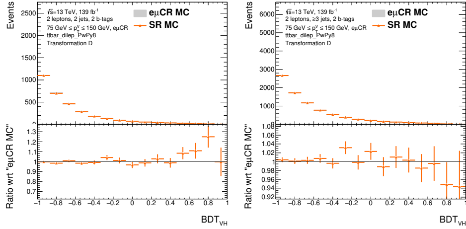
Figure 7.8: Comparison of the BDT distribution in the SR and the e\mu CR in the categories with 2 jets (left) and more than 2 jets (right) for the fully leptonic t\bar{t} events with 75 \leq p_T^V < 150 GeV.
