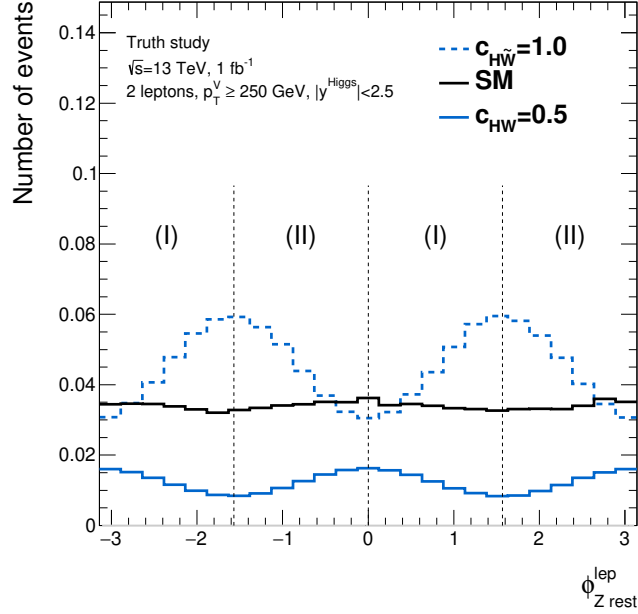
Figure 11.8: BSM terms ( |\mathcal{M}_{\text{dim-6}}|^2 ) as functions of \phi_{\text{lep}} of the ZH production with the CP-even and -odd interactions. The black histograms shows the distribution in the SM for comparison. The distributions are computed with the SMEFTsim package [51] at the LO accuracy utilizing MADGRAPH 5+PYTHIA 8 [159, 160]. These distributions are normalized using the cross-section of qq \rightarrow ZH times the branching ratios of Z \rightarrow \ell\ell and H \rightarrow b\bar{b} computed in the NNLO (QCD) and NLO (EW) prediction. The luminosity used to normalize the distributions is 1 \text{ fb}^{-1} . A cut |y^{\text{Higgs,truth}}| < 2.5 is applied.
