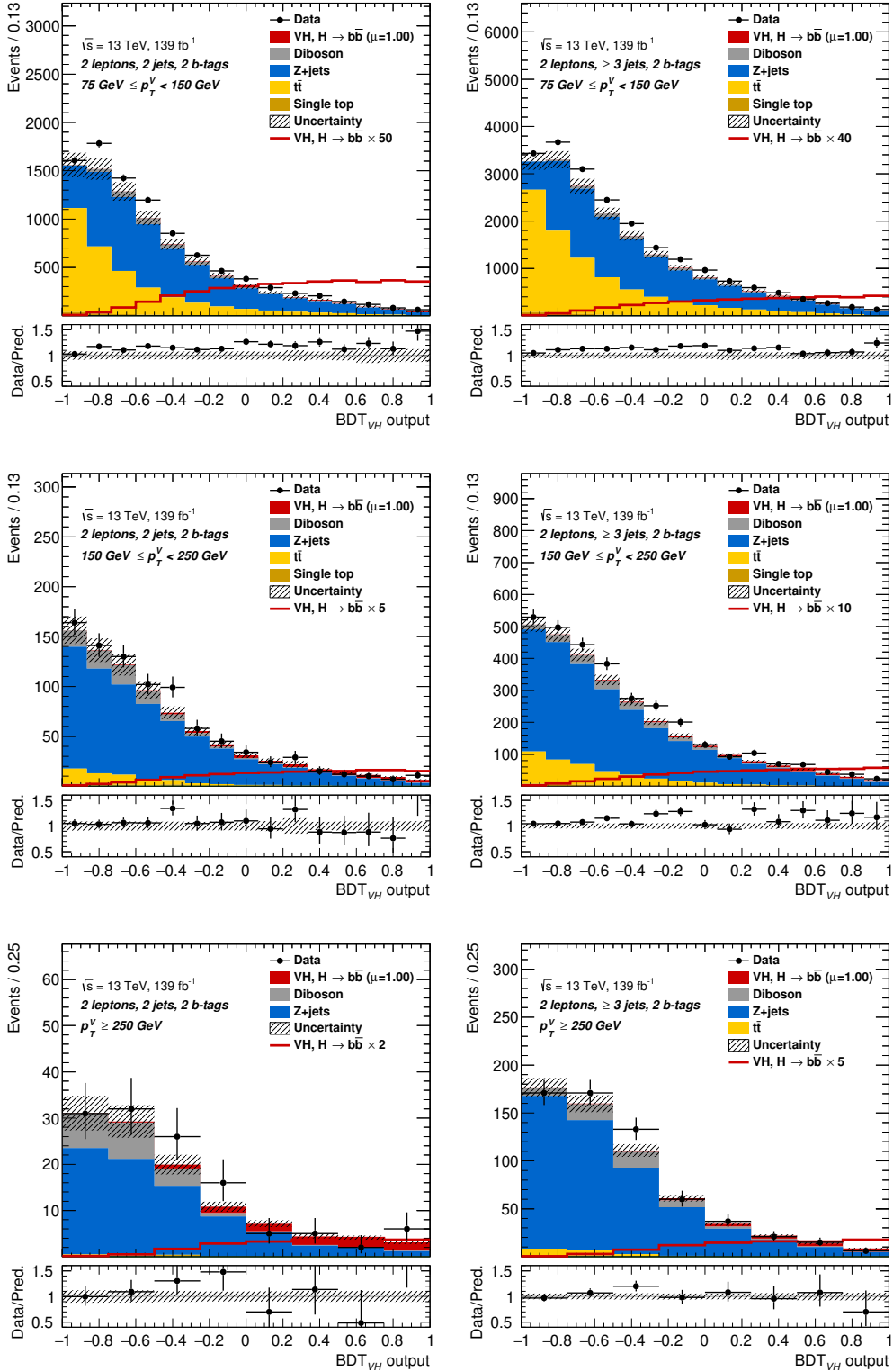
Figure 6.23: Comparisons of the data and the prediction in the distributions of \text{BDT}_{VH} in the six signal regions of the 2-lepton channel. These distributions are obtained before the fitting. The red unstaked and unfilled histograms show the Higgs signals with the scale factors indicated in the legend. The lower panels in each plot show the ratio of the data and the predictions of the signals and the backgrounds. The hatched bands in the upper and lower panels show the total uncertainty, which includes the statistical and systematic uncertainties.
