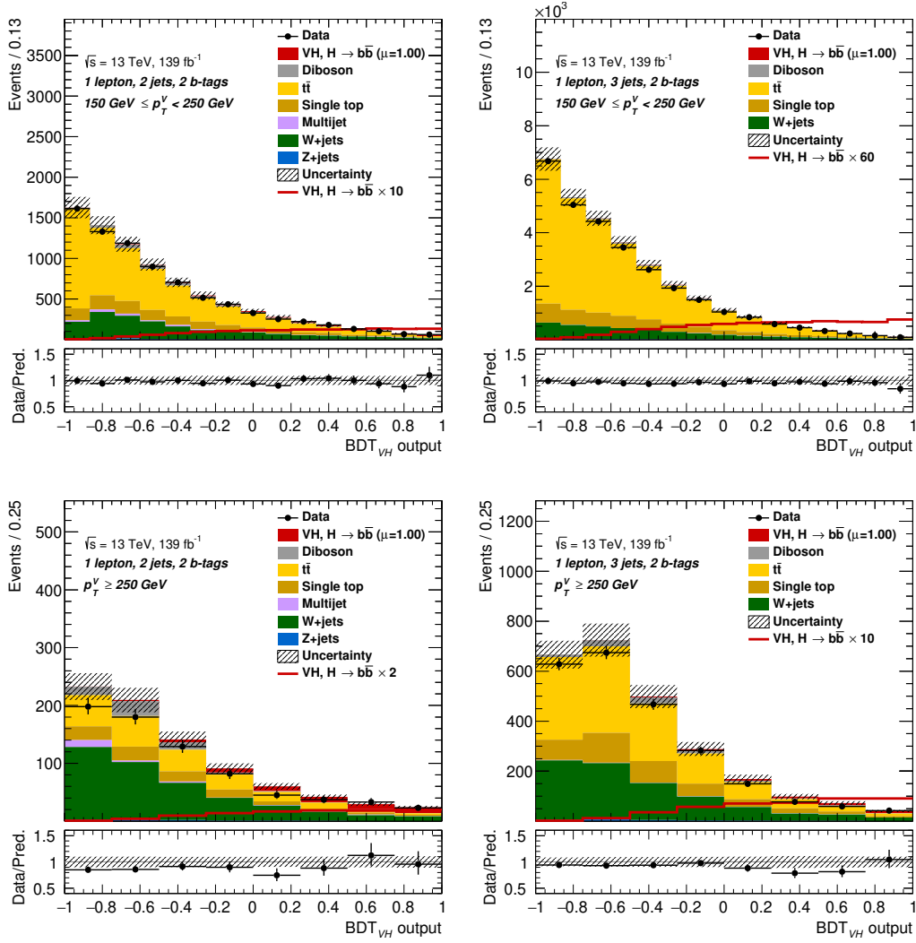
Figure 6.22: Comparisons of the data and the prediction in the distributions of \text{BDT}_{VH} in the four signal regions of the 1-lepton channel. These distributions are obtained before the fitting. The red unstacked and unfilled histograms show the Higgs signals with the scale factors indicated in the legend. The lower panels in each plot show the ratio of the data and the predictions of the signals and the backgrounds. The hatched bands in the upper and lower panels show the total uncertainty, which includes the statistical and systematic uncertainties.
