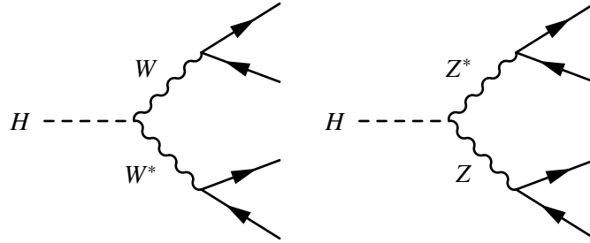
Figure 2.7: Higgs decays to a pair of vector bosons
