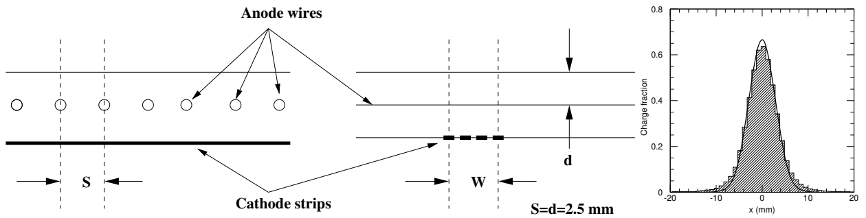
Figure 3.15: Left: Structure of anode wires and cathode strips in a CSC gas gap. Right: Charge distribution induced on the CSC cathode.
