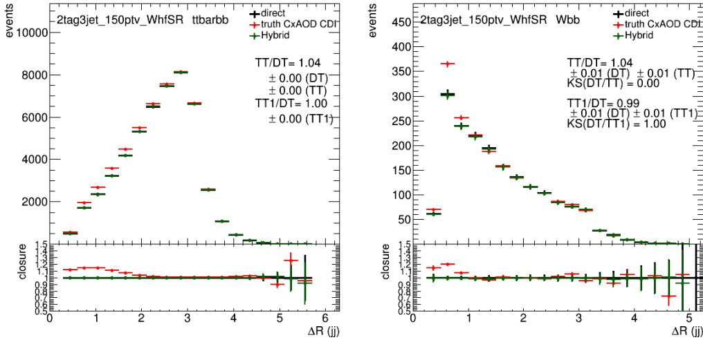
Figure B.1: \Delta R_{b\bar{b}} distributions for t\bar{t} (left) and W + b\bar{b} (right) events with the direct b -tagging (black), the truth b -tagging (red) and the hybrid truth b -tagging (green). The study is performed with events with one charged lepton (more precisely, a signal region of a 1-lepton channel defined in Section 6.3), one non- b -jet in addition to two b -jets and the reconstructed p_T^{\ell + E_T^{\text{miss}}} greater than 150 GeV are used in these plots. The plots in the bottom panes show the ratio of each method to the direct b -tagging. Non-closure is observed for the truth b -tagging, and the closure is recovered by the hybrid truth b -tagging.
