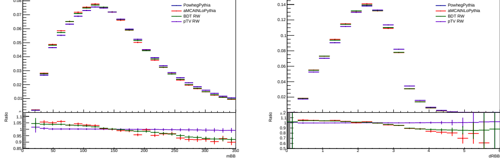
Figure G.2: The m_{b\bar{b}} and \Delta R_{b\bar{b}} distributions of the nominal POWHEG+PYTHIA8 and re-weighted samples are compared to those of the MADGRAPH5_AMC@NLO+PYTHIA8 sample in the 1-lepton channel. The p_T^V distribution is shown in blue for POWHEG+PYTHIA8 and in red for MADGRAPH5_AMC@NLO+PYTHIA8. The green graph shows POWHEG+PYTHIA8 re-weighted by the systematic variation with the multidimensional parametrization. The purple graph shows POWHEG+PYTHIA8 re-weighted by the systematic variation for p_T^V . The green graph shows agreement with MADGRAPH5_AMC@NLO+PYTHIA8.
