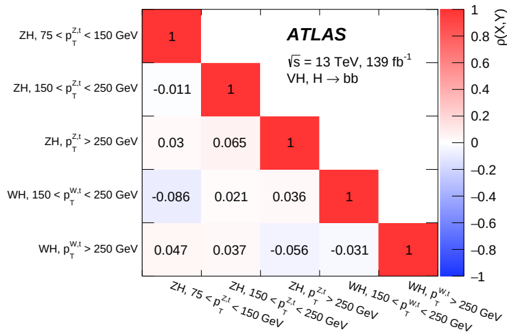
Figure I.11: Correlations of the Measured cross sections of the VH production ( \sigma ) times the branching ratio of the V \rightarrow \text{leptons} and H \rightarrow b\bar{b} decays ( B ). The \sigma \times B values are unfolded to the indicated bins.
