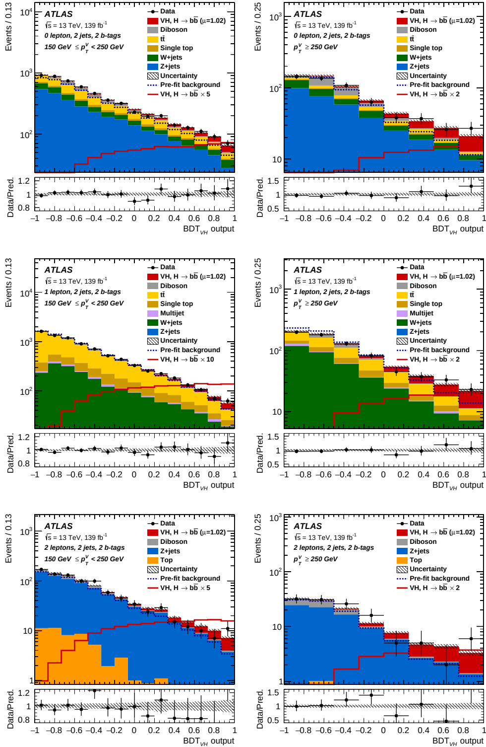
Figure 10.1: The distributions of the BDT_{VH} scores in the categories with 2 jets and 150 \leq p_T^V < 250 GeV, p_T^V \geq 250 GeV of the 0-, 1- and 2-lepton channels. The stacked histograms show the prediction after the fitting. The red unstacked and unfilled histograms show the VH signals with the scale factors indicated in the legend. The lower panels show the ratio of the data and the prediction of the signals and the backgrounds. The hatched bands in the lower and upper panels show the total uncertainty that includes both the statistical and systematic uncertainties.
