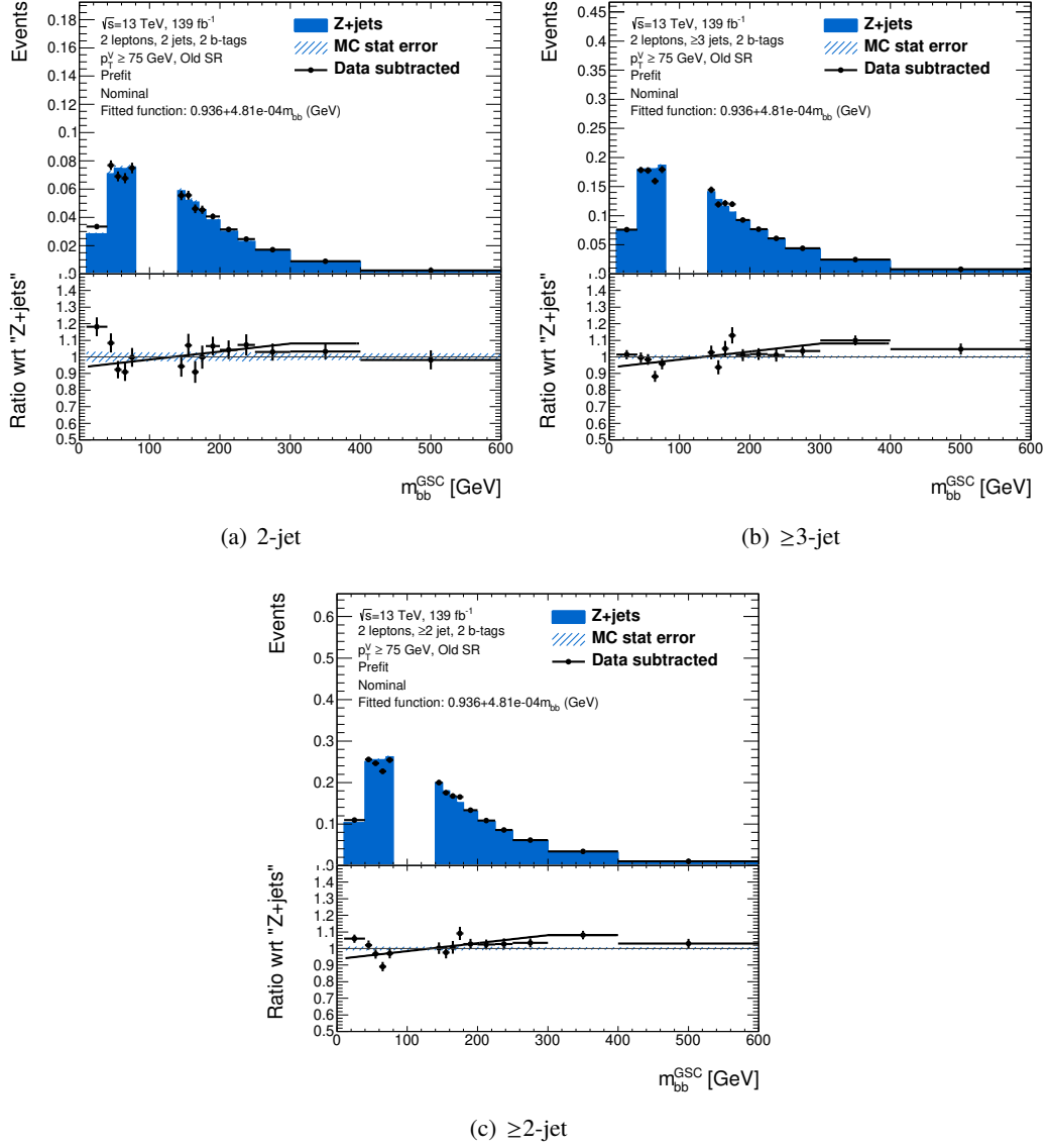
Figure G.9: Comparison of the SHERPA sample and the data after the subtraction of the data from the e\mu control region and the non-Z + jets MC backgrounds in the m_{b\bar{b}} distributions. The black curves in the bottom panes represent a function fitted to the ratio in the \geq 2 -jet region, and defines the m_{b\bar{b}} shape uncertainty. The analytic expression is 0.936 + 0.000481m_{b\bar{b}} as also indicated in the plots.
