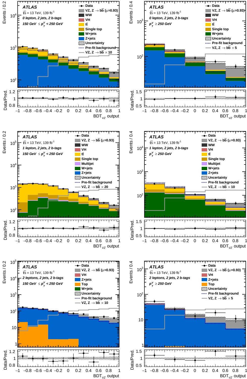
Figure 10.4: Distributions of the BDT_{VZ} scores for the prediction and the data in the categories with 2 jets and 150 \leq p_T^V < 250 GeV, p_T^V \geq 250 GeV of the 0-, 1- and 2-lepton channels. The stacked histograms show the prediction after the fitting. The gray unstacked and unfilled histograms show the diboson signals with the scale factors indicated in the legend. The lower panels show the ratio of the data and the prediction of the signals and the backgrounds. The hatched bands in the lower and upper panels show the total uncertainty that includes both the statistical and systematic uncertainties.
