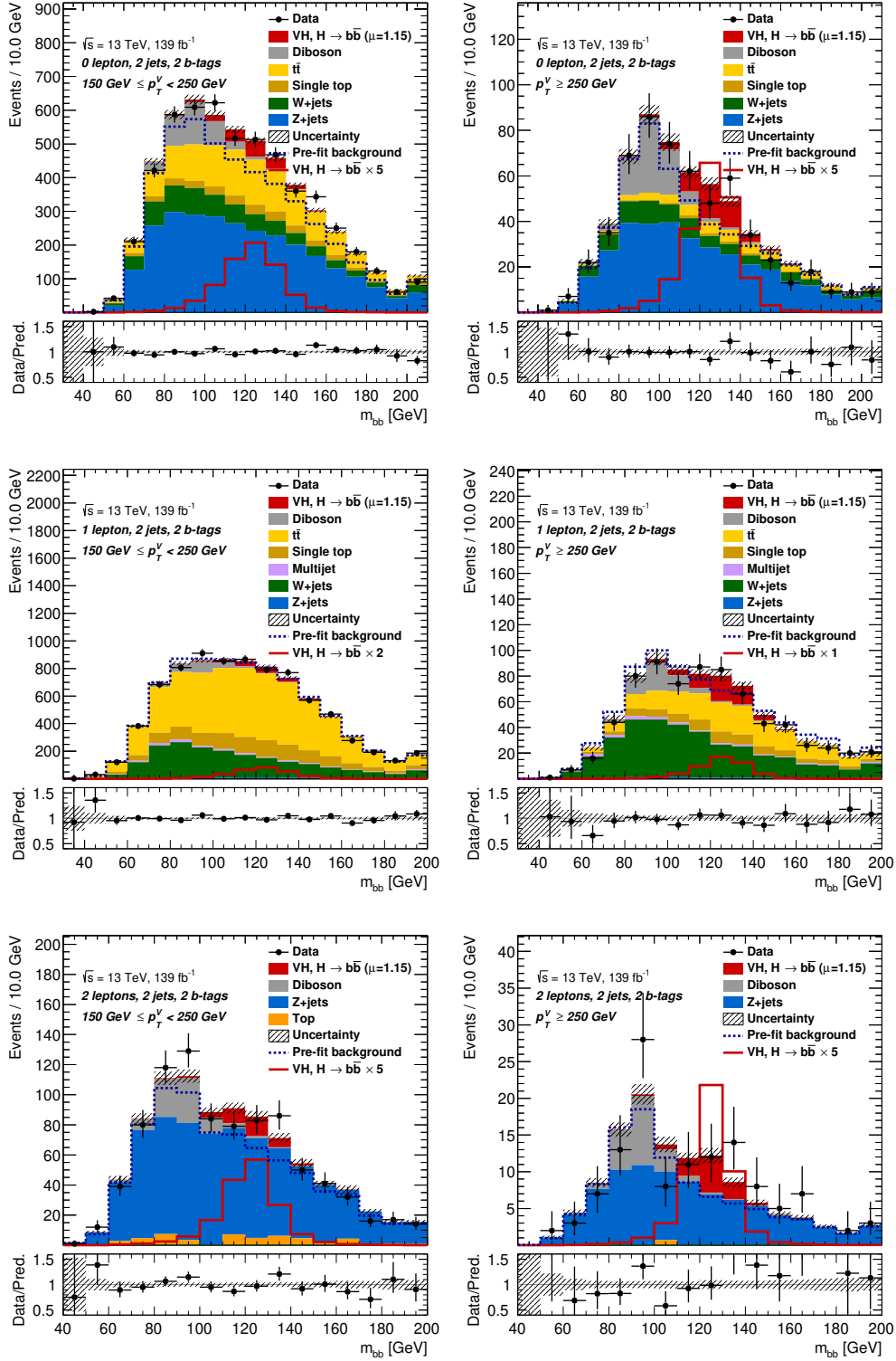
Figure 10.6: Distributions of the m_{b\bar{b}} in the categories with 2 jets and 150 \leq p_T^V < 250 GeV, p_T^V \geq 250 GeV of the 0-,1- and 2-lepton channels. The stacked histograms show the prediction after the fitting. The red unstaked and unfilled histograms show the VH signals with the scale factors indicated in the legend. The lower panels show the ratio of the data and the prediction of the signals and the backgrounds. The hatched bands in the lower and upper panels show the total uncertainty that includes both the statistical and systematic uncertainties.
