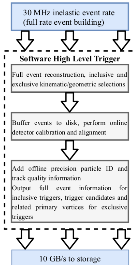
Figure 2.8: LHCb upgrade trigger diagram.
