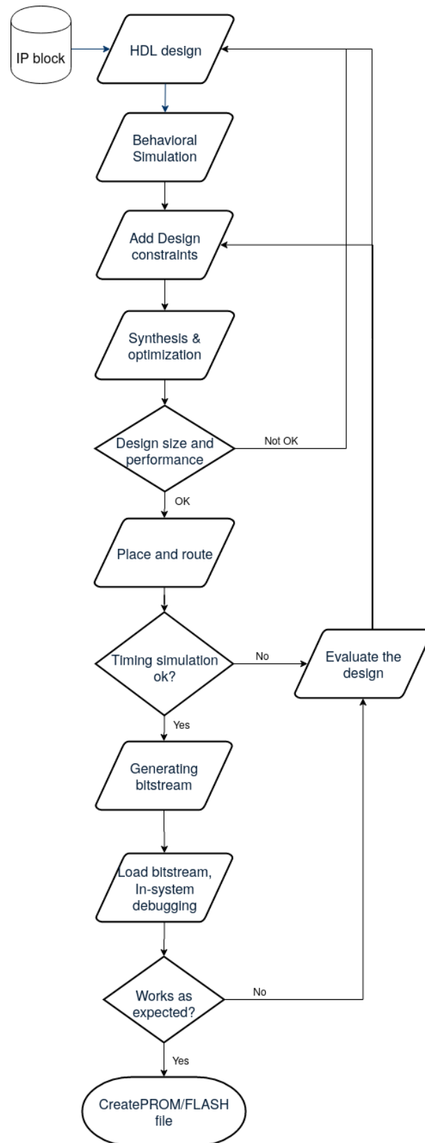
Figure 5.2: FPGA design flow.
