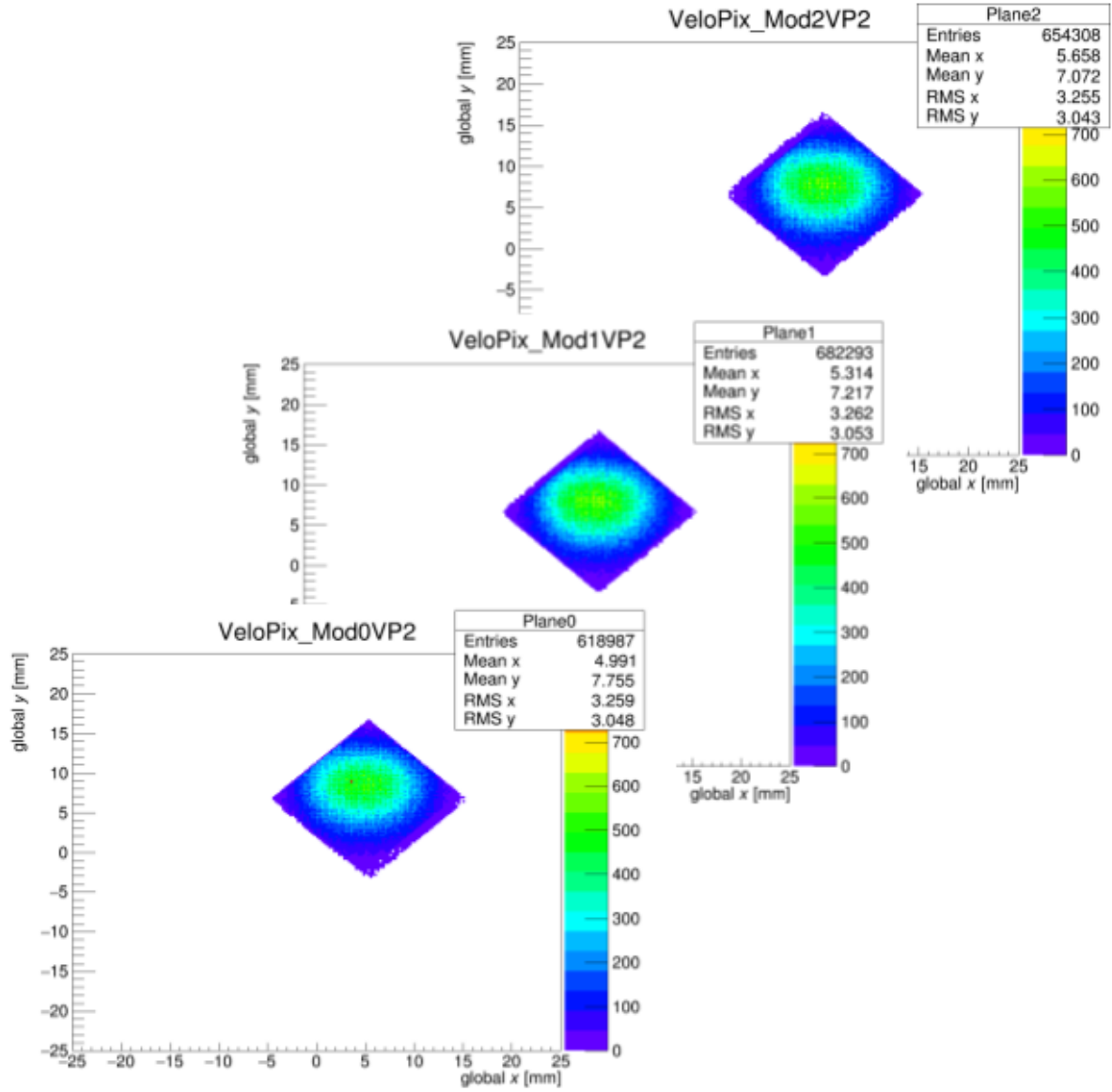
Figure 5.16: Preliminary VELO telescope data.
