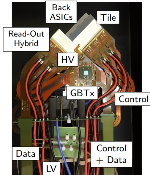
Figure 3.12: VELO module.
