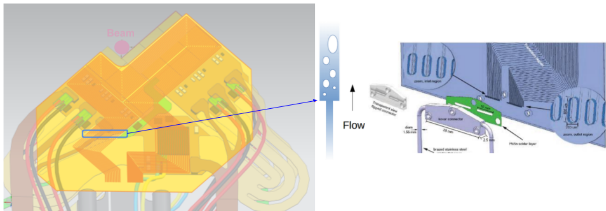
Figure 3.13: (Left) Cross section scheme for the microchannel cooling with a superposition of the VeloPix ASICs. (Right) Schematic of the microchannel attachment of the fluidic connector.
