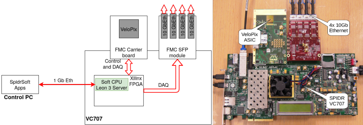
Figure 5.3: SPIDR readout system.
