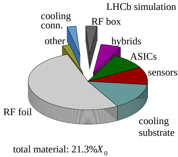
Figure 3.15: Pie chart showing the contributions from different components to the total material budget in the upgraded VELO within the pseudorapidity angles 0.8^\circ and 15.4^\circ .
