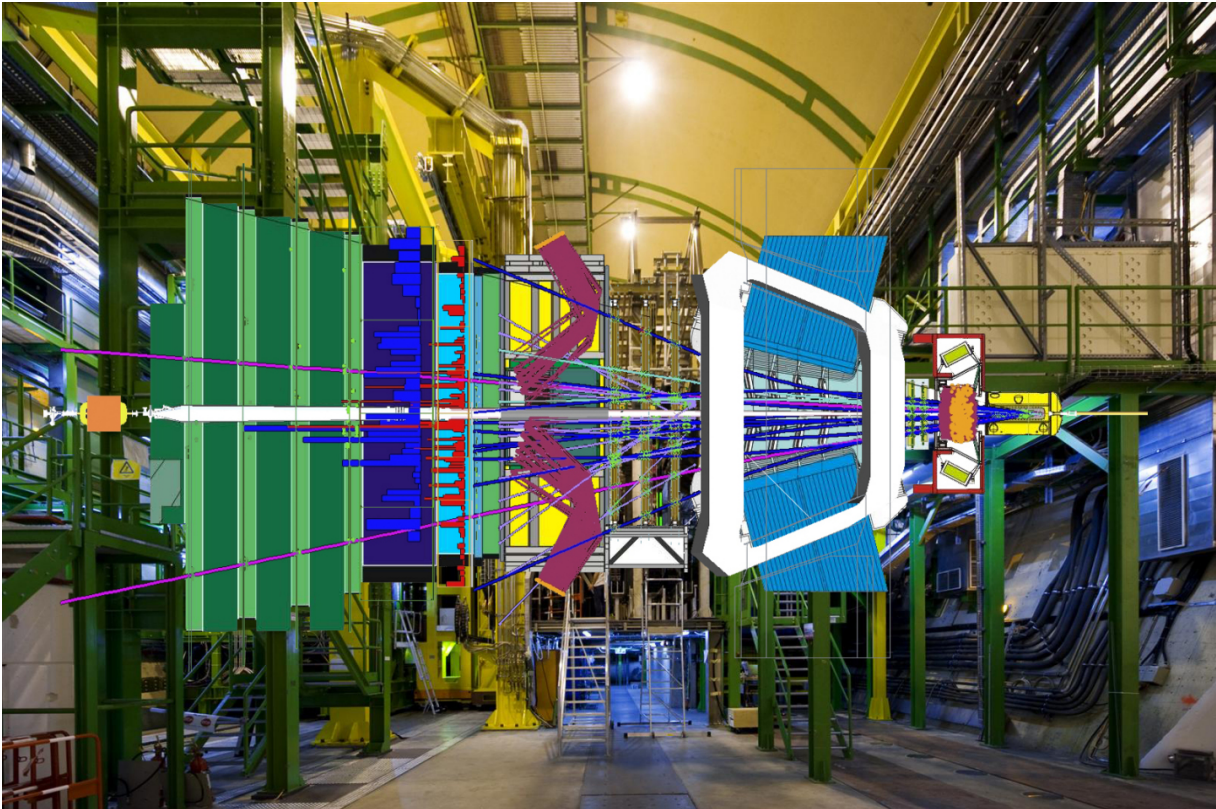
Figure 2.4: LHCb detector.
