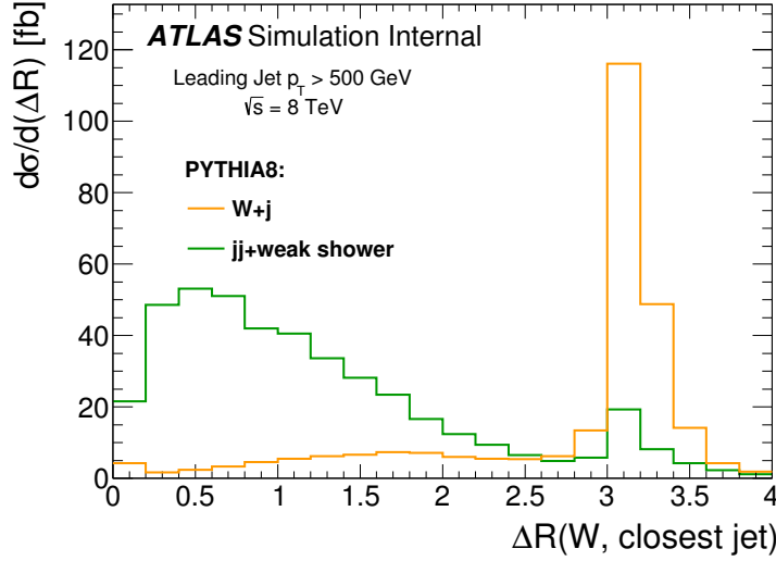
Figure 2.8: Differential cross-section for the angular separation between the W boson and the closest jet for W + 1 -jet production (orange) and QCD dijet production with electroweak parton showering (green), as calculated by PYTHIA. Events are required to have a jet with p_T > 500 GeV.
