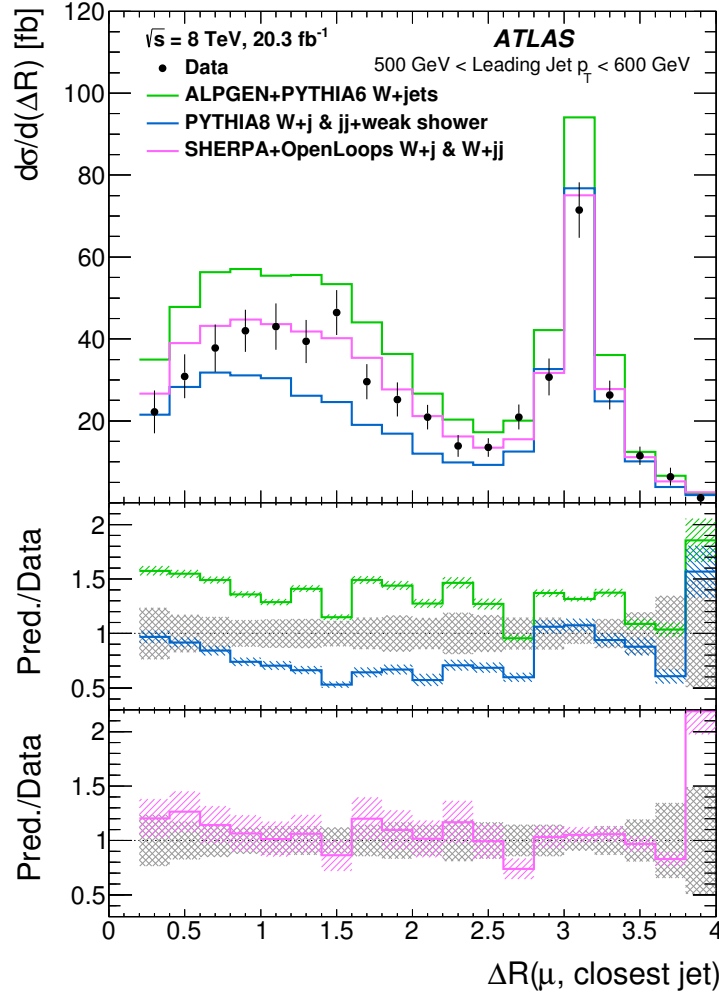
Figure 7.11: Differential cross-section of W(\rightarrow \mu\nu) + \geq 1 jet as a function of the angular separation between the muon and the closest jet as measured in data for 500 \text{ GeV} < p_{\text{T}}^{\text{leading jet}} < 600 \text{ GeV} , along with several predictions from theory calculations. The lower panels show the ratio of the theory predictions to the measurement from data. The error bars in the upper panel and the grey shaded error bands in the lower ratio panels are the sum of the statistical and systematic uncertainties in the measurement. The shaded error band on the ALPGEN+PYTHIA6 calculation is statistical uncertainty, the band on the PYTHIA8 calculation is statistical and PDF uncertainties and the band on the SHERPA+OpenLoops calculation is scale uncertainty.
