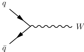
Figure 2.3: Feynman diagram for leading-order W boson production.
