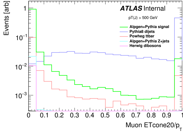
Figure 5.6: Predicted distributions from MC simulation of calorimeter isolation energy for the signal and background processes. Calorimeter isolation energy is defined as the scalar sum of the p_T in all calorimeter cells in a cone of radius \Delta R = 0.2 around the muon divided by the muon p_T . Here the baseline event selections are applied. The signal and total background are both normalized to unity. The rightmost histogram bin includes overflow values that are larger than the axis range of the plot.
