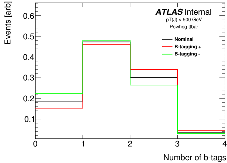
Figure 6.5: The effect of the uncertainty in the b -tagging efficiency and inefficiency on the number of b -tags in simulated t\bar{t} events. The black represents the nominal efficiencies, and the red and green represents a \pm 1\sigma shift. The signal region selection, except for the requirement on the number of b -tags, has been applied.
