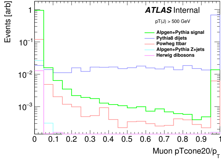
Figure 5.5: Predicted distributions from MC simulation of track isolation energy for the signal and background processes. Track isolation energy is defined as the scalar sum of the p_T of all tracks with p_T > 1 GeV in a cone of radius \Delta R = 0.2 around the muon divided by the muon p_T . Here the baseline event selections are applied. The signal and total background are both normalized to unity. The rightmost histogram bin includes overflow values that are larger than the axis range of the plot.
