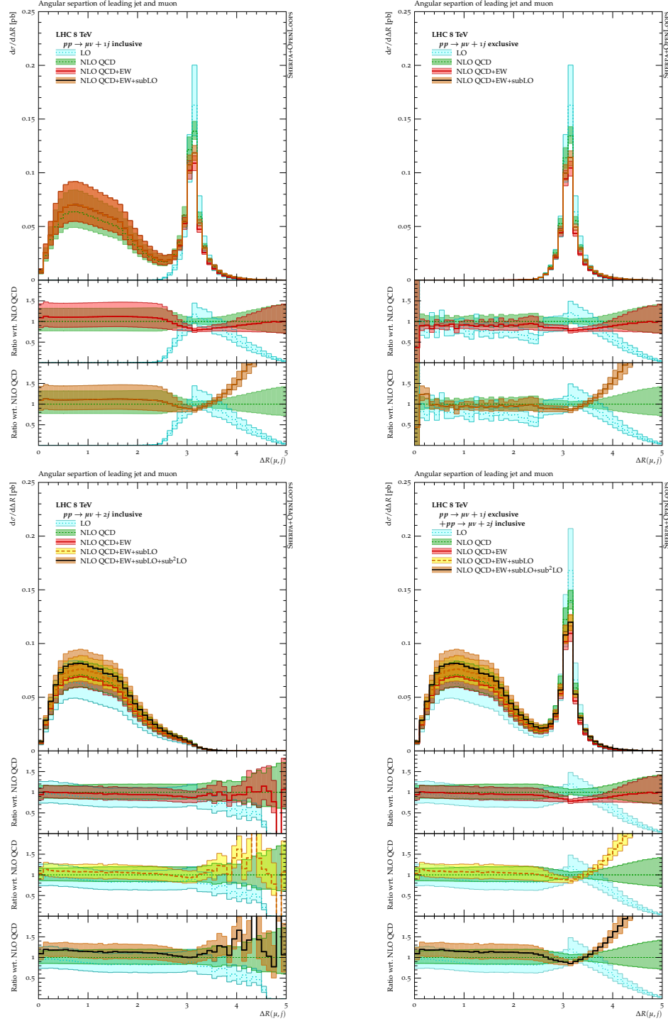
Figure 2.9: Differential cross-section for the angular separation between the muon and the closest jet for W + 1 -jet inclusive (upper left), W + 1 -jet exclusive (upper right), W + 2 -jet inclusive (lower left) and the exclusive sums combination of W + 1 -jet and W + 2 -jet (lower right), as calculated by SHERPA+OpenLoops. The NLO QCD and NLO EW corrections are shown in the lower panels. Events are required to have a jet with p_T > 500 GeV. The shaded bands represent the scale uncertainties. Source: [43]
