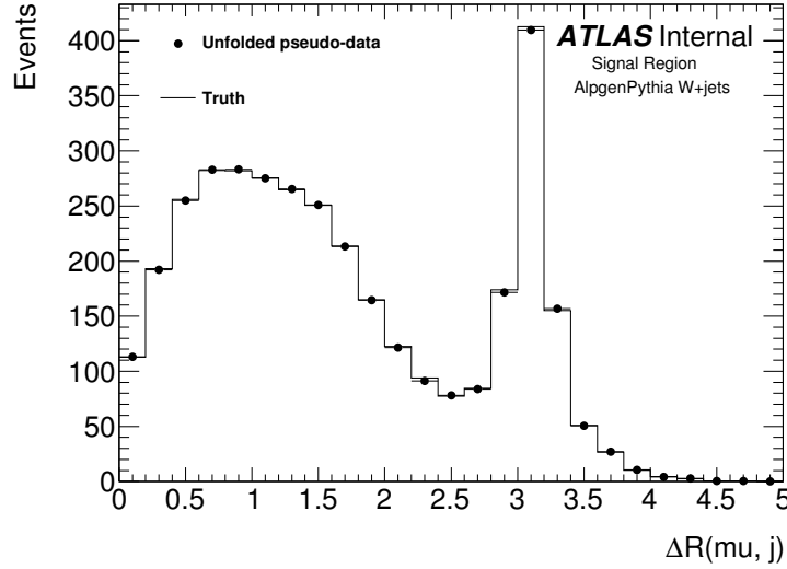
Figure A.2: Distributions of \Delta R from unfolded pseudo-data, where the pseudo-data is taken from simulated W + \text{jets} events, and from MC truth. The error bars shown here are not the statistical uncertainty in the psuedo-data, but the uncertainty due to the finite number of MC toys used in the unfolding.
