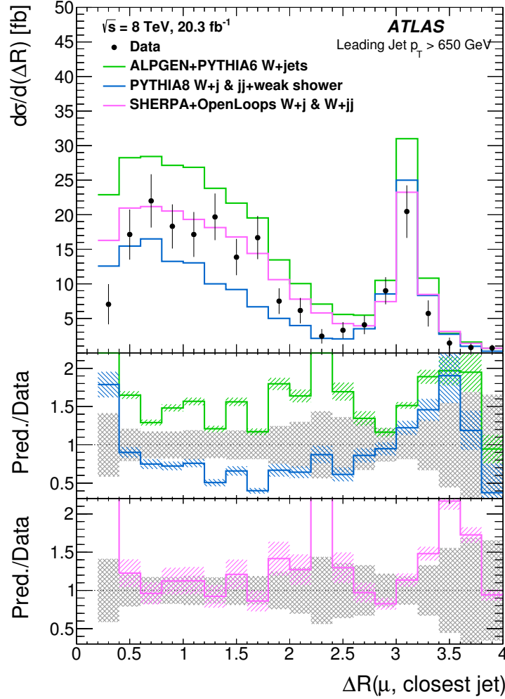
Figure 7.12: Differential cross-section of W(\rightarrow \mu\nu) + \geq 1 jet as a function of the angular separation between the muon and the closest jet as measured in data for p_{\text{T}}^{\text{leading jet}} > 650 GeV, along with several predictions from theory calculations. The lower panels show the ratio of the theory predictions to the measurement from data. The error bars in the upper panel and the grey shaded error bands in the lower ratio panels are the sum of the statistical and systematic uncertainties in the measurement. The shaded error band on the ALPGEN+PYTHIA6 calculation is statistical uncertainty, the band on the PYTHIA8 calculation is statistical and PDF uncertainties and the band on the SHERPA+OpenLoops calculation is scale uncertainty.
