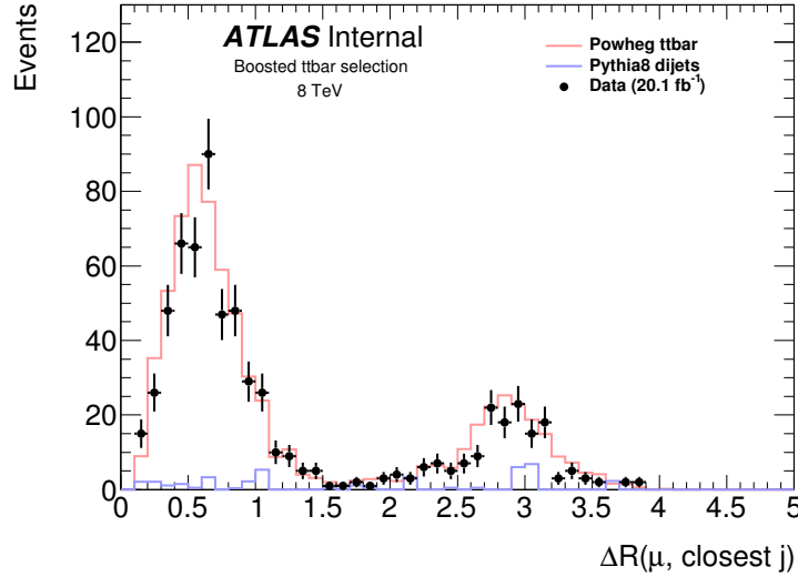
Figure A.1: Distribution of the angular separation between the muon and the closest jet in events from data and from simulated MC samples using the boosted t\bar{t} selection of Appendix A.1.
