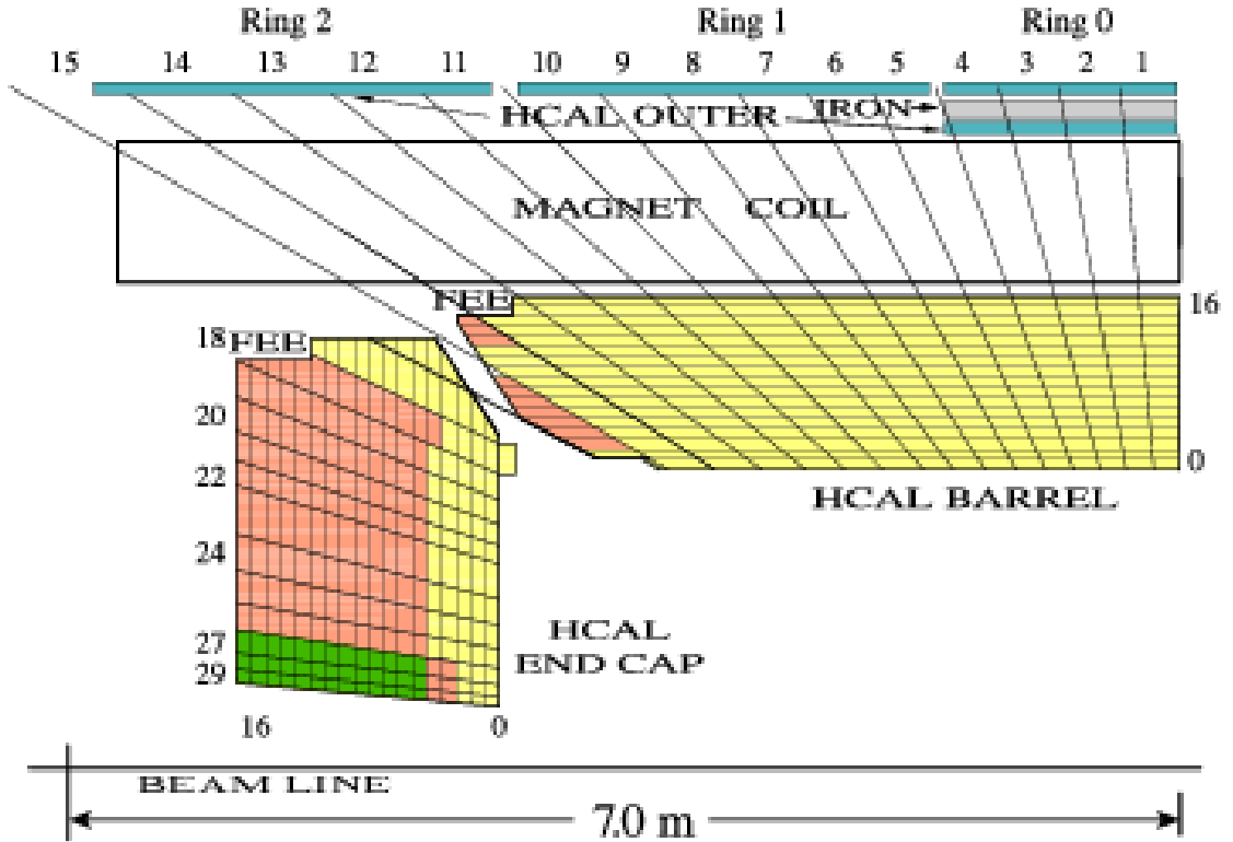
Figure 4.5: A schematic diagram of the CMS HCAL[24].
