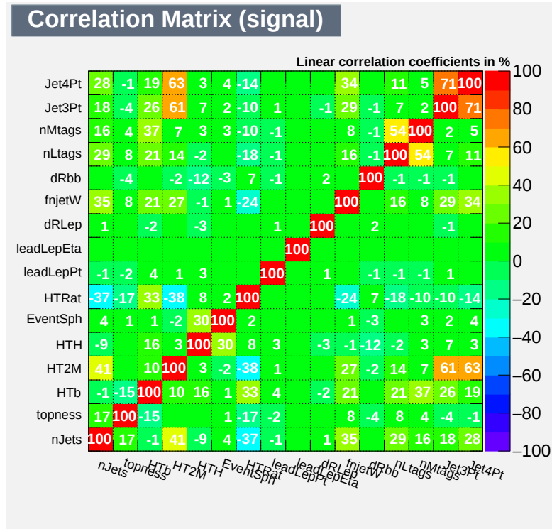
Figure 9.12: Correlation Matrix of BDT variables after training for Signal.
