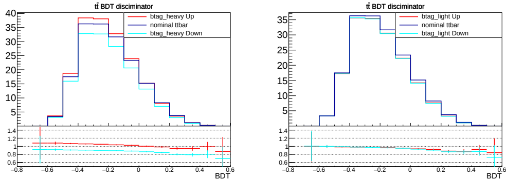
Figure D.1: Heavy (left) and Light (right) btagging uncertainties (up/down) on the BDT classifier distributions from t\bar{t} samples.
