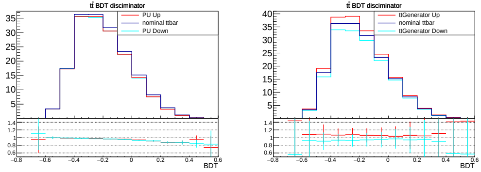
Figure D.3: PU (left) and Generator Choice (right) uncertainties (up/down) on the BDT classifier distributions from t\bar{t} samples.
