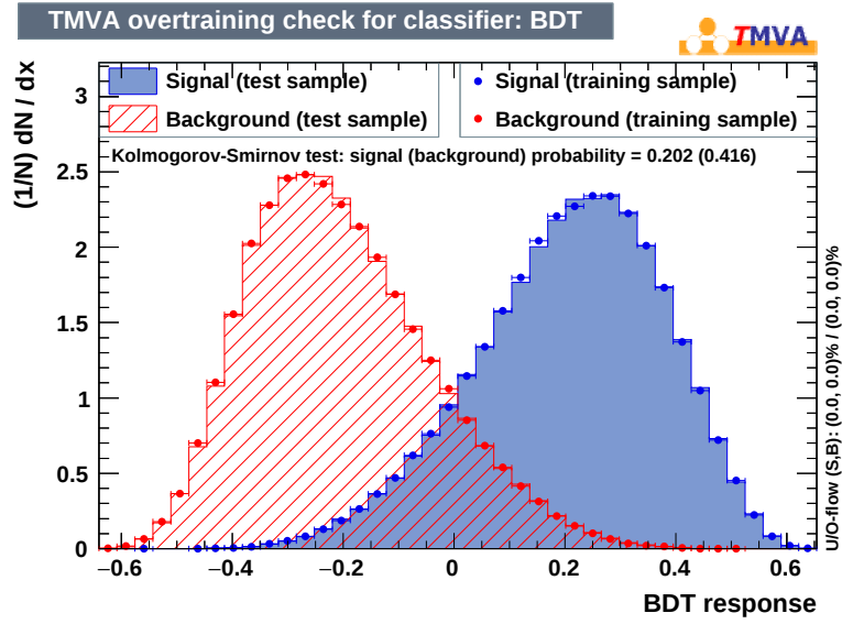
Figure 9.11: Classifier response for the trained BDT.
