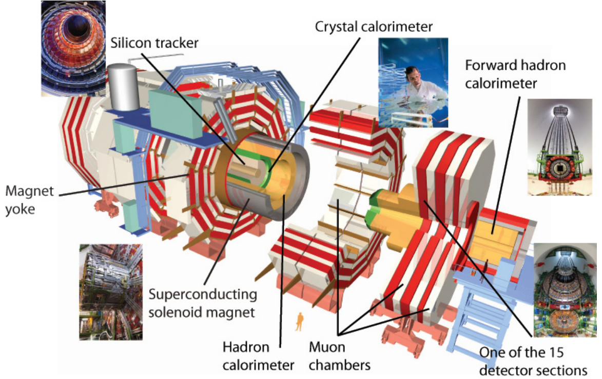
Figure 4.1: The Compact Muon Solenoid.
