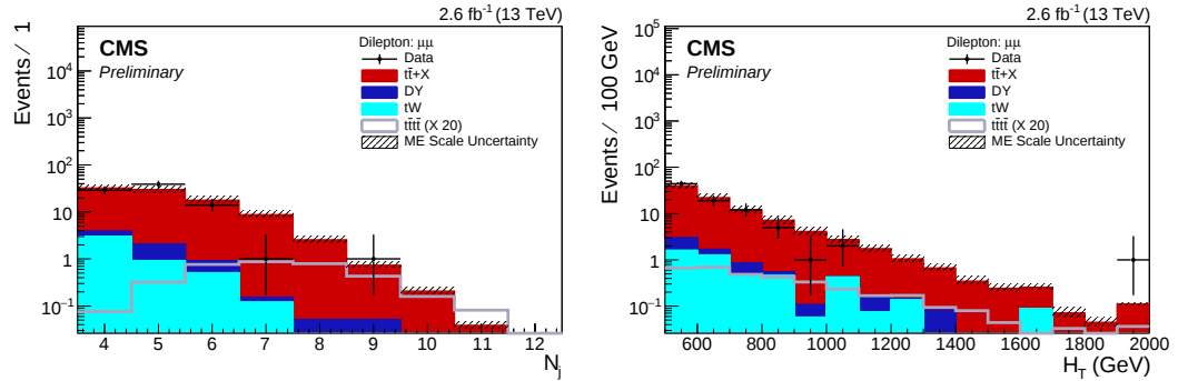
Figure 8.1: Number of jets (left) and the scalar sum of transverse jet energy (right) for the \mu\mu channel.
