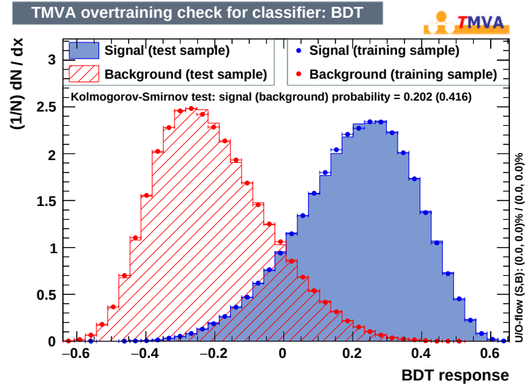
Figure 9.11: Classifier response for the trained BDT.
