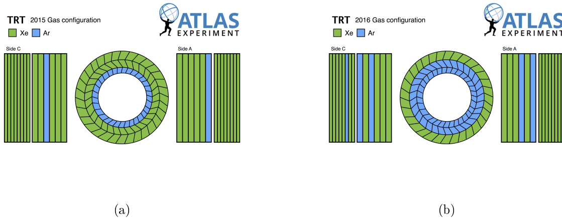
Figure 2.7: TRT gas configuration used in the year (a) 2015 and (b) 2016.
