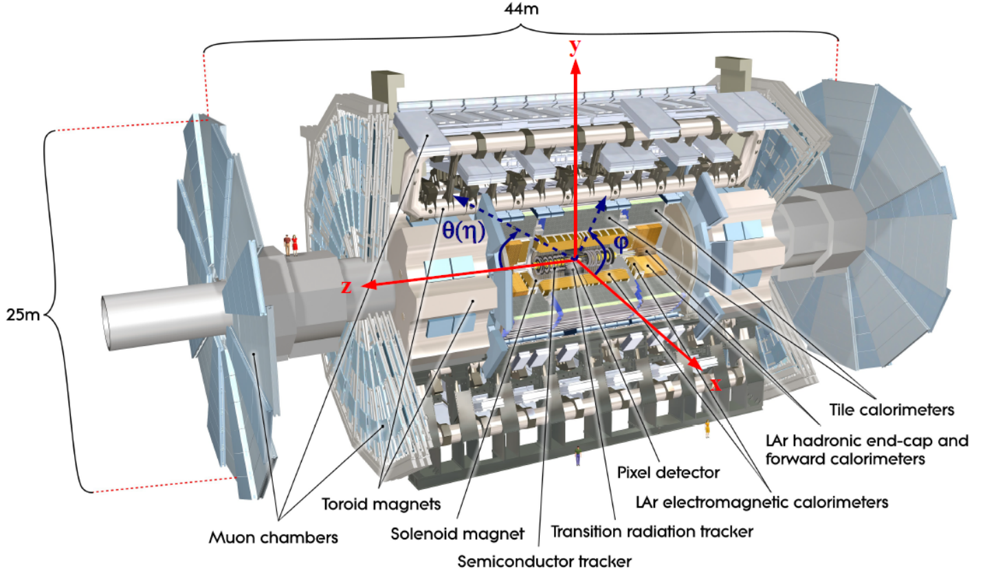
Figure 2.4: View of the ATLAS detector along with the coordinate system.
