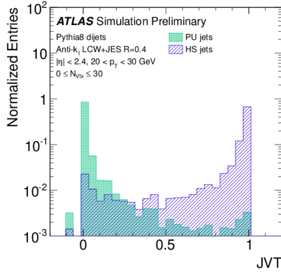
Figure 4.14: JVT distribution for hard-scatter jets (blue shaded histogram) and pileup jets (green histogram) with 20 < p_T < 30 GeV and |\eta| < 2.4 in simulated dijet events. From Ref. [158].
