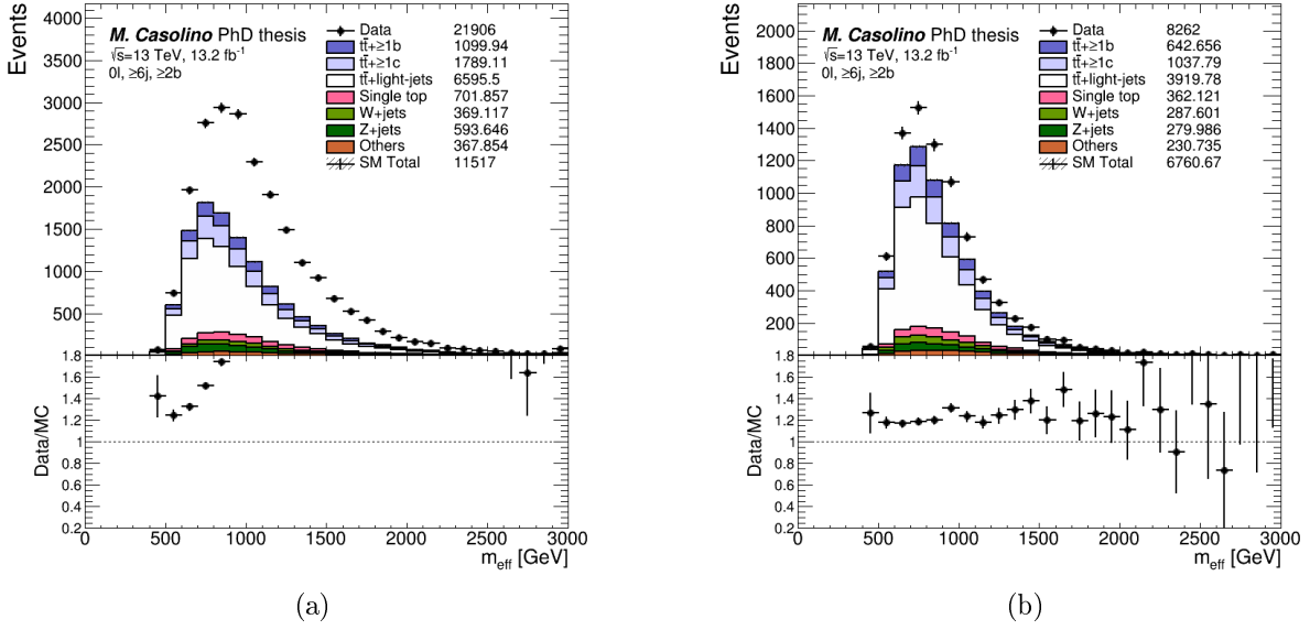
Figure 6.2: m_{\text{eff}} distribution (a) before and (b) after the \Delta\phi_{\min}^{4j} > 0.4 cut.
