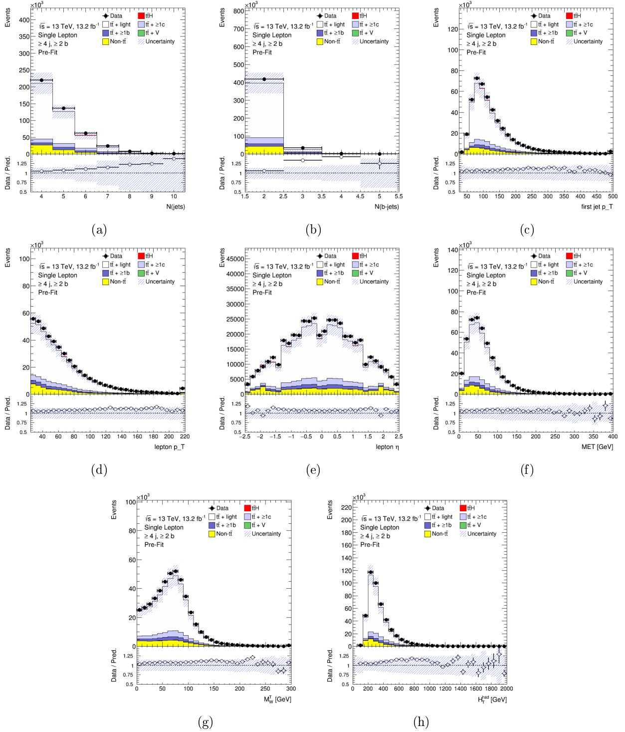
Figure 7.1: Comparison between data and prediction in at the preselection level in the tt\bar{H} search for (a) jet multiplicity, (b) b -tag multiplicity, (c) leading jet p_T , (d) lepton p_T , (e) lepton \eta , (f) E_T^{\text{miss}} , (g) transverse mass of the W boson ( m_T^W ), and (h) scalar sum of jet p_T ( H_T^{\text{had}} ). The hashed area represents the total uncertainty on the background.
