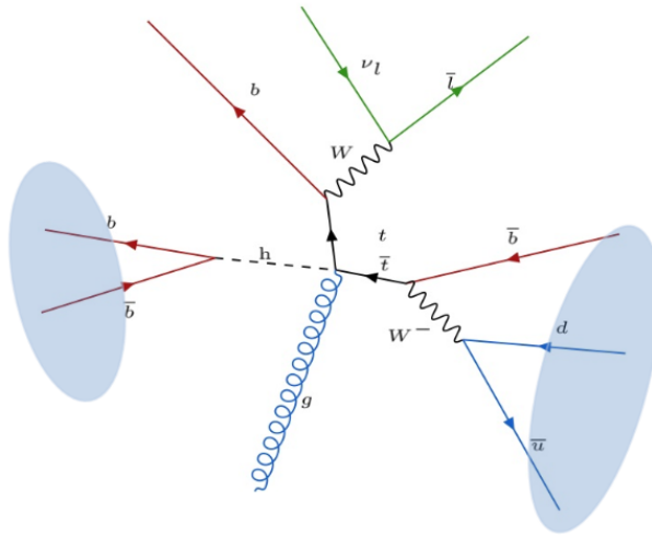
Figure 7.16: Sketch of boosted t\bar{t}H event in which the Higgs and the hadronic top are reconstructed as large- R jets. From reference [256].
