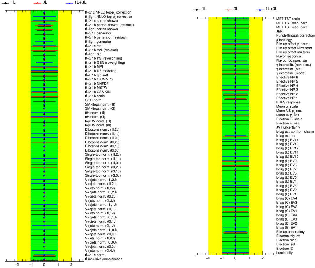
Figure 6.15: Fitted NPs from a fit to the Asimov dataset under the background-only hypothesis. Shown are the fits using the 1-lepton channel only (black), 0-lepton channel only (red), and the combination of both channels (blue). A detailed description of the naming of the NPs can be found in appendix B.
