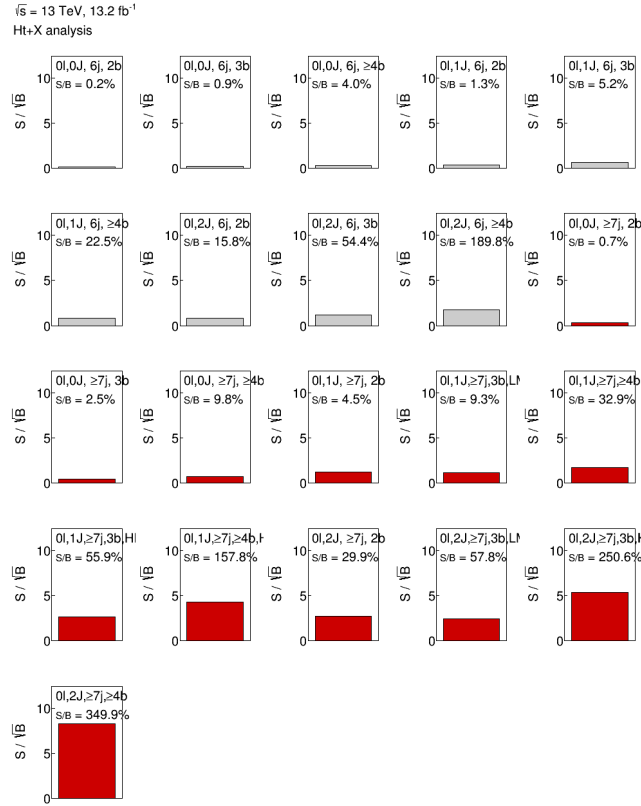
Figure 6.11: S/B and S/\sqrt{B} in the 0-lepton regions. The search (validation) regions are highlighted in red (grey). The signal assumed is T\bar{T} production in the weak-isospin doublet and m_T = 0.8 \text{ TeV} .
