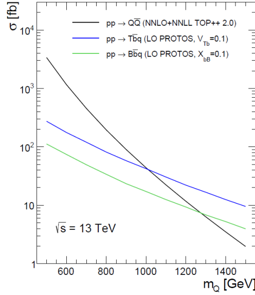
Figure 1.12: Production cross sections for pair and single production of VLQs in pp collisions at \sqrt{s}=13 TeV. Pair production is computed at NNLO+NNLL order in QCD using TOP++ 2.0 while single production is computed at LO in QCD with PROTOS assuming V_{Tb} = 0.1 and X_{bB} = 0.1 .
