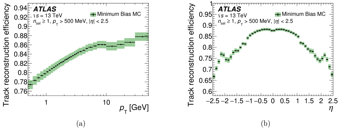
Figure 4.2: The track reconstruction efficiency as a function of (a) p_T and (b) \eta as estimated in simulated minimum bias events. The statistical uncertainties are shown as black vertical bars, the combination of statistical and systematic uncertainties as green shaded areas. From reference [144].
