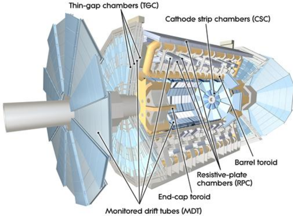
Figure 2.10: Schematic view of the ATLAS muon spectrometer.
