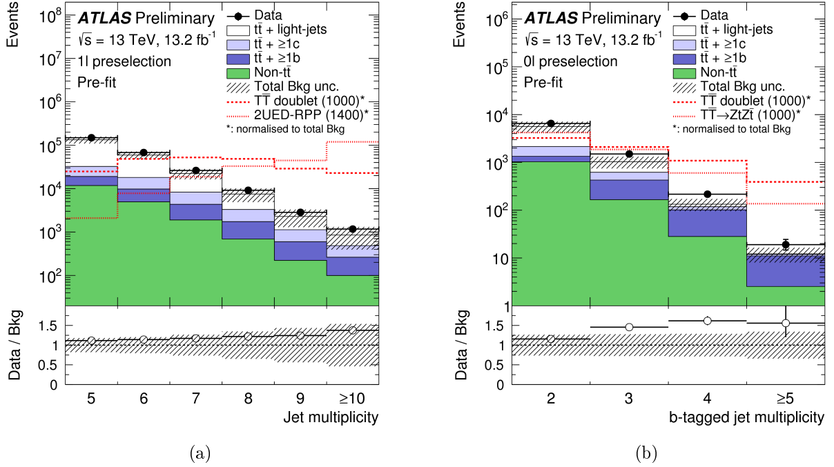
Figure 6.5: Comparison between data and prediction before performing the fit to data for (a) the jet multiplicity in 1-lepton channel and (b) the b -tag multiplicity in 0-lepton channel. The small contributions from t\bar{t}V , t\bar{t}H , single top, W/Z +jets, diboson, and multijet backgrounds are combined into a single background source referred to as “Non- t\bar{t} ”. The expected signal distributions are shown, normalised to the total background prediction, for three scenarios considered in this search: T\bar{T} production in the weak-isospin doublet scenario and for \text{BR}(T \rightarrow Zt) = 1 assuming m_T = 1000 GeV (red dashed and continuous histogram respectively), and t\bar{t}t\bar{t} production within the 2UED/RPP model assuming m_{KK} = 1400 GeV (red dotted histogram). The last bin in all figures contains the overflow. The normalisation uncertainty on the t\bar{t} + \geq 1b background is not included in the background uncertainty band.
