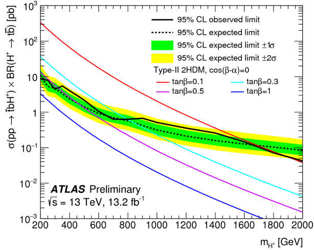
Figure 6.32: Observed (solid line) and expected (dashed line) 95% CL upper limits on \sigma(pp \rightarrow t\bar{b}H^+) \times \text{BR}(H^+ \rightarrow t\bar{b}) as a function of the heavy Higgs-boson mass m_{H^+} , compared to the theoretical predictions assuming a Type-II 2HDM. For the values of \tan\beta displayed, the predictions from a Type-I 2HDM are very close to those from a Type-II 2HDM. The surrounding shaded bands correspond to \pm 1 and \pm 2 standard deviations around the expected limit. The coloured thin lines show the theoretical predictions corresponding to different values of \tan\beta , assuming \cos(\beta - \alpha) = 0
