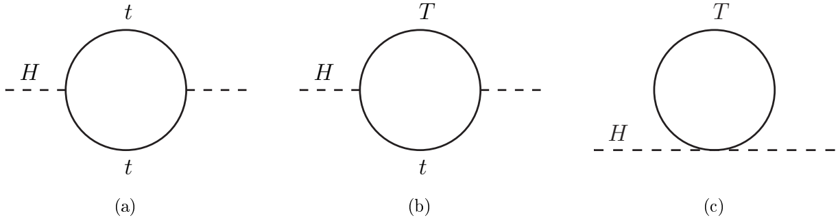
Figure 1.9: One-loop contributions to the Higgs boson mass term from (a) the top quark and (b, c) a vector-like top-quark partner T .
