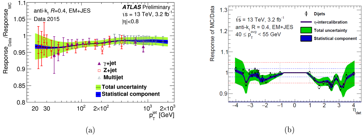
Figure 4.11: Ratio of the average jet response in data to that measured in MC simulation (a) as a function of jet p_T for different in-situ calibration techniques ( \gamma +jet, Z+jet, and multijet balance) and (b) as a function of jet \eta for jets with 40 < p_T < 55 GeV using the dijet balance technique.
