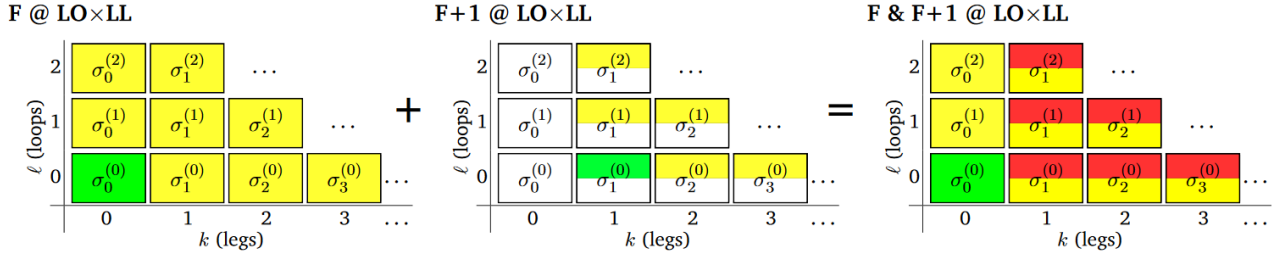
Figure 3.4: The double-counting problem caused by adding cross sections involving matrix elements with different numbers of legs when interfaced to parton showers. From reference [110].
