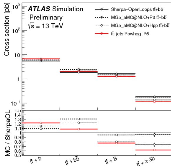
Figure 5.5: Cross section for different categories of t\bar{t} + \geq 1b events. The three 4FNS NLO samples are compared to the POWHEG-BOX+PYTHIA t\bar{t} +jets sample.
