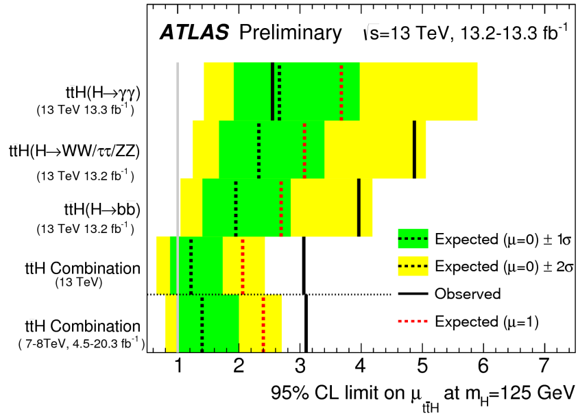
Figure 7.15: Summary of the 95% CL upper limits on \sigma(t\bar{t}H) relative to the SM prediction.
