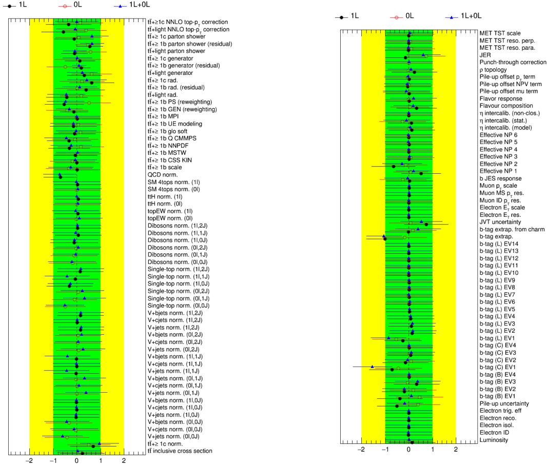
Figure 6.16: Fitted NPs from a fit under the background-only hypothesis. Shown are the fits using the 1-lepton channel only (black), 0-lepton channel only (red), and the combination of both channels (blue). A detailed description of the naming of the NPs can be found in appendix B.
