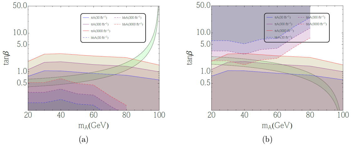
Figure A.5: Sensitivity reach (at 95% CL) of the b\bar{b}A and t\bar{t}A channels within the (a) Type-I 2HDM and (b) Type-II 2HDM. The green bands represent a region where the recently observed gamma-ray excess from the Galactic Centre can be explained.
