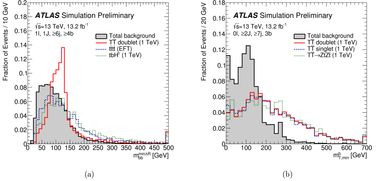
Figure 6.8: Comparison of the shape of (a) the invariant mass distribution of the two b -tagged jets with lowest \Delta R separation ( m_{bb}^{min\Delta R} ), and (b) the distribution of the minimum transverse mass between E_T^{miss} and any of the three leading b -tagged jets in the event ( m_{T,min}^b ), between the total background (shaded histogram) and several signal scenarios considered in this search. The signals shown are: T\bar{T} production in the weak-isospin doublet and singlet scenarios, and for \text{BR}(T \rightarrow Zt) = 1 , assuming m_T = 1 TeV; t\bar{t}t\bar{t} production within an EFT model; and tbH^\pm(\rightarrow tb) production assuming m_{H^\pm} = 1 TeV. The selection used in (a) corresponds to events in the (1J, \geq 6j, \geq 4b) region of the 1-lepton channel, whereas the selection used in (b) corresponds to events in the (\geq 2J, \geq 7j, 3b) region of the 0-lepton channel. The last bin contains the overflow.
