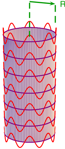
Figure 1.8: Representation of an extra spatial dimension with radius R . From reference [54].
