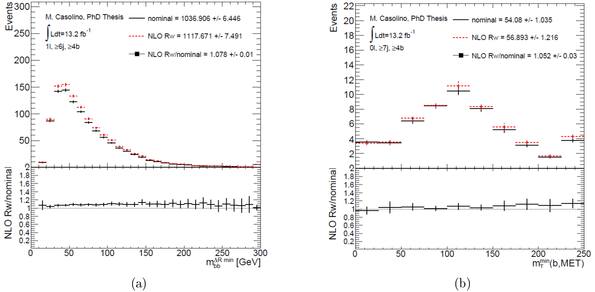
Figure 5.7: (a) The mass of the b\bar{b} pair with smallest \Delta R distance, m_{bb}^{\text{min}\Delta R} for events with one lepton at least six jets and at least four b -tags, and (b) the minimum transverse mass between E_T^{\text{miss}} and any of the three leading b -tagged jets in the event, m_{T,\text{min}}^b , for events with no lepton at least seven jets and at least four b -tags. In red the prediction obtained with the reweighting to SHERPAOL and in black the nominal prediction.
