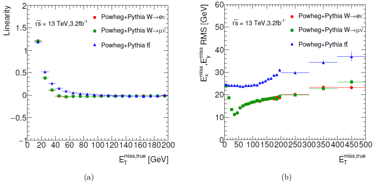
Figure 4.23: The E_T^{\text{miss}} (a) response and (b) resolution evaluated in W \rightarrow \ell\nu and t\bar{t} simulated events. From reference [171].
