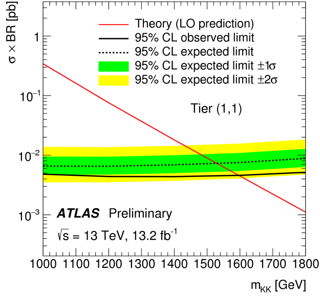
Figure 6.29: Observed (solid line) and expected (dashed line) 95% CL upper limits on the production cross section times branching ratio of four-top-quark events as a function of the Kaluza-Klein mass ( m_{KK} ) from tier (1,1) in the symmetric case ( \xi = R_4/R_5 = 1 ). The surrounding shaded bands correspond to \pm 1 and \pm 2 standard deviations around the expected limit. The thin red line shows the theoretical prediction, computed at LO in QCD, for the production cross section of four-top-quark events by tier (1,1) assuming BR(A^{(1,1)} \rightarrow t\bar{t}) = 1 , where the heavy photon A^{(1,1)} is the lightest particle of this tier.
