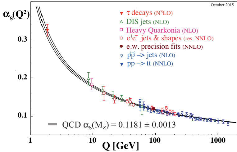
Figure 1.1: Evolution of the strong coupling constant \alpha_s with energy scale Q , as probed by different measurements. From reference [5].
