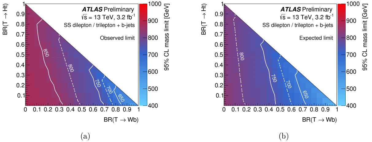
Figure 6.28: (a) Observed and (b) expected limit (95% CL) on the mass of the T quark in the plane of \text{BR}(T \rightarrow Ht) versus \text{BR}(T \rightarrow Wb) for the same-charge dileptons/trileptons search. Contour lines are provided to guide the eye.
