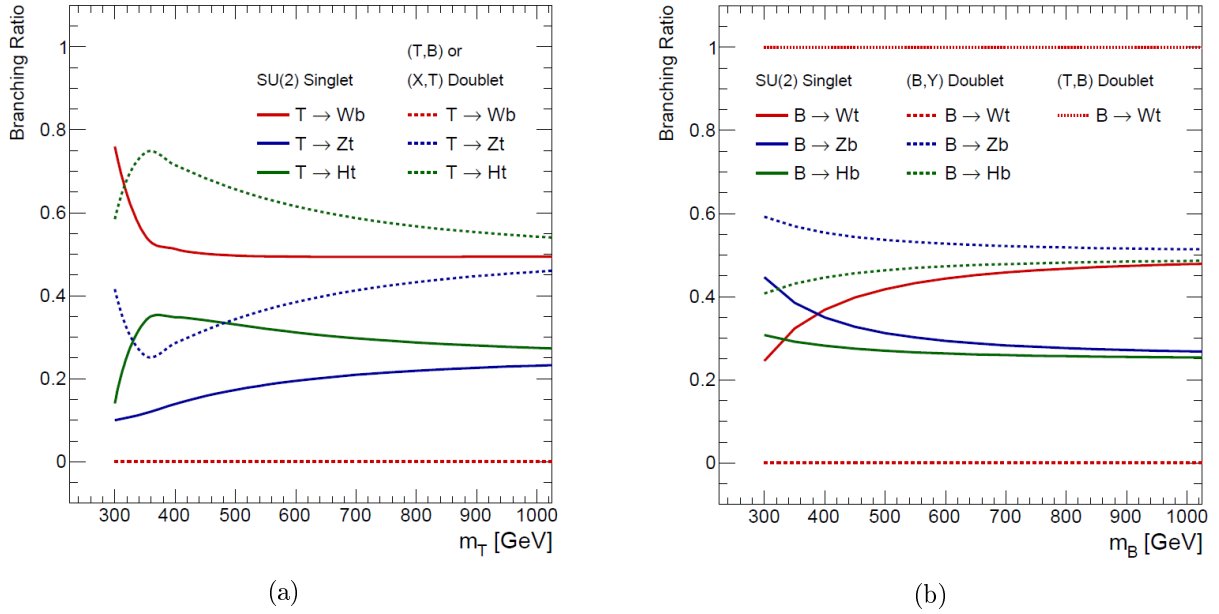
Figure 1.10: Branching ratios for vector-like (a) top and (b) bottom partners as function of the heavy-quark mass m_T and m_B respectively for singlets and doublets. From reference [70].
