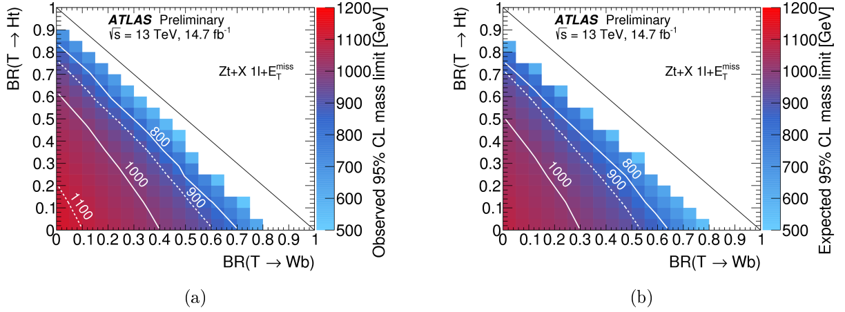
Figure 6.27: (a) Observed and (b) expected limit (95% CL) on the mass of the T quark in the plane of \text{BR}(T \rightarrow Ht) versus \text{BR}(T \rightarrow Wb) for the Zt + X search. Contour lines are provided to guide the eye.
