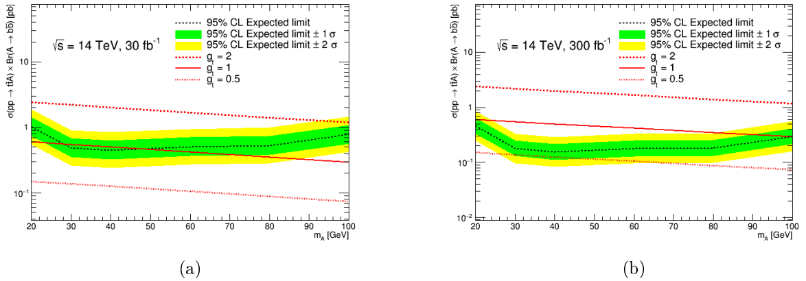
Figure A.4: Expected 95% CL upper limits on \sigma(t\bar{t}A) \times \text{BR}(A \rightarrow b\bar{b}) as a function of m_A in pp collisions at \sqrt{s} = 14 \text{ TeV} for an integrated luminosity of (a) 30 \text{ fb}^{-1} and (b) 300 \text{ fb}^{-1} . The green and yellow bands correspond to 1 and 2 standard deviations respectively around the median expected limit under the background-only hypothesis. Also shown are the theoretical cross sections for \sigma(t\bar{t}A) for different assumed values of g_t (0.5, 1.0, and 2.0) and \text{BR}(A \rightarrow b\bar{b}) = 1 .
