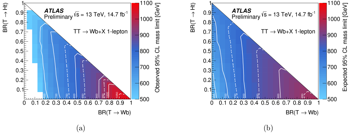
Figure 6.26: (a) Observed and (b) expected limit (95% CL) on the mass of the T quark in the plane of \text{BR}(T \rightarrow Ht) versus \text{BR}(T \rightarrow Wb) for the Wb+X search. Contour lines are provided to guide the eye.
