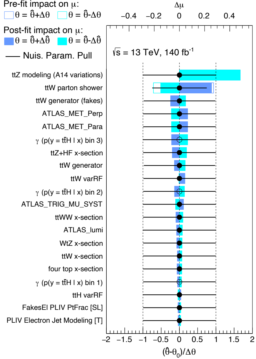
Figure 3.4: Ranking plot for systematic uncertainties.
