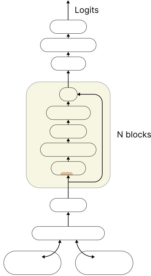
Figure 2.5: ResNet architecture.
