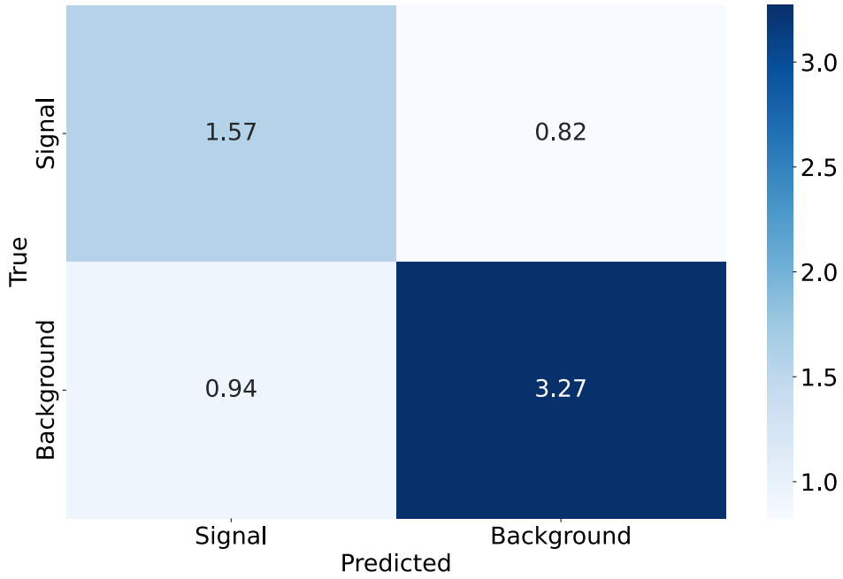
Figure 2.2: Confusion matrix for a binary classification task. This confusion matrix is produced using 5-blocks FT-Transformer (subsection 2.3.5) trained on the extended training set (section 2.4) evaluated on the validation set, that contains 20% of the SR events. Signal refers to t\bar{t}H , and background refers to all the other classes. The arg max classification strategy was used. Note that the classifier was trained to differentiate between all the classes, but during evaluation, all the non- t\bar{t}H events are grouped together.
