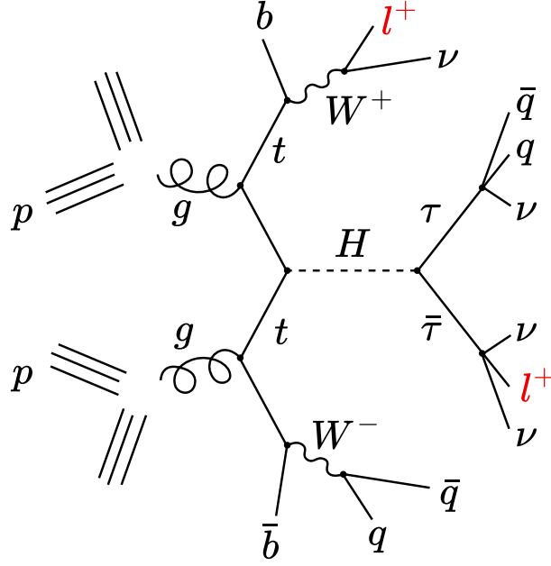
Figure 1.4: Feynman diagram of the 2l_{SS} + 1\tau_{\text{had}} process.
