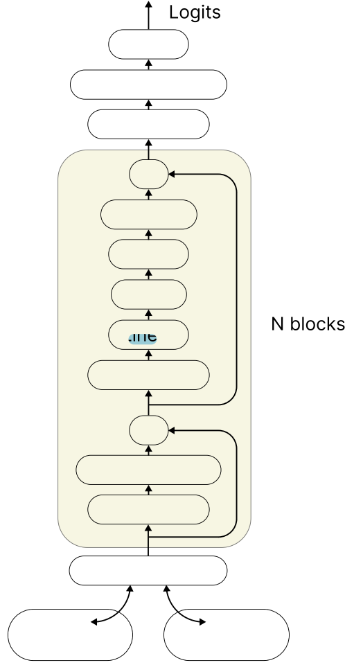
Figure 2.8: FT-Transformer architecture.
