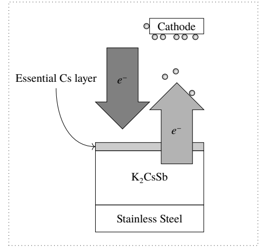
(b) Dynode with sufficiently eroded Caesium layer to enter the down-drift regime.
