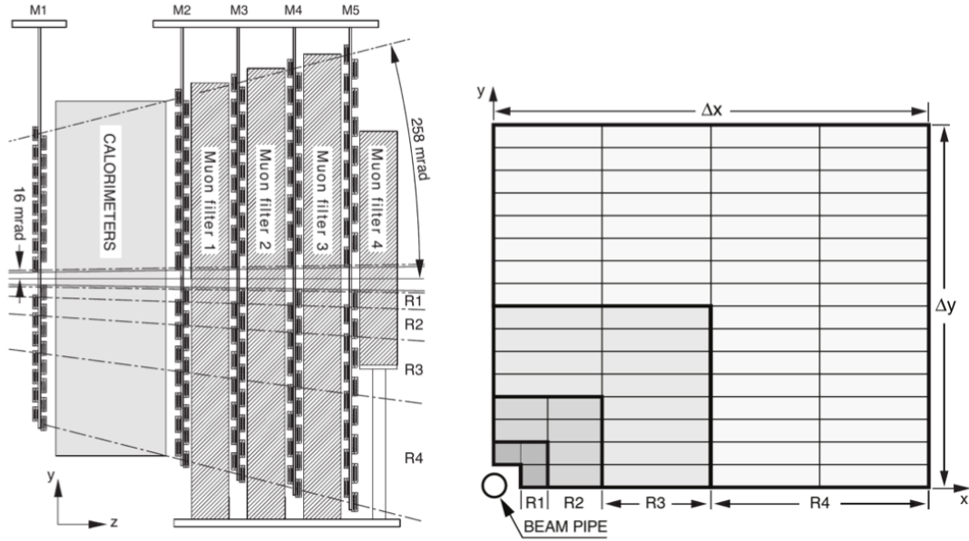
Figure 2.12: Schematic design of the muon stations [30].
