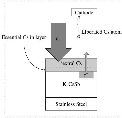
(a) Dynode with a Caesium layer that is too thick, i.e. the 'extra' amount of Cs makes the dynode performance worse.
