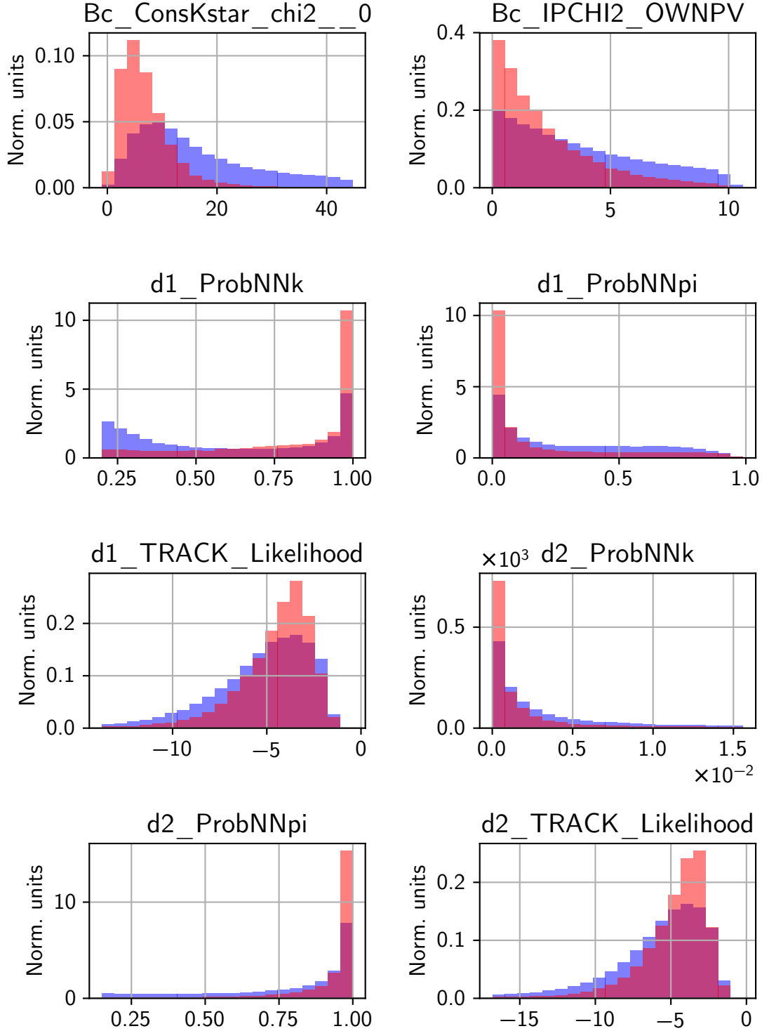
Figure 5.5: Input variable distributions for the BDT for B^+ \rightarrow K^{*0}(892)(\rightarrow K^+\pi^-)\pi^+ 2011. Red is simulated data (signal) and blue is data sidebands (background). x -axes are dimensionless. y -axes are normalised counts (such that the area under each individual histogram is 1).
