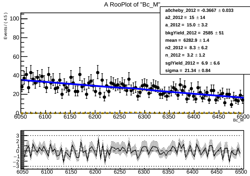
(b) Fit of 2012 signal channel ( B_c^+ \rightarrow \bar{K}^{*0}(892)(\rightarrow K^- \pi^+) K^+ ) data
