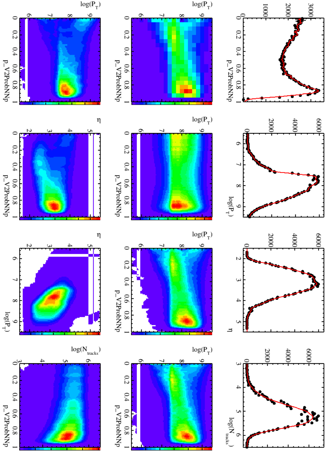
Figure 5.2: Results of the calculation of the KDE for ProbbNNP [78].
