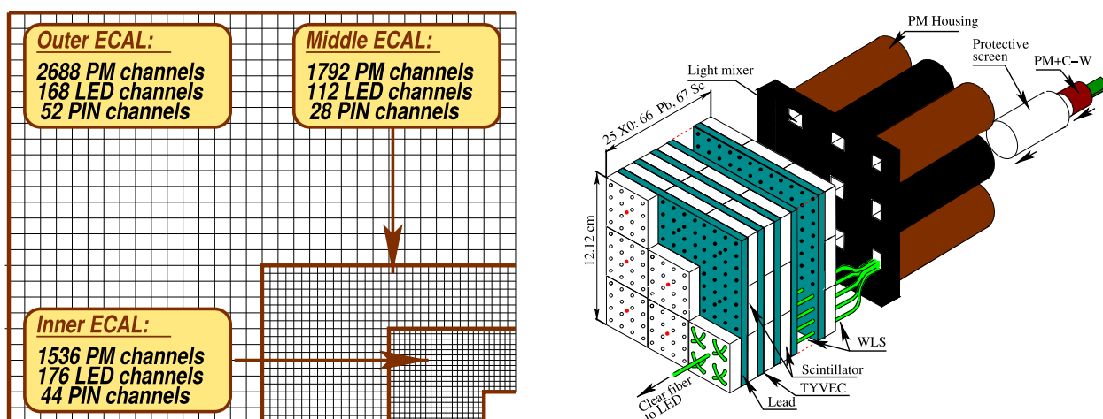
Figure 2.10: Schematic diagram of the ECAL [39]. (left) a schematic diagram of cell size. (right) an example of the inner section of the ECAL
