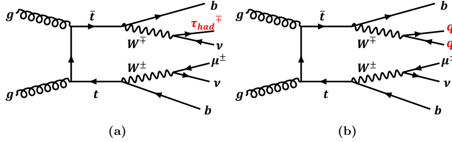
Figure 4.35.: Feynman diagrams for t\bar{t} event. (a) shows the signal process with one \tau_{\text{had}} , and (b) present the background process includes W boson decay to quark production.
