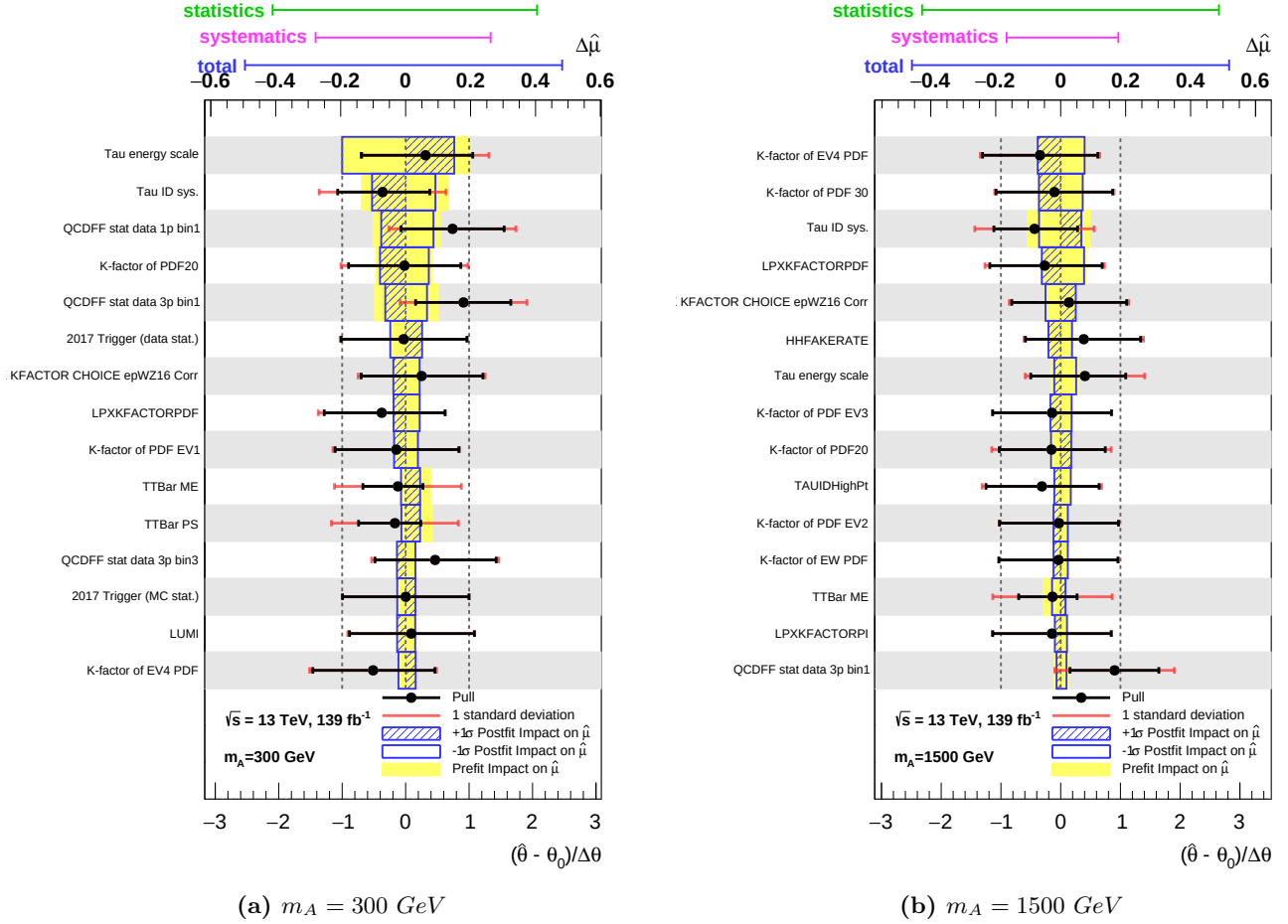
Figure 8.5.: Impact from each nuisance parameter on the fitted signal strength for m_A = 300 GeV and m_A = 1500 GeV. The corresponding \tan\beta hypotheses for m_A = 300 GeV and m_A = 1500 GeV Higgs are assumed as 2 and 23. The red lines in the ranking plots are shown as “1 standard deviation”. The black points with the black lines in the plots are the fitted value and corresponding \pm 1 - \sigma values after the shifting, so called as “pull value”. The pull value is quantified to as \text{pull}(\theta) = (\hat{\theta} - \theta_0)/\sigma_\theta [201]. It shows the difference between the expected value and the fitting result of MLE. The nuisance parameters are ordered by their impact on the signal strength \hat{\mu} . The blue opened box presents the impact on post-fit result and the impact on the pre-fit result is shown as the yellow box. The impact on \hat{\mu} from overall systematic uncertainties is illustrated as pink line in the top of ranking plots. The statistical uncertainty is also presented as green line. The combined uncertainty of statistic and systematic is shown as blue line.
