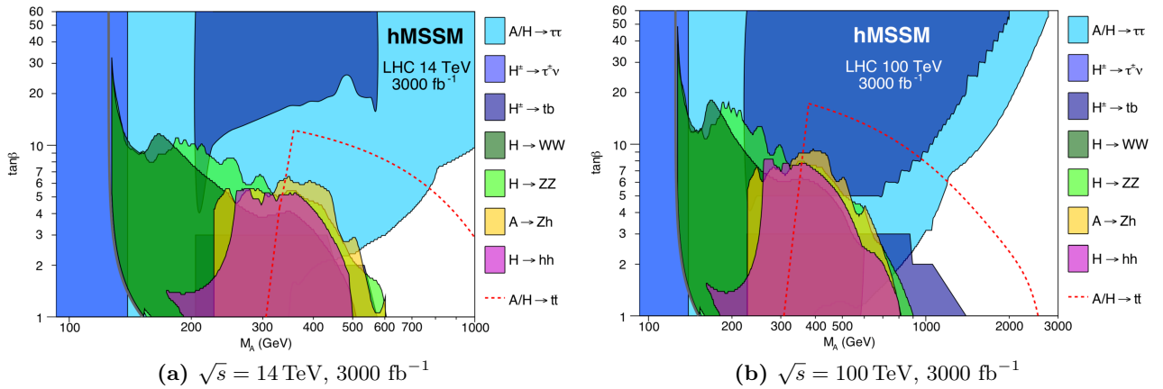
Figure 9.2.: Projections for the limit of the 2\sigma sensitivity in the hMSSM ( \tan\beta, m_A ) plane corresponding to 3000 \text{ fb}^{-1} data. (a) shows the one for the HL-LHC at a center-of-mass energy of \sqrt{s} = 14 \text{ TeV} and the expected limit for FCC at a center-of-mass energy of \sqrt{s} = 100 \text{ TeV} is presented in (b) [34, 204].
