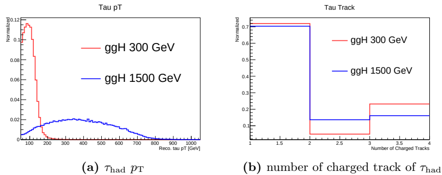
Figure 4.32.: The p_T distribution of gen-matching \tau_{had} in (a) shows the importance of high- p_T \tau_{had} in the heavy Higgs search. (b) shows the number of charged tracks associated to \tau_{had} in signal with different mass region.
