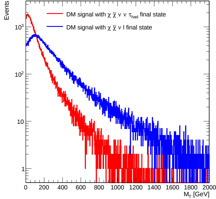
Figure 12.1.: The M_T distribution of a DM signal ( pp \rightarrow \chi\chi l\nu ) shows that the tau decay process pp \rightarrow \chi\chi\tau^{\text{had}}\nu\nu has substantially less events at high M_T than the light lepton final states.
