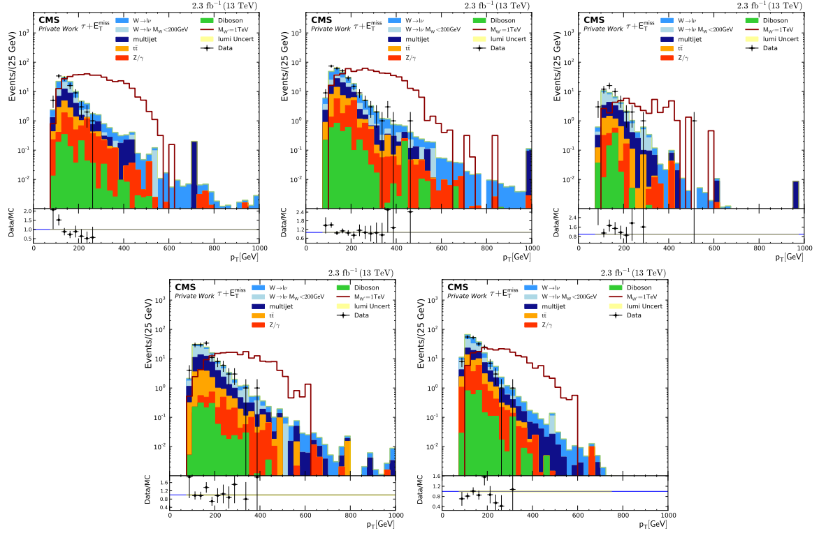
Figure A.22.: Control plots for the full selection split into the decay mode. The order is 1Prong 0 \pi^0 , 1Prong 1 \pi^0 and 2Prong 0 \pi^0 at the top and 2Prong 1 \pi^0 and 3Prong 0 \pi^0 in the bottom.
