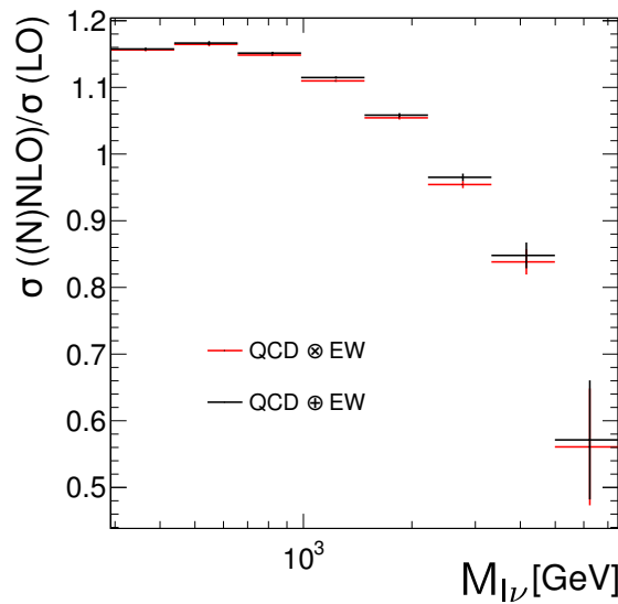
Figure 8.1.: k-factors for the additive and factorial combination of NNLO QCD and NLO EW corrections for the pp \rightarrow W \rightarrow \tau\nu process.
