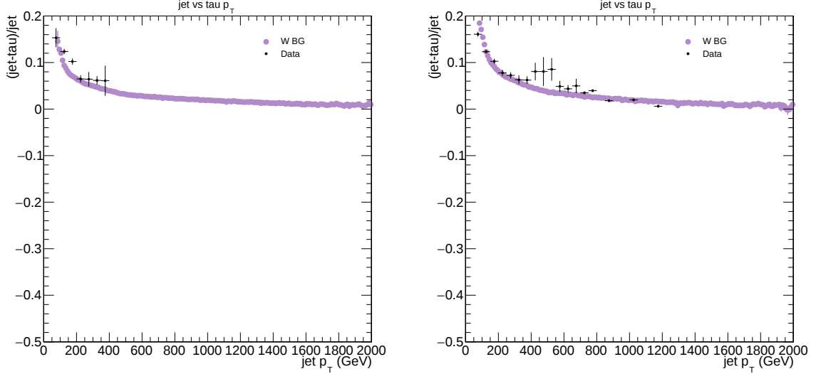
Figure 4.21.: Tau response shown in comparison with the jet response in data and simulation. This comparison is done for the events selected for the analysis as described in Section 8.4. In the left plot the full signal selection is applied and in the right plot only the one tau passing the trigger and identification is required.
