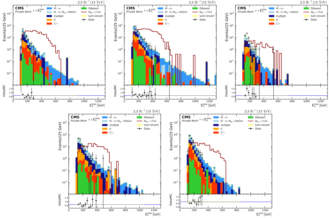
Figure A.20.: Control plots for the full selection split into the decay mode. The order is 1Prong 0 \pi^0 , 1Prong 1 \pi^0 and 2Prong 0 \pi^0 at the top and 2Prong 1 \pi^0 and 3Prong 0 \pi^0 in the bottom.
