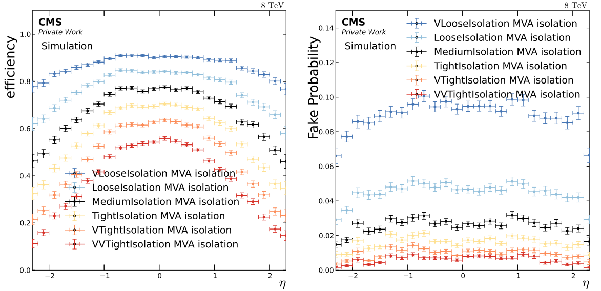
Figure A.4.: The tau identification efficiencies (left) and fake probability (right) for high p_T taus as a function of \eta .
