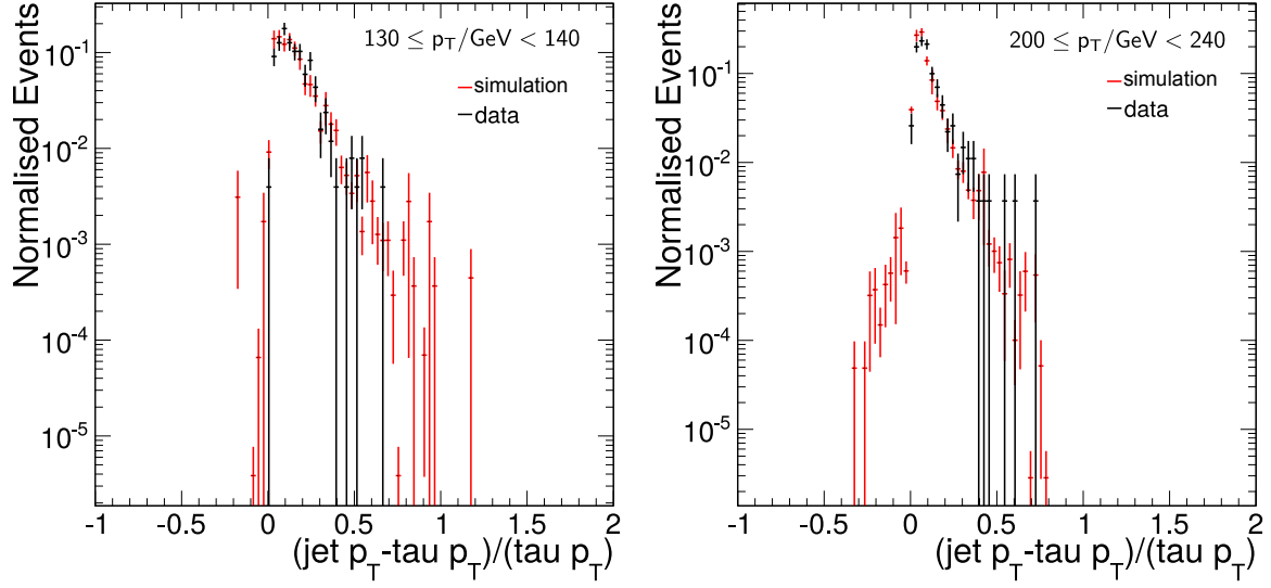
Figure 4.18.: The plots show the ratio of the jet and \tau^{\text{had}} p_T difference to the \tau^{\text{had}} p_T ( 130 \leq p_T/\text{GeV} < 140 and 200 \leq p_T/\text{GeV} < 240 ).
