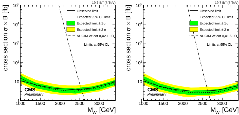
Figure 10.4.: The plots show the limits for \cot \theta_E = 2.1 (left) and \cot \theta_E = 1.6 (right). For the first parameter, W' masses below 2.5 TeV are excluded and for the second one W' masses below 2.6 TeV are excluded at 95 % CL.
