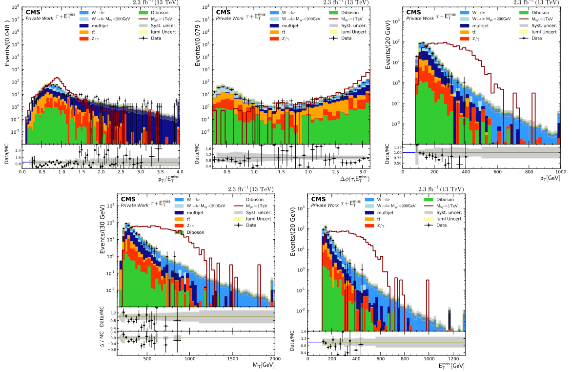
Figure A.27.: Plots for the same selection but with the "old" decay mode, where 2 prongs are not reconstructed.
