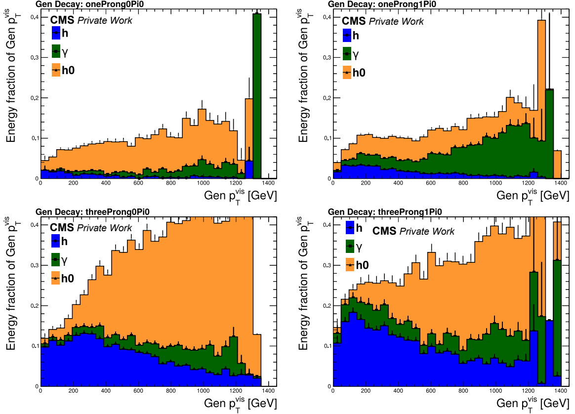
Figure 4.6.: The plots show the stacked fraction of energy w.r.t. the not picked up pfCandidates in a \Delta R < 0.12 cone around the tau. The plots are separated into generator level decay mode, which is denoted at the top of the plots.
