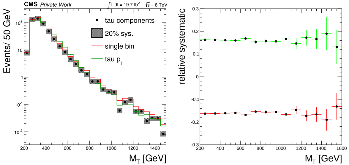
Figure 7.15.: If the fake probability is evaluated in a single bin (red curve) and as a function of \tau p_T^{\text{had}} (green curve), the prediction agrees with the prediction from the decay mode binned fake probability almost within 20% uncertainty (left). Relative systematic shift in the M_T distribution from the shifts in Figure 7.12 for the loose isolation (right).
