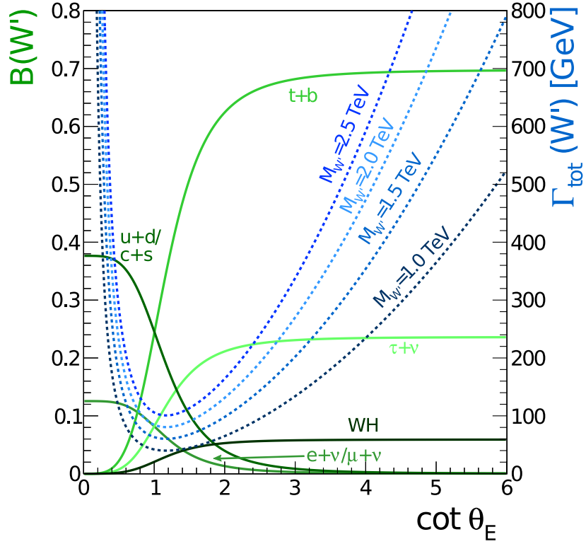
Figure 2.6.: Branching fractions (left-hand scale and solid lines) and total width (right-hand scale and dotted lines) for W' decays in the NUGIM. For \cot \theta_E = 1 the values are the same as those in the SSM, rescaled to accommodate the W' \rightarrow Wh decay channel.
