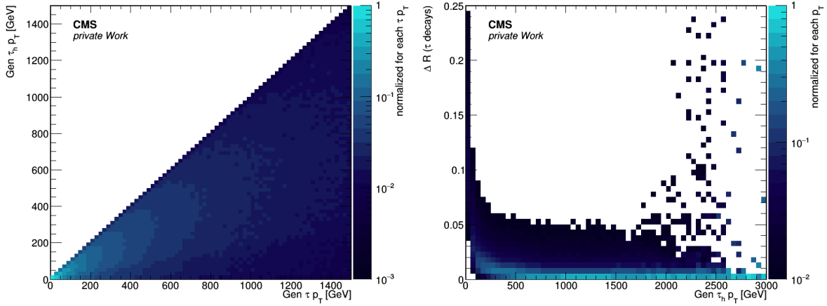
Figure 4.1.: The left plots shows the p_T of the \tau^{\text{had}} with respect to the p_T of the undecayed tau. For each \tau p_T the evnets are nomalized to show the relative distribution. On the right, the opening angle of the \tau^{\text{had}} \Delta R = \sqrt{(\Delta\phi)^2 + (\Delta\eta)^2} is shown with respect to the p_T of the tau evaluated with PYTHIA 8.
