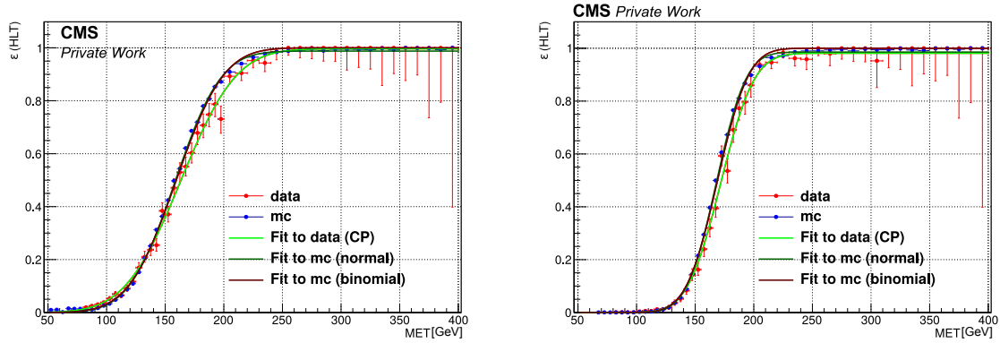
Figure 7.3.: The E_T^{\text{miss}} trigger turn on curve for calorimeter based E_T^{\text{miss}} (left) and \text{pf}E_T^{\text{miss}} (right). The turn on was measured with the tau E_T^{\text{miss}} trigger (tau p_T > 35 GeV and \text{pf}E_T^{\text{miss}} > 70 GeV), which has a much lower threshold in E_T^{\text{miss}} and therefore can be seen as independent.
