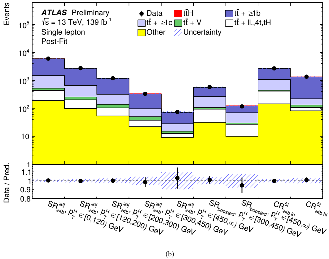
Figure 14.5.: Predicted and observed event yields in all regions of the lepton+jets channel (a) before the fit and (b) after the fit to data [5]. The uncertainty band of the pre-fit distribution (a) contains all uncertainties except the uncertainty of k(\text{t}\bar{\text{t}} + \geq 1\text{b}) which is only defined post-fit. In the post-fit version (b) all uncertainties with their correlations are considered.
