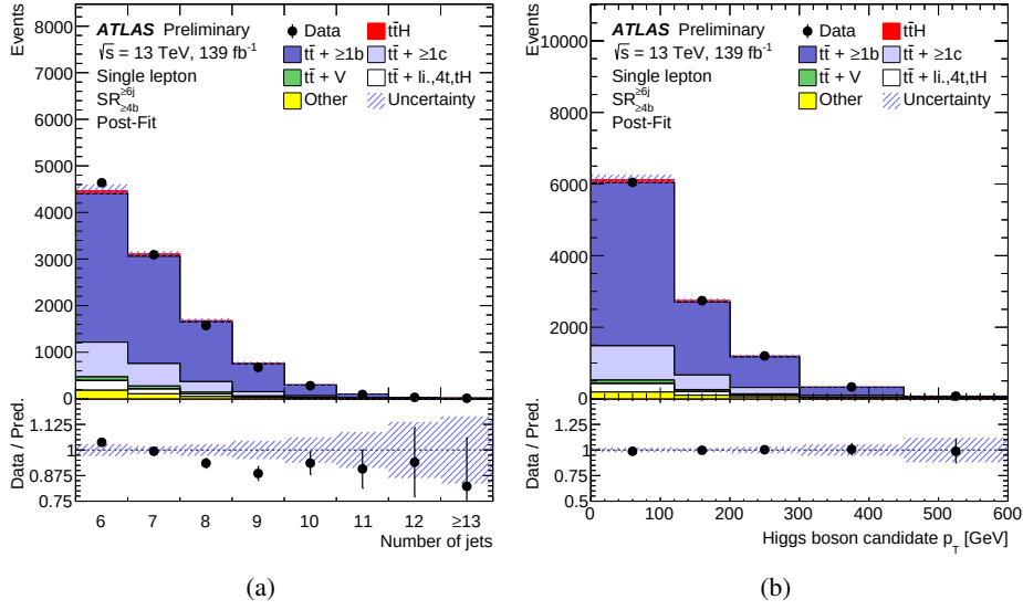
Figure 14.9.: Post-fit distributions of the (a) number of jets and (b) the reconstructed Higgs boson candidate p_T in the lepton+jets resolved SR_{\geq 4b}^{\geq 6j} signal regions. The t\bar{t}H signal yield (solid red) is normalised to the fitted \mu value from the inclusive fit. The uncertainty band includes all uncertainties and their correlations [5].
