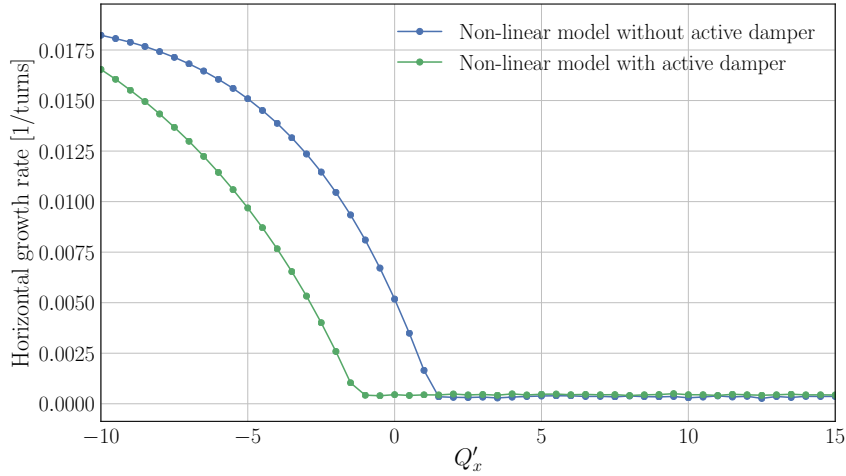
Figure 5.20: Simulated chromaticity scan for the non-linear machine model. The horizontal instability growth rate is plotted against the horizontal chromaticity Q'_x . The simulations have been run without (blue) and with active bunch-by-bunch damper with a damping time of 100 turns (green).
