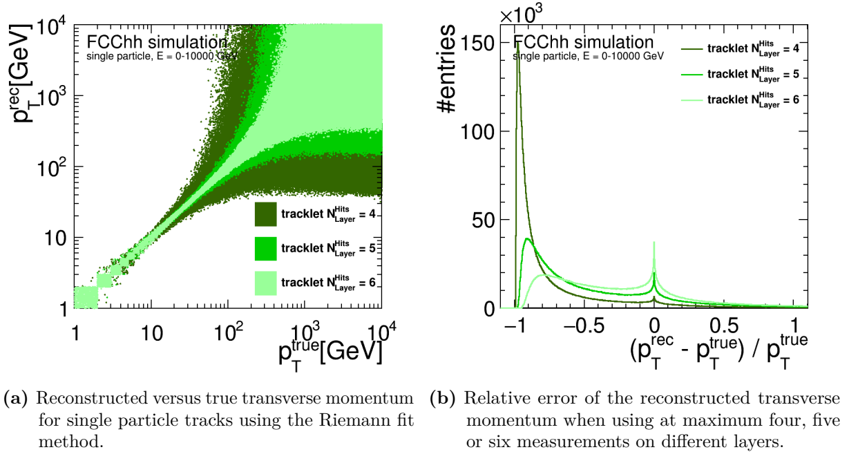
fig. A.28: Transverse momentum resolution for single particle tracks. The tracks have been created using a "toy"-model.
