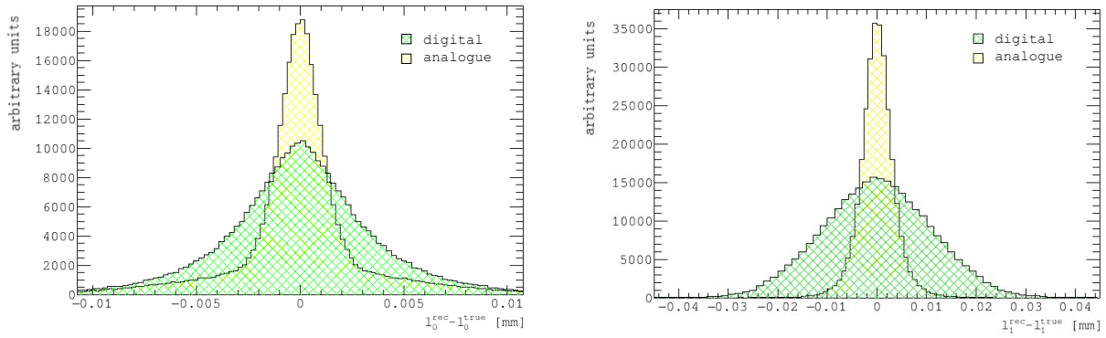
(a) Cluster position resolution for 25 \mu\text{m} pixel width in local x , global r/\phi . (b) Cluster position resolution for 50 \mu\text{m} pixel length in local y , global z .
