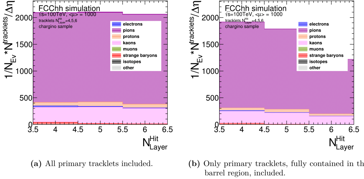
fig. 6.6: Number of different layers hit by primary tracklets of the underlying event and pile-up. The plot is stacked and shows the composition of tracklets.
