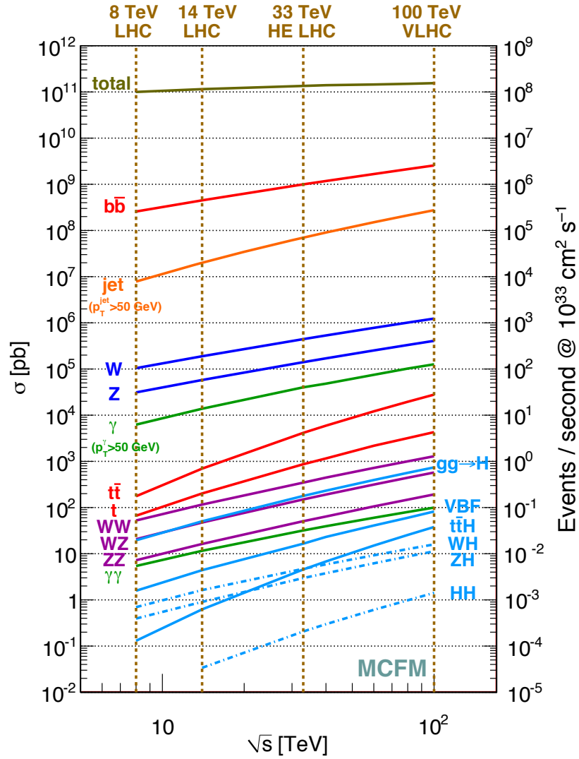
fig. 2.2: Standard Model process cross sections at hadron colliders as a function of centre-of-mass energy ( \sqrt{s} ) and Higgs-boson production cross sections as a function of centre-of-mass energies (light blue). The axis on the right, shows the corresponding number of expected events per second. Source of figure: [52].
