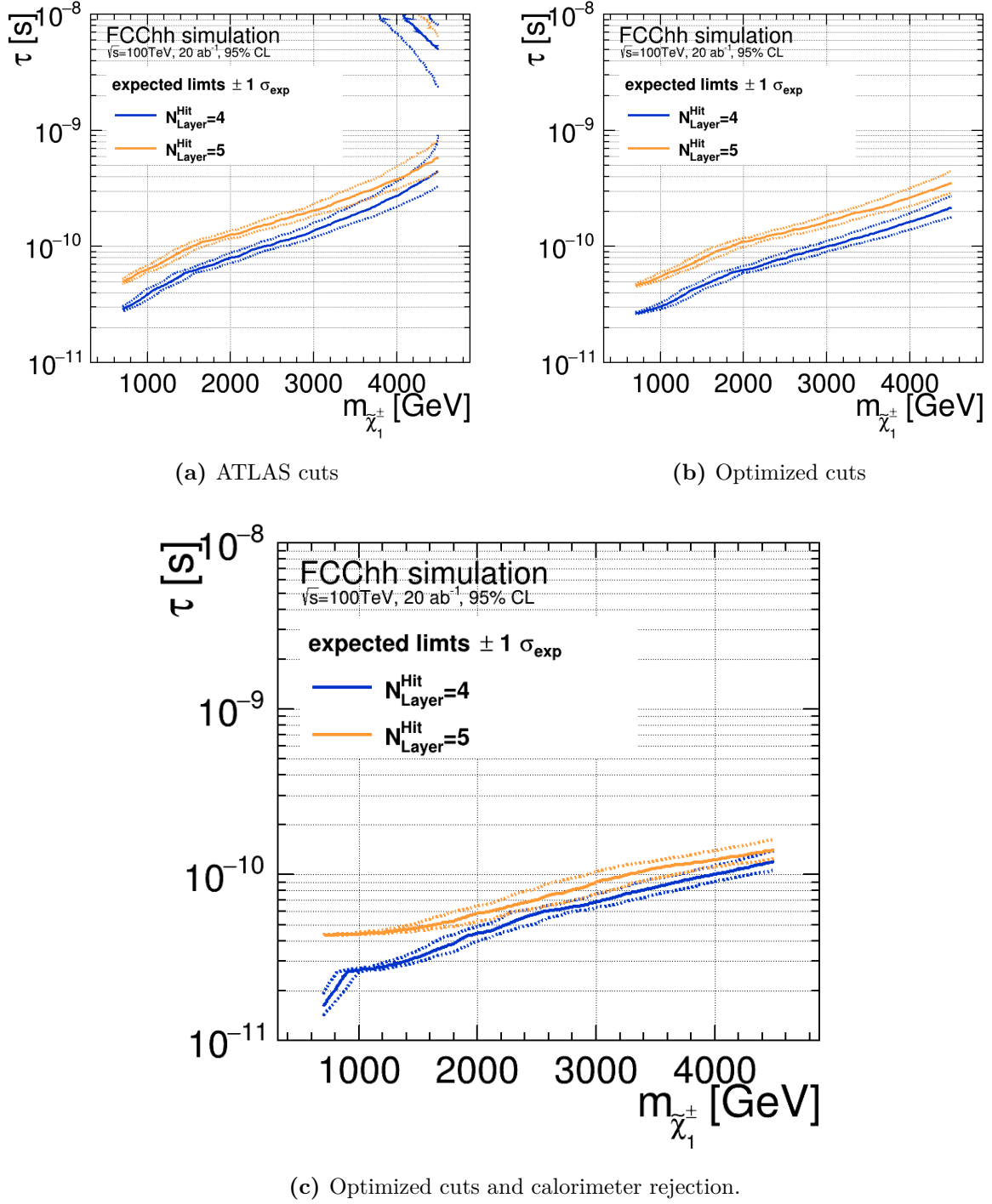
fig. 6.22: Expected exclusion limits at 95 % confidence level, as a function of wino mass and lifetime, assuming an integrated luminosity of L = 20 \text{ ab}^{-1} . The dashed lines, show the 1\sigma region of the expected limits and the median is displayed as solid line. The limits are given for the different cuts and for assuming different number of layers hit.
