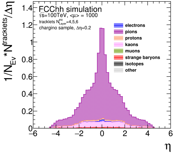
(a) All primary tracklets of underlying event included.
