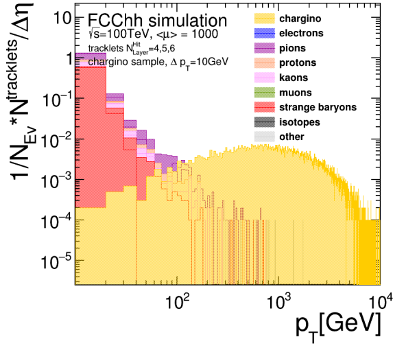
(a) All primary tracklets included.
