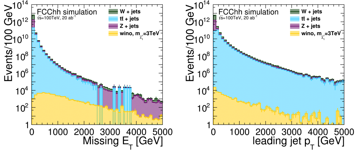
(a) Stacked SM background contributions, overlaid with the wino signal for \tau_{\tilde{\chi}_1^\pm} = 0.2 ns and m_{\tilde{\chi}_1^\pm} = 3 TeV. Total number of expected events (for an integrated luminosity of 20 \text{ ab}^{-1} ) is plotted versus the missing transverse energy of the event. (b) Stacked SM background contributions, overlaid with the wino signal for \tau_{\tilde{\chi}_1^\pm} = 0.2 ns and m_{\tilde{\chi}_1^\pm} = 3 TeV. Total number of expected events (for an integrated luminosity of 20 \text{ ab}^{-1} ) is plotted versus the leading jet transverse momentum of the event.
