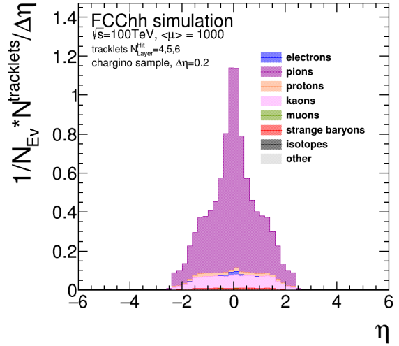
(b) Only primary tracklets of the underlying event, fully contained in the barrel region, included.
