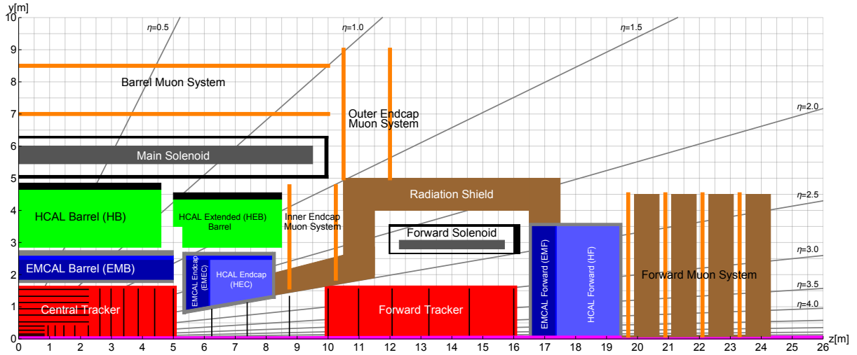
fig. 2.4: The cross section of the FCC-hh reference detector design showing the y coordinate versus z, consisting of the different detector-subsystems, magnetic coils and shieldin is shown. Only the first quadrant of the detector is shown. Source if figure: [52].
