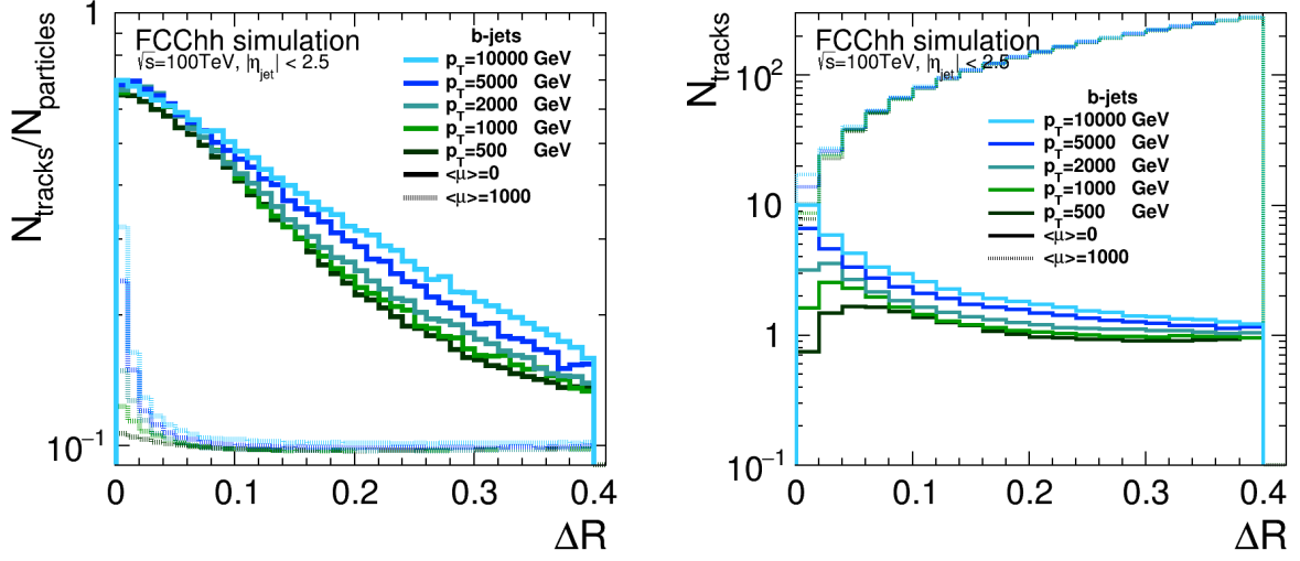
(a) Fraction of reconstructable particles (making at least eight hits on different layers) to the total number of particles, produced during simulation, which make at least one hit, against the distance from the jet core, for different jet p_T 's. The dashed lines show the results including pile-up. (b) Number of reconstructable particles over the angular distance of the jet-axis, for different jet transverse momenta.
