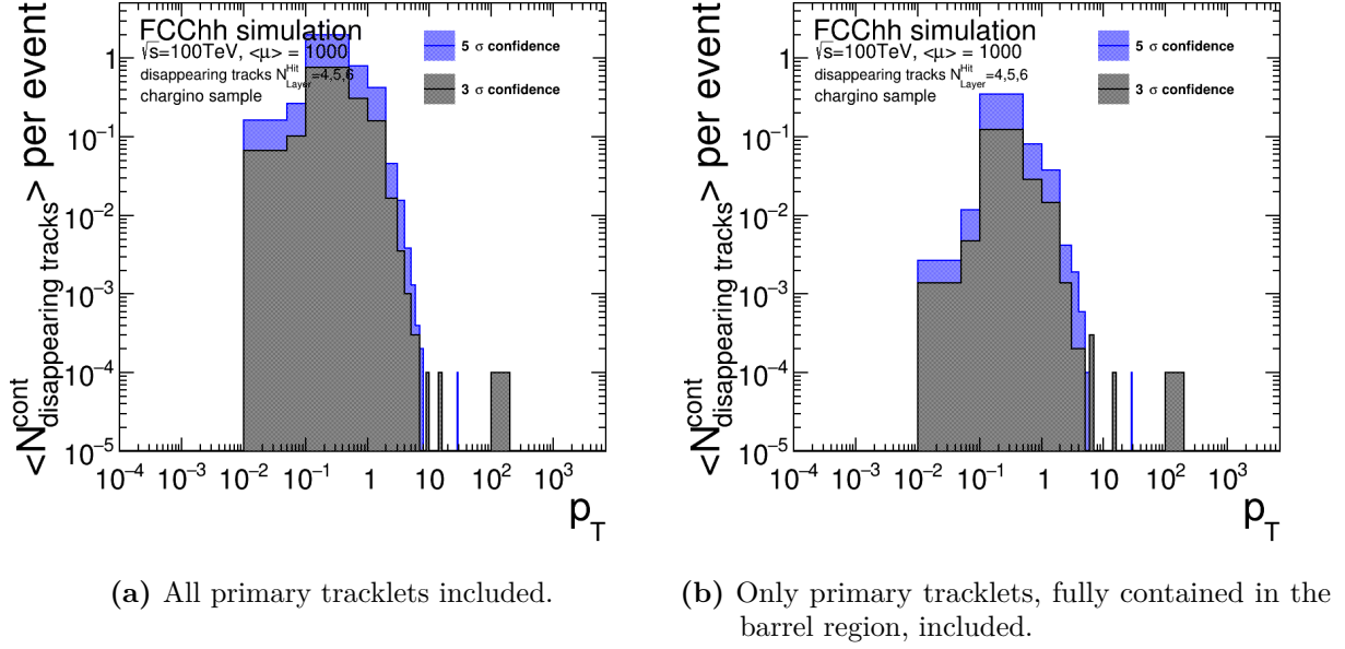
fig. 6.12: Transverse momentum distribution of primary vertices of tracklets contaminating the primary signal vertex.
