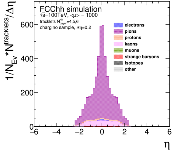
(b) Only primary tracklets, fully contained in the barrel region, included.
