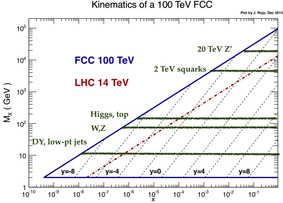
fig. 2.1: Kinematical coverage in the (x, M_X) plane of a \sqrt{s} = 100 \text{ TeV} hadron collider (solid blue line), compared to the corresponding coverage of the LHC at \sqrt{s} = 14 \text{ TeV} (dot-dashed red line). With M_X being the invariant mass of the produced final states and x being the fraction of momentum of the parton with respect to the hadron. The dotted lines indicate regions of constant rapidity y at the FCC. Relevant M_X regions for phenomenologically important processes, from low masses (Drell-Yan, low p_T jets), electroweak scale processes (Higgs, W, Z, top), and possible new high-mass particles (squarks, Z' ) are indicated. Source of figure: [56]
