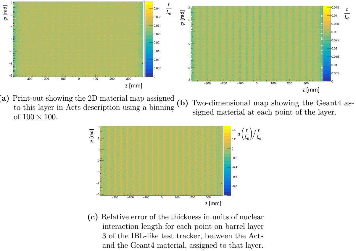
fig. 3.29: Comparison of thickness ( t ) in units of nuclear interaction length ( L_0 ) between the full Geant4 material assigned to the third layer and the mapped material in Acts description using 1M single muon Events.
