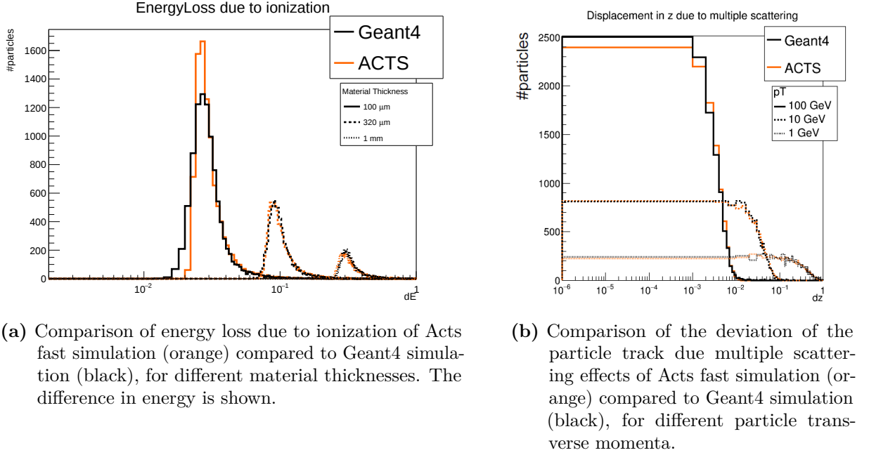
fig. 3.33: Validation of Acts FATRAS material effects against Geant4, using single muons.
