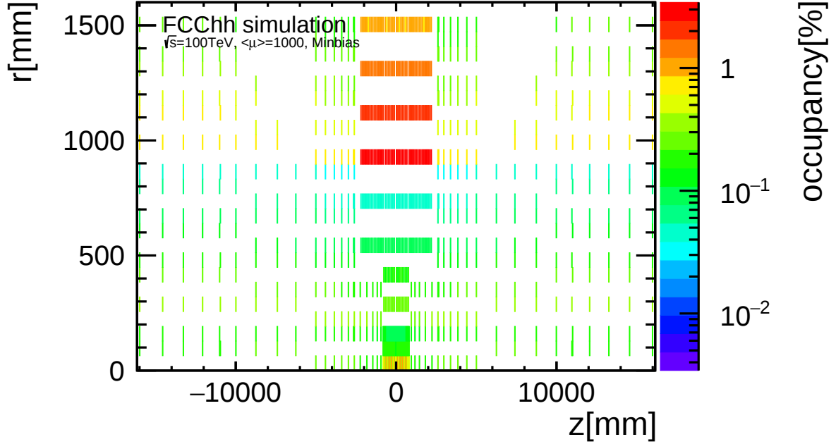
fig. 4.12: Channel occupancy map at \langle\mu\rangle = 1000 , showing the average channel occupancy of each module of the whole tracker.
