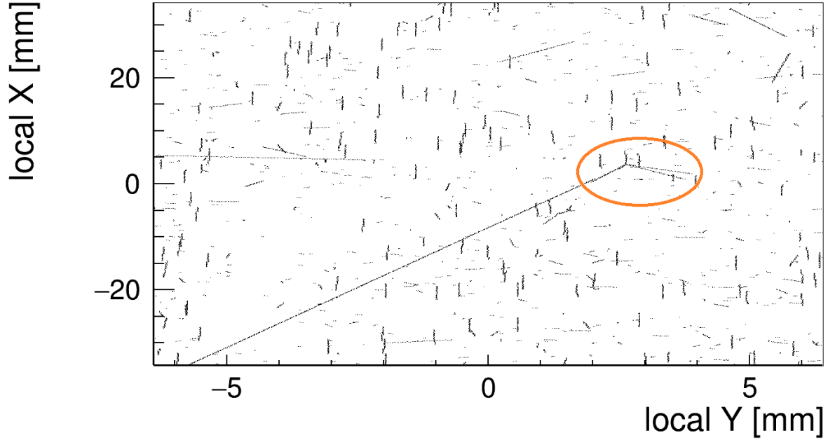
fig. 4.7: Activated cells in a module in the outermost ring of the first barrel layer at 100 TeV and \langle \mu \rangle = 1000 . The orange ellipse highlights a hadronic interaction occurring in the sensitive detector module, after a particle traversed a significant amount of material.
