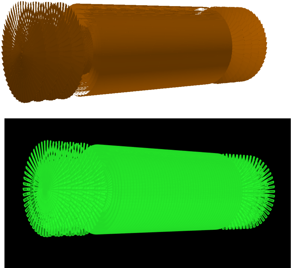
fig. A.1: On top, the DD4hep input of the sensitive modules of an "ATLAS-style" test tracker (with tilted silicon modules) is displayed. The bottom shows the translated surfaces in Acts, using JSON output of the Acts test framework, with an event display.
