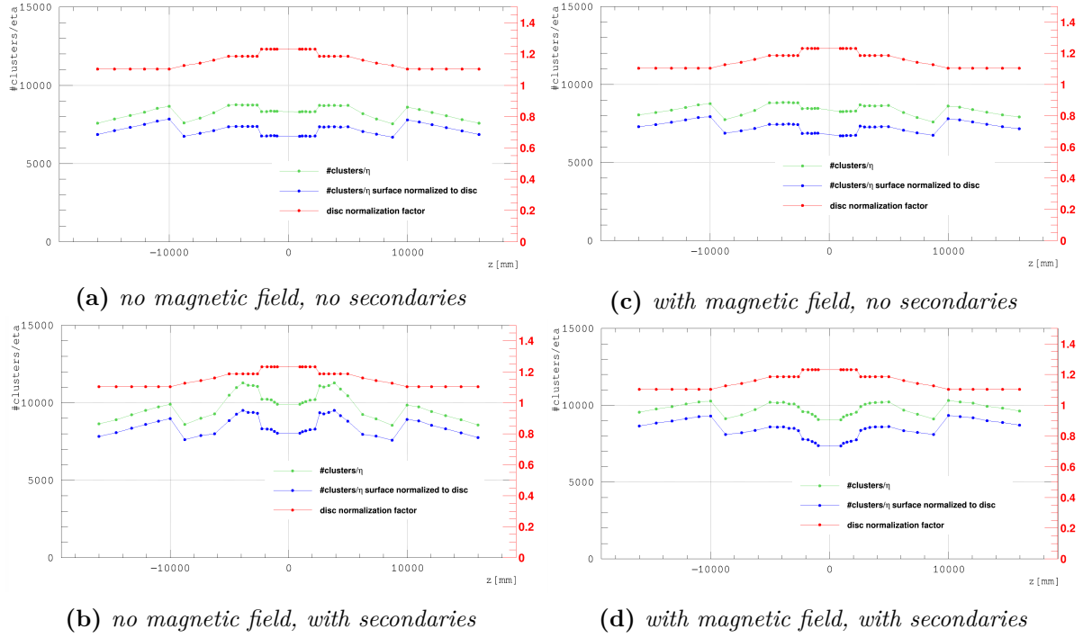
fig. A.15: Each point displays the number of cluster-measurements for the muon case divided by the \eta -coverage of each endcap disc layer, plotted against the endcap layer's position in z . Four different variations are shown: turning on/off the magnetic field and including/excluding secondary particles produced in the detector during simulation. The green line shows the pure value, while the blue line shows the values, when dividing by the surface normalization factor (accounting for overlap) of each layer displayed in red, with the corresponding axis labels on the right in red.
