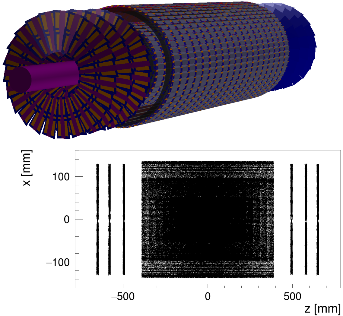
fig. A.7: On top, the DD4hep input of the sensitive modules of a test tracker to a more realistic material description. following the example of the ATLAS IBL-Module is displayed. The bottom shows the translated sensitive surfaces in Acts, as seen through fast simulation.
