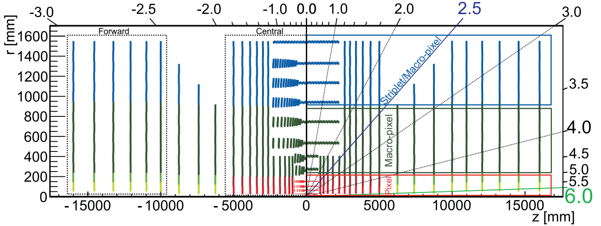
fig. 2.7: The detector modules of the FCC-hh Tracker in r/z -cross section. The tracker consists of a central, a transition and a forward region. The detector modules use silicon technology and are segmented with different granularities into pixel, macro-pixel and triplet modules. The figure is split into two halves, where the right side shows the flat and the left side the tilted layout. The dotted lines show the pseudorapidity coverage at different points. Figure by Z. Drasal [52, 65, 66].
