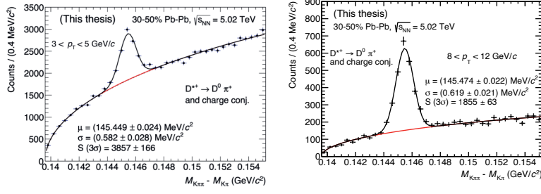
FIGURE 6.31: \Delta M invariant-mass of D^{*+} in the 30–50% centrality class in the transverse momentum ranges 3 < p_T < 5 GeV/ c and 8 < p_T < 12 GeV/ c [66].
