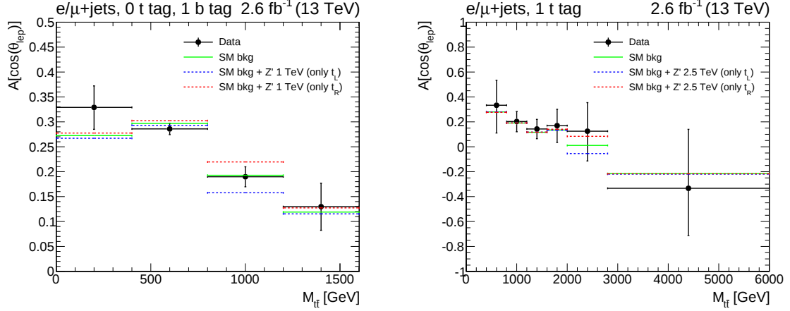
Figure 6.6: Average \cos\theta_\ell polarization asymmetry as a function of the reconstructed t\bar{t} mass: (left) T0B1 category, (right) T1 category. In both plots, the asymmetry in data is compared to the expected asymmetry from SM backgrounds and a model with background plus a Z' signal with LH or RH top quarks; the signal contribution in the left (right) plot corresponds to a Z' \rightarrow t\bar{t} resonance with M_{Z'} = 1 (2.5) TeV, normalized to the theoretical cross section for a leptophobic Z' boson in the topcolor model. Each distribution includes the events of both the \mu + \text{jets} and e + \text{jets} channels.
