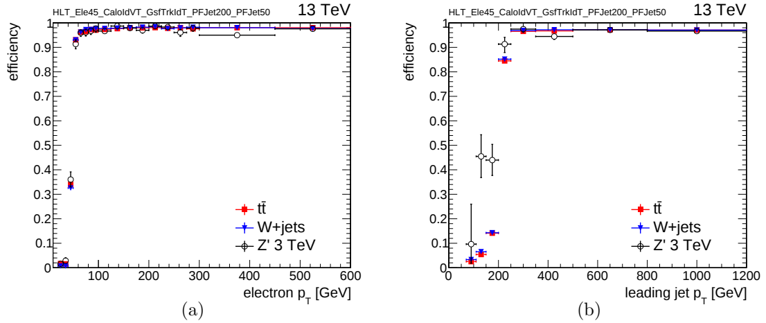
Figure 5.23: Efficiency of the e + 2 \text{ jets} trigger used in the electron channel as a function of the offline electron p_T and leading-jet p_T , for events passing the \ell + \text{jets} preselection (without cutting on the variable for which the efficiency is measured). Efficiencies are shown for the t\bar{t} MC, the W + \text{jets} MC and a Z' signal sample.
