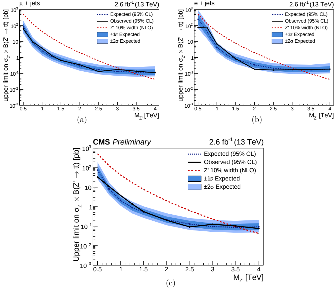
Figure 5.48: 95% CL Bayesian upper limits on the production cross section times branching ratio for a Z' boson with a relative width (\Gamma_{Z'}/M_{Z'}) of 10% decaying to a t\bar{t} pair, shown as a function of the signal mass hypothesis. The theoretical predictions correspond to the QCD-NLO cross sections for a leptophobic Z' boson in the topcolor model [139]. Limits are shown for the \mu + \text{jets} (a) and e + \text{jets} (b) channels separately and for the statistical combination of the two channels (c) [4].
