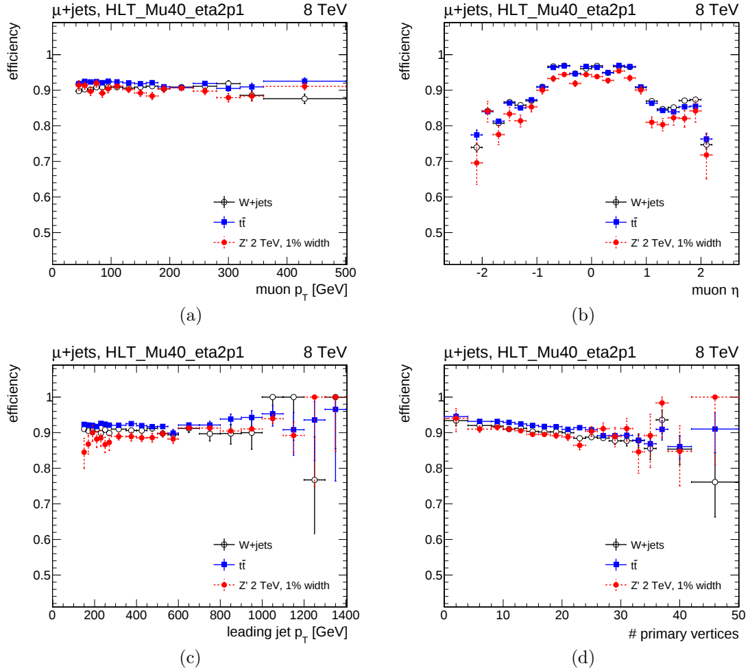
Figure 4.14: Efficiency of the single-muon trigger path \text{HLT\_Mu40\_eta2p1\_v*} , as a function of different kinematic quantities, for events passing the \mu + \text{jets} preselection: (a) muon p_T , (b) muon \eta , (c) AK5 leading jet p_T and (d) number of reconstructed primary vertices. In each plot, efficiencies are shown for W + \text{jets} , t\bar{t} and a Z' signal with M_{Z'} = 2 \text{ TeV} and \Gamma_{Z'}/M_{Z'} = 1\% .
