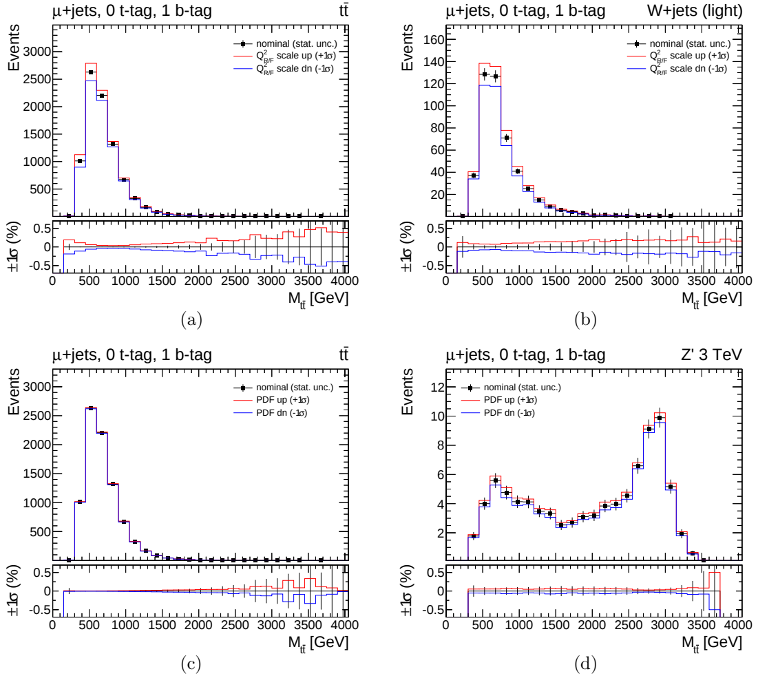
Figure 5.33: Variation of the M_{t\bar{t}} distribution due to the theoretical uncertainties associated to the MC simulation: Top: ME Q^2 -scale uncertainties for the t\bar{t} (a) and W+jets (b) MC samples. Bottom: PDF uncertainty for t\bar{t} background (c) and a Z' signal with M_{Z'} = 3 TeV (d). Each of these distributions refers to the T0B1 category of the \mu + \text{jets} analysis.
