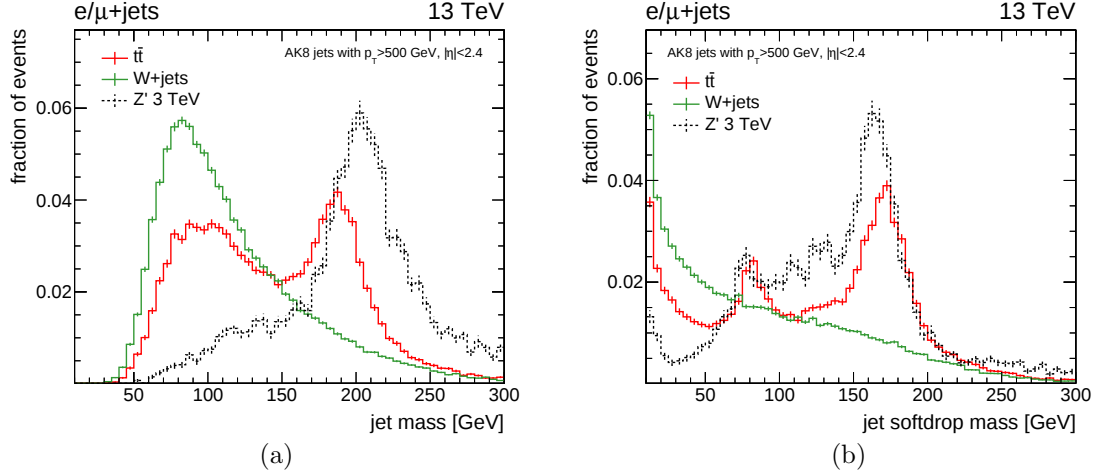
Figure 5.6: Ungroomed (a) and groomed (b) masses of AK8 jet candidates (before any t -tagging requirement) for W + \text{jets} , t\bar{t} and a Z' signal with M_{Z'} = 3 TeV in events passing the \ell + \text{jets} preselection. Each distribution is normalized to unity.
