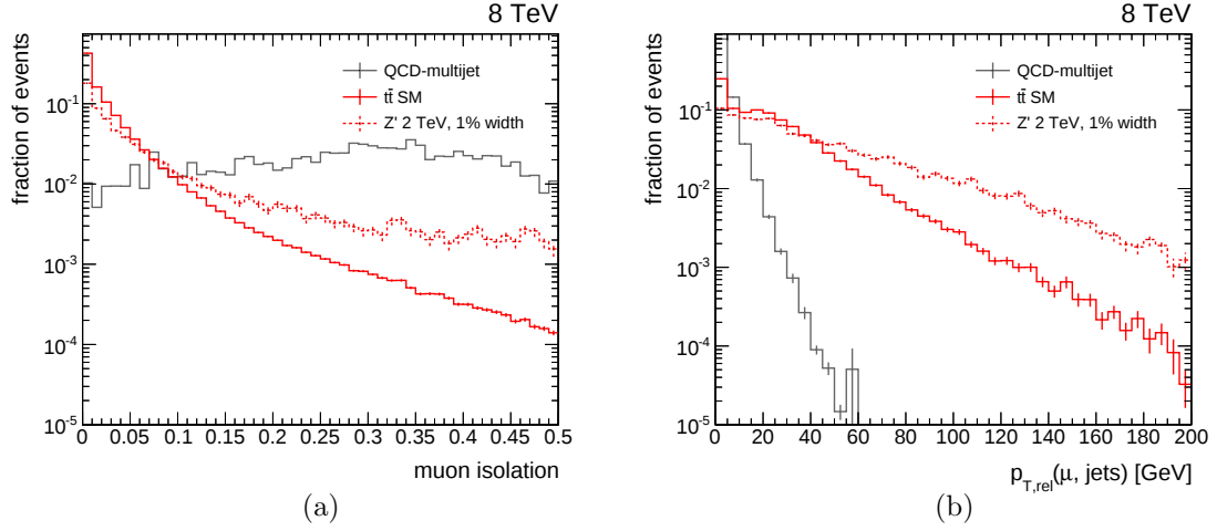
Figure 4.5: Comparison between the lepton fixed-cone isolation (a) and the p_{T,\text{rel}}(\ell, j) distribution (b) for simulated events passing the \mu + \text{jets} preselection, except for the lepton 2D-cut requirement; the p_{T,\text{rel}}(\ell, j) distribution includes only events with \Delta R_{\min}(\ell, j) < 0.5 , which is the region potentially affected by the lepton 2D-cut. Distributions are shown for QCD-multijet production, SM t\bar{t} production and a Z' resonance with a mass of 2 TeV and 1% width. Each of these distributions is normalized to unity.
