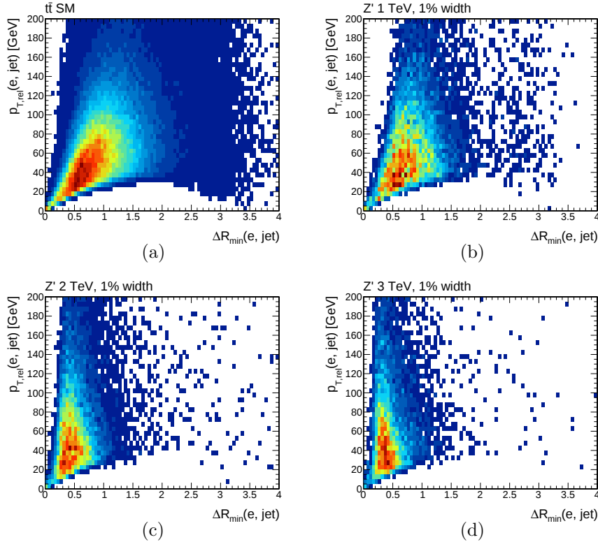
Figure 4.6: Two-dimensional distributions of \Delta R_{\min}(\ell, j) versus p_{T,\text{rel}}(\ell, j) for events passing the e + \text{jets} preselection, except for the lepton 2D-cut requirement. Distributions are shown for SM t\bar{t} production (a) and a Z' signal with 1%-width and M_{Z'} = 1 TeV (b), M_{Z'} = 2 TeV (c) and M_{Z'} = 3 TeV (d).
