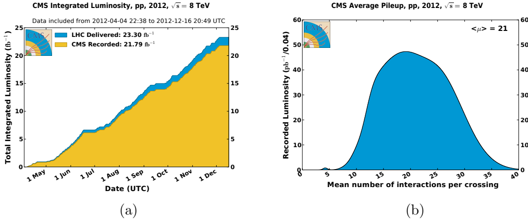
Figure 4.1: (a) Total integrated luminosity delivered to and recorded by the CMS experiment in 2012 in pp collisions at \sqrt{s} = 8 TeV. (b) Integrated luminosity in the CMS pp data set of 2012, as a function of the average number of pileup interactions.
