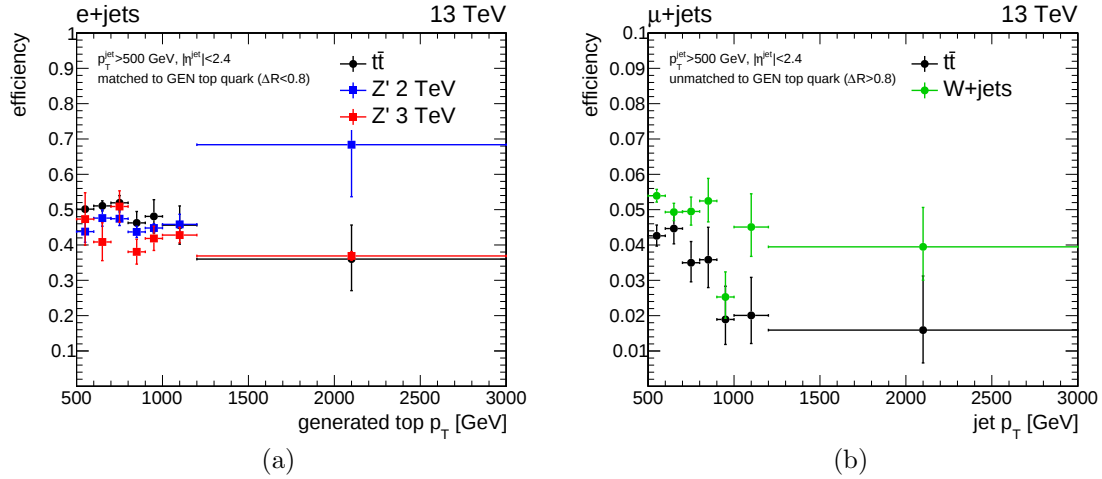
Figure 5.28: MC efficiencies for the t-tagging selection used in the \ell + \text{jets} analysis, based on the softdrop mass and \tau_{32} ratio. The efficiencies are measured in events passing the analysis selection described in Section 5.3.2: (a) t-tagging efficiency in the e + \text{jets} channel for AK8 jets matched to a generated top quark as a function of the generated top p_T , (b) t-mistag rate in the \mu + \text{jets} channel for AK8 jets unmatched to a generated top quark as a function of the jet p_T .
