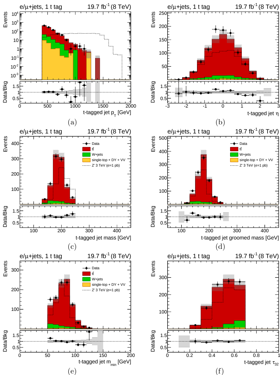
Figure 4.44: Data/MC comparison for the kinematics of the CA8 t-tagged jet in the T1 category of the \ell + jets SR: (a) jet p_T , (b) jet \eta , (c) jet ungroomed mass, (d) jet groomed mass, (e) subjects' minimum pairwise mass, (f) jet \tau_{32} . The expected background is determined after the fit described in the text. The background error band includes the MC statistical error and the overall post-fit systematic uncertainty; in the ratio plots, the statistical (light gray) and total uncertainty (dark gray) are shown separately. Each plot includes the distribution expected for a narrow-width Z' signal with M_{Z'} = 3 TeV normalized to a cross section of 1 pb, which corresponds to the theoretical cross section times a factor 670.
