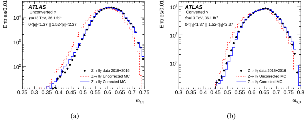
Figure 4.1: Distributions of the photon shower-shape variable w_{s3} in Z \rightarrow ll\gamma events in data and MC (before and after correction) for (a) unconverted and (b) converted photons [83].
