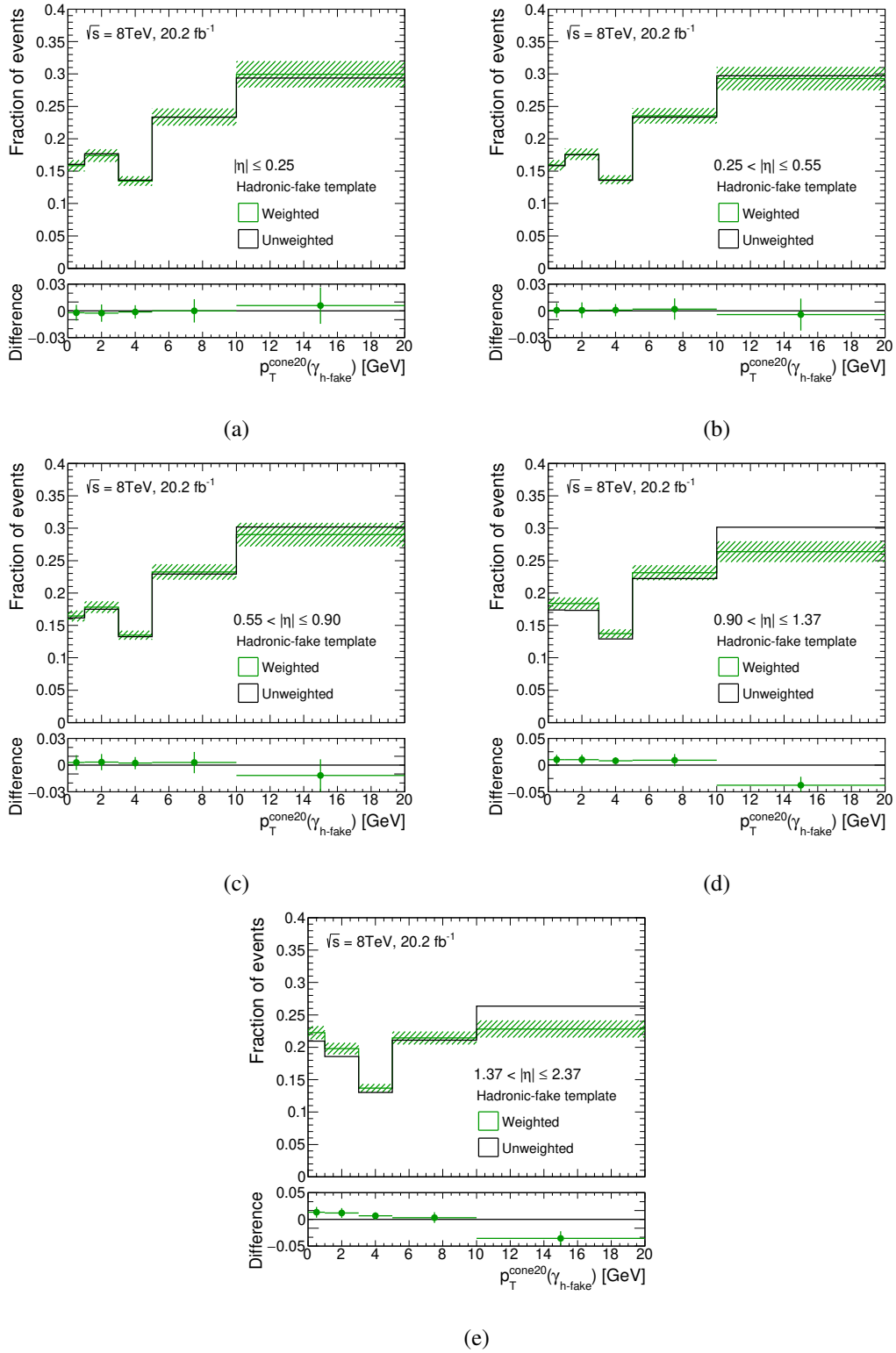
Figure 7.9: Hadronic-fake templates for differential fiducial measurements in photon \eta bins of (a) |\eta| \leq 0.25 , (b) 0.25 < |\eta| \leq 0.55 , (c) 0.55 < |\eta| \leq 0.90 , (d) 0.90 < |\eta| \leq 1.37 and (e) 1.37 < |\eta| \leq 2.37 , before (black) and after (green) re-weighting, with their difference shown in the lower panels. Distributions are normalised to unity and the last bin contains the overflow. The statistical uncertainties are too small to be visible, while the green bands show the weighting uncertainties. The weighted templates are the nominal templates used in the cross-section measurements.
