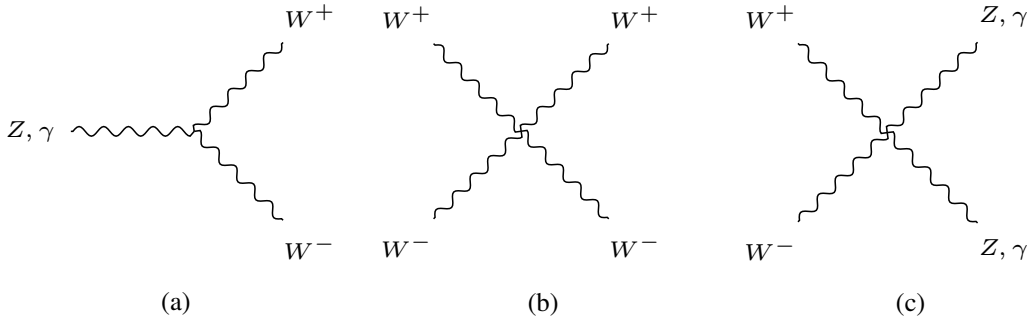
Figure 2.5: Feynman diagrams for Electroweak gauge bosons self-interaction.
