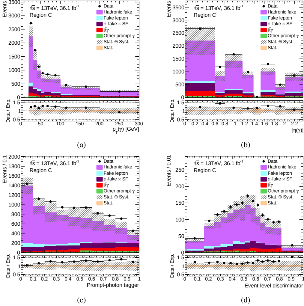
Figure 8.6: Plots of region C in single-lepton channel, where photons are non-isolated and identified as Tight. In each plot, the dashed area shows the total uncertainty of the total expectation while the solid band in the ratio panel shows the statistical uncertainty of the total expectation.
