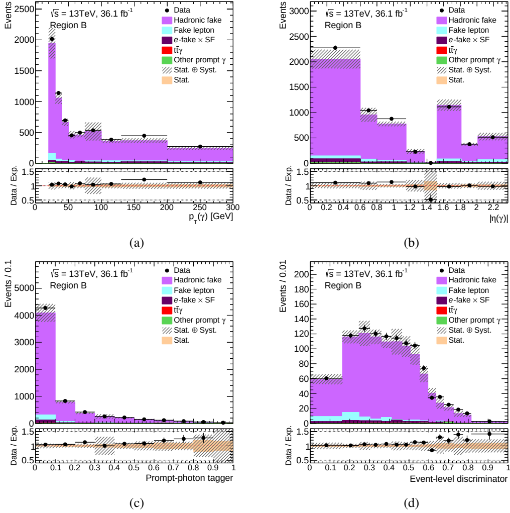
Figure 8.5: Plots of region B in single-lepton channel, where photons are identified as fail-Tight as well being non-isolated. In each plot, the dashed area shows the total uncertainty of the total expectation while the solid band in the ratio panel shows the statistical uncertainty of the total expectation.
