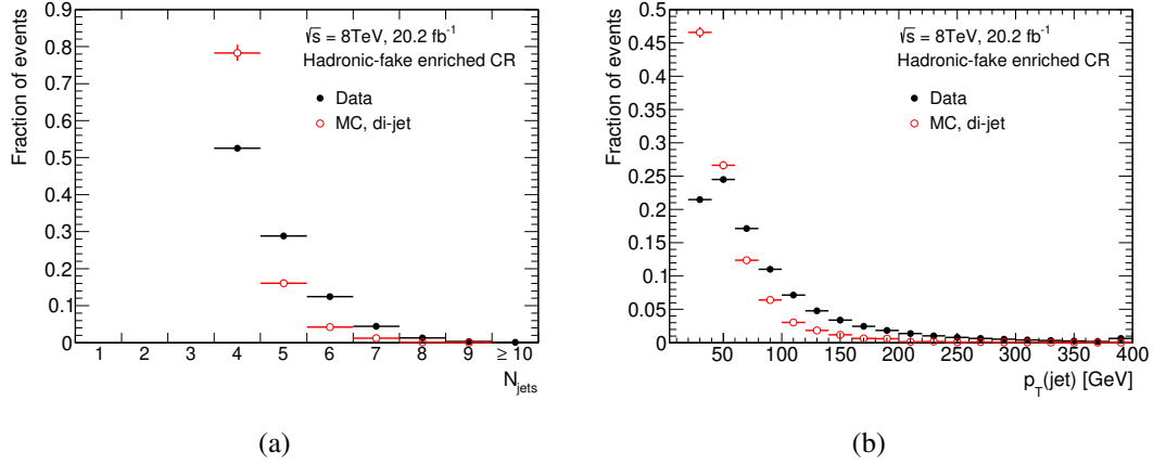
Figure 7.11: Comparison of the shape of (a) jet multiplicity and (b) jet p_{\text{T}} distributions between data and MC in the hadronic-fake enriched control region. Distributions are normalised to unity and the last bin contains the overflow.
