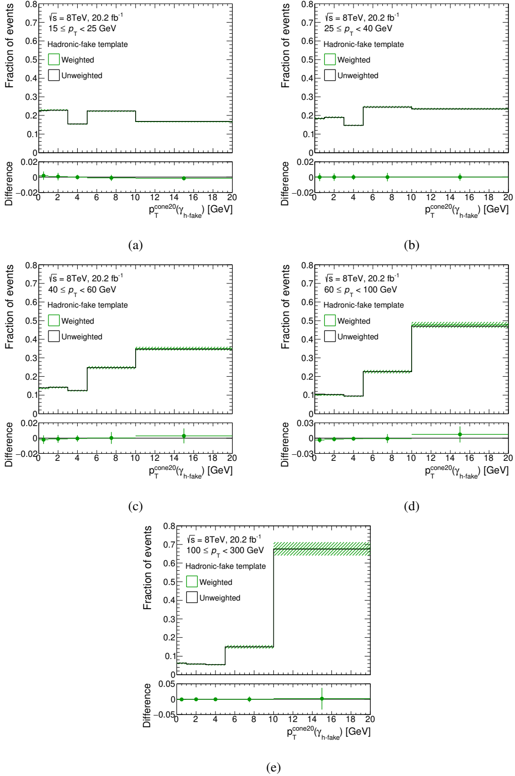
Figure 7.10: Hadronic-fake templates for differential measurements in photon p_T bins of (a) 15 \leq p_T < 25 GeV, (b) 25 \leq p_T < 40 GeV, (c) 40 \leq p_T < 60 GeV, (d) 60 \leq p_T < 100 GeV and (e) 100 \leq p_T < 300 GeV, before (black) and after (green) re-weighting, with their difference shown in the lower panels. Distributions are normalised to unity and the last bin contains the overflow. The statistical uncertainties are too small to be visible, while the green bands show the weighting uncertainties. The weighted templates are the nominal templates used in the cross-section measurements.
