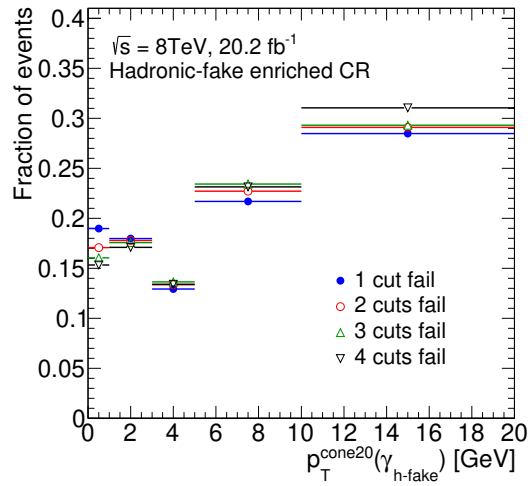
Figure 7.12: The p_{\text{T}}^{\text{cone20}} distribution of the hadronic-fake photon candidates in the hadronic-fake enriched control region in data selected by requiring exactly one to four specific Tight identification cuts to fail. The distributions are normalised to unity and the last bin contains the overflow. The statistical uncertainties are too small to be visible.
