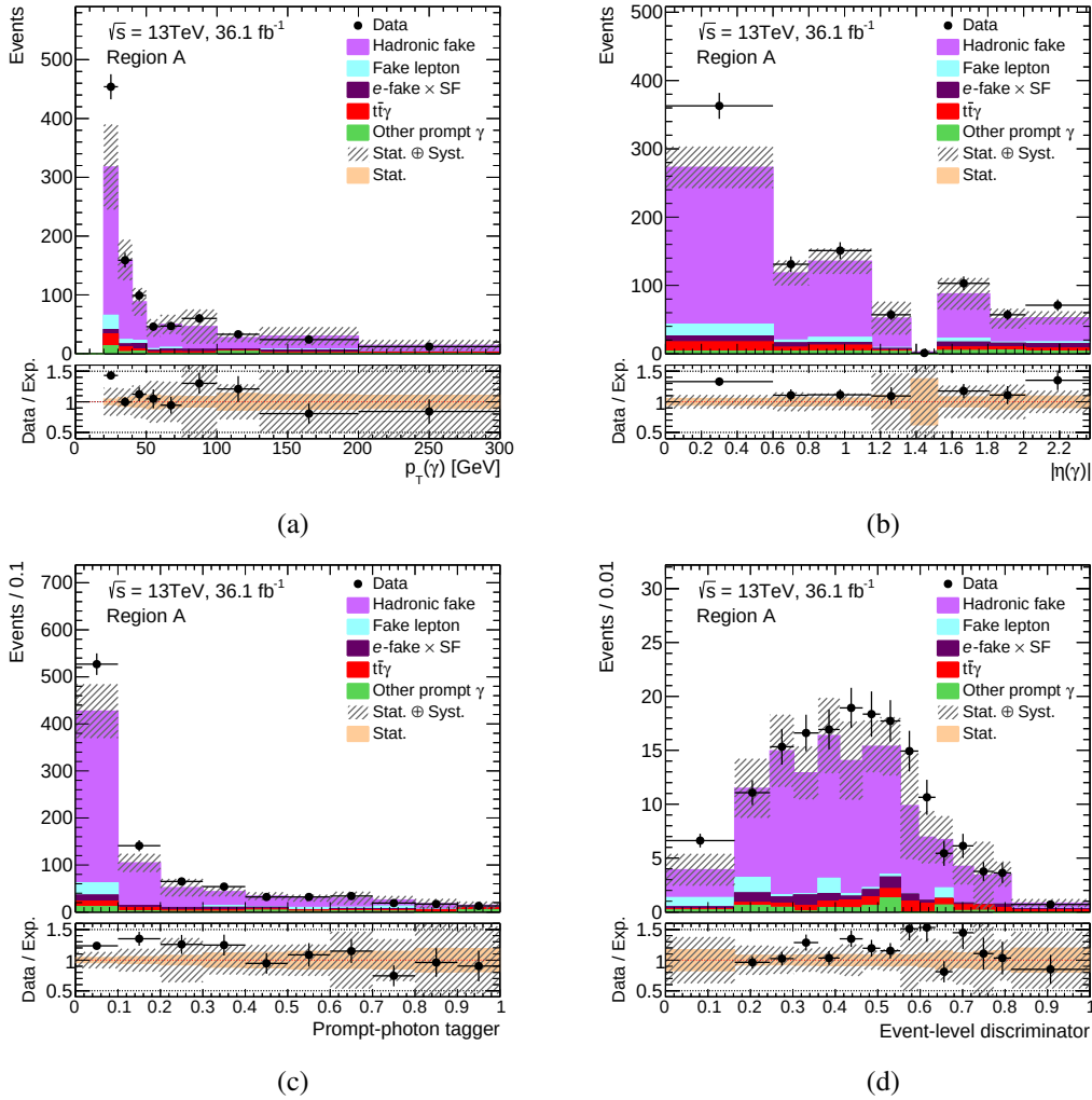
Figure 8.4: Plots of region A in single-lepton channel, where photons are isolated and identified as fail-Tight. In each plot, the dashed area shows the total uncertainty of the total expectation while the solid band in the ratio panel shows the statistical uncertainty of the total expectation.
