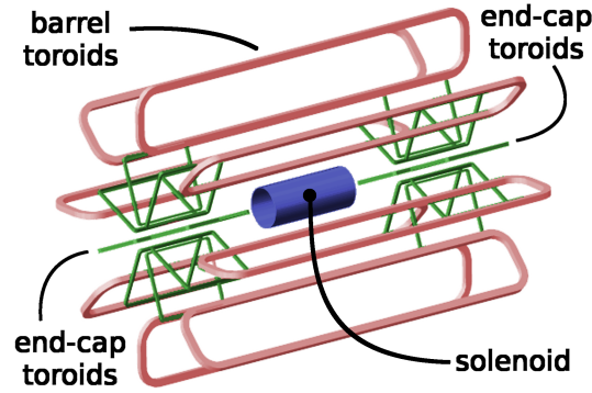
Figure 3.5: Layout of the ATLAS magnet system. Taken from Ref. [51].
