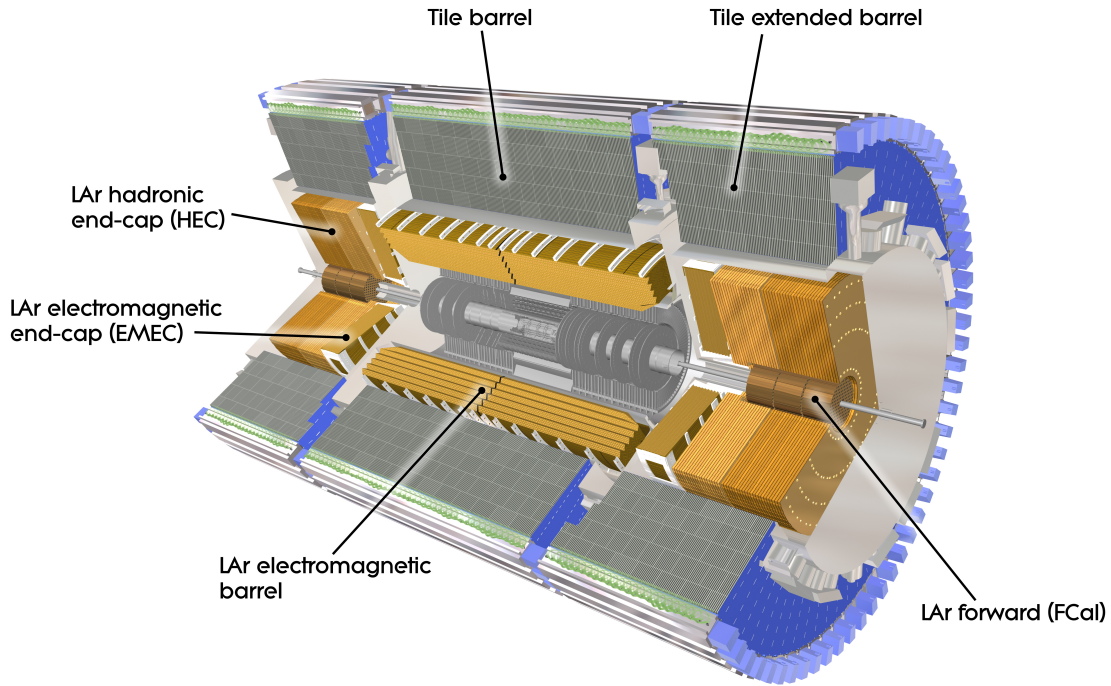
Figure 3.8: Cut-away views of the ATLAS calorimeters system [50].
