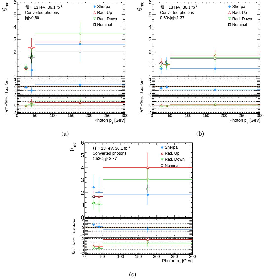
Figure 8.7: The MC-based double ratio \theta_{\text{MC}} measured in three different photon \eta slices as function of photon p_T for converted photons, from nominal MC and alternative MC samples that are used for systematic uncertainty evaluation. The error bars show the statistical uncertainties.
