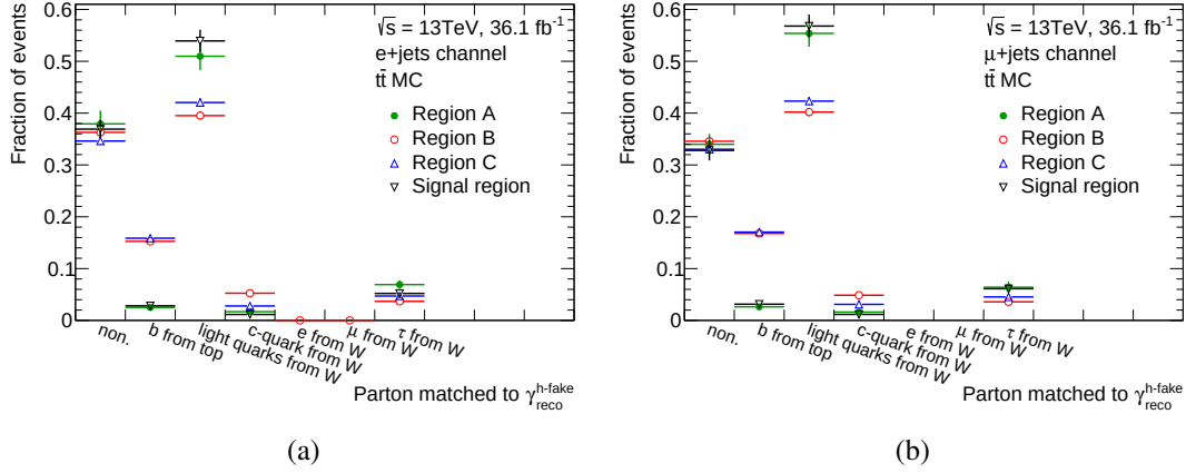
Figure B.3: Partons matched to a hadronic-fake photon in (a) e+\text{jets} and (b) \mu+\text{jets} channel, using t\bar{t} simulated sample. The first bin shows the fraction of events where no matched parton is found (within a \Delta R < 0.2 distance), therefore it includes the events with hadronic-fake photons originated from extra jets.
