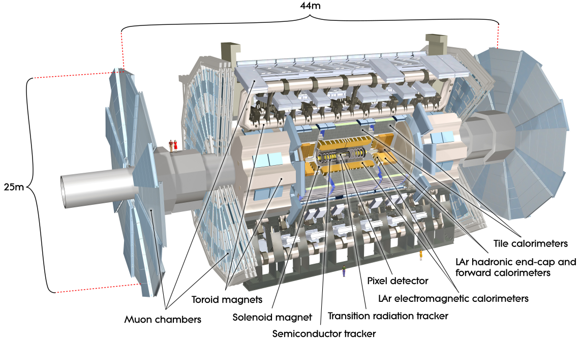
Figure 3.3: Cut-away view of the ATLAS detector [50].
