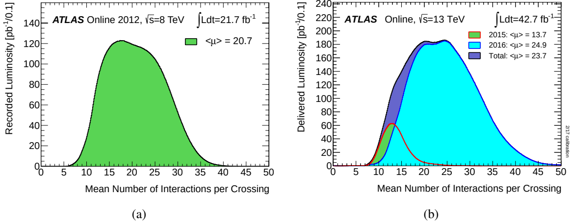
Figure 5.1: The average number of interactions per bunch crossing in pp collisions (a) at \sqrt{s} = 8 TeV during 2012 [86] (b) at \sqrt{s} = 13 TeV during 2015 and 2016 [87]. All data delivered to ATLAS during stable beams are shown.
