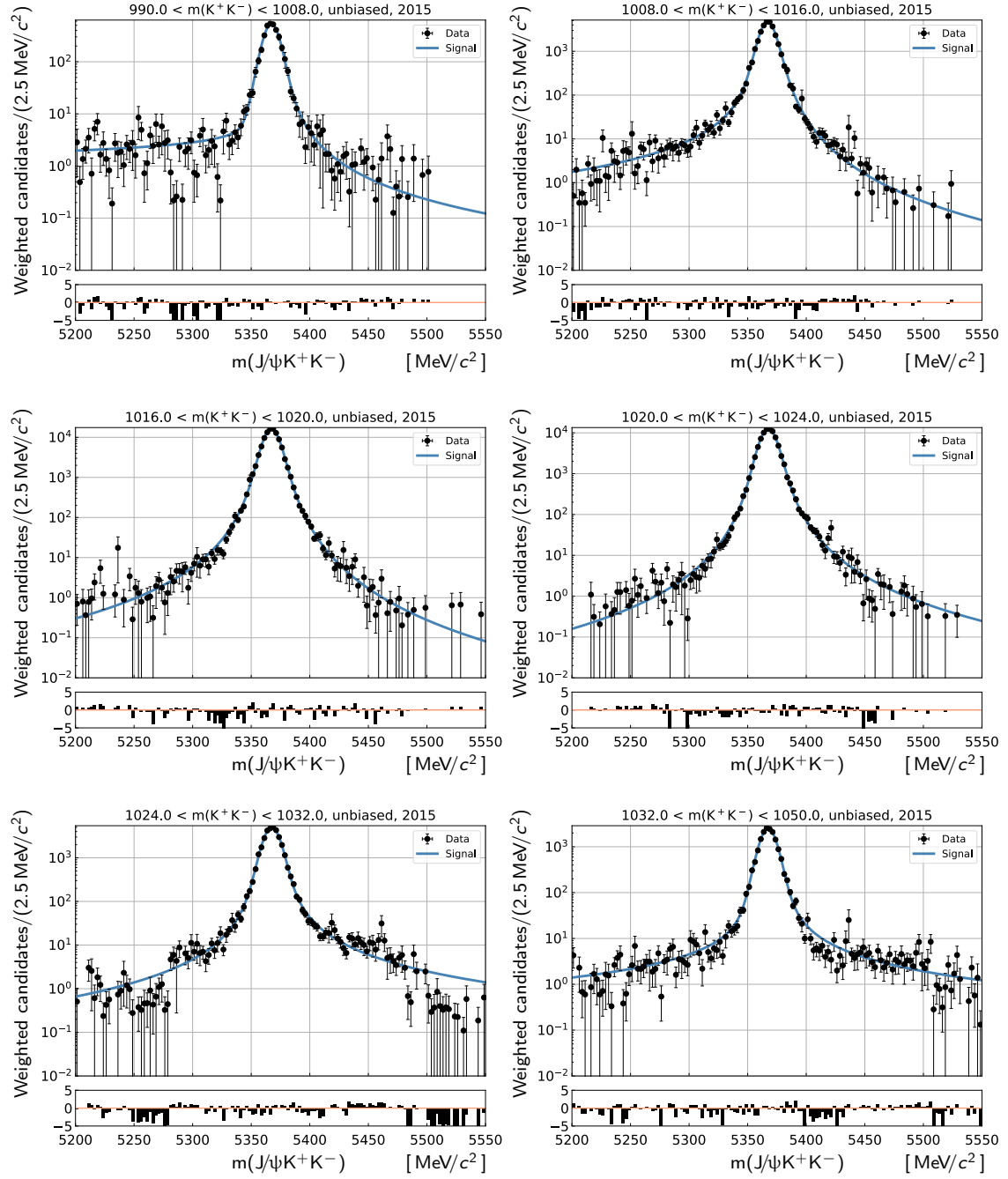
Figure A.2: Fit to the m(J/\psi K^+ K^-) distribution divided into six bins in m_{KK} , namely [990, 1008, 1016, 1020, 1024, 1032, 1050] \text{MeV}/c^2 , obtained in unbiased signal and FSR category of the 2015 simulation sample (solid blue line) and pull plot.
