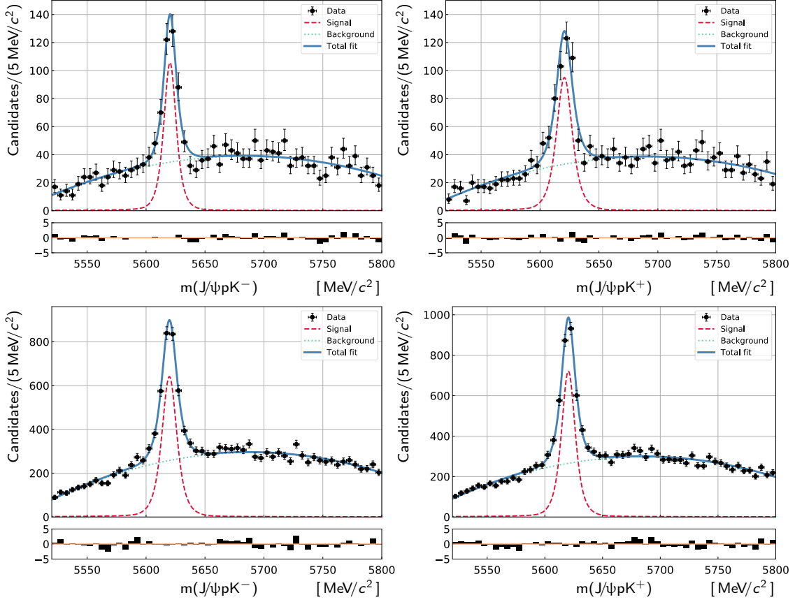
Figure 4.2: The invariant-mass distribution from J/\psi p K^- (left) and J/\psi \bar{p} K^+ (right) combinations obtained with 2015 (top) and 2016 (bottom) data sample.
