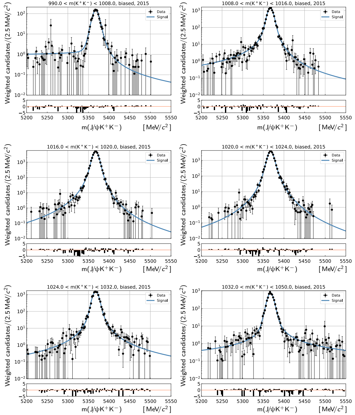
Figure A.1: Fits to the m(J/\psi K^+ K^-) distribution divided into six bins in m_{KK} , namely [990, 1008, 1016, 1020, 1024, 1032, 1050] MeV/c², obtained in the biased signal and FSR categories of the 2015 simulation sample (solid blue line) and pull plot.
