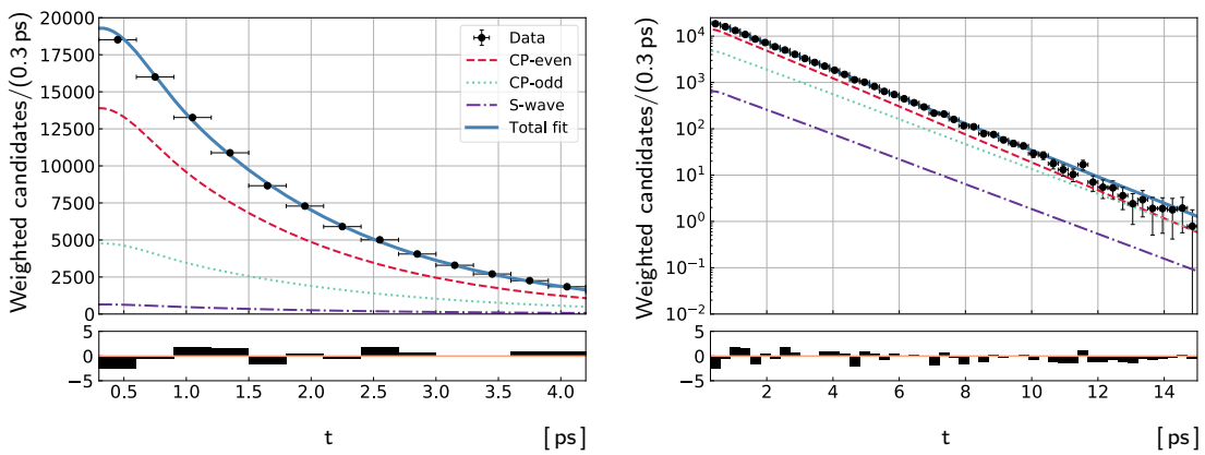
Figure 6.1: Decay-time distributions for background-subtracted B_s^0 \rightarrow J/\psi K^+ K^- decays (data points) with one-dimensional projections of the PDF at the maximum-likelihood point. The solid blue line shows the total signal contribution, which consists of (long-dashed red) CP-even, (short-dashed green) CP-odd and (dotted-dashed purple) S-wave contributions.
