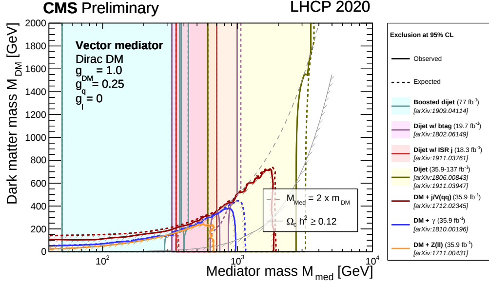
Figure 5.15: The 95% CL observed (solid) and expected (dashed) excluded regions in the plane of dark matter particle mass ( m_{\text{DM}} ) vs. mediator mass ( m_{\text{Med}} ), for vector mediators. The results are shown for dijet searches and different p_{\text{T}}^{\text{miss}} based DM searches from CMS. A branching fraction of 100% is assumed for a leptophobic vector mediator decaying to dijets. The exclusion is computed for a quark coupling choice g_q = 0.25 and for a dark matter coupling g_{\text{DM}} = 1 . The results of the search presented in this chapter are shown in light blue. The excluded regions from the dijet resolved analysis (Dijet + ISR) using early 2016 data [8] are also shown. Results are compared to constraints from the cosmological relic density of DM (light gray) determined from astrophysical measurements [150, 151] and MADDM version 2.0.6 [152, 153] as described in Ref. [154]. It should also be noted that the absolute exclusion of the different searches as well as their relative importance, will strongly depend on the chosen coupling and model scenario. Therefore, the exclusion regions, relic density contours, and unitarity curve shown in this plot are not applicable to other choices of coupling values or model. This figure is reproduced from Ref. [136].
