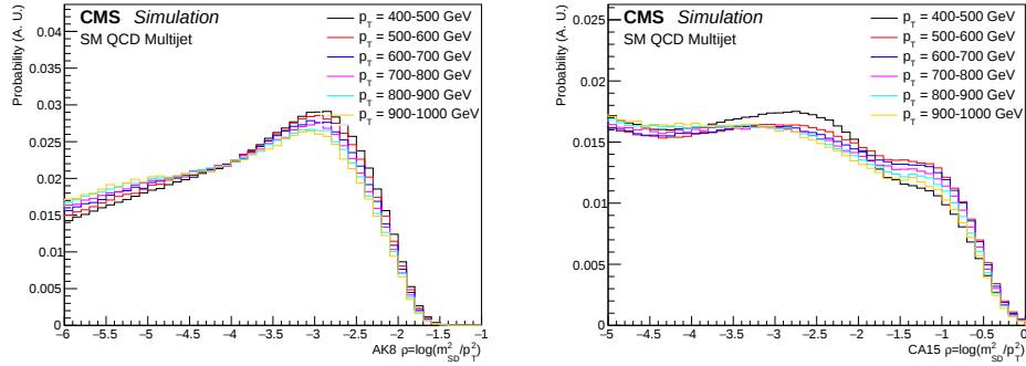
Figure 4.10: Shape of the jet \rho = \log \frac{m^2}{p_T^2} shown for QCD multijet events. The distributions are normalized to unity and shown for different p_T ranges and different radius parameters, for AK8 (left) and CA15 (right) jets.
