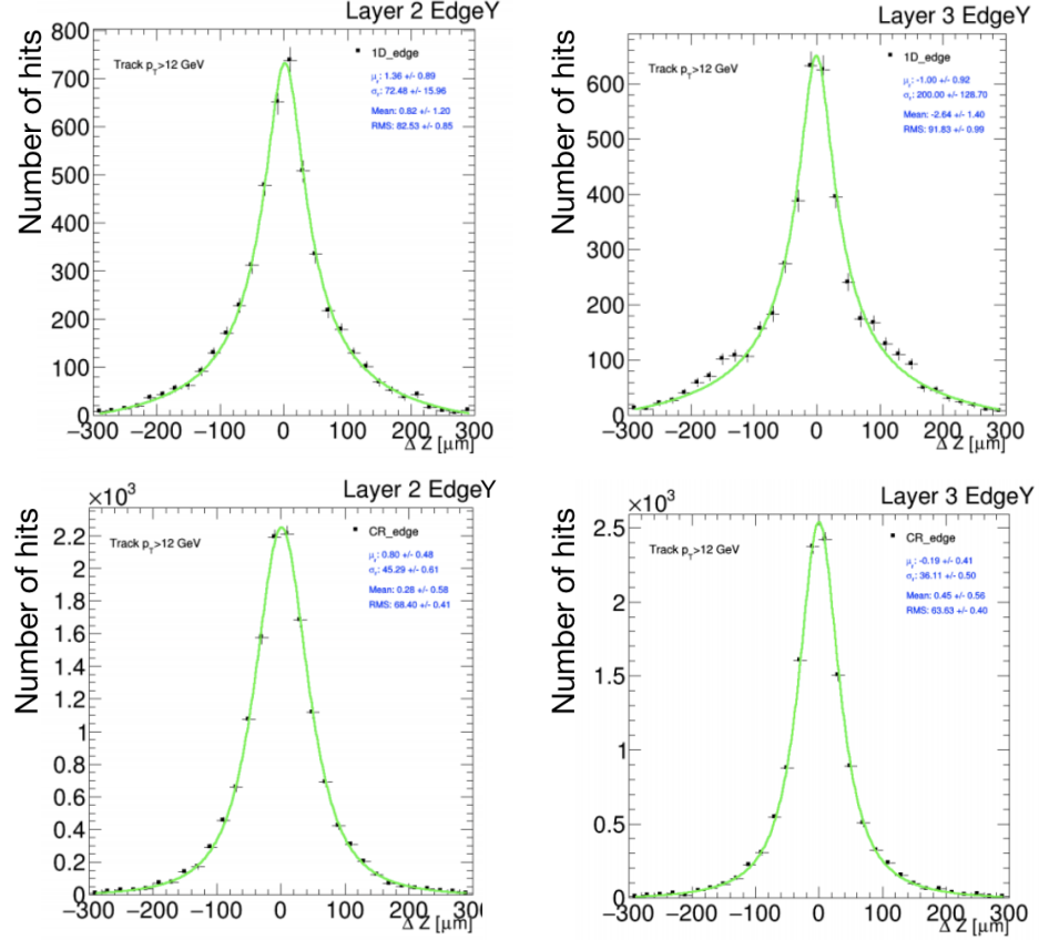
Figure 3.20: Hit residuals for physical-edge-y clusters in the layers 2 and 3 of the barrel inner tracker. The top panel shows residuals using the 1D-template reconstruction, which uses x – and y –projections of pre-determined cluster shapes to determine the hit position. The bottom panel shows residuals that use the full 2D information to fit the pre-determined cluster shapes to predict the hit position. These residuals in the z –direction were computed using a track re-fitting method. The method drops hits from a given layer, re-fits the track, and computes the residual by comparing the hit position from the re-fitted track with respect to the measured hit position. The resolution is improved by at least 20% in both layers, although edge clusters only represent in average 3% of the total number of clusters in an event.
