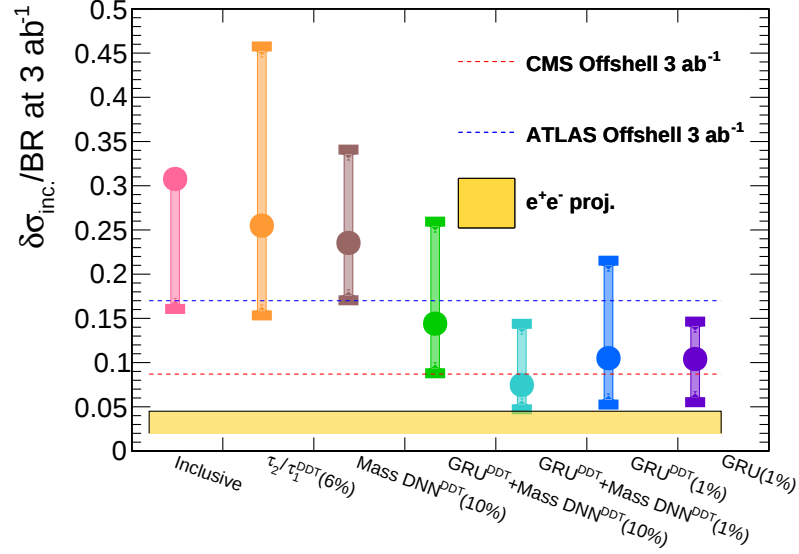
Figure 6.10: Estimated 1\sigma sensitivity for selections on various working points and discriminators extrapolated to 3 \text{ ab}^{-1} . For each point, the upper bound of the band indicates the sensitivity using a fourth-order Bernstein polynomial to fit the background. The lower bound of the band shows the result when no systematic uncertainties are included in the calculation and the point indicates the performance when a template fit is utilized for the signal extraction. The inclusive bin has a tadpole-like point indicating that the Bernstein polynomial fit did not converge. Our benchmark result, \text{GRU}^{\text{DDT}} + \text{mass} - \text{DNN}^{\text{DDT}} , results in a 1\sigma bound on the inclusive SM Higgs boson signal of \delta\sigma = 0.14 \times \sigma_{\text{SM}} . Additionally, we quote the projected extrapolations of the width for both the ATLAS and CMS off-shell interference analyses. This is done by taking the benchmark numbers used in Eq. 6.9 and subtracting the width uncertainty with the projected uncertainties on the various Higgs boson projection modes; if the projected uncertainties are reduced then the lines from the off-shell width measurements will increase. Lastly, we show a band for the quoted uncertainties from electron colliders. The various projected results range from 2% to 4.5% [181, 182, 192–194].
