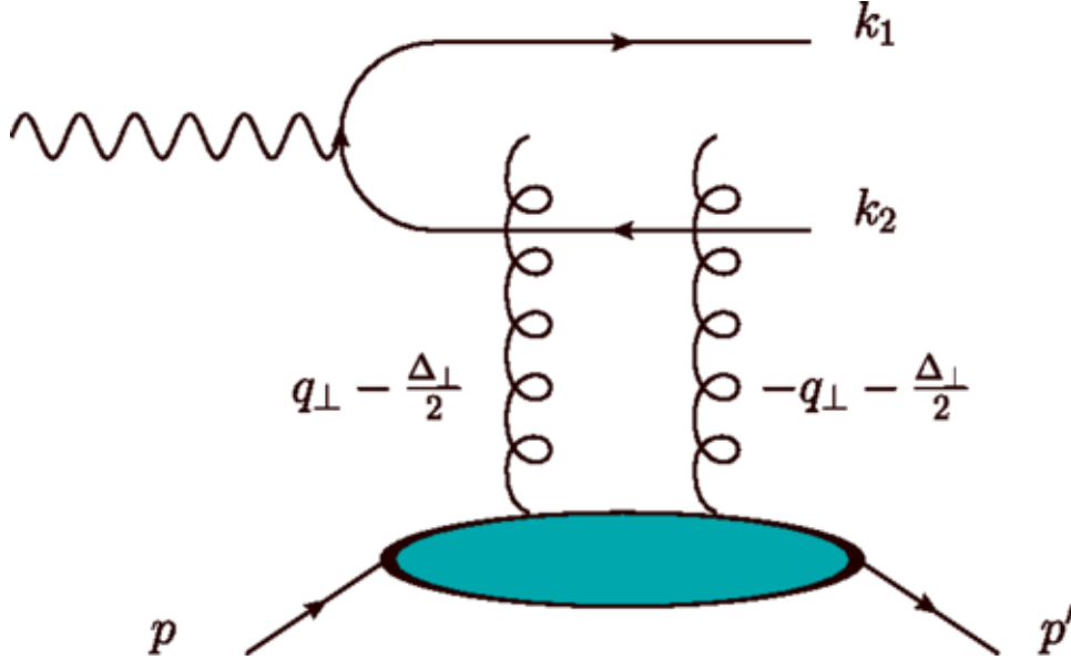
Figure 1.1: Feynman diagram of coherent dijets in dipole framework [12].
