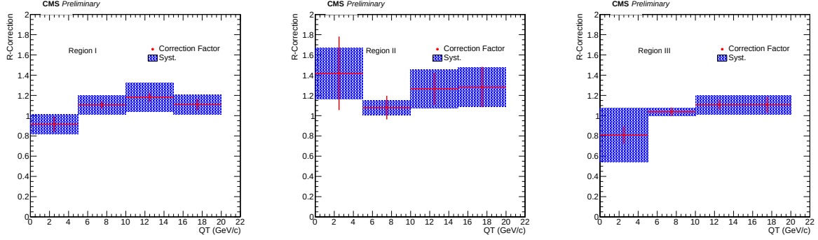
Figure 6.6: Resolution factor (R) including the systematic uncertainty for Regions I, II, and III (see text for details).
