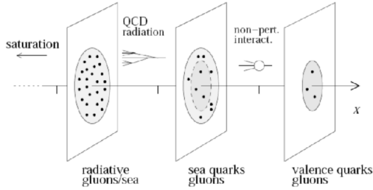
Figure 1.5: Subnuclear tomography. This figure illustrates that at higher energies the substructure of the hadron can be resolved until searching the gluon saturation regime. [33].
