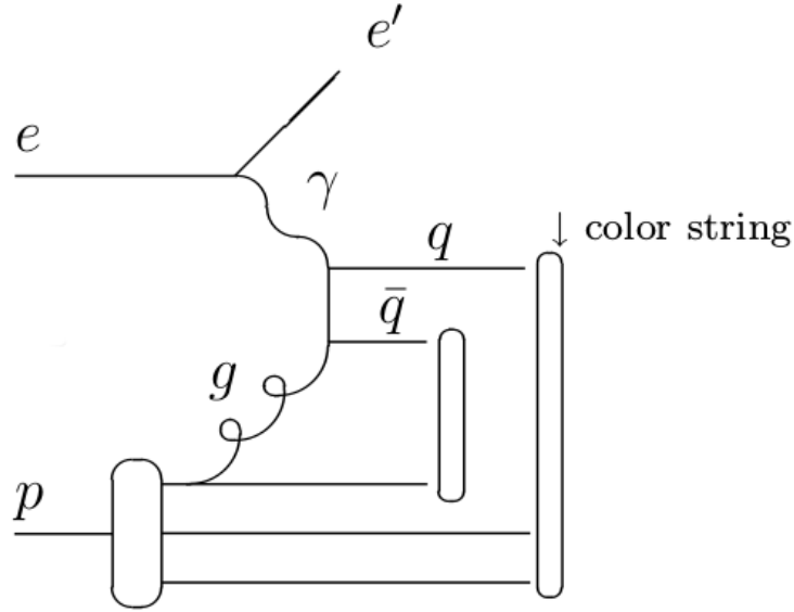
Figure A.1: RAPGAP process: boson-gluon fusion.
