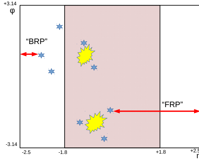
Figure 5.12: An example of an coherent dijet candidate, characterized by a large forward rapidity gap.
