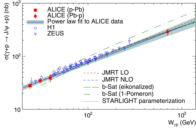
Figure 2.5: \gamma +proton \rightarrow J/\psi +proton cross section, showing the ALICE and HERA data [84].
