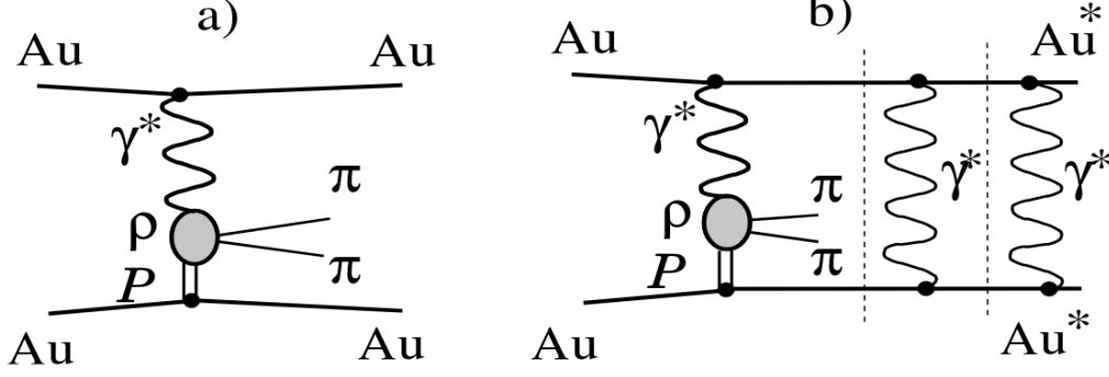
Figure 2.2: AuAu \rightarrow AuAu\rho^0 , (a.) UPC exclusive \rho^0 diagram, (b.) with mutual nuclei excitation [74].
