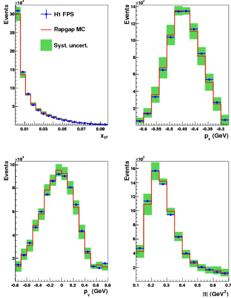
Figure 2.10: H1, diffractive e + p products, kinematics [104].
