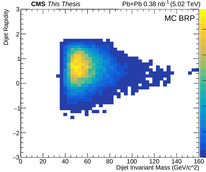
Figure 5.38: Scatter plot between the dijet rapidity and dijet invariant mass for BRP in the RAP-GAP+STARLIGHT and requiring Q_T < 20 GeV and P_T < 40 GeV.
