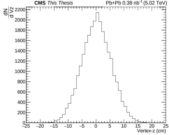
Figure 5.1: Measured vertex- z distribution for events that passed the trigger and dijet selection.
