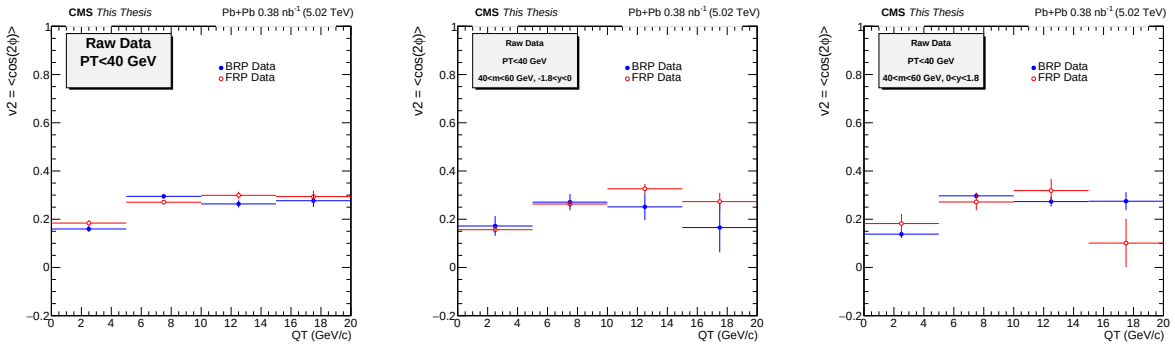
Figure 6.1: Raw data, differential analysis regions, LRG selection systematics on v_2 . The BRP results (blue points) and the FRP results (red points) are compared.
