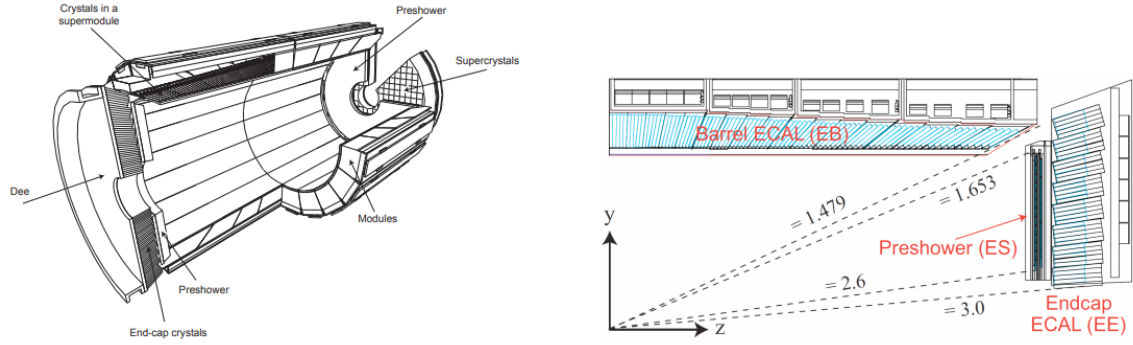
Figure 3.3: ECAL components [119].
