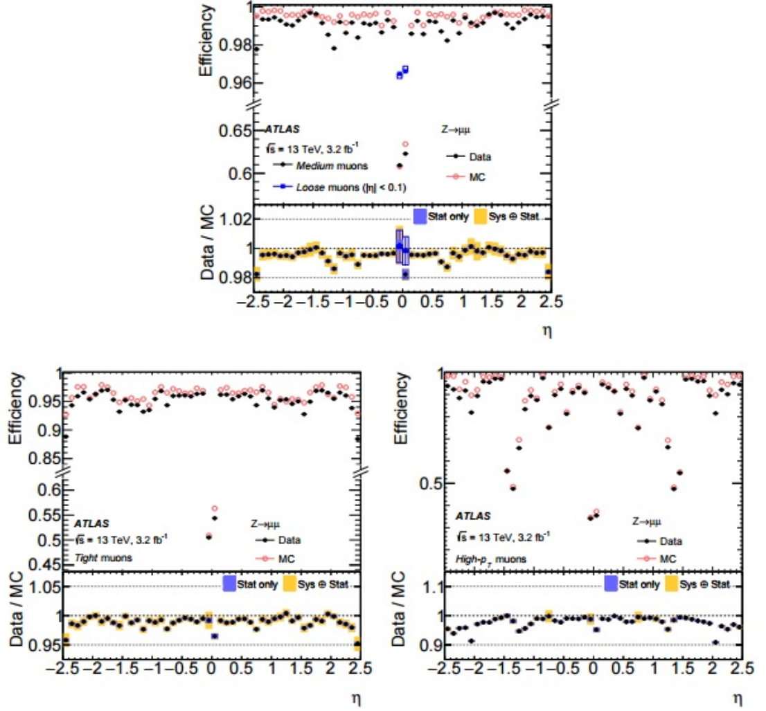
Figure 4.8: Muon reconstruction efficiency as a function of \eta for muons with p_T > 10 \text{ GeV} using Z \rightarrow \mu\mu sample, shown for medium and loose (top), tight (bottom left), and High- p_T (bottom right) muon selections. In addition, the top plot also shows the efficiency of the loose selection (squares) in the region |\eta| < 0.1 where the loose and medium selections differ significantly. Data is in black, MC in red [27].
