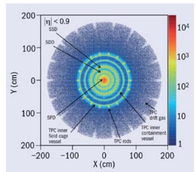
Fig. 1. Top left: Cross-section of the ALICE experiment in the X–Y plane as used in the 2012 run. Top right: Y-distribution versus X-distribution of the reconstructed photon conversion vertices for |\eta| < 0.9 .
