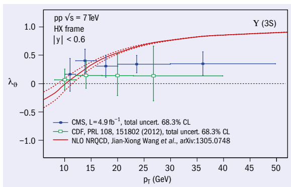
Polarization parameter \lambda_\theta as a function of p_T for \Upsilon(3S) , left, and \psi(2S) , right. The measurements of CDF and CMS are compared with predictions from NRQCD.
