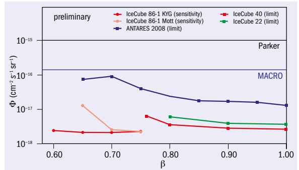
A summary of current flux limits on relativistic ( \beta > 0.6 ) monopoles, from the neutrino telescopes ANTARES and IceCube, together with an older limit from the MACRO experiment and the Parker bound. (Image credit: Anna Obertacke, Wuppertal.)
