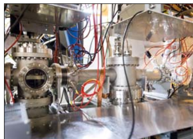
Above: Lasers are a key component at the ISOLDE facility. Right: The MR-TOF device at ISOLTRAP.
