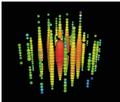
The two observed events from, left, August 2011 and, right, January 2012. Each sphere represents an optical module, where the size is a measure of the recorded number of photo-electrons. Colours represent the arrival times of the photons, where red indicates early and blue late times. (Image credit: IceCube collaboration.)
