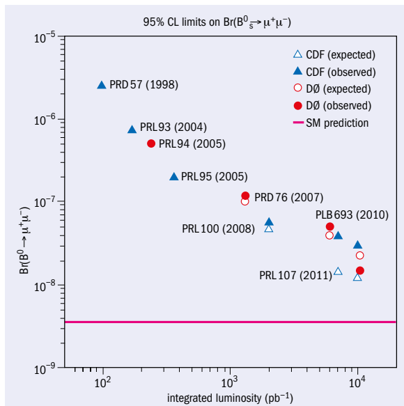
Fig. 5. Steady improvements in the search for rare decay B_s \rightarrow \mu\mu at the Tevatron over many years. These results excluded many models of beyond-Standard-Model physics, with the LHCb experiment observing evidence for this rare decay at the Standard-Model predicted level in late 2012.
