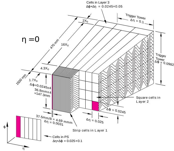
Figure 1.7: Sketch of a barrel module of the ATLAS Pb-LAr electromagnetic calorimeter, where the different layers are clearly visible. The granularities in \eta and \phi of the cells of each of the three layers, of the presampler and of the trigger towers are also shown.
