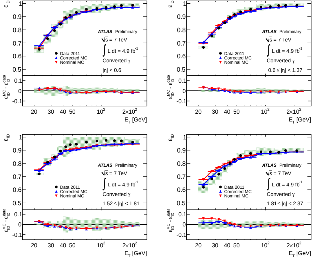
Figure 2.11: Comparison of the weighted mean of the data-driven measurements of converted \varepsilon_{ID} to the nominal and corrected MC predictions in the region 15 \text{ GeV} < E_T < 300 \text{ GeV} . The \varepsilon_{ID} curves are shown in four different \eta regions. The green uncertainty band corresponds to the addition in quadrature of the statistical and systematic uncertainties estimated for the combination of the data-driven methods. Only the statistical uncertainties are shown for the MC predictions. The bottom insets in each figure show the difference between the data-driven curve and nominal and corrected MC predictions.
