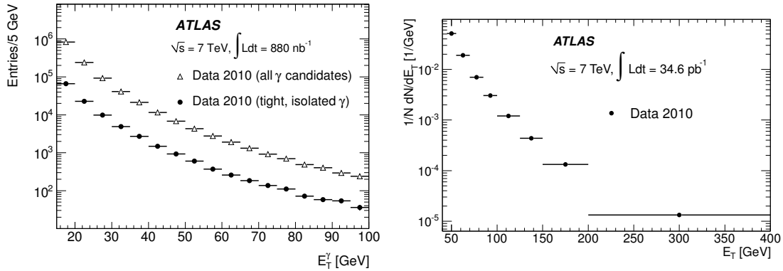
Figure 3.5: Left: transverse energy distribution of photon candidates selected in 0.88 \text{ pb}^{-1} of pp collisions at \sqrt{s} = 7 TeV, before (open triangles) or after (full circles) requiring tight identification criteria and isolation transverse energy lower than 3 GeV [14]. Right: transverse energy distribution of photon candidates in 35 \text{ pb}^{-1} of pp collisions at \sqrt{s} = 7 TeV, after the final selection [15].
