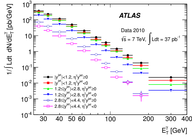
Figure 3.15: Transverse energy distribution of photon candidates in photon+jet candidate events selected in the pp collisions at \sqrt{s} = 7 TeV collected by ATLAS in 2010. The distribution is normalized by the integrated luminosity and the transverse-energy bin width.
