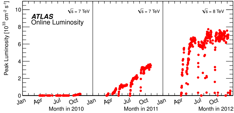
Figure 1.1: The peak instantaneous luminosity delivered to ATLAS per day versus time during the pp LHC runs of 2010, 2011 and 2012. The ATLAS online luminosity measurement is used.
