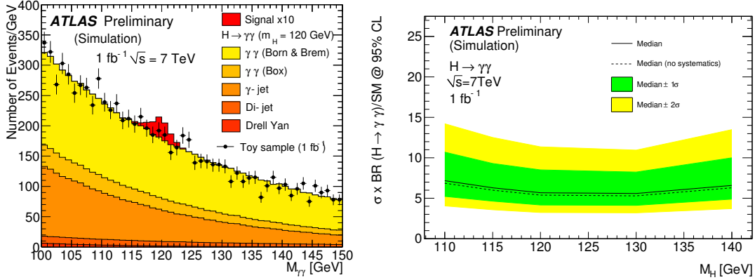
Figure 4.5: Left: expected invariant mass distribution of di-photon candidate events selected at \sqrt{s} = 7 \text{ TeV} for an integrated luminosity of 1 \text{ fb}^{-1} . The SM Higgs boson contribution is enhanced by a factor 10. Right: estimated median number of Standard Model signal cross-section excluded at 95% C.L. as a function of the Higgs mass for the same amount of data, using the CL_s technique. The green and yellow bands represent the range in which we expect the observed limit to lie (at 68% and 95% C.L. respectively), depending on the data.
