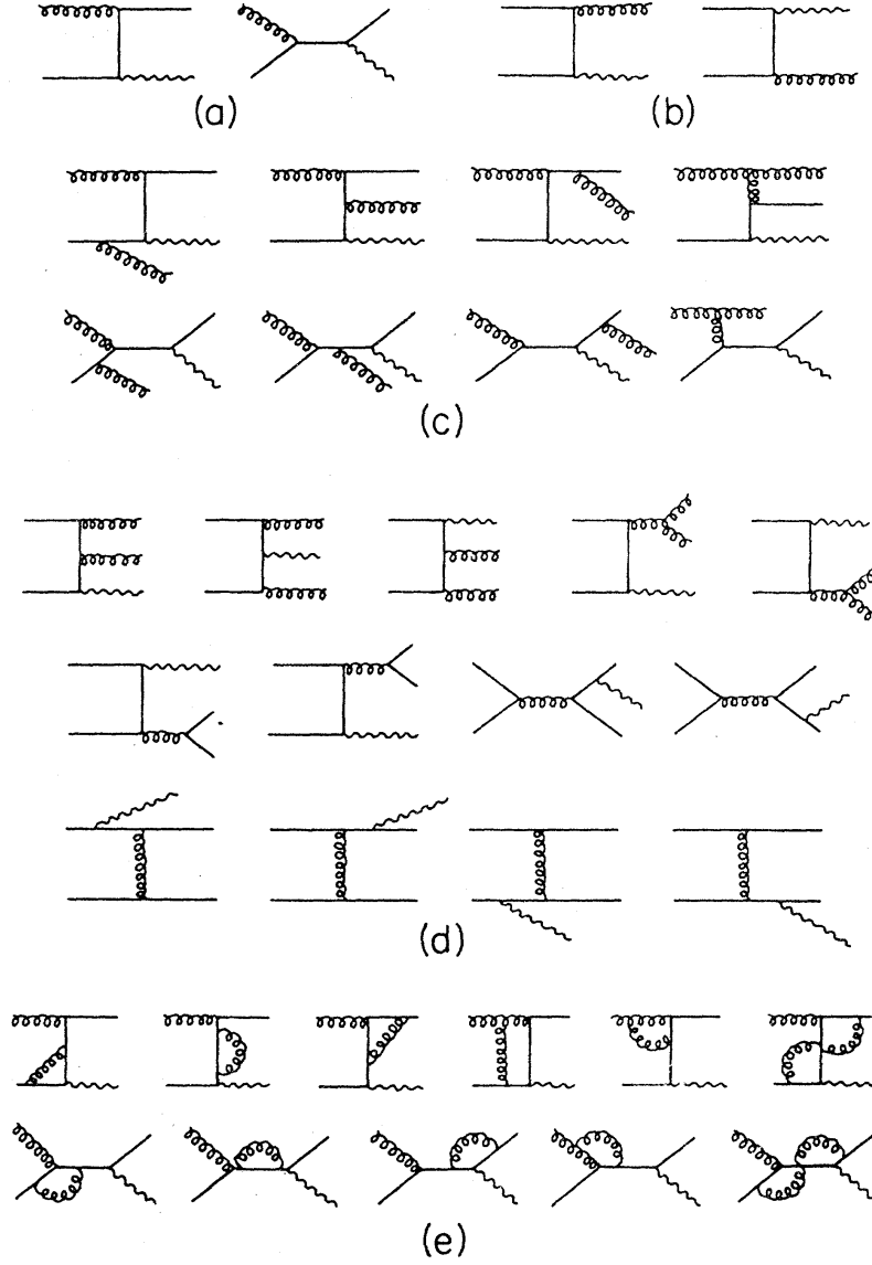
Figure 3.1: Selection of Feynman diagrams for prompt photon production: (a) \mathcal{O}(\alpha\alpha_s) Compton subprocess, qg \rightarrow q\gamma (and \bar{q}g \rightarrow \bar{q}\gamma ); (b) \mathcal{O}(\alpha\alpha_s) annihilation subprocess, q\bar{q} \rightarrow g\gamma ; (c) \mathcal{O}(\alpha\alpha_s^2) subprocess qg \rightarrow \gamma qg (and \bar{q}g \rightarrow \gamma \bar{q}g ); (d) \mathcal{O}(\alpha\alpha_s^2) subprocesses q\bar{q} \rightarrow \gamma gg and q\bar{q} \rightarrow \gamma q\bar{q} ; (e) one-loop graphs for the Compton subprocess that contribute to the \mathcal{O}(\alpha\alpha_s^2) calculation [129].
