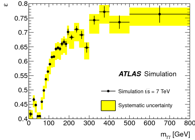
Figure 2.13: Efficiency of the tight identification criteria as a function of the di-photon invariant mass, from a corrected simulation of SM isolated-photon pair events where the two photons have E_T > 25 and 22 GeV, respectively [18]. Systematic uncertainties are included. The curve corresponds to the photon identification criteria used for the analysis of the \sqrt{s} = 7 TeV ATLAS data collected in 2011.
