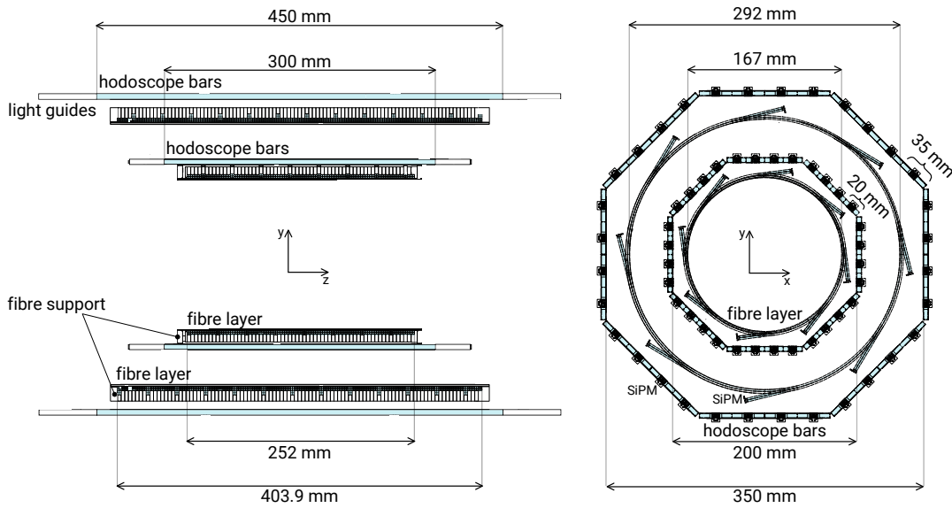
Fig. 4.1.: Cross sections of the hodoscope in the y-z plane (left) and x-y plane (right). In the left the hodoscope bars with lightguides as well as the fibre layers including their support are shown and on the right also the SiPM positions are shown. The dimensions of the parts are indicated [16].
