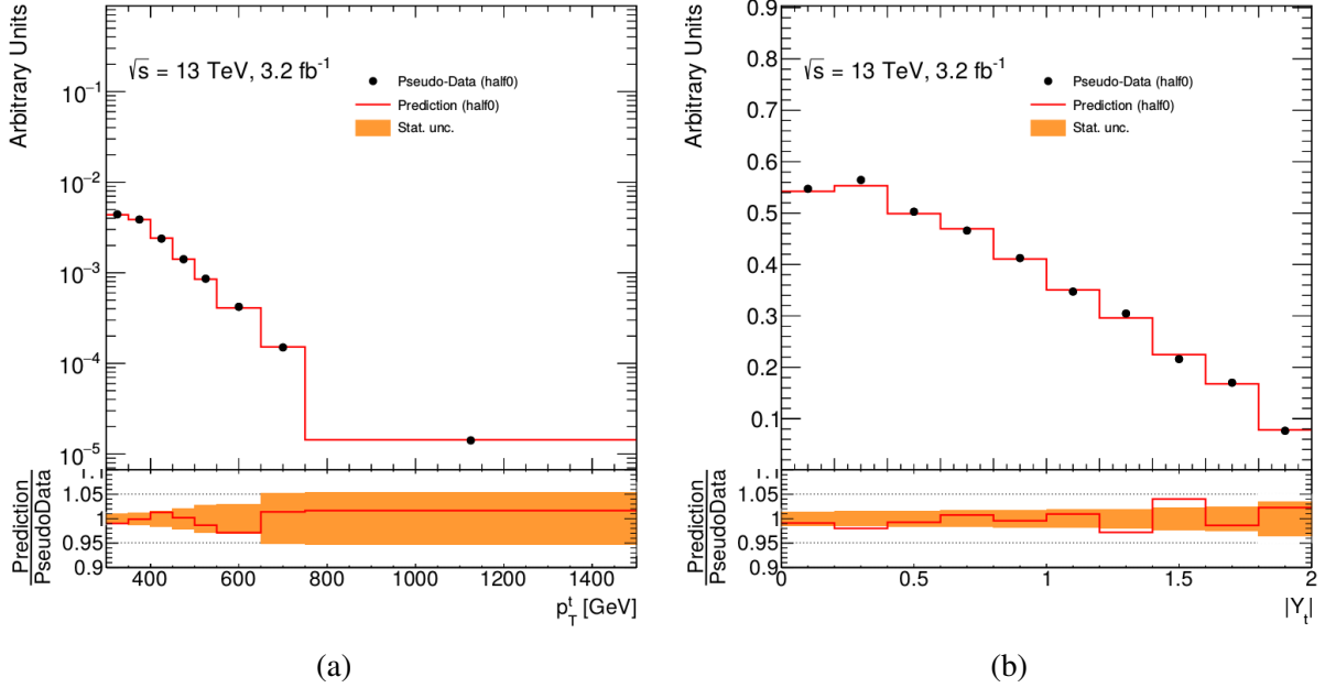
Figure 7.10: The (a) p_T^{t, \text{had}} , and (b) |y_t^{t, \text{had}}| closure tests, comparing the actual particle level distribution (labelled “prediction”) with the unfolded detector level distribution (labelled “pseudo-data”).
