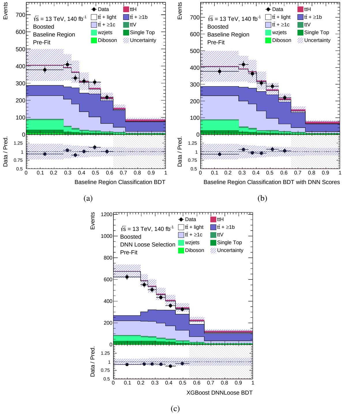
Figure 9.31: The data and MC distributions, for (a) the retrained baseline BDT, (b) the baseline+DNN BDT, and (c) the DNN region BDT. Bins which contain more than 5% signal in MC are blinded in data. The hashed area represents the systematic uncertainties including only the instrumental systematics.
