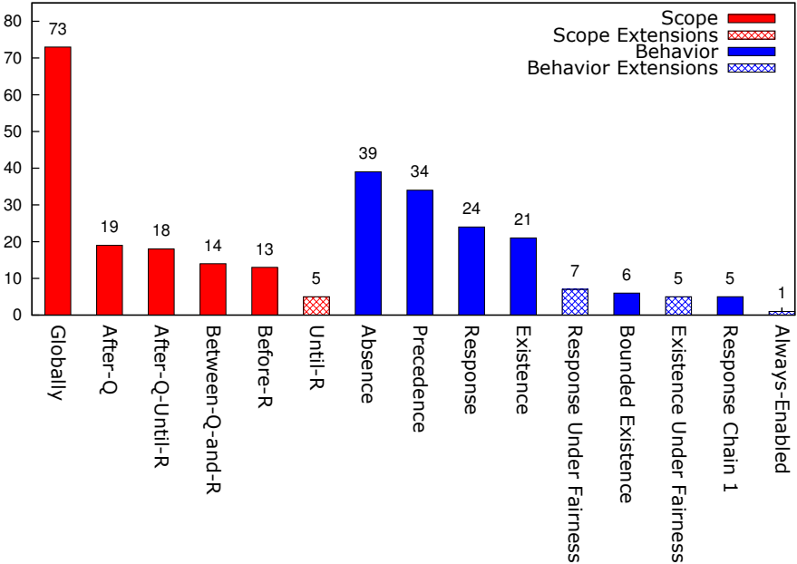
Figure 5.18: Survey of \mu -calculus specifications: patterns distribution
