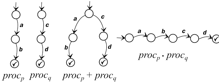
Figure 3.4: Alternative and sequential process composition
