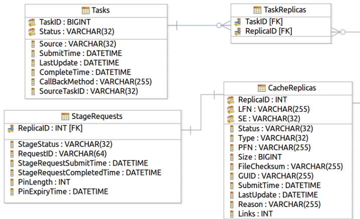
Figure 2.8: Relationships between StorageManagement DB entities
