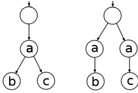
Figure 5.4: Branching versus linear time Logic
