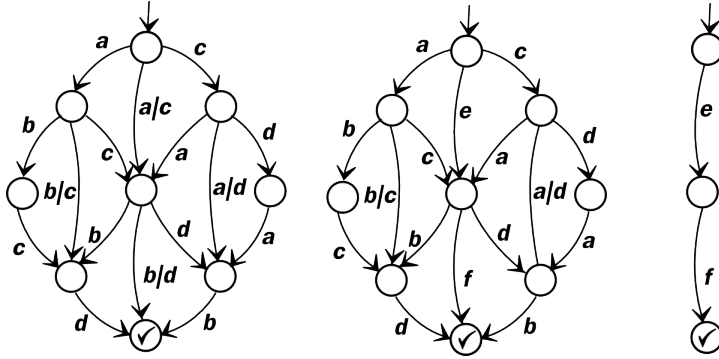
Figure 3.5: Parallel process composition.
