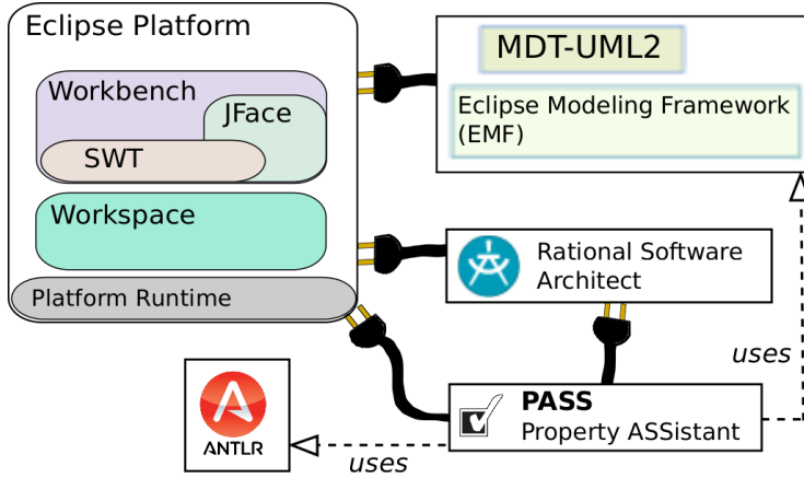
Figure 5.9: PASS integration in Eclipse
