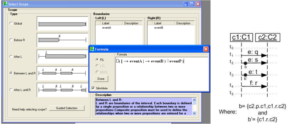
Figure 5.2: Left: Prospector tool; right: CHARMY PSC graphical notation
