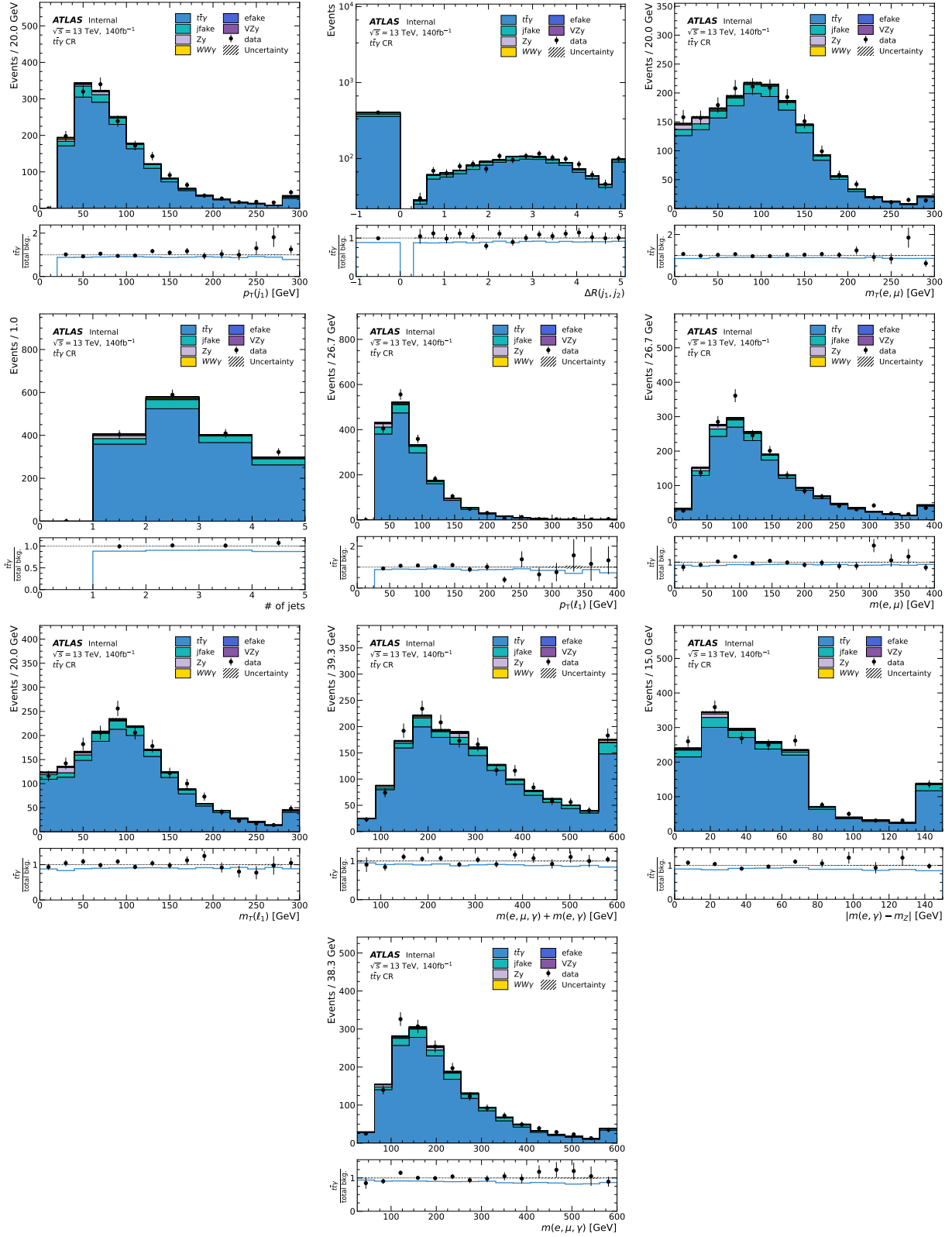
Figure 4.11: Various kinematic distributions in the t\bar{t}\gamma CR. Uncertainty is statistical only. Last bin includes overflow. \Delta R(j_1, j_2) < 0 indicates < 2 jets in the event.
