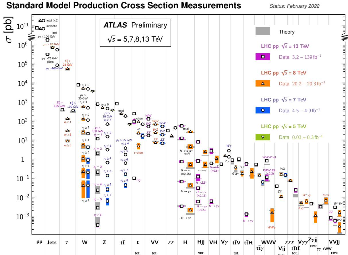
Figure 2.3: Standard Model production cross section measurements by the ATLAS experiment. Triboson production processes like W^{\pm}W^{\mp}\gamma are rarer than diboson production processes by an order of magnitude or more. There is good experimental agreement with theory across many diverse final states. Source: Ref. [11].
