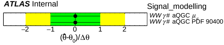
Figure 6.18: Signal modeling nuisance parameter pulls and constraints in the M0 EFT fit.
