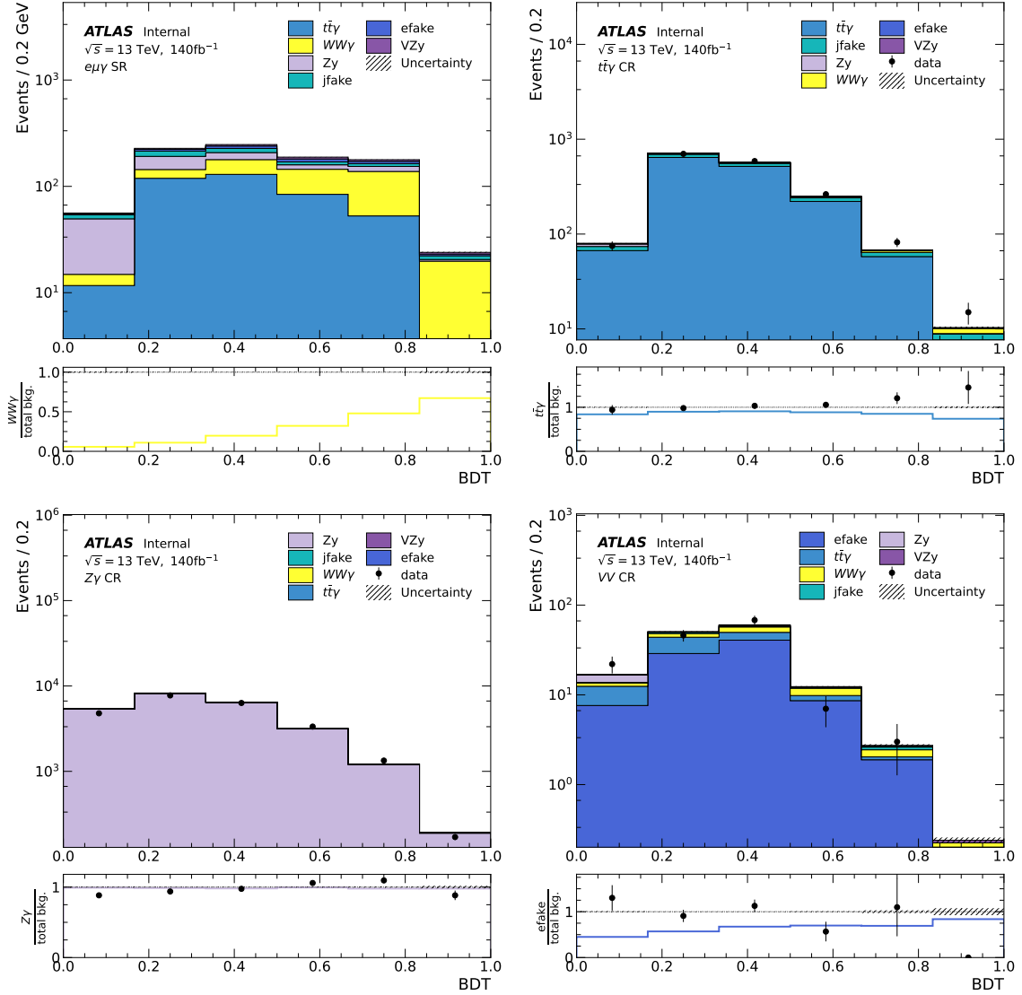
Figure 5.8: BDT distribution in the e^\pm\mu^\pm\gamma SR (top left), t\bar{t}\gamma CR (top right), Z\gamma CR (bottom left), and VV CR (bottom right).
