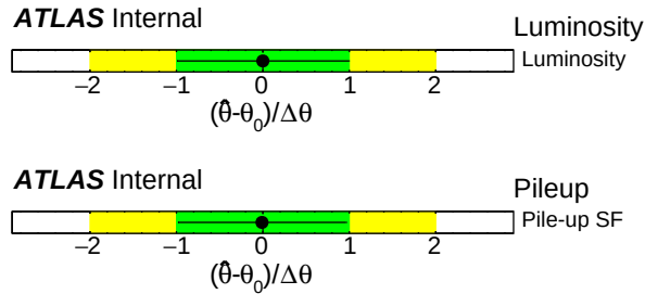
Figure 5.12: Luminosity and pile-up nuisance parameter pulls and constraints.
