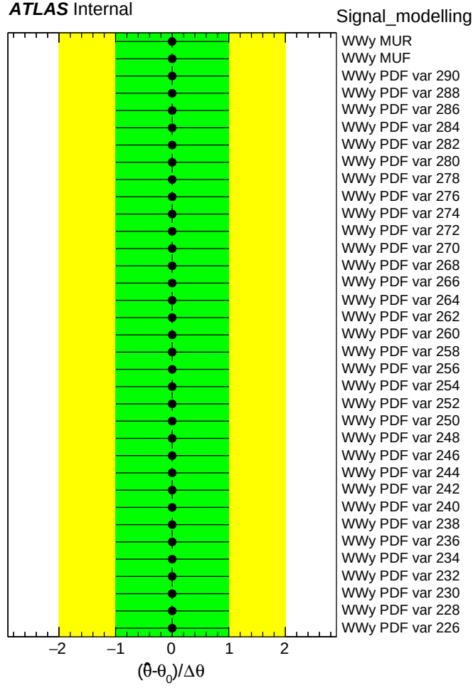
Figure 5.13: Signal modeling nuisance parameter pulls and constraints.
