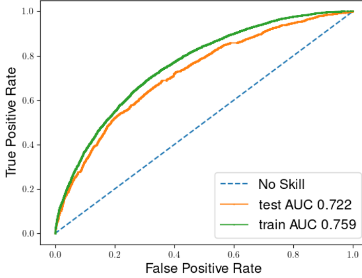
Figure 5.7: ROC curves for the training and test set of one fold of the BDT in the e^\pm\mu^\mp\gamma SR.
