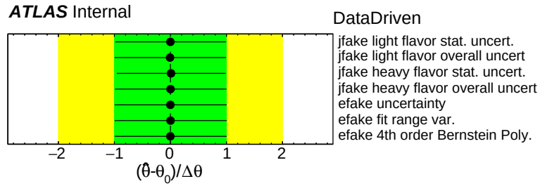
Figure 5.16: Data driven nuisance parameter pulls and constraints.
