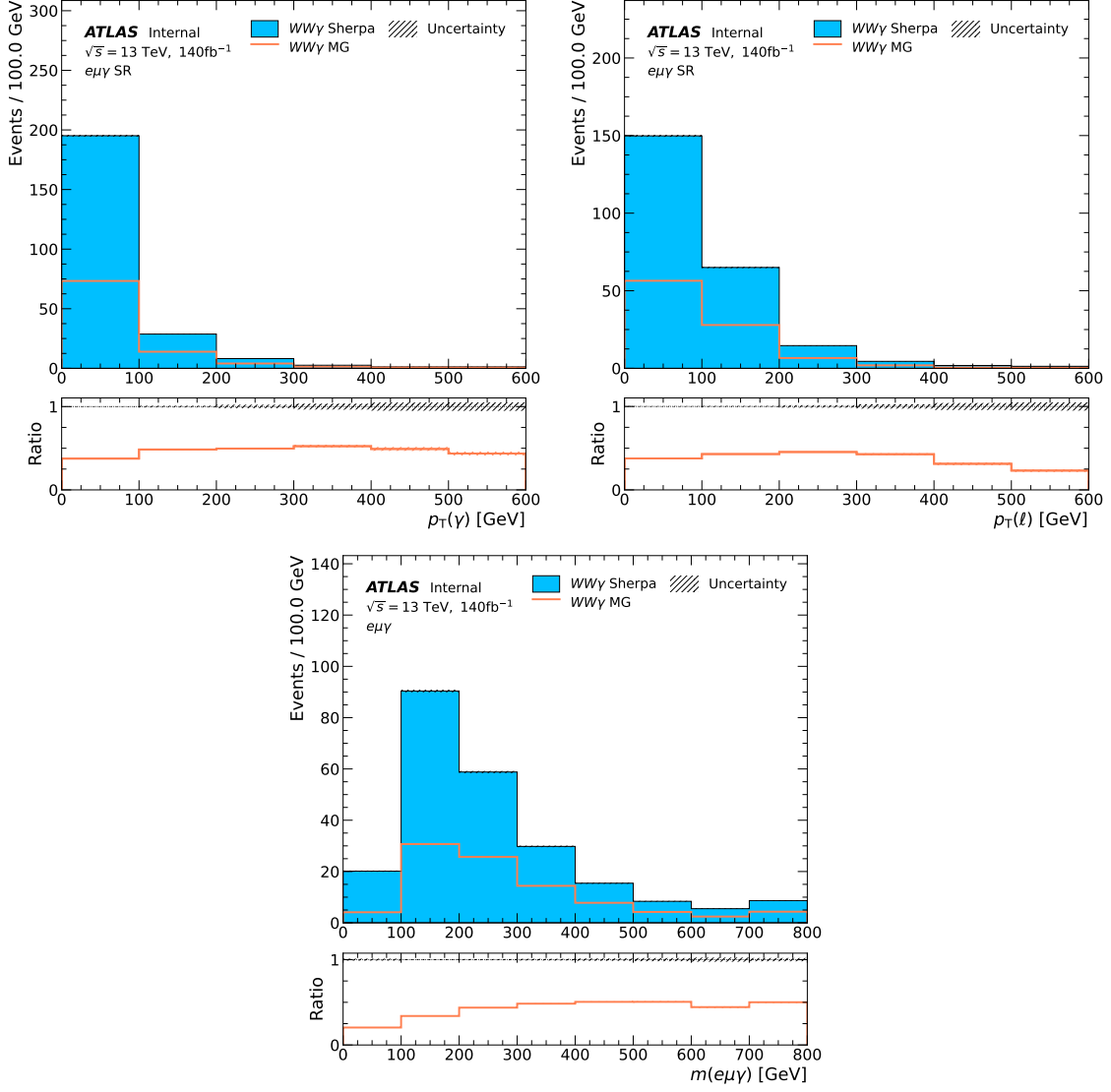
Figure 6.2: Distributions of p_T(\gamma) (upper left), p_T(\ell_1) (upper right), and m(e, \mu, \gamma) (bottom) in the inclusive e^\pm\mu^\mp\gamma region comparing the W^\pm W^\mp\gamma SM SHERPA and MADGRAPH samples. Uncertainties are statistical only. Last bin includes overflow.
