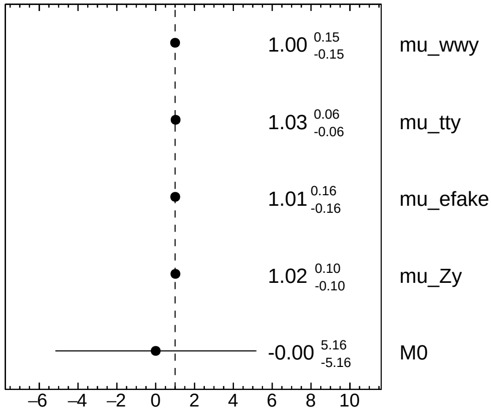
Figure 6.15: Best-fit normalization factors for the M0 Wilson coefficient, W^\pm W^\mp \gamma , t\bar{t}\gamma , Z\gamma , e \rightarrow \gamma fakes with \pm 1\sigma uncertainties.
