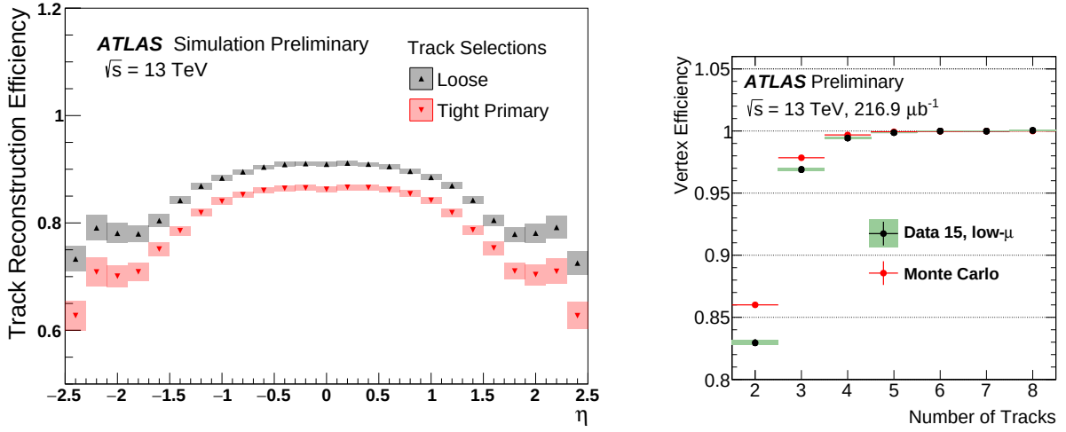
Figure 4.2: (Left) Track reconstruction efficiency vs. \eta ; efficiency is about 85-90% in the central region of the detector. Source: Ref. [64] (Right) Vertex reconstruction efficiency vs. \# of tracks; efficiency exceeds 95% when at least 3 tracks are present. Source: Ref. [65]
