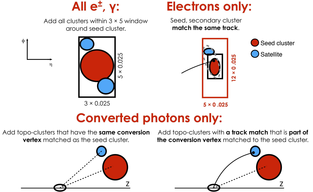
Figure 4.4: Track-matching criteria used for EM supercluster-building. Source: Ref. [70]
