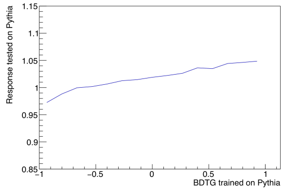
Figure 6: Average response of jets with a certain classifier output.
