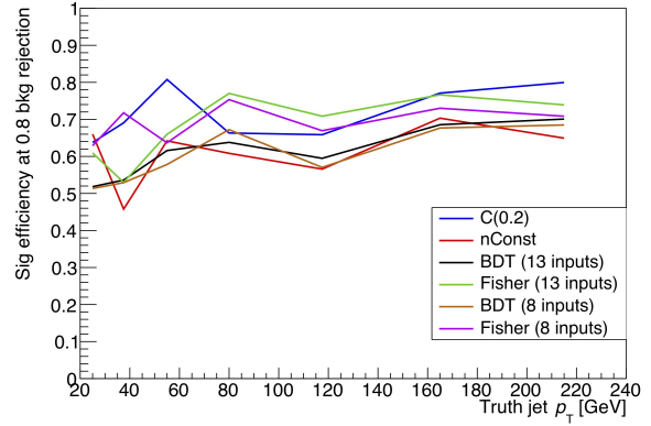
Figure 5: Signal efficiency of four MVA classifiers trained on Pythia at 80% background rejection.
