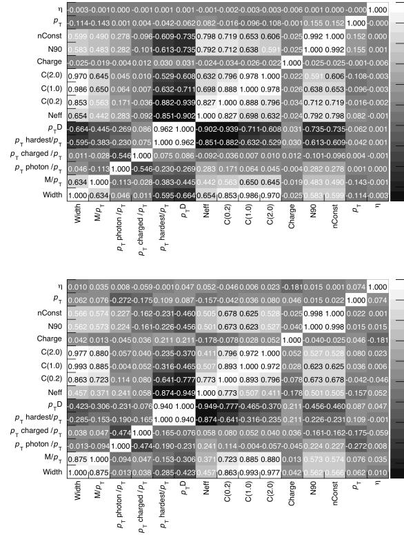
Figure 3: Input variable linear correlation coefficients in Pythia at 20 < p_T < 30 and 190 < p_T < 240 respectively.
