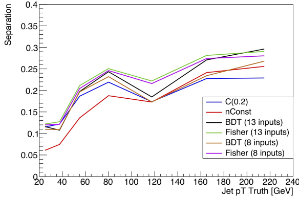
Figure 4: Separation of four MVA classifiers trained on Pythia.
