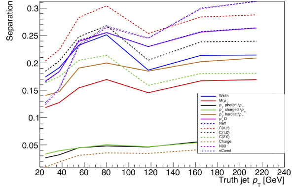
Figure 1: Quark/gluon separation of the 13 input variables.
