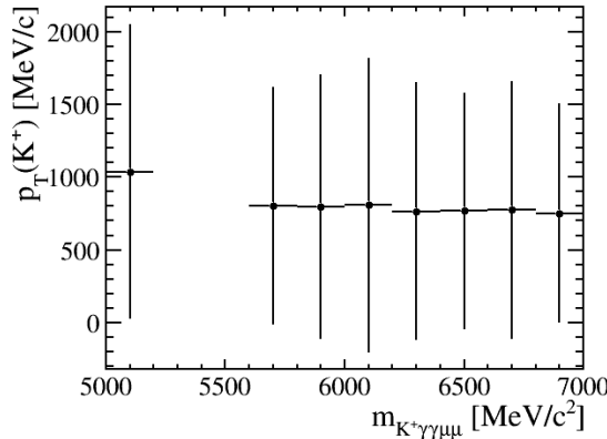
Figure 27: Profile of the mean (points) and RMS (error bars) of p_T(K^+) in bins of the B mass.
