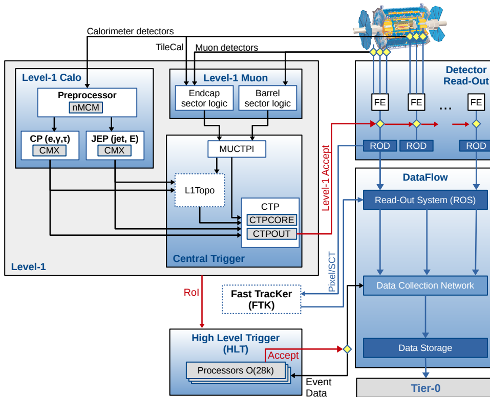
Figure 2.6: A flowchart showing the ATLAS TDAQ system [8]. Events that satisfy the hardware (L1) trigger requirements move onto the software-based High Level Trigger. Only events that pass both triggers are recorded and saved to disk.
