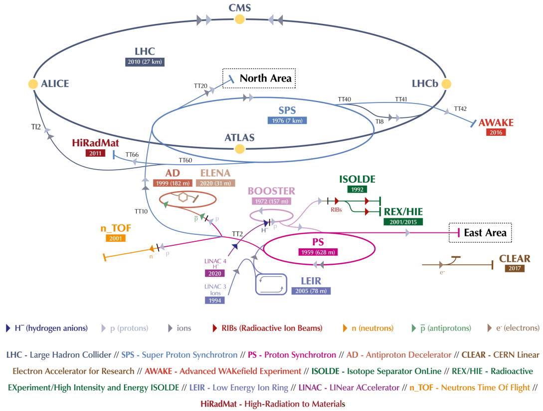
Figure 2.1: The LHC accelerator complex [6] including the Linac-4 replacement of Linac-2. Protons are accelerated through the complex starting in the Linac and moving through the chain before entering the LHC.
