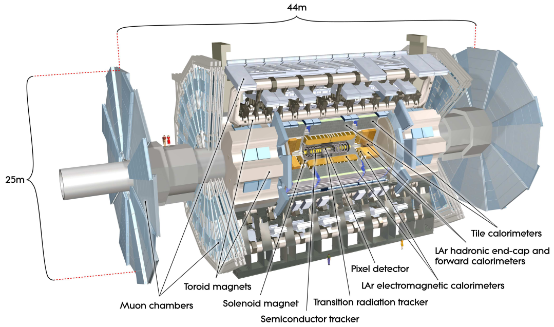
Figure 2.2: Schematic of the ATLAS detector [7]. The various subdetectors are arranged symmetrically around the collision point in the centre, beginning with the Inner Detector (pixel detector, silicon tracker and transition radiation tracker), the Calorimetry system (ECal, HCal and FCal) and the muon spectrometers. Toroid magnets are used to bend the trajectories of charged particles to allow their charges and momenta to be determined.
