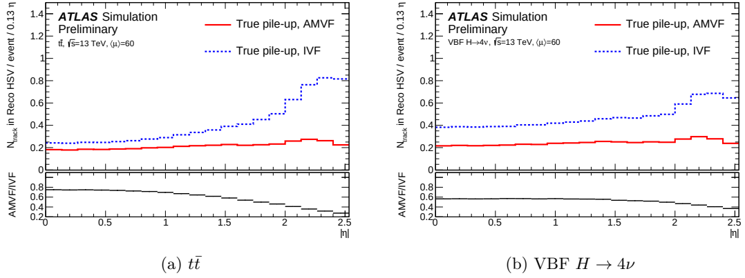
Figure 3.15: Comparison of IVF and AMVF HS track contamination as a function of |\eta| for (a) t\bar{t} and (b) VBF H \rightarrow 4\nu samples. Each plot shows the number of compatible reconstructed tracks per |\eta| bin originating from pile-up interactions that are incorrectly associated with the HS vertex. The AMVF sees reduced impurity across the entire |\eta| range, especially in the forward regions.
