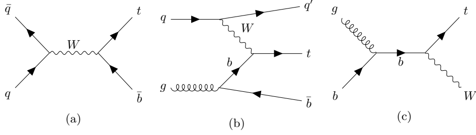
Figure 1.8: LO Feynman diagrams for single-top production, showing (a) s-channel, (b) t-channel and (c) Wt-channel.
