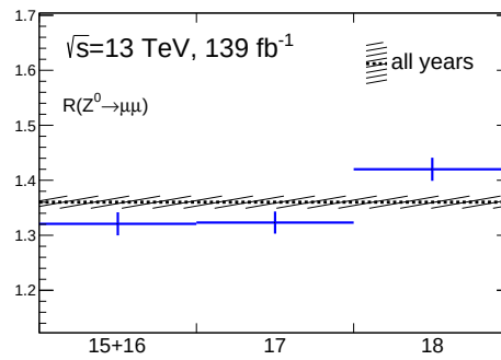
Figure 4.40: The Z^0(\rightarrow \mu\mu) + (b\text{-})\text{jets} background scale factors calculated in the different data-taking periods, compared against the inclusive value. Only statistical uncertainties are shown. Good agreement is seen for 2015+16 and 2017, though in 2018 the value is higher.
