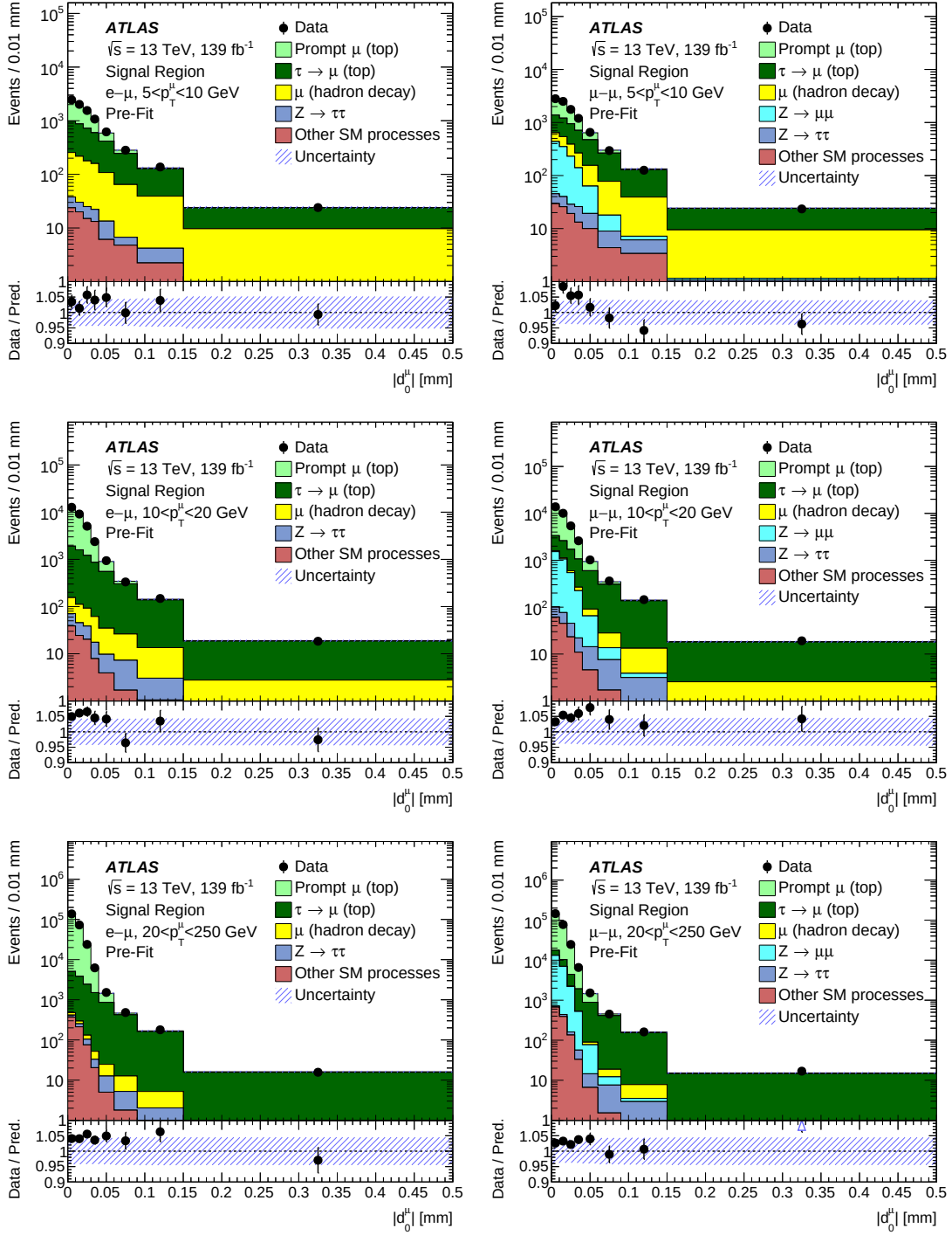
Figure 4.41: Pre-fit |d_0^\mu| distributions for data and MC. The background scale factors have already been applied. The bottom panel shows the ratio of the data to the expectation, with the blue bands representing the uncertainty. The t\bar{t} normalisation uncertainty is not included as this is a free-floating parameter in the fit. Data and prediction are seen to agree within the uncertainties.
