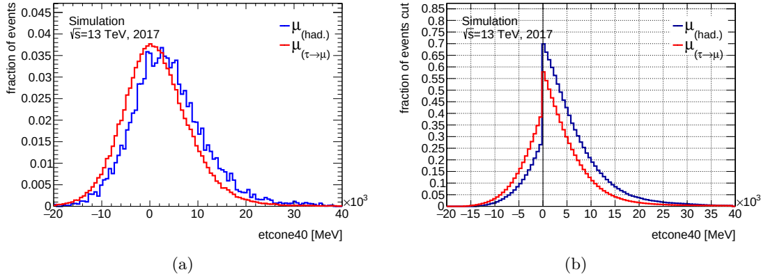
Figure 4.12: (a) the difference in shape between \mu_{\tau(\rightarrow\mu)} signal and \mu_{had} background and (b) the reduction in background and loss in signal for the variable etcone40 . The distributions are very similar in both cases such that this variable was not considered for further study.
