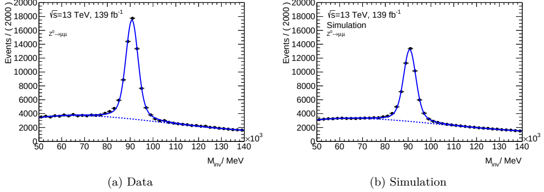
Figure 4.36: The invariant mass distribution in the Z^0 \rightarrow \mu\mu control region used to extract the Z^0(\rightarrow \mu\mu) + (b\text{-})\text{jets} scale factor, in (a) data and (b) simulation. The solid line represents the sum of the fitted Voigt profile and 3rd-order Chebychev polynomial, whilst the dashed line represents the 3rd-order Chebychev polynomial only.
