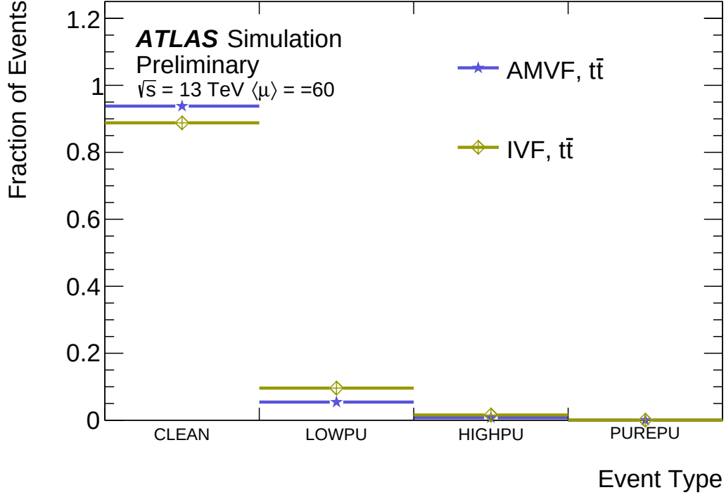
Figure 3.9: Fraction of events in each HS vertex reconstruction classification, for the IVF and AMVF. A higher fraction of CLEAN events are reconstructed with the AMVF, which indicates superior performance.
