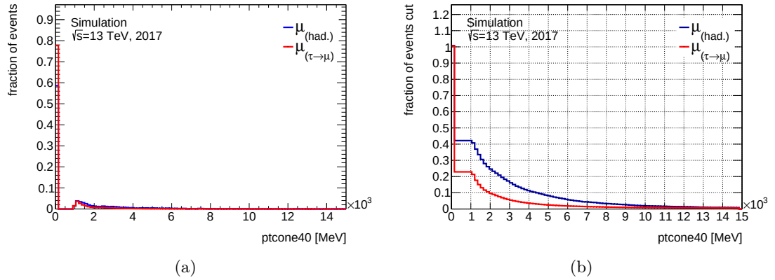
Figure 4.16: (a) the difference in shape between \mu_{\tau(\rightarrow\mu)} signal and \mu_{had} background and (b) the reduction in background and loss in signal for the variable ptcone40 . The tails of this distribution are quite different between \mu_{had} and \mu_{\tau(\rightarrow\mu)} , a feature which could be used to reduce background whilst maintaining signal.
