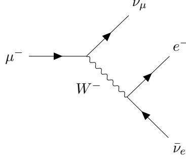
Figure 1.3: Lowest-order Feynman diagram of a muon decay. The muon decays to a muon neutrino and a virtual W^- , which subsequently decays to an electron and electron anti-neutrino.
