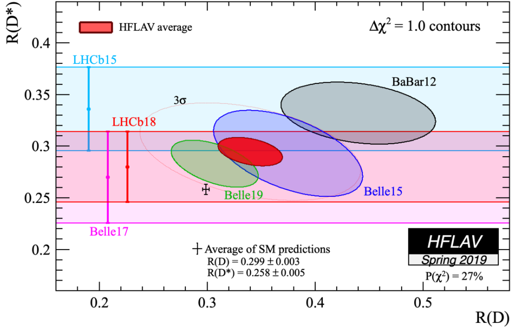
Figure 1.6: HFLAV R(D^{(*)}) averages [5]. The average of the Standard Model predictions are R_D = 0.299 \pm 0.003 , and R_{D^*} = 0.258 \pm 0.005 [5]. When taken together, including correlations, the R_{D^{(*)}} results agree with the Standard Model at the level of 3.08\sigma .
