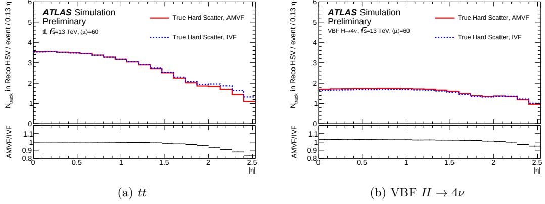
Figure 3.14: Comparison of IVF and AMVF HS track efficiency as a function of |\eta| for (a) t\bar{t} and (b) VBF H \rightarrow 4\nu samples. Each plot shows the number of correctly associated compatible reconstructed tracks per |\eta| bin originating from the generated HS vertex. The AMVF shows a higher efficiency by a few percent for VBF H \rightarrow 4\nu across almost the entire |\eta| range, and equal performance in t\bar{t} up to around |\eta| < 1.5 . The AMVF sees slightly lower efficiency in the forward region compared to the IVF.
