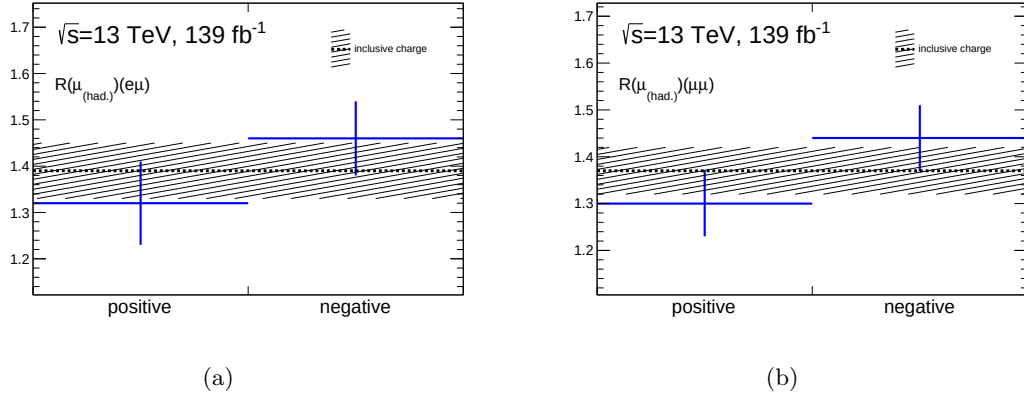
Figure 4.34: The muon from hadron decays background scale factors calculated exclusively in charge, compared against the inclusive value. Only statistical uncertainties are shown. The values obtained for both charges agree well within uncertainties.
