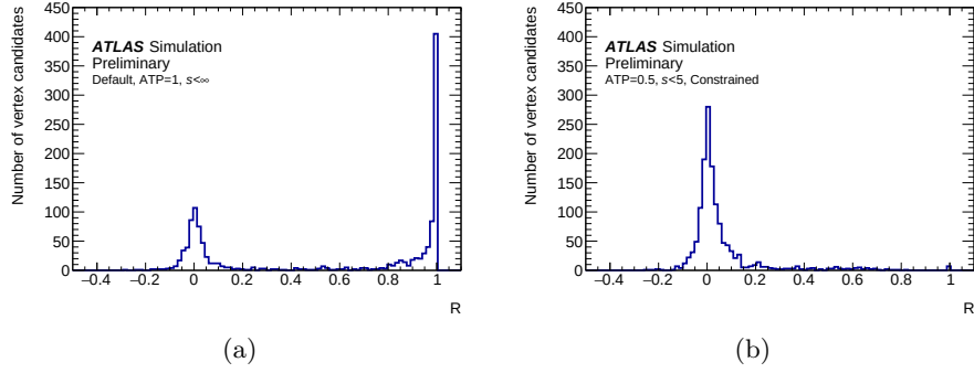
Figure 3.6: Vertex migration metric (a) before and (b) after introduction of a track assignment cut on impact parameter significance ( s ), stiffer annealing temperature power (ATP), and a longitudinal constraint. After fixing this issue, the vertex finder reconstructs 15% more vertices compared to the previous default, and does not suffer from multiple reconstructed vertices at the exact same location. Due to the “finding-through-fitting” approach, different numbers of vertex candidates will be found in the two scenarios.
