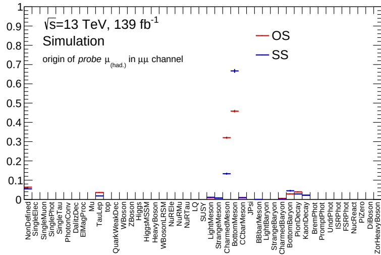
Figure 4.25: Sources of muons from hadron decays for same-sign (SS) and opposite-sign (OS) \mu\mu events. The dominant contributions are seen to come from the decays of charmed and bottom hadrons. There is a difference in the contributions in the same-sign and opposite-sign regions. The larger charmed meson contribution in the opposite-sign region arises from a W^\pm decaying to c\bar{s} , as muons produced in the c decay will have opposite charge to the tag lepton. Little difference is seen between the e\mu and \mu\mu channels, which can be seen by comparing with Figure 4.24.
