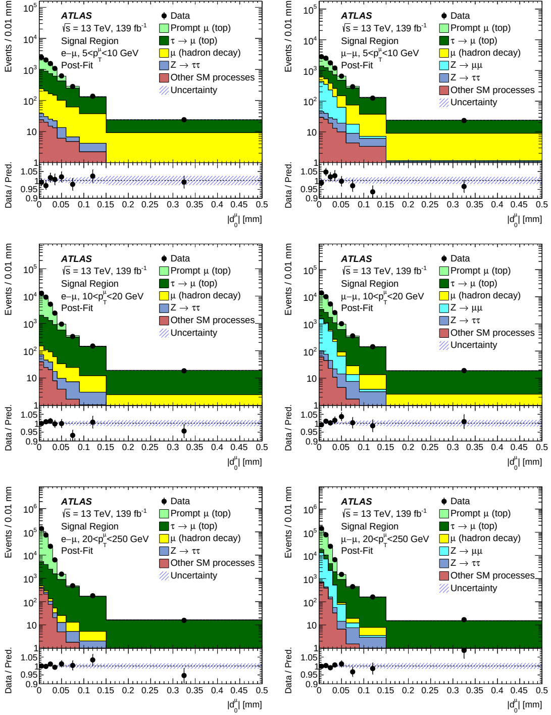
Figure 4.42: Post-fit |d_0^\mu| distributions for data and MC. The bottom panel shows the ratio of the data to the expectation, with the blue bands representing the uncertainty. After the fit, the agreement between prediction and data is seen to improve.
