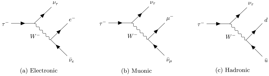
Figure 1.4: Lowest-order Feynman diagrams of a tau decay. The tau decays to a tau neutrino and virtual W^- , which subsequently decays to either light leptons or light quarks.
