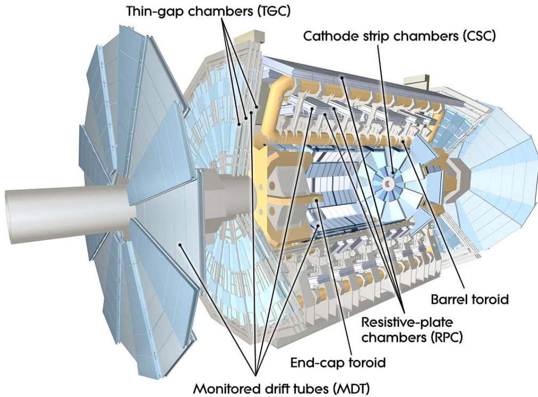
Figure 2.5: The ATLAS Muon System [7]. The components are arranged into large wheels covering the forward regions, as well as being arranged around the barrel. The muon detectors are placed around the outside of the detector as muons usually pass through the calorimeters.
