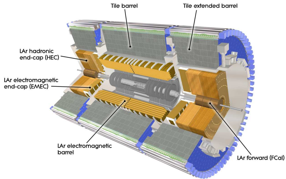
Figure 2.4: The ATLAS Calorimetry System [7]. The ECal is located around the Inner Detector. The HCal (tile) surrounds the ECal. The ECal and HCal endcaps and the FCal are located in the forward region.
