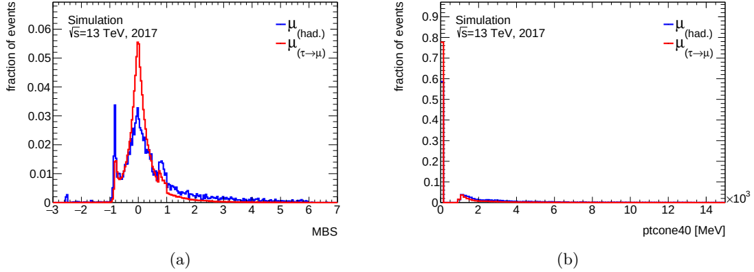
Figure 4.5: Distributions of (a) MBS and (b) ptcone40 for \mu_{\text{had}} and \mu_{\tau(\rightarrow\mu)} , normalised to unity. The differences in these distributions can be used to better discriminate signal from background.
