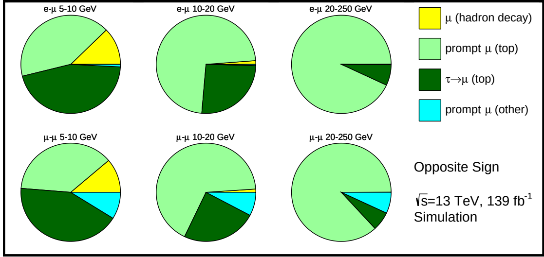
Figure 4.22: Proportions of probe muons in the opposite-sign signal region that are from hadron decays, from intermediate tau decays, prompt, or charge-flipped. The largest contributions from \mu_{\text{had}} are in the lowest p_T bins, where they are a significant background to the \mu_{\tau(\rightarrow\mu)} signal.
