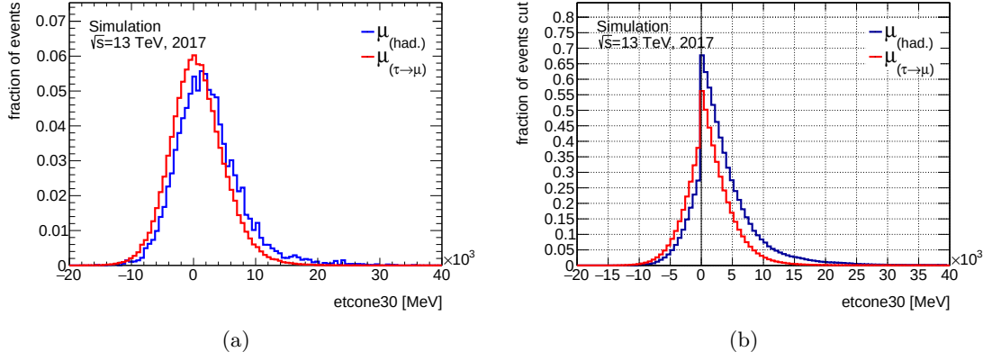
Figure 4.11: (a) the difference in shape between \mu_{\tau(\rightarrow\mu)} signal and \mu_{had} background and (b) the reduction in background and loss in signal for the variable etcone30 . The distributions are very similar in both cases such that this variable was not considered for further study.
