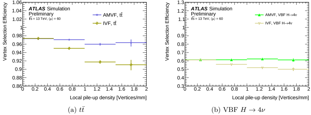
Figure 3.11: Comparison of IVF and AMVF HS vertex selection efficiency as a function of local pile-up density, for (a) t\bar{t} and (b). The two signal processes use different scales on the y -axis. The selection efficiency is the fraction of events where the reconstructed vertex with highest \Sigma p_T^2 contains the largest total track weight from the generated HS tracks. The AMVF significantly reduces the pile-up dependency.
