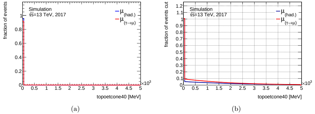
Figure 4.20: (a) the difference in shape between \mu_{\tau(\rightarrow\mu)} signal and \mu_{\text{had}} background and (b) the reduction in background and loss in signal for the variable topoetcone40 . The distributions are very similar in both cases such that this variable was not considered for further study.
