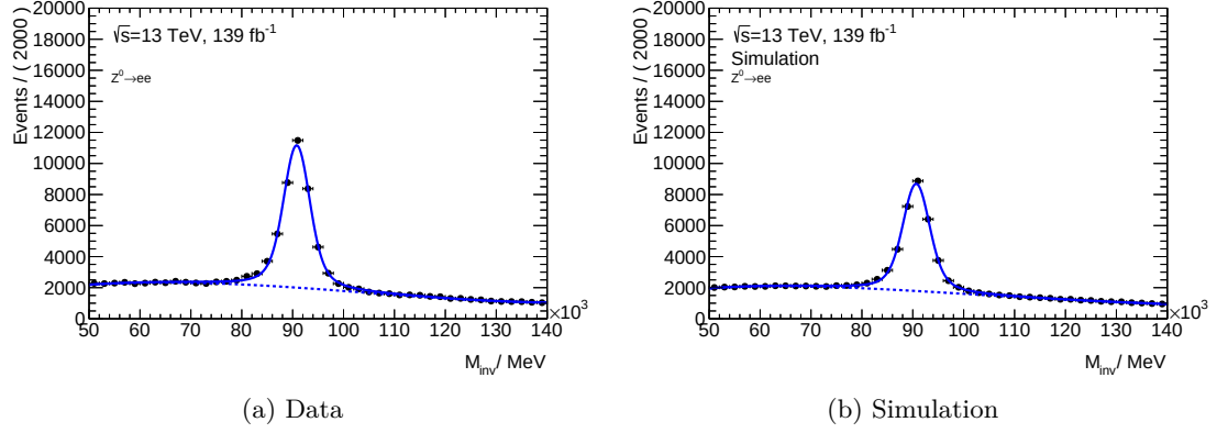
Figure 4.38: The invariant mass distribution in the Z^0(\rightarrow ee) + (b\text{-})\text{jets} control region used to extract the Z^0(\rightarrow ee) + (b\text{-})\text{jets} scale factor, in (a) data and (b) simulation. The solid line represents the sum of the fitted Voigt profile and 3rd-order Chebychev polynomial, whilst the dashed line represents the 3rd-order Chebychev polynomial only.
