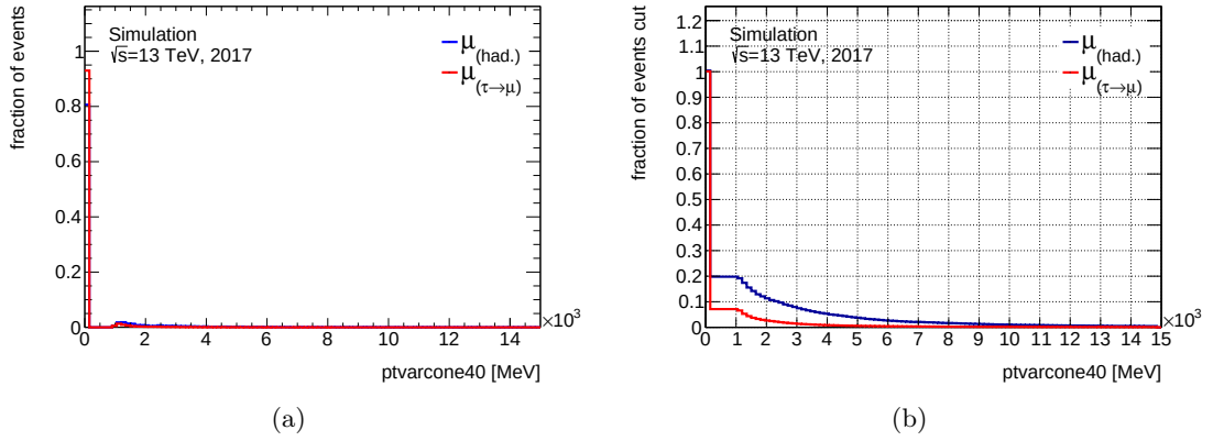
Figure 4.18: (a) the difference in shape between \mu_{\tau(\rightarrow\mu)} signal and \mu_{\text{had}} background and (b) the reduction in background and loss in signal for the variable ptvarcone40 . The tails of this distribution are quite different between \mu_{\text{had}} and \mu_{\tau(\rightarrow\mu)} , a feature which could be used to reduce background whilst maintaining signal.
