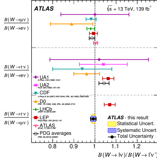
Figure 4.48: Measured value of R(\tau/\mu) , shown in comparison to previous tests of Lepton Flavour Universality using W^\pm boson decays. The precision of the measured values has improved over time.
