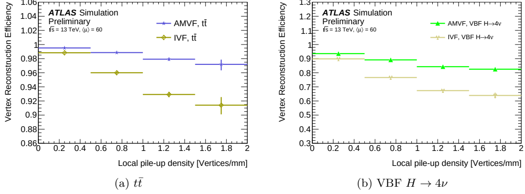
Figure 3.10: Comparison of IVF and AMVF HS vertex reconstruction efficiency as a function of local pile-up density, for (a) t\bar{t} and (b) VBF\ H \rightarrow 4\nu . The two signal processes use different scales on the y -axis. The reconstruction efficiency is the fraction of events where the generated HS interaction is successfully reconstructed (classified as CLEAN/MATCHED, LOWPU or HIGHPU). The AMVF sees a higher reconstruction efficiency and reduced pile-up dependence in both cases. The efficiency gains are particularly prominent at high pile-up densities in for VBF\ H \rightarrow 4\nu , with around 50% of lost efficiency recovered.
