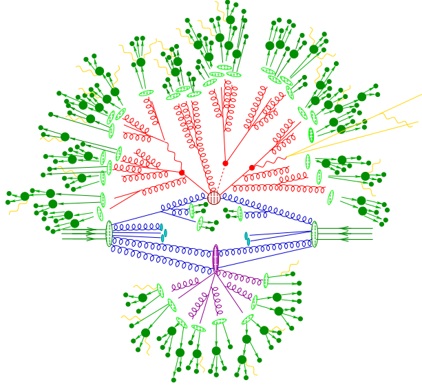
Figure 2.7: A diagram of a Higgs boson produced in association with t\bar{t} , as produced by an event generator. As shown in Ref. [9]. The hard scatter interaction is indicated by the large red circle, and the decays of the t\bar{t} and Higgs boson are indicated by the small red circles. Additional hard QCD radiation is produced (indicated by red lines) and a secondary interaction takes place (purple), before the final-state partons hadronise (indicated by light green) and hadrons decay (indicated by dark green). QED radiation can occur at any stage (yellow).
