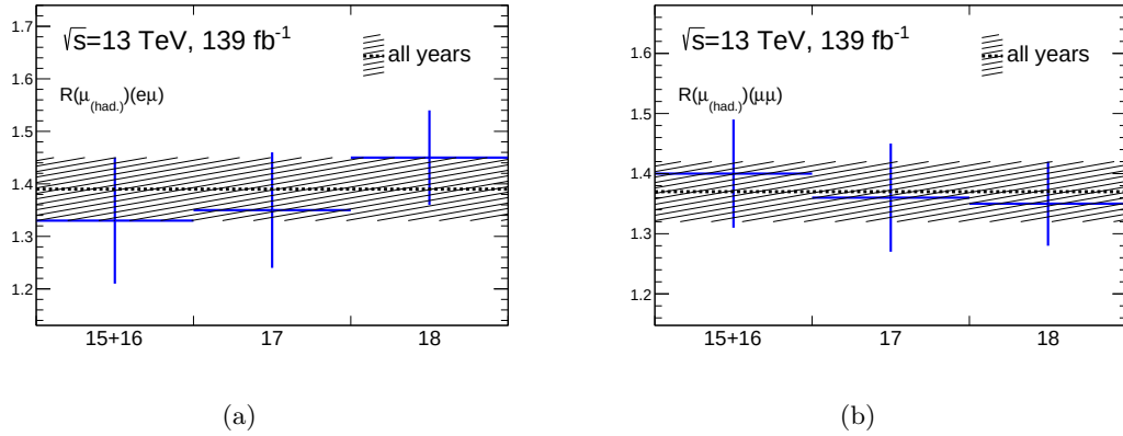
Figure 4.33: The muon from hadron decays background scale factors calculated in the different data-taking periods, compared against the inclusive value. Only statistical uncertainties are shown. The values obtained in each of the periods all agree well within uncertainties.
