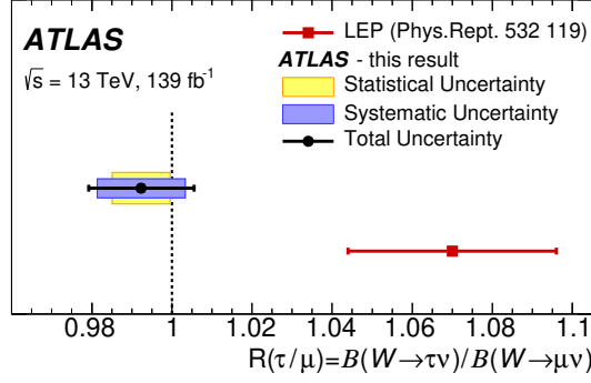
Figure 4.44: Measured value of R(\tau/\mu) , shown in comparison to the previous LEP result. The result obtained in this analysis shows good agreement with the Standard Model assumption of unity.
