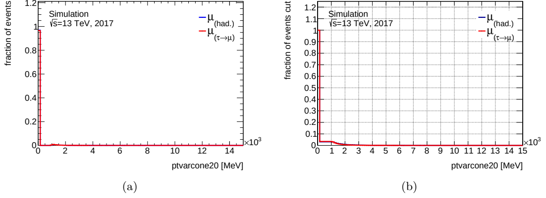
Figure 4.17: (a) the difference in shape between \mu_{\tau(\rightarrow\mu)} signal and \mu_{\text{had}} background and (b) the reduction in background and loss in signal for the variable ptvarcone20 . The distributions are very similar in both cases such that this variable was not considered for further study.
