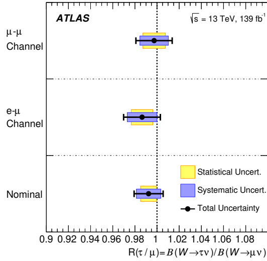
Figure 4.47: The nominal result (bottom) compared with the independent fits using only the \mu - \mu channel (top) and e - \mu channel (middle). A single fit is performed using the same correlation model as the nominal fit, but using two parameters of interest for R(\tau/\mu) , one for each of the e - \mu and \mu - \mu channels. Good agreement is seen between both channels.
