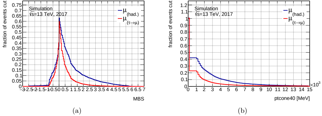
Figure 4.6: Distributions of the estimated signal loss and background reductions in (a) MBS and (b) ptcone40 for \mu_{\text{had}} and \mu_{\tau(\rightarrow\mu)} . This suggests additional cuts will have very different effects on the background and signal yields. For example, \text{MBS} < 2 could reduce the background by \sim 10\% whilst only having a \sim 2\% impact on signal.
