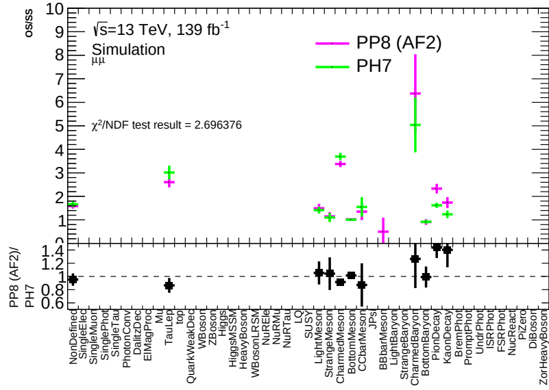
Figure 4.27: OS/SS for each muons from hadron decays background lepton source for \mu\text{-}\mu channel for POWHEG+PYTHIA8 and POWHEG+HERWIG. Very good agreement is seen for the dominant bottom and charmed meson components.
