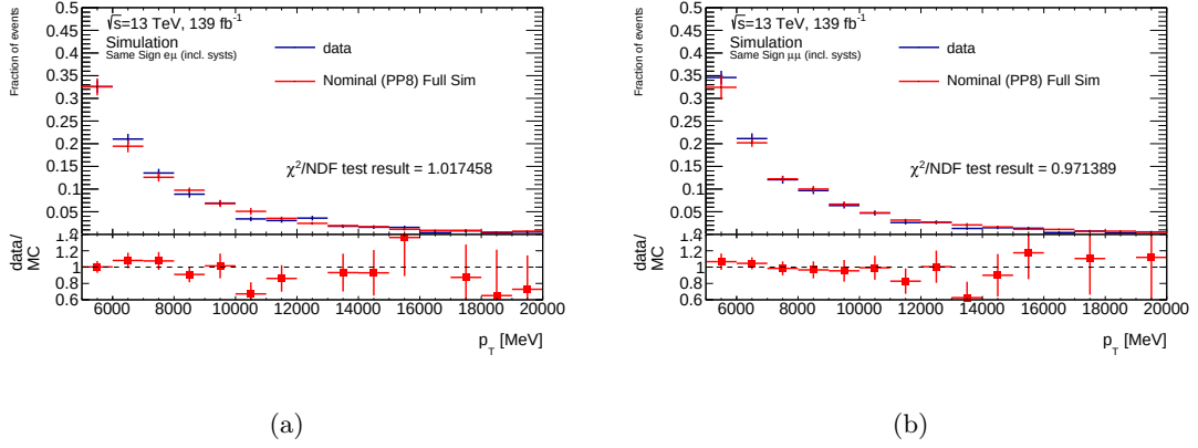
Figure 4.30: Comparison of distributions of p_T^\mu in same-sign (a) e\text{-}\mu and (b) \mu\text{-}\mu events in data and simulation for the full dataset. The systematic uncertainty in each bin of this histogram is calculated as half the difference between the highest and lowest MC generator. The \chi^2 test is performed after adding this systematic uncertainty in quadrature with the statistical uncertainty. The results of the \chi^2 test are shown in the legend. This systematic is applied only to these same-sign distributions for this comparison.
