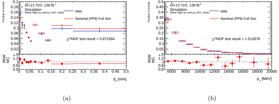
Figure 4.28: Comparison of distributions of (a) |d_0^\mu| and (b) p_T^\mu in same-sign e\text{-}\mu and \mu\text{-}\mu events in data and simulation for the full dataset. The |d_0^\mu| distributions are not normalised to the bin widths. The systematic uncertainty in each bin of this histogram is calculated as half the difference between the highest and lowest MC generator. The \chi^2 test is performed after adding this systematic uncertainty in quadrature with the statistical uncertainty. The results of the \chi^2 test are shown in the legend. This systematic is applied only to these same-sign distributions for this comparison.
