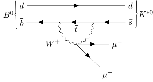
Figure 1.5: Feynman diagram of a Standard Model B^0 , consisting of d and \bar{b} quarks, decaying to K^{*0} , which consists of d and \bar{s} quarks, as well as a dimuon pair.
