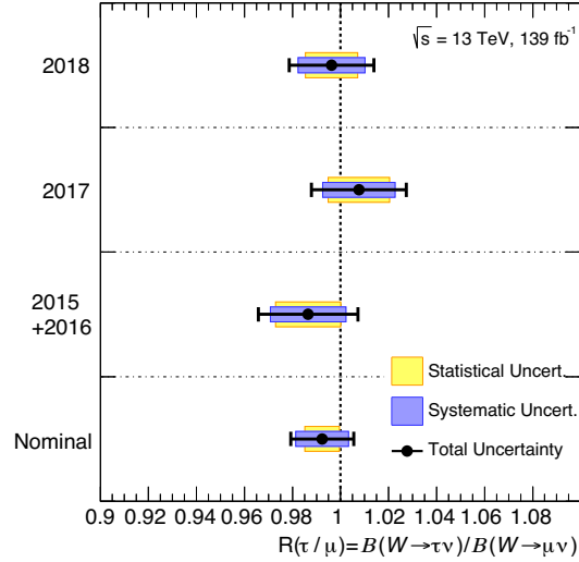
Figure 4.45: The nominal result (bottom) compared with the independent fits using only data from 2015+2016, 2017 and 2018 respectively. Good agreement is seen for the values obtained in each of the data-taking periods.
