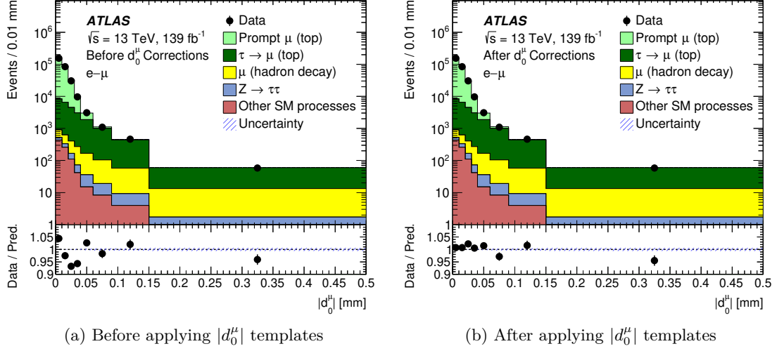
Figure 4.2: Data/MC agreement in the signal region, inclusive in p_T^\mu , (a) before and (b) after applying the estimated |d_0^\mu| templates for prompt muons, in the e\text{-}\mu channel. By applying the the templates, the agreement between observation and prediction is seen to improve. The bias corrections described in Section 4.4.3 are applied in both (a) and (b) as a first step, such that the effect of this particular correction is not compared in this figure.
