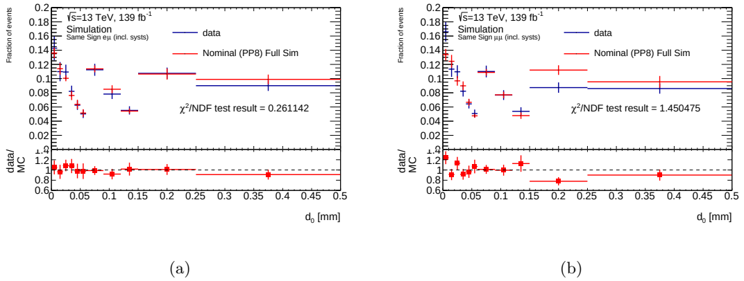
Figure 4.29: Comparison of distributions of |d_0^\mu| in same-sign (a) e\text{-}\mu and (b) \mu\text{-}\mu events in data and simulation for the full dataset. The distributions are not normalised to the bin widths. The systematic uncertainty in each bin of this histogram is calculated as half the difference between the highest and lowest MC generator. The \chi^2 test is performed after adding this systematic uncertainty in quadrature with the statistical uncertainty. The results of the \chi^2 test are shown in the legend. This systematic is applied only to these same-sign distributions for this comparison.
