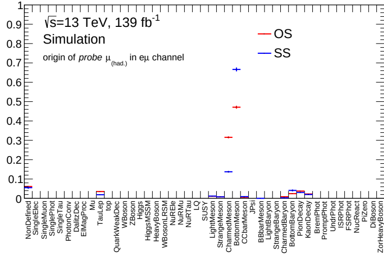
Figure 4.24: Sources of muons from hadron decays for same-sign (SS) and opposite-sign (OS) e\mu events. The dominant contributions are seen to come from the decays of charmed and bottom hadrons. There is a difference in the contributions in the same-sign and opposite-sign regions. The larger charmed meson contribution in the opposite-sign region arises from a W^\pm decaying to c\bar{s} , as muons produced in the c decay will have opposite charge to the tag lepton. Little difference is seen between the e\mu and \mu\mu channels, which can be seen by comparing with Figure 4.25.
