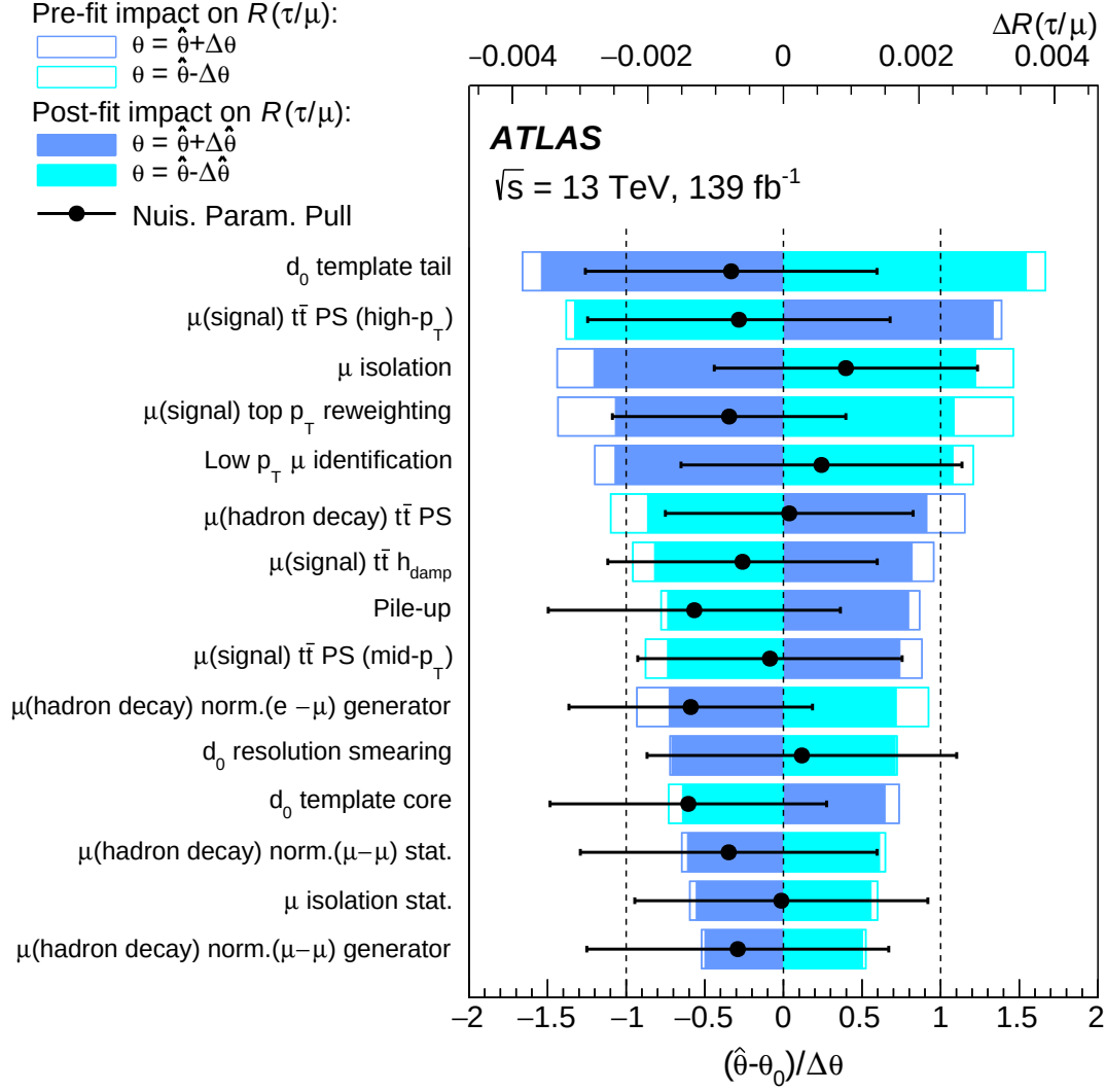
Figure 4.43: The ranked impacts of the different systematic uncertainties on the parameter of interest, R(\tau/\mu) .
