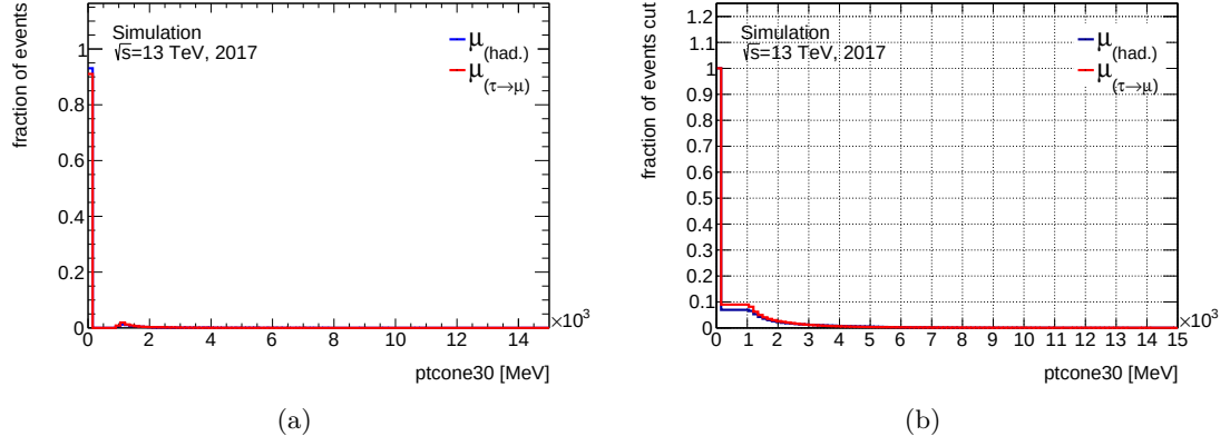
Figure 4.15: (a) the difference in shape between \mu_{\tau(\rightarrow\mu)} signal and \mu_{had} background and (b) the reduction in background and loss in signal for the variable ptcone30 . The distributions are very similar in both cases such that this variable was not considered for further study.
