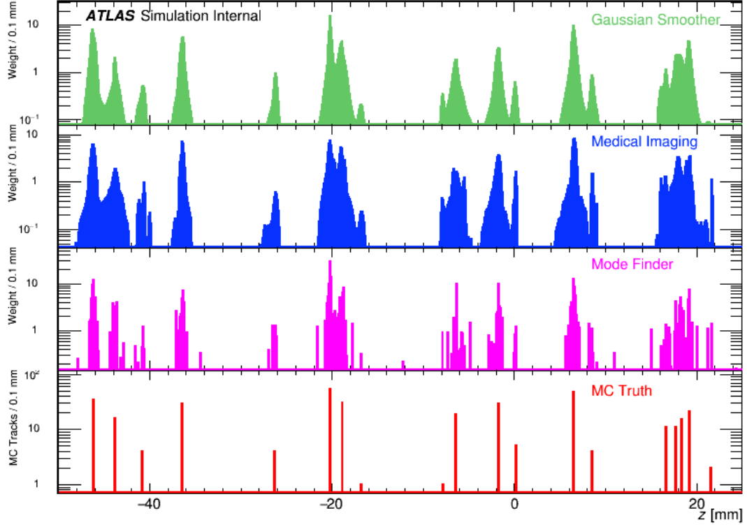
Figure 3.3: A single MC event analysed by three different primary vertex seed finders. The bottom plot indicates the locations of the pp interactions along the beamline as generated in MC, along with the number of tracks passing quality cuts. The top three plots show the track density estimators computed using the different seed finders. The approximate locations of the primary vertices, including pile-up interactions, are indicated by local maxima. The FSMW mode finder (labelled “Mode Finder”) was used by ATLAS during Run-1 and Run-2. The medical imaging and Gaussian methods were both studied to improve high luminosities, with the Gaussian seed finder (labelled “Gaussian smoother”) to be used from Run-3 onwards. As shown in Ref. [1].
