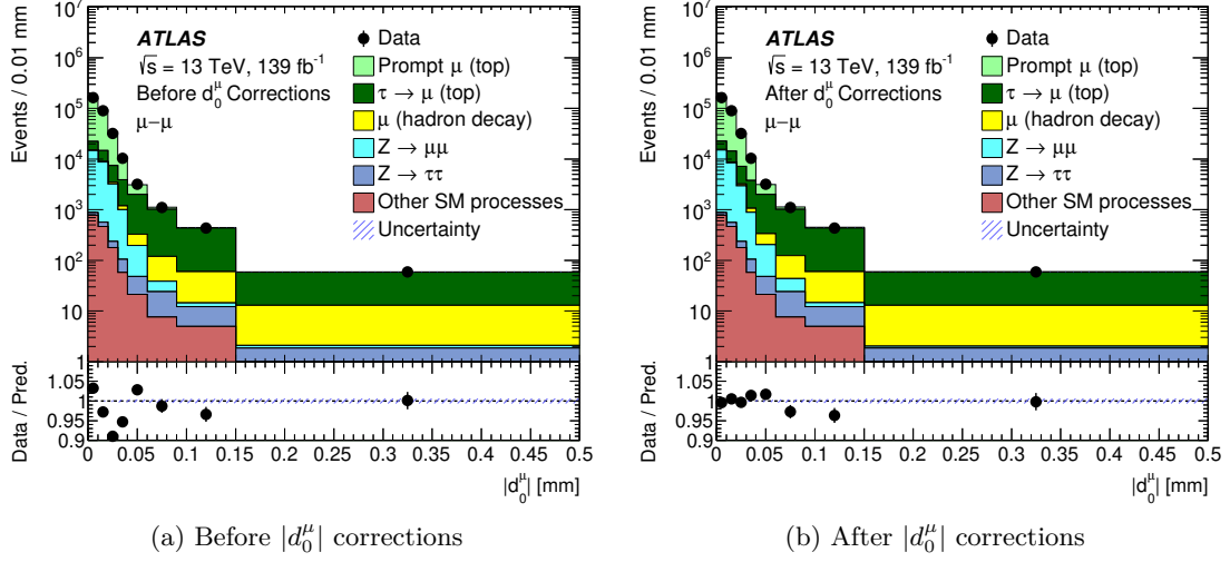
Figure 4.3: Data/MC agreement in the signal region, inclusive in p_T^\mu , (a) before and (b) after applying |d_0^\mu| corrections to prompt muons, in the \mu - \mu channel. By applying the templates, the agreement between observation and prediction is seen to improve. The bias corrections described in Section 4.4.3 are applied in both (a) and (b) as a first step, such that the effect of this particular correction is not compared in this figure.
