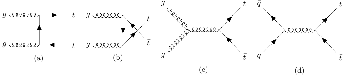
Figure 1.7: LO Feynman diagrams for top quark pair-production through (a), (b), (c) gluon-gluon fusion and (d) quark-antiquark annihilation.
