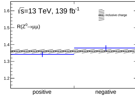
Figure 4.39: The Z^0(\rightarrow \mu\mu) + (b\text{-})\text{jets} background scale factors calculated exclusively in charge. Only statistical uncertainties are shown. The values obtained for both charges agree well within uncertainties.
