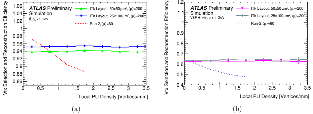
Figure 3.4: The primary vertex candidate reconstruction and selection efficiency for (a) t\bar{t} and (b) VBF H \rightarrow 4\nu as a function of local pile-up density in events with \langle \mu \rangle = 200 . Results use analogue clustering and pixel sizes of 50 \times 50 \mu\text{m}^2 or 25 \times 100 \mu\text{m}^2 for the ITk layout. The primary vertex is selected as the vertex with the highest \Sigma p_T^2 of associated tracks [10].
