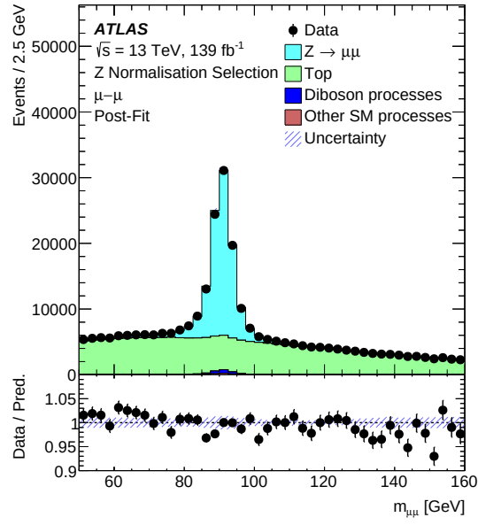
Figure 4.37: The invariant mass distribution in the Z^0 \rightarrow \mu\mu control region used to extract the Z^0(\rightarrow \mu\mu) + (b\text{-})\text{jets} normalisation, with the calculated scale factor applied. The bottom panel shows the data/MC comparison. The blue bands indicate the systematic uncertainties with the constraints from the analysis fit of the signal region data applied. Good agreement is seen between data and prediction which gives confidence in the method used to calculate the scale factor.
