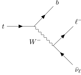
Figure 1.2: Lowest-order Feynman diagram of top quark decaying to a bottom quark and a W^- boson, with the W^- boson decaying to leptons. Here \ell = e, \mu, \tau .
