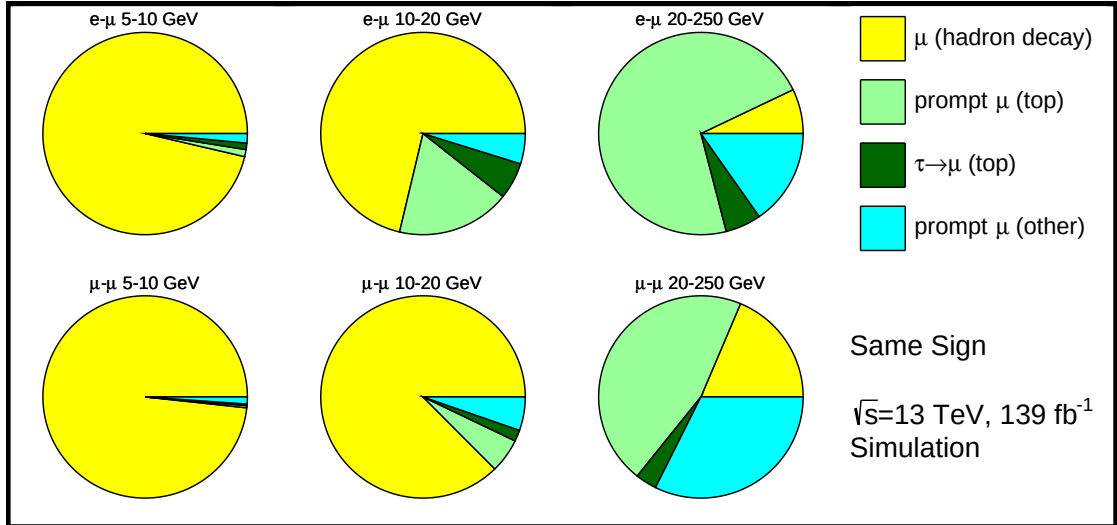
Figure 4.23: Proportions of probe muons in the same-sign control region that are from hadron decays, from intermediate tau decays, prompt, or charge-flipped. The \mu_{\text{had}} contributions dominate the same-sign region in all but the highest p_T bin. At higher p_T there are prompt contributions arising from t\bar{t} + V . The e\text{-}\mu channel also sees contributions from events with tag electrons that have misidentified charge.
