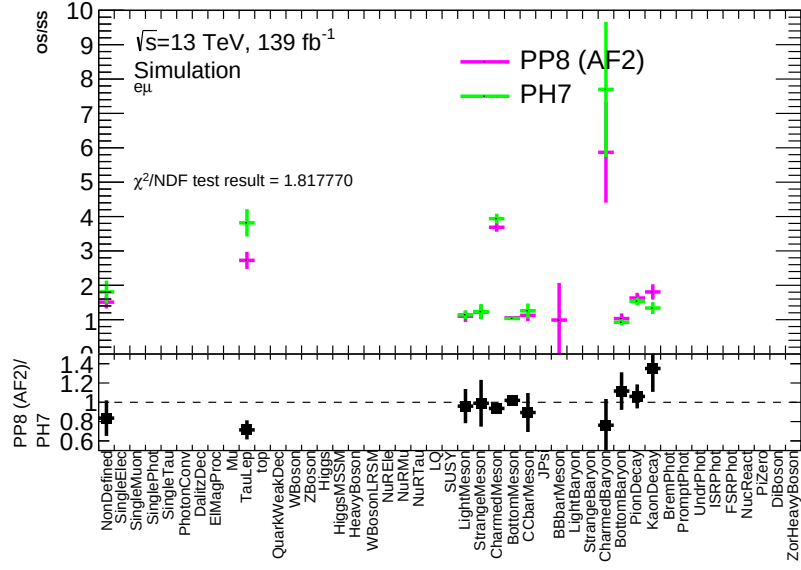
Figure 4.26: OS/SS for each muons from hadron decays background lepton source for e\text{-}\mu channel for POWHEG+PYTHIA8 and POWHEG+HERWIG. Very good agreement is seen for the dominant bottom and charmed meson components.
