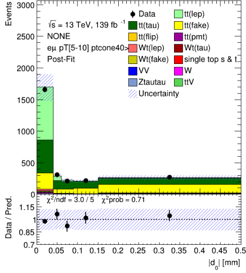
(a) e - \mu channel, pt_{cone40} > 1 \text{ GeV}
