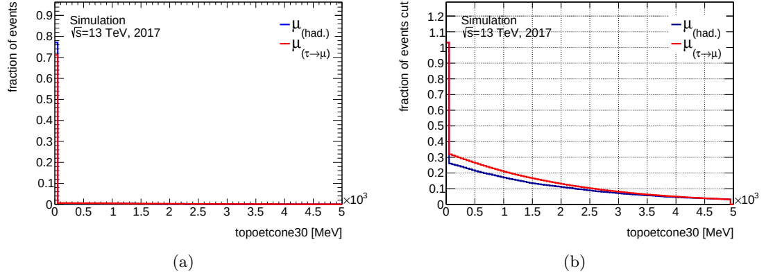
Figure 4.19: (a) the difference in shape between \mu_{\tau(\rightarrow\mu)} signal and \mu_{\text{had}} background and (b) the reduction in background and loss in signal for the variable topoetcone30 . The distributions are very similar in both cases such that this variable was not considered for further study.
