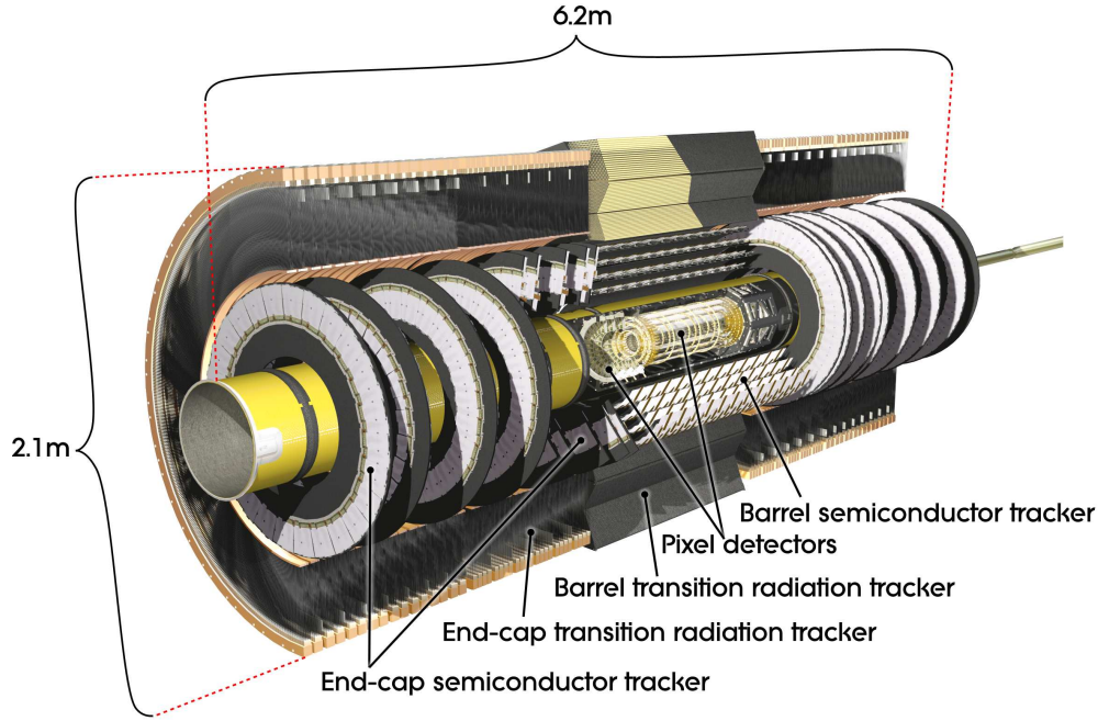
Figure 2.3: The ATLAS Inner Detector [7]. The pixel detector is found the in region closest to the beamline, and is surrounded by the silicon tracker and the transition radiation tracker.
