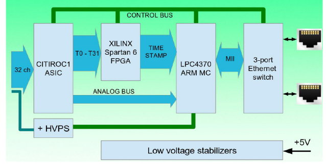
Figure 6.1: DT5702 as integrated as the initial prototype's readout electronics (left) and DT5702 block diagram (right) [386].
