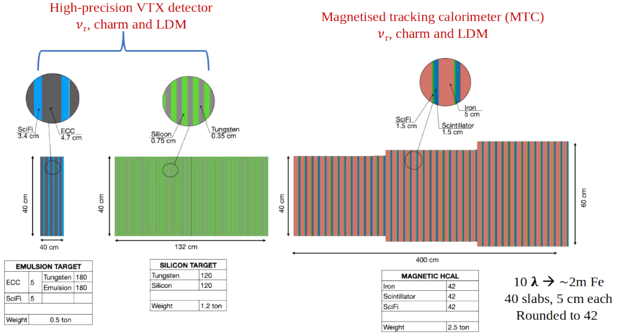
Figure 2.23: SND@SHiP Magnetised tracking calorimeter.
