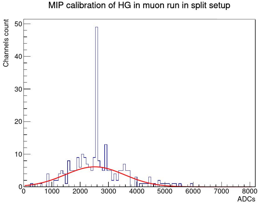
Figure 7.15: Calibration values of all channels, the red line represents the gaussian fit whose mean was used to assign MPV calibration peaks to channels for which the calibration fit couldn't converge for lack of statistics.
