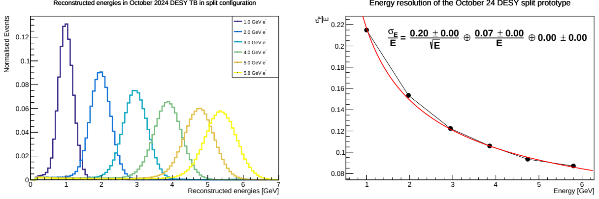
Figure 7.32: TB3 energy reconstruction (left) and resolution (right) in the split configuration using the simple scaling technique.
