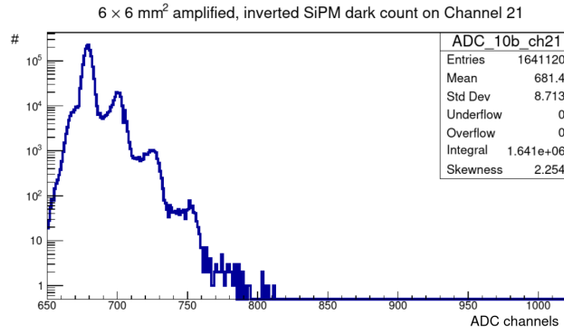
Figure 6.31: Amplified dark count pulse onto the KLauS HG17 using a custom charge-sensing amplifier.
