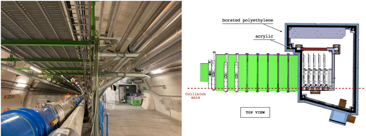
Figure 2.12: Picture of SND@LHC after February 2022, the ATLAS interaction point lies outside the picture, 480 m towards the viewer [291] (left) and schematic drawing of the neutron shield [100]. The interaction point is there to the left. (right).
