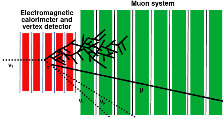
Figure 2.15: Visualisation of a \nu_\tau reconstruction, dotted lines are unseen particles. The shower structure has been simplified and scales have been adjusted for maximum clarity.
