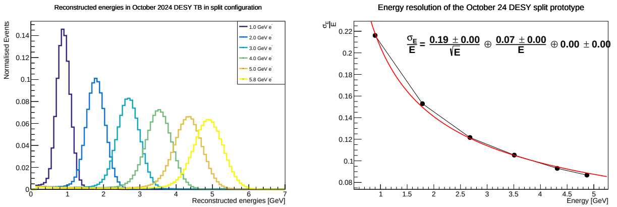
Figure 7.33: TB3 energy reconstruction (left) and resolution (right) in the split configuration using the interpolation technique.
