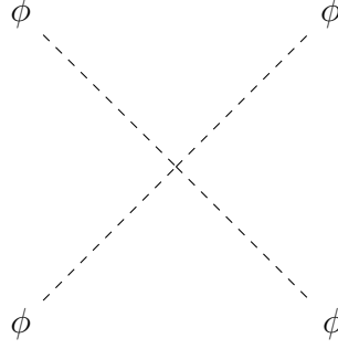
Figure 1.5: Scalar field 4-point coupling.
