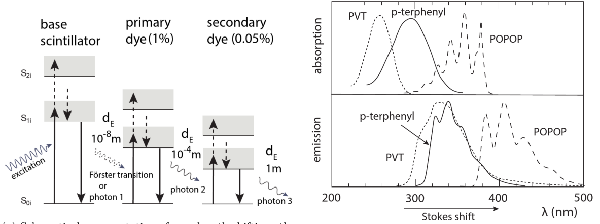
(a) Schematic representation of wavelength shifting: the base scintillator (here PVT) is excited and its deexcitation photon or Förster transition excites the primary agent (here p-terphenyl) the deexcitation photon of which excites the secondary agent (here POPOP). Spatial distances d_E are also shown [330].
