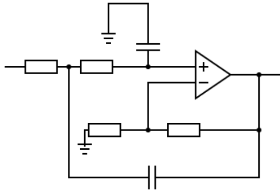
Figure D.10: Sallen-Key shaper topology.
