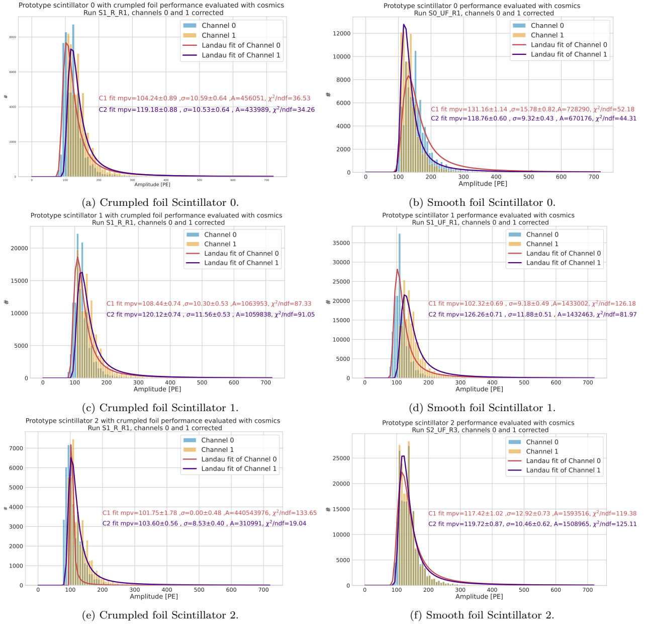
Figure C.1: Crumpled and smooth foil light output in all configurations.
