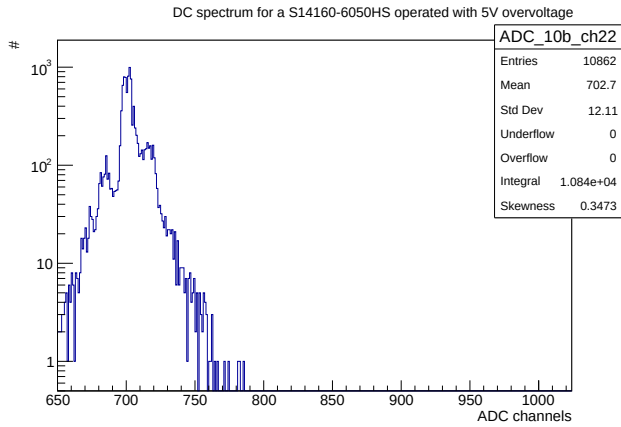
Figure 6.28: Dark count spectrum of a S14160-6050HS SiPM in HG11.
