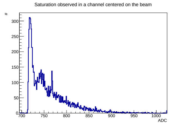
Figure 7.12: Saturation for LG=60 (left). Saturation is significant. Saturation for LG=200 (right). No saturation is observed. The same channel and same energy (5 GeV) is considered in both cases.
