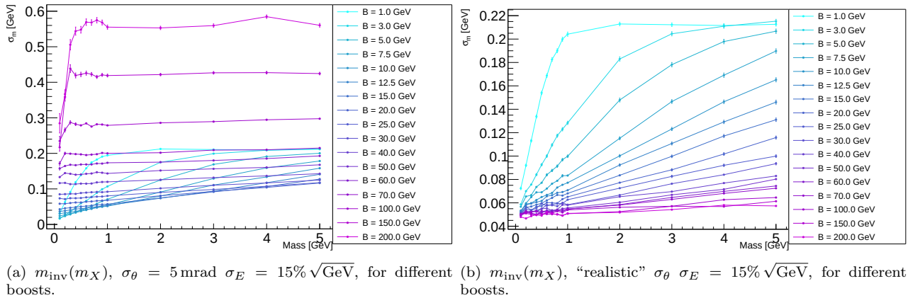
Figure 4.8: Absolute invariant mass resolution as a function of X mass, given standard calorimeter energy resolution, good and realistic calorimeter angular resolutions, for different X boosts.
