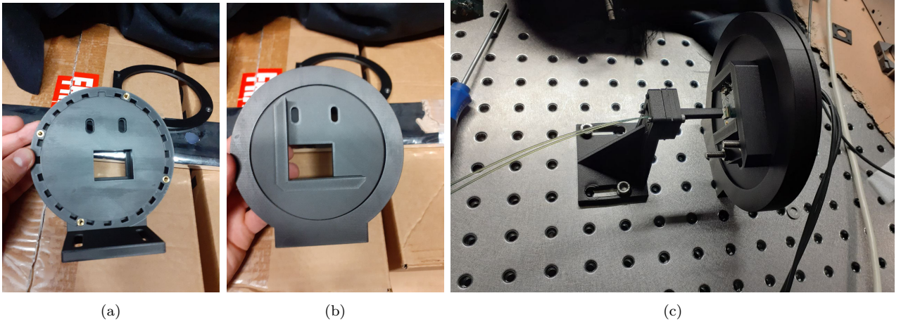
Figure 5.42: SiPM rotation device. Angles may be varied in steps of 15^\circ with the SiPM remaining aligned on the fibres.
