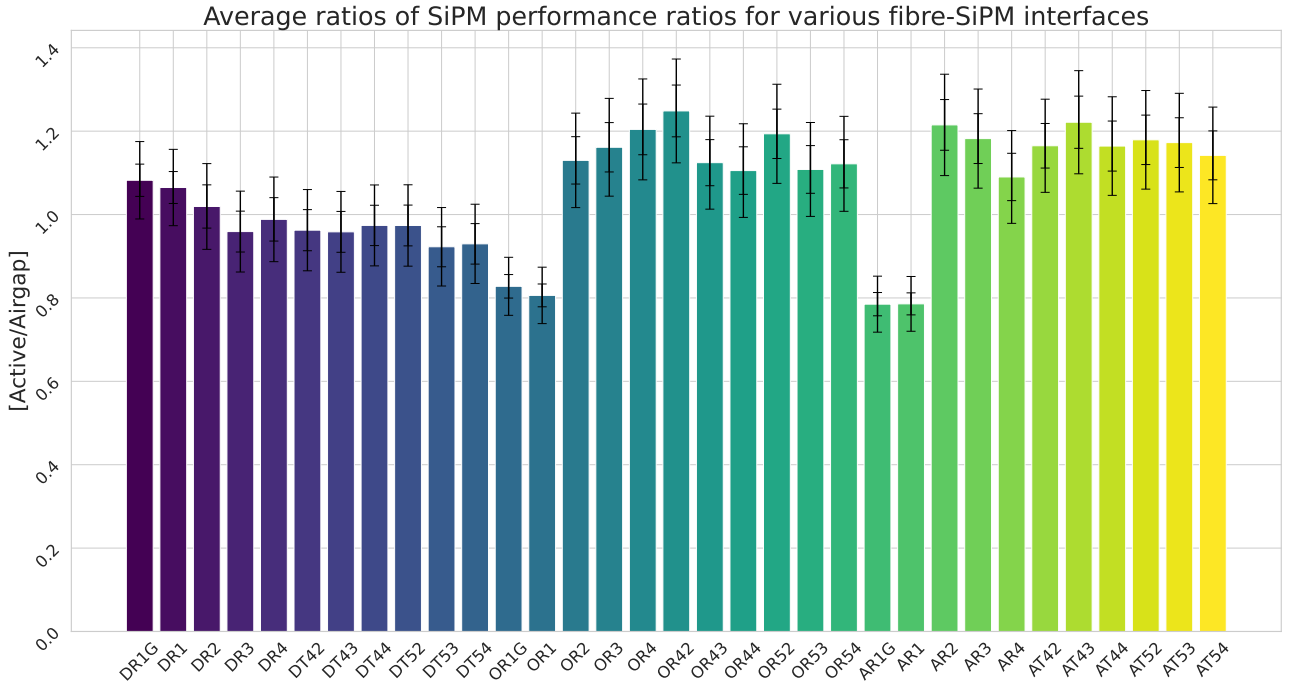
Figure 5.36: Evaluation of the ratio of the ratios between both sides of the SiPM for different interfaces \frac{A_{\text{test\_test}}/A_{\text{ref\_test}}}{A_{\text{test,Airgap\_ref}}/A_{\text{ref,Airgap\_ref}}} . The inner error bars are statistical whereas the outer ones are systematic.
