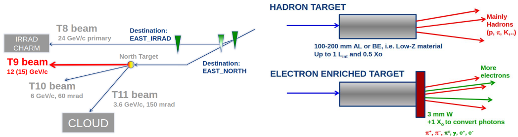
Figure 7.3: PS beam line topology [398] (left) and secondary beam creation process [398] (right).
