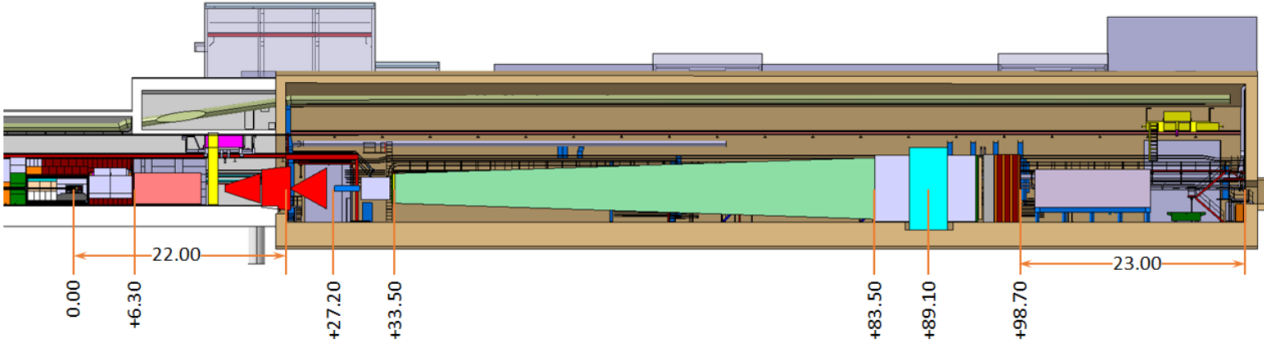
Figure 2.17: BDF/SHiP component sizes [26].
