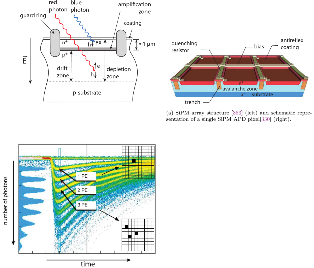
Figure 3.13: SiPM output pulses for different PE counts. One PE corresponds to one pixel firing, two PE correspond to two pixels firing and three PE correspond to three pixels firing [330].
