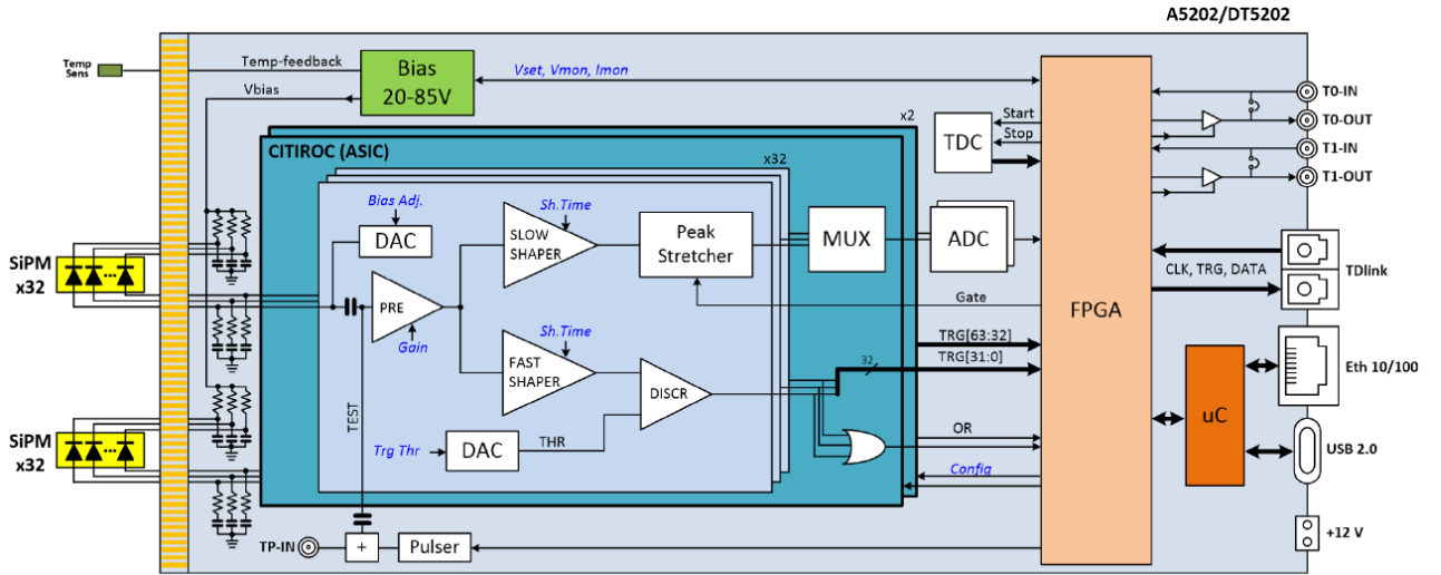
Figure 6.4: Block diagram of the CAEN DT5202 [386].
