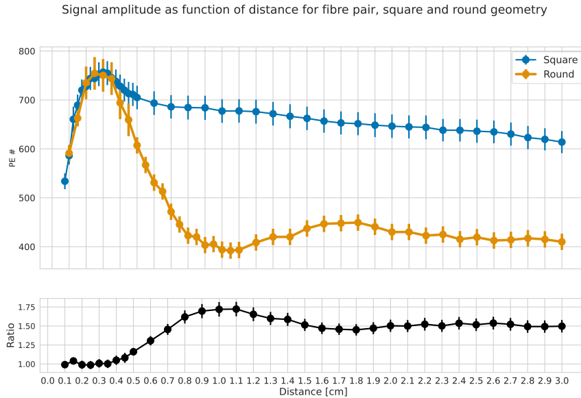
Figure 5.33: SiPM average PE counts as a function of distance for square and round geometries of T2.
