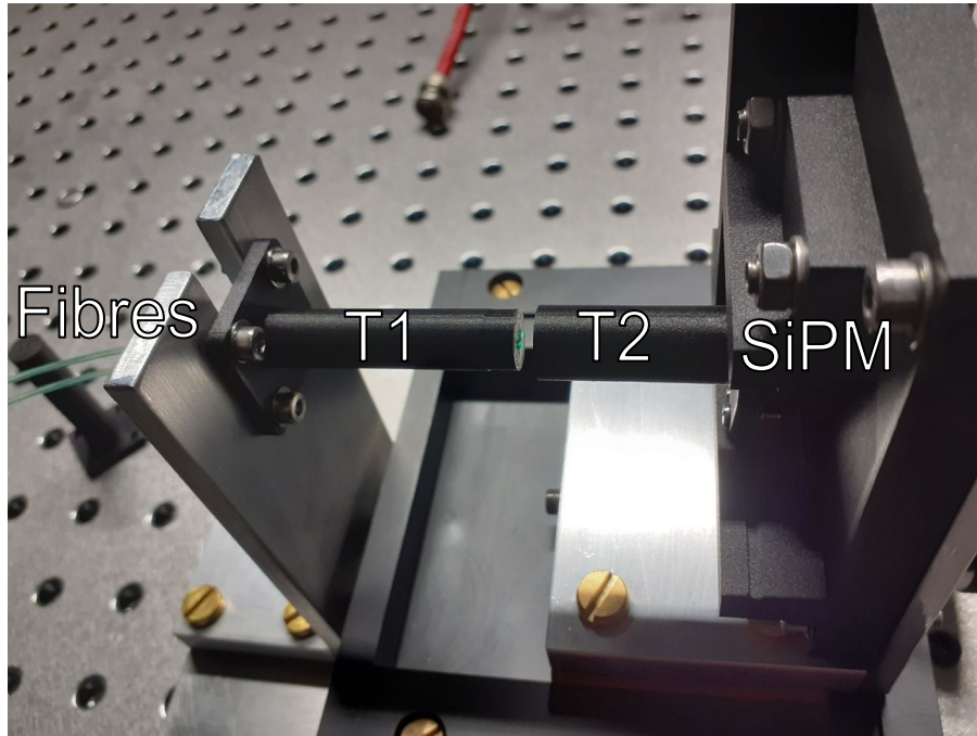
Figure 5.28: Fibre screw device. The fibres enter T1 which is inserted into T2 fixed to the SiPM.
