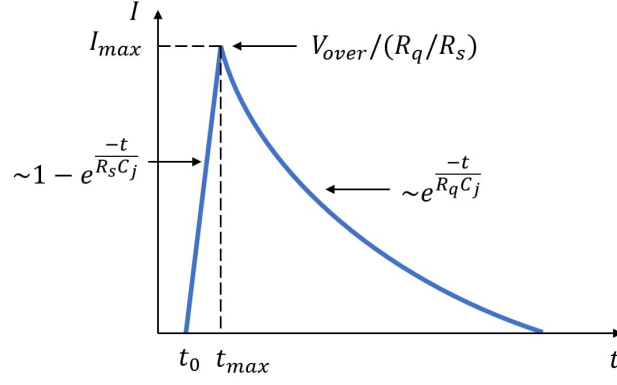
Figure 3.16: Example of a SiPM output pulse as a function of its parameters. V_{\text{over}} is the SiPM overvoltage.
