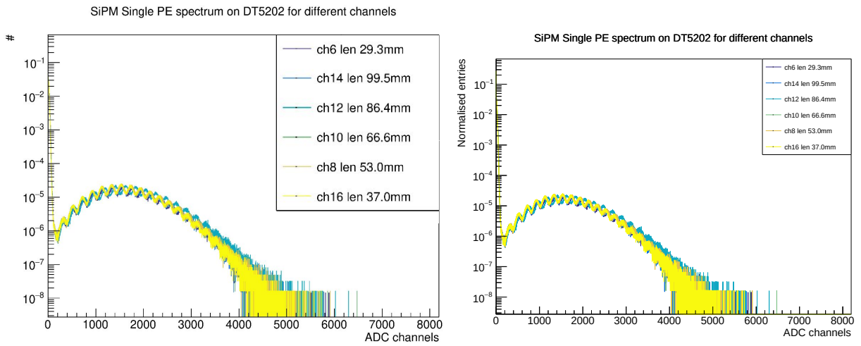
Figure 6.8: Single PE spectrum as seen from low intensity laser irradiation for different channels. Noise can be induced (left) and the PE spectra are progressively dephased as higher amplitudes are reached (right). Different gains are used in both cases.
