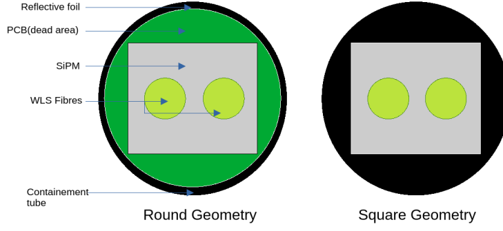
Figure 5.29: Fibre and SiPM system as seen from above.
