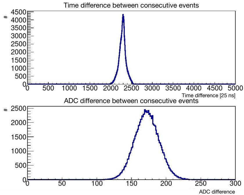
Figure 6.29: Time and HG17 ADC difference of event pairs (even and odd) in a 1 kHz laser irradiated data sample. Time units are provided in increments of 25 ns with positive difference indicating that the pulse from the second peak was integrated afterwards. ADC difference is between the first and second event.
