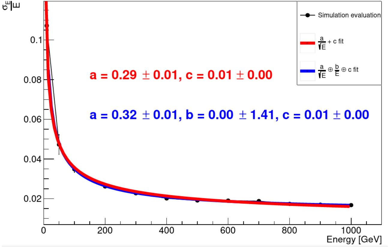
Figure 8.29: Energy resolution in emulsions using a 300 μm evaluation radius.
