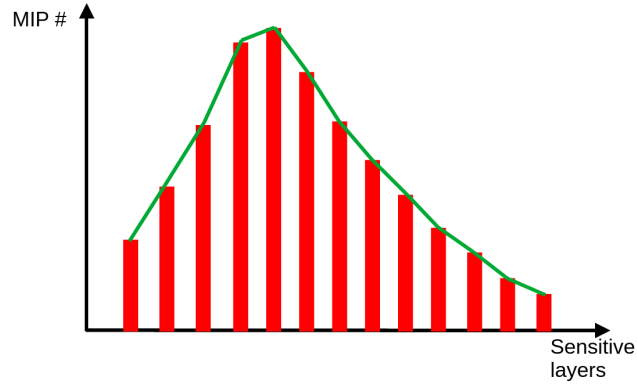
Figure 7.19: Principle of interpolation-based energy reconstruction: each red bar represents a sensitive layer with the green curve representing the interpolated longitudinal shower shape which is similar to the total shower energy.
