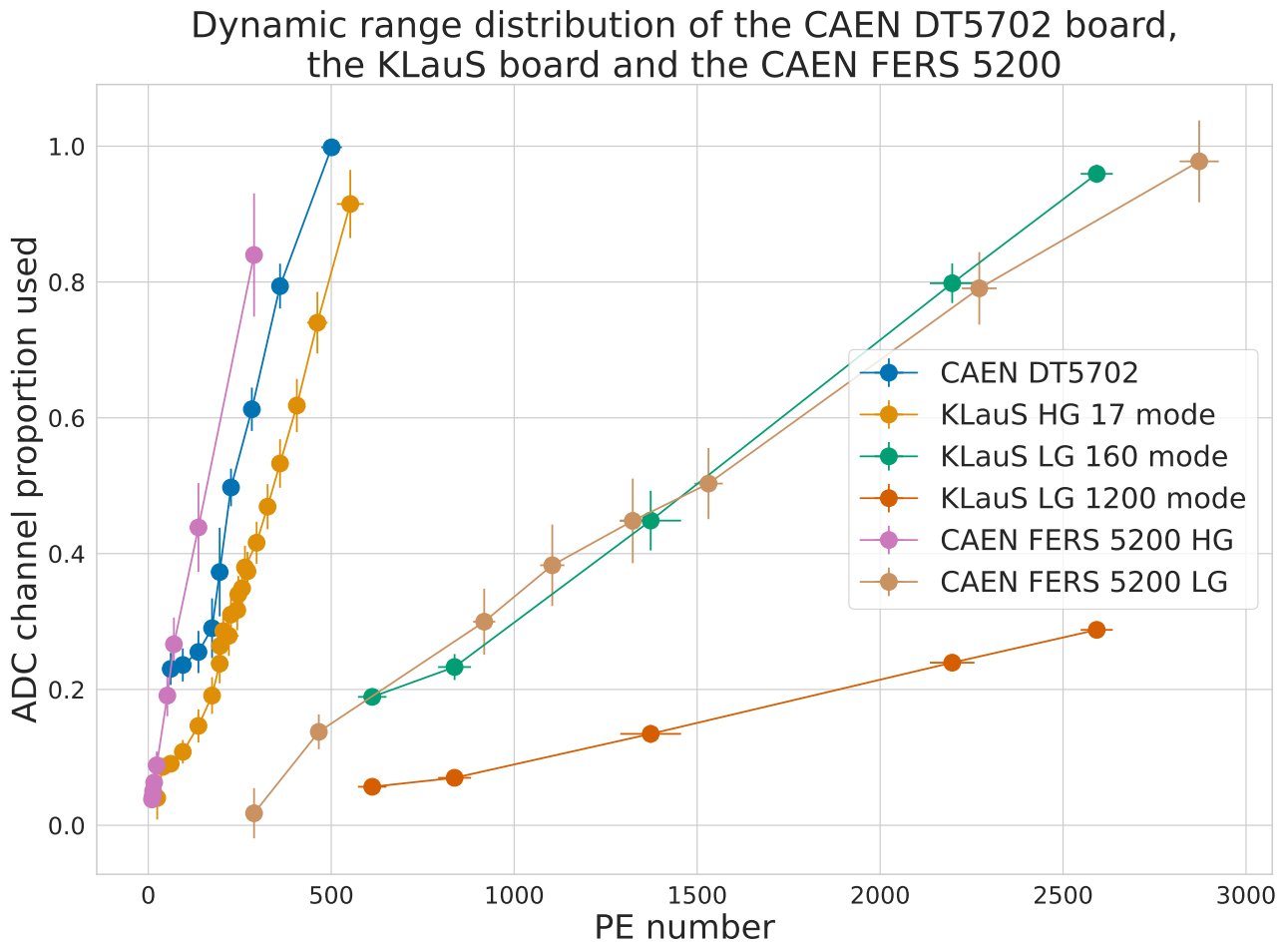
Figure 6.34: Dynamic range of the DT5702, DT5202 and KLauS chip. Saturation of the KLauS 1:200 branch could not be achieved for lack of sufficient coherent light input.
