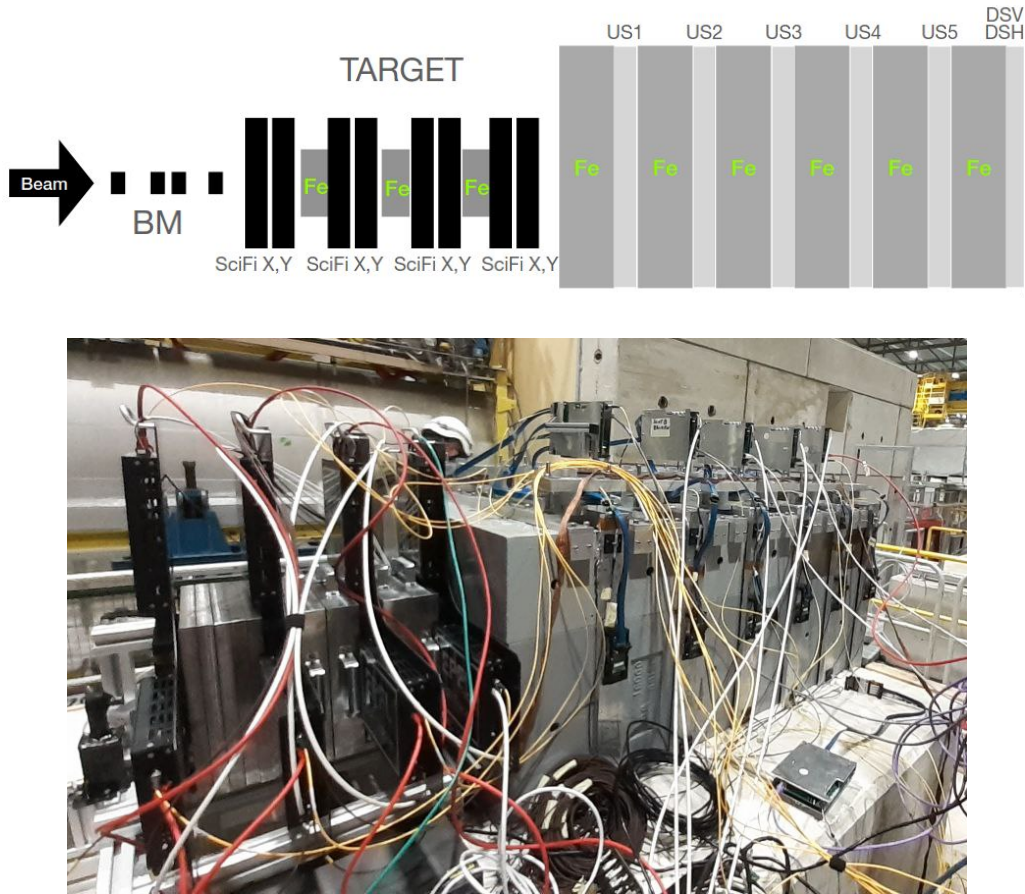
Figure 8.1: Test beam configuration, top graphic from [402].
