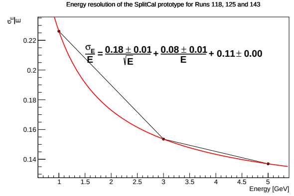
Figure 7.10: Reconstructed energies (left) and fitted resolution (red curve) (right) using gain 760.
