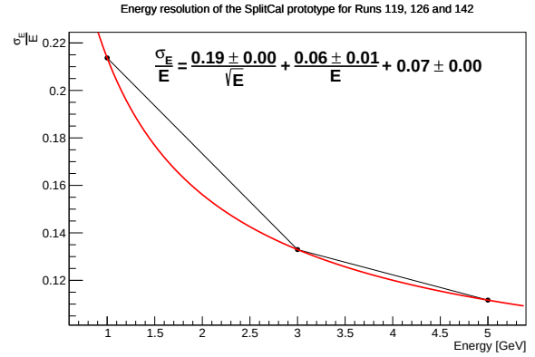
Figure 7.11: Reconstructed energies (left) and fitted resolution (red curve) (right) using gain 7200.
