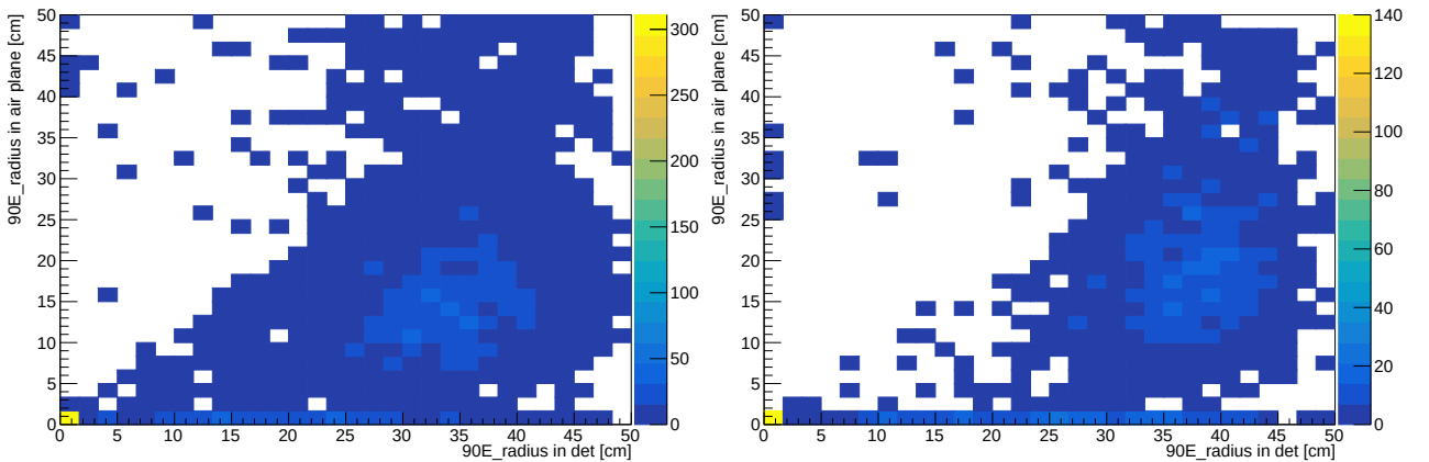
Figure 8.10: Correlation between 90E_radius in the air plane and in US1 for 100 GeV (left) \pi^+ and 300 GeV (right) \pi^- .
