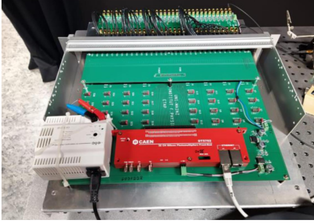
Figure 6.1: DT5702 as integrated as the initial prototype's readout electronics (left) and DT5702 block diagram (right) [386].
