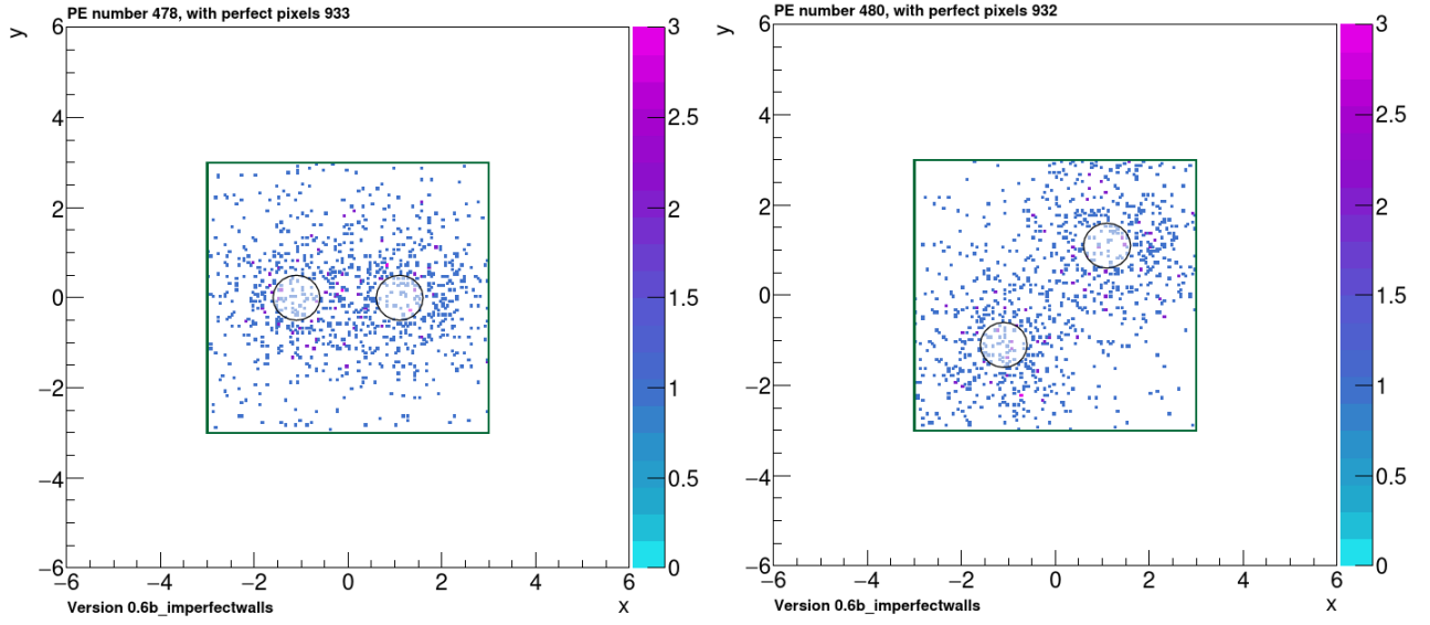
Figure 5.41: PE count for straight fibres (left) and fibre rotated by \frac{\pi}{4} (right) for 1000 incoming photons: 478 and 480 rPEs are found respectively. The green square delimits the SiPM sensitive area.
