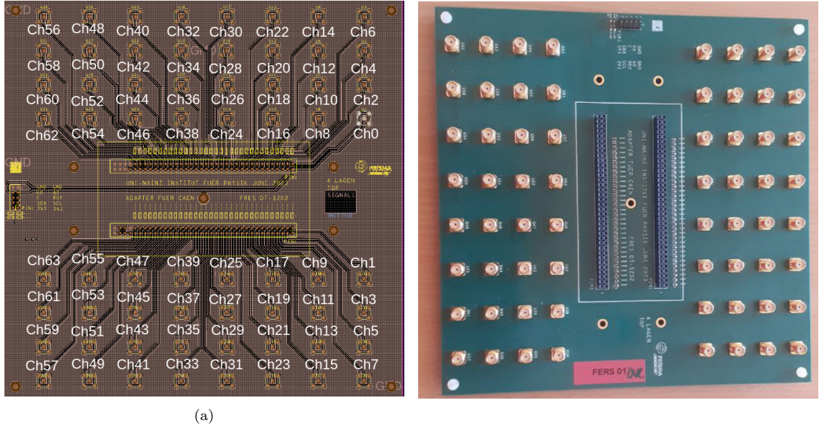
Figure 6.5: Layout (left) and top layer of the designed adapter board. The FERS system is plugged into it from the top
