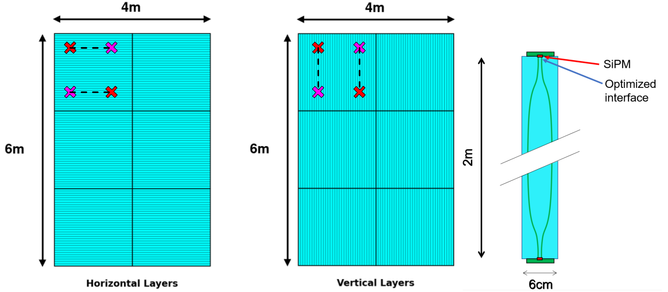
Figure 4.11: SHiP calorimeter system module and single bar design for the energy reconstruction layers. The red crosses represent real hits whereas the pink ones represent ambiguities.
