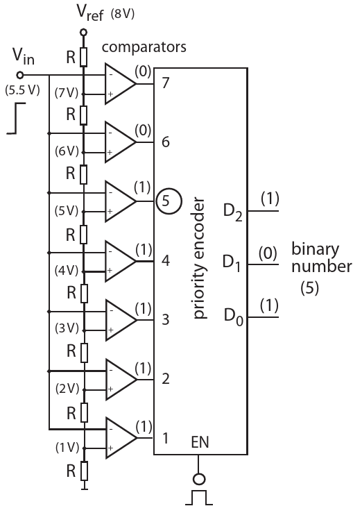
(a) Flash ADC block diagram. Each comparator has a threshold higher than its predecessor in the chain. A priority encoder finds the highest comparator (5 in this example) and delivers a code based on its inputs [330]. (b) Architecture of 4-bit SAR ADC. The capacitor array is digitally weighted: 16C, 8C, 4C, 2C and C [413].
