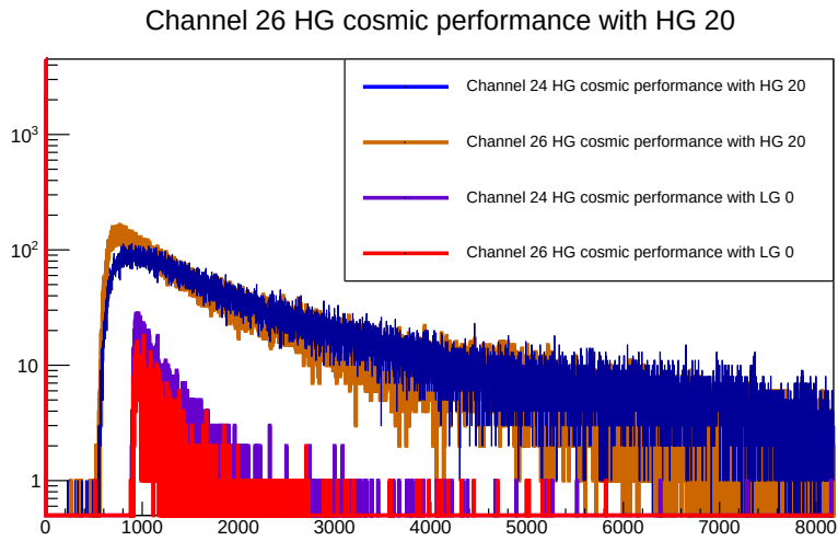
Figure 6.18: Example transition between HG and LG in cosmoics radiation.
