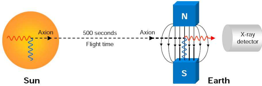
Figure 1.9: Detection concept for the magnet helioscope idea. Where the Sun is used as an intense source of axions.
