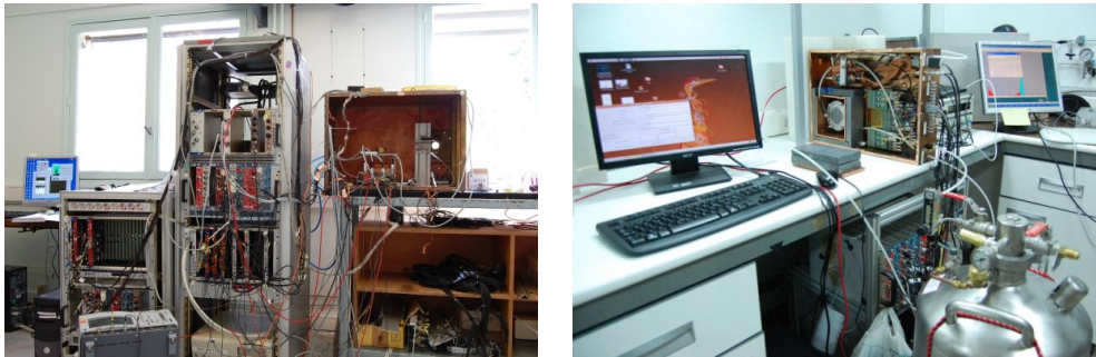
Figure 10.7: On the left, Micromegas acquisition set-up at CEA Saclay. On the right, Micromegas acquisition set-up at Zaragoza.
