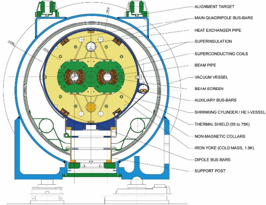
Figure 2.3: Schematic of the dipole magnet cross-section.
