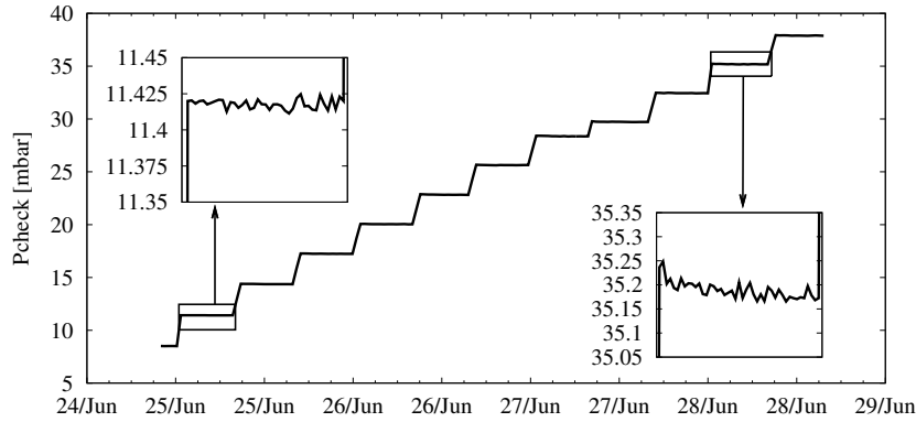
Figure 6.8: Plot representing the measured pressure, already corrected with the temperature of the magnet. The different steps observed in the plot correspond to the 8 hours stabilization time of the system. In the last steps it is already observed a dependency with the windows temperature.
