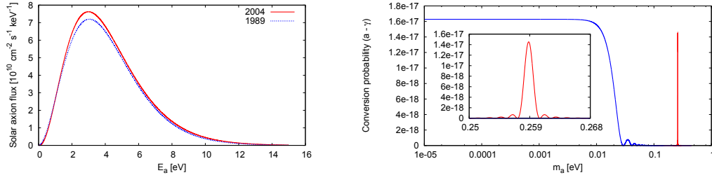
Figure 9.2: Expected axion solar flux on Earth (left) and probability conversion of axion to photon in the presence of a transversal magnetic field in CAST conditions (CAST vacuum phase and a resonance given by a fixed density in the magnet bore).
