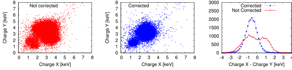
Figure 4.5: On the left, the distribution map of chargeX and chargeY , generated by an ^{55}\text{Fe} X-ray source, for a detector with missing strips charge. On the middle, the same distribution map after applying the dead strips virtual charge correction. On the right, the effect of the correction in the deviation of chargeX and chargeY parameters.
