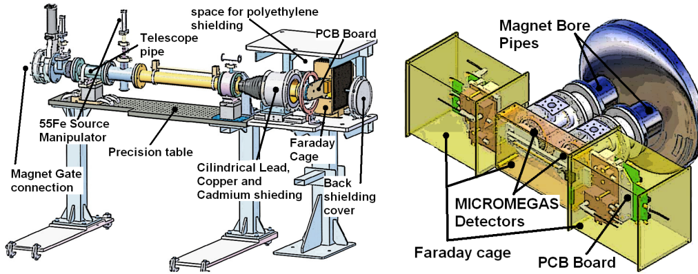
Figure 9.6: Drawing from the new Micromegas detection line installed at the sunrise side (left) and the new Micromegas detectors system installed at the sunset side (right).
