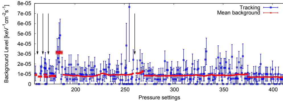
Figure 10.8: Tracking rates and mean background rate defined as a function of the step numbers measured in 2008.
