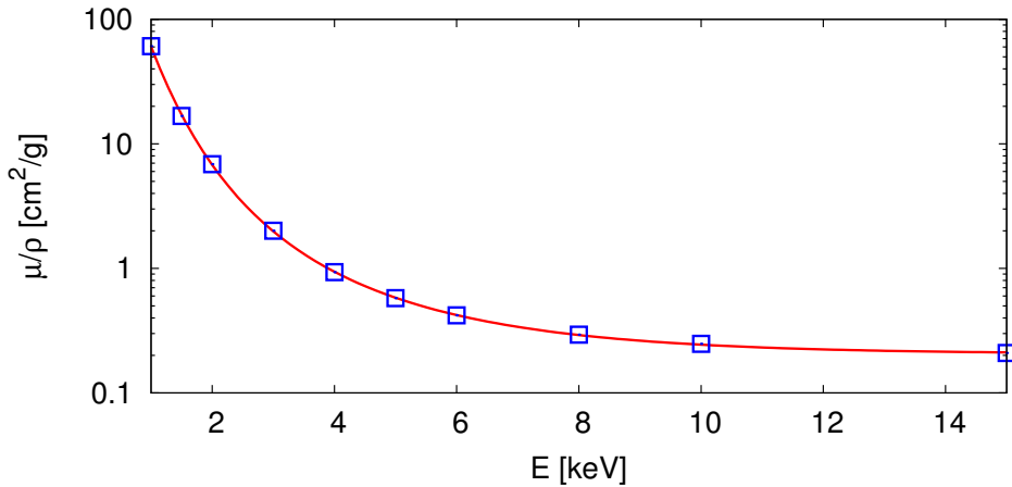
Figure 8.1: The helium mass absorption coefficient data obtained from NIST database, and the interpolated curve obtained with expression 8.1
