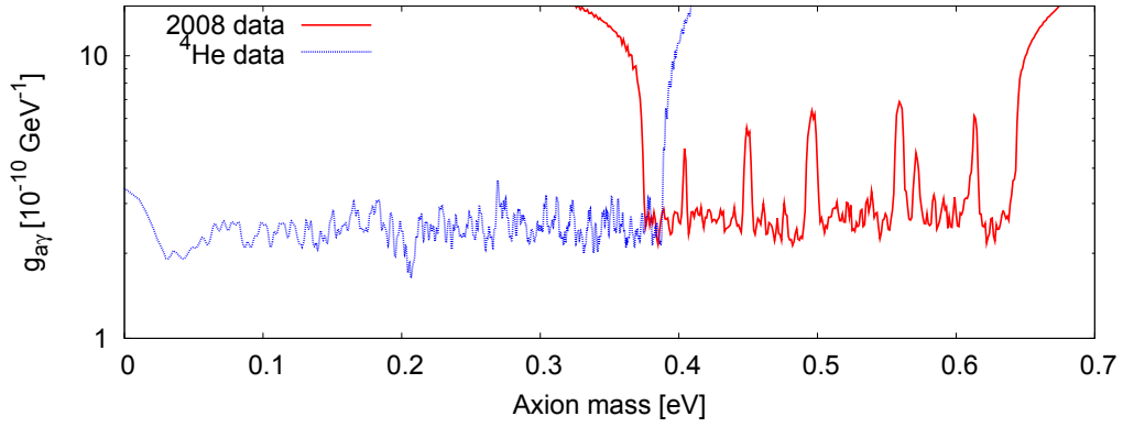
Figure 8.5: Axion-photon coupling limit for the second phase of CAST, corresponding to ^4\text{He} Phase data taking period in 2005 and 2006, and ^3\text{He} Phase in 2008, reached with the micromegas Sunrise Line.
