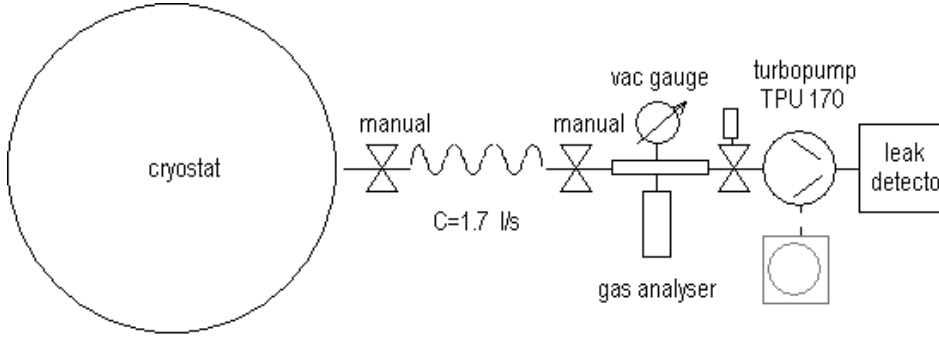
Figure 6.3: Schematic of the system connected to the CAST magnet cryostat for direct leak detection.
