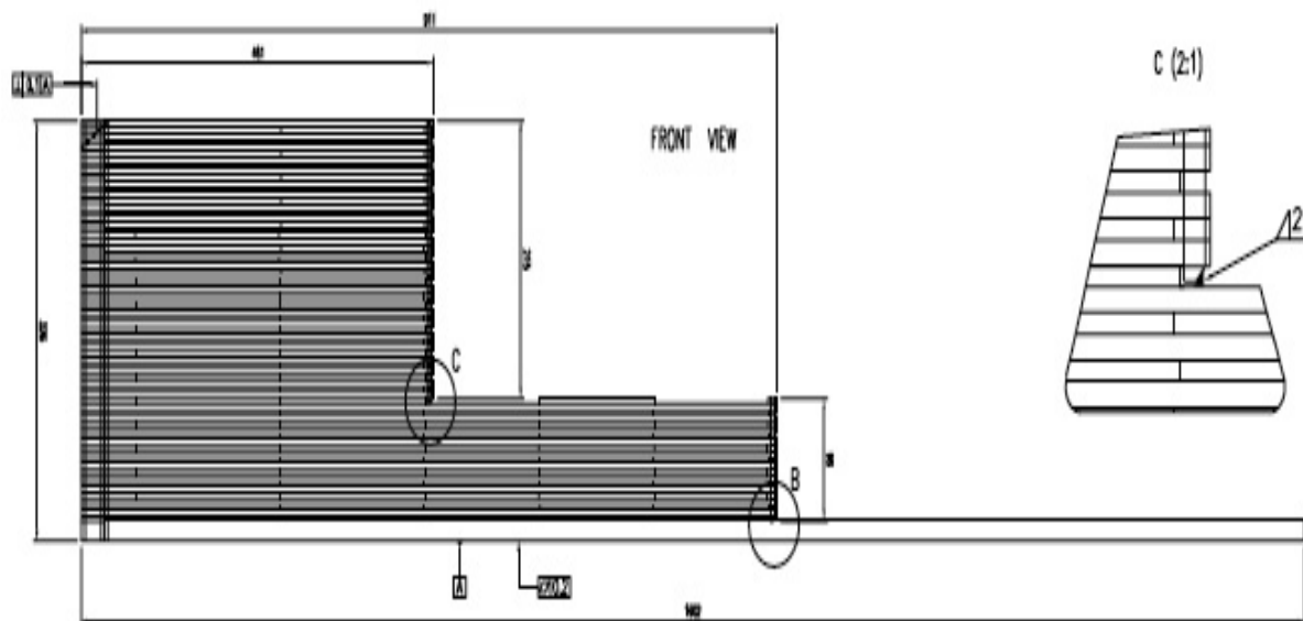
Figure 3.3. Transverse View of an ITC Module.
