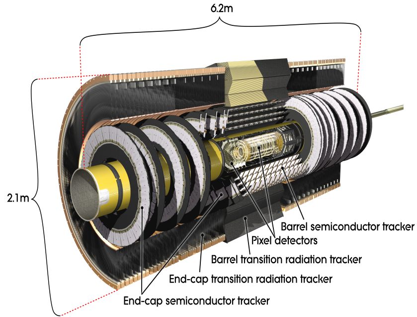
Figure 1.5. 3-Dimensional computer generated image of the Inner Detector.
