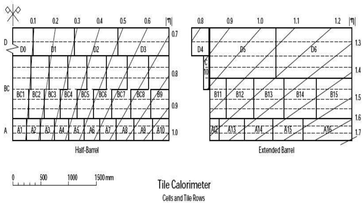
Figure 3.2. Schematic of Tile Calorimeter Cells and Rows.
