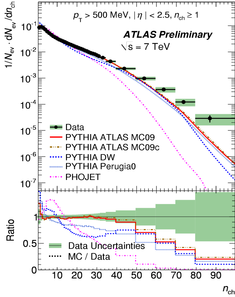
Figure 4.8. Multiplicity distribution for charged particles for \sqrt{s} = 7 TeV.
