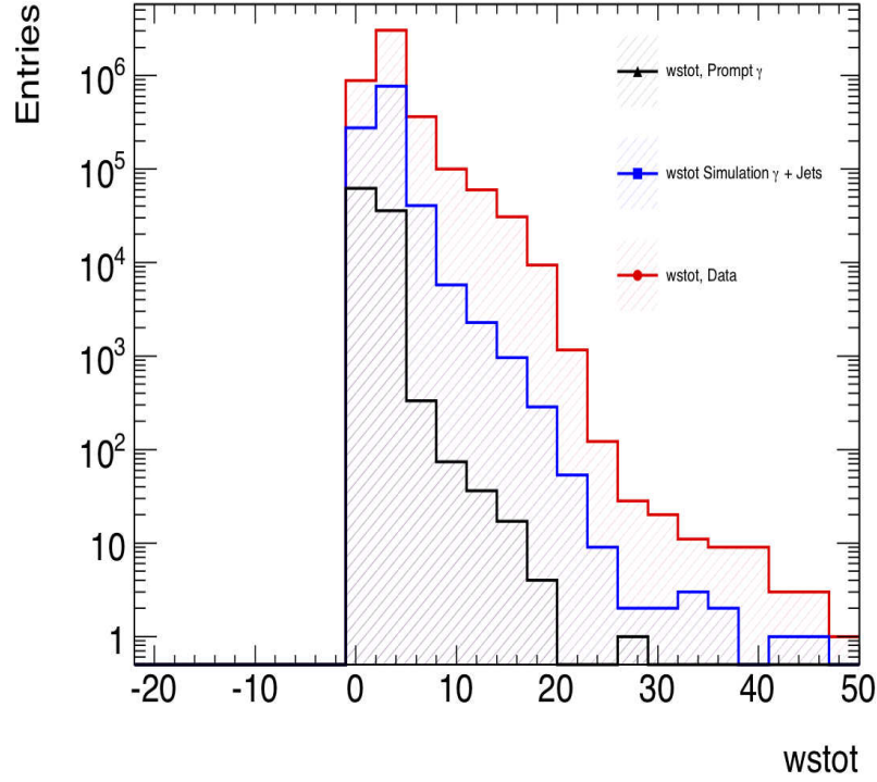
Figure 6.13. w_{tot} distribution for data and Monte Carlo.
