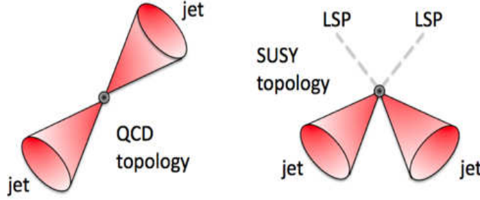
Figure 5.7. Diagrammatic representation of the difference in topologies for QCD events and SUSY events.
