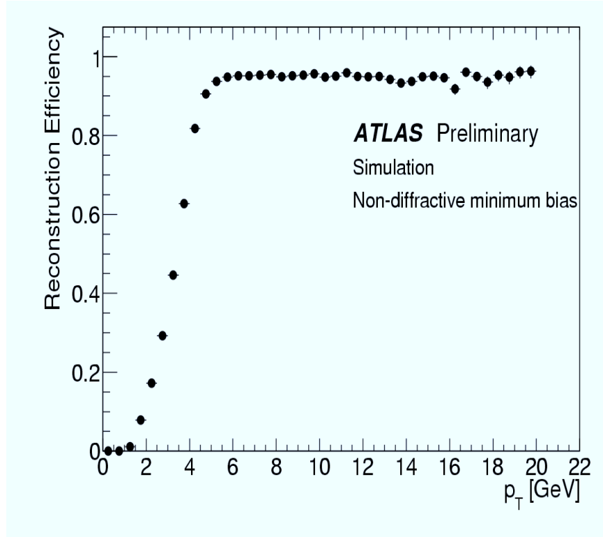
Figure 3.1. Muon reconstruction efficiency as a function of muon transverse momentum.
