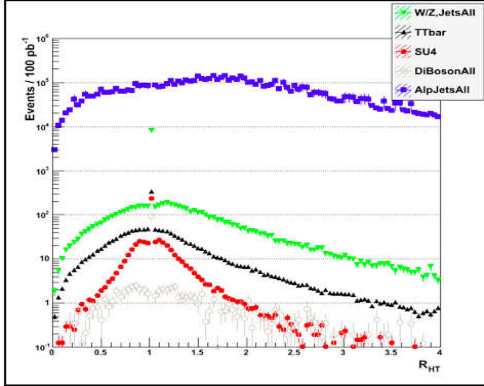
Figure 5.19. Distribution of R(H_T) for multi-jet case.
