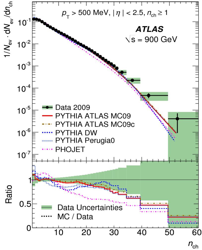
Figure 4.9. Multiplicity distribution for charged particles for \sqrt{s} = 0.9 TeV.
