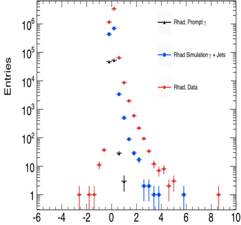
Figure 6.8. R_{had} distribution for data and Monte Carlo.
