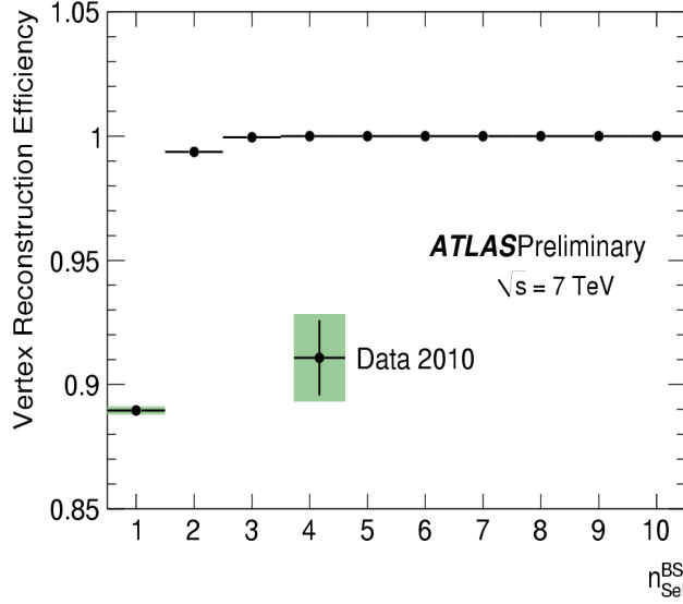
Figure 4.5. Vertex reconstruction efficiency as a function of n_{sel}^{BS} .
