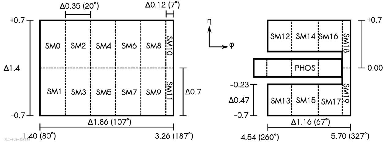
Figure 2.10: Layout of the EMCal and DCal supermodules in the \eta - \phi plane. Taken from Ref. [30]
