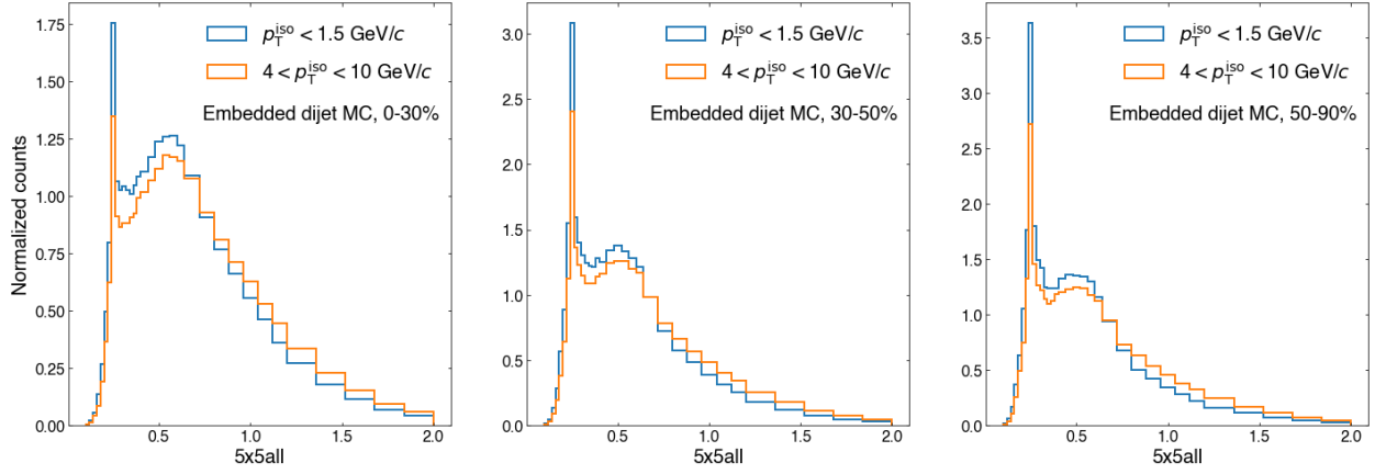
Figure 3.7: \sigma^2_{\text{long}(5 \times 5)} distributions in embedded dijet MC with the isolation (blue) and anti-isolation (orange) cuts
