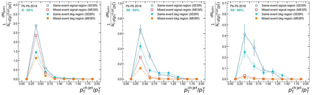
Figure 3.19: Raw p_T^{\text{jet}}/p_T^\gamma correlations for 2018 data
