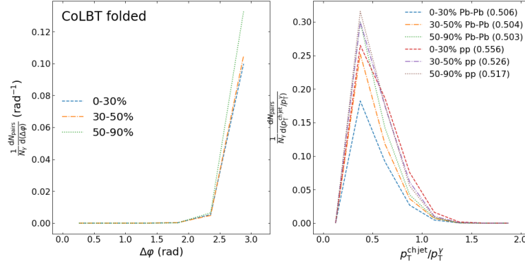
(b) CoLBT folded distributions; note that the right panel ( p_T^{\text{jet}}/p_T^\gamma ) is a one-dimensional unfolding and therefore does not have the p_T^{\text{jet}} > 10 GeV/ c cut
