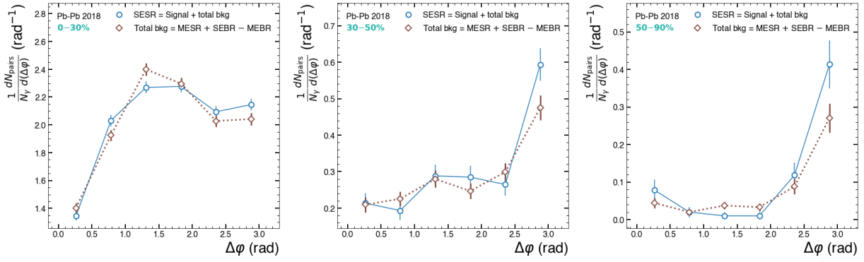
Figure 3.22: Signal and total background \Delta\varphi correlations for 2018 data
