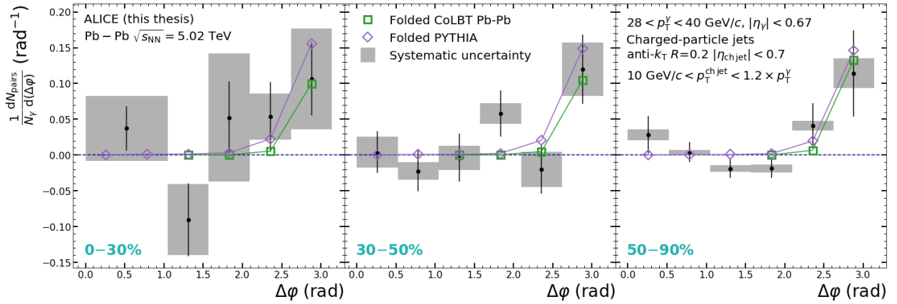
Figure 5.3: Comparison of data with folded theory calculations for \Delta\phi
