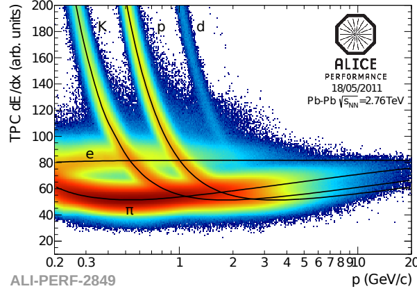
Figure 3.5.: The plot shows the dE/dx measurement versus momentum for data taken in Pb-Pb collisions in November 2010 (ALI-PERF-2849), and the theoretical Bethe-Bloch-Curves according to Equation 3.1 (black lines) for positrons, pions, kaons and protons.
