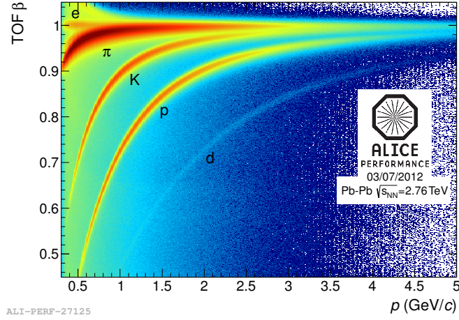
Figure 3.6.: Performance plot (ALI-PERF-27125) of the measured \beta = \frac{v}{c} in the ALICE TOF detector versus momentum for data taken in Pb–Pb collisions in 2011. This measurement can provide an e/\pi separation between 0.3 GeV/ c and 0.5 GeV/ c as well as separation of pions and kaon up to \sim 3 GeV/ c and kaons and proton up to \sim 4 GeV/ c . Even deuterons can be seen and separated by this measurement from 1 GeV/ c up to 5 GeV/ c .
