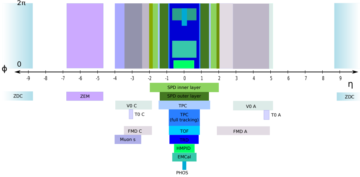
Figure 3.3.: Pseudo-rapidity and azimuthal coverage of the ALICE detector system.
