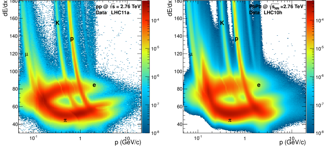
Figure 4.6.: dE/dx distribution in the TPC as a function of momentum for all secondary tracks, normalized to the number of events, after the basic track and V0 selection cuts for minimum bias pp (left) and Pb–Pb collisions (right).
