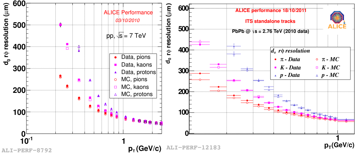
Figure 3.11.: Impact parameter resolution in pp (left, ALI-PERF-8792) and Pb–Pb collisions (right, ALI-PERF-12183) for different particle species as a function of p_T . For pp combined tracking of ITS and TPC is used, while in the Pb–Pb case the parameters are shown for ITS standalone tracking.
