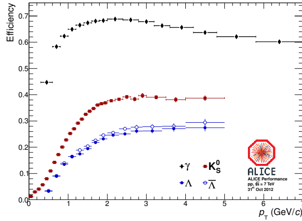
Figure 3.13.: Reconstruction efficiency of the On-the-flight V^0 finder for all reconstructible V^0 s versus p_T .
