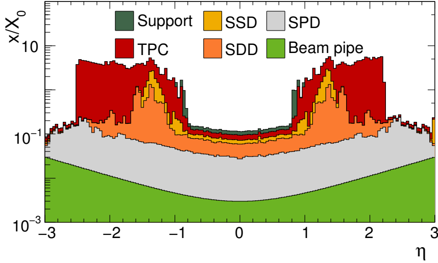
Figure 5.1.: Material distribution (in radiation length X_0 ) of the ALICE central tracking region as implemented in the simulation, averaged over the azimuthal angle [159]. Contributions of individual sub-detectors include services and support structures.
