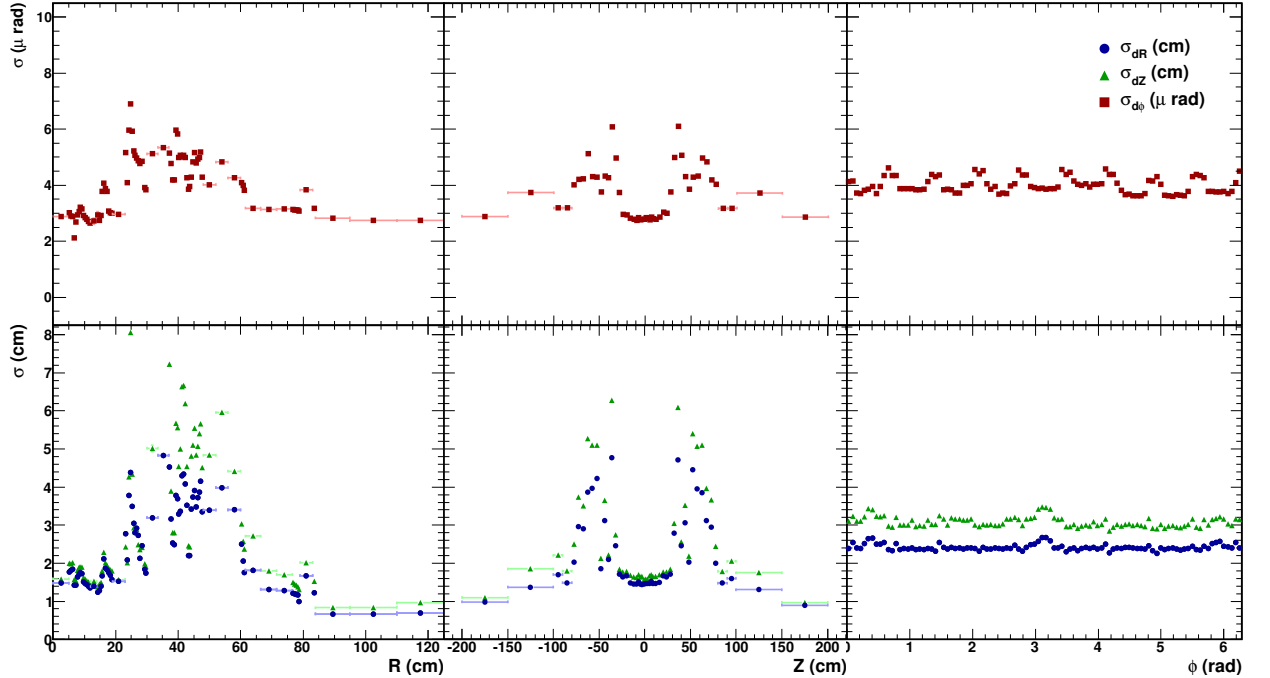
Figure 5.8.: Resolution of the reconstructed coordinates, \varphi (top), R and Z (bottom), of the conversion point versus R (left), Z (middle) and \varphi (right) for 0.9 < |\eta| < 1.4 . The resolutions are calculated fitting a Gaussian distribution to the dX = X_{\text{rec}} - X_{\text{MC}} ( X = R, Z, \Phi ), identifying the \sigma of the Gaussian distribution with the resolution in the corresponding coordinate.
