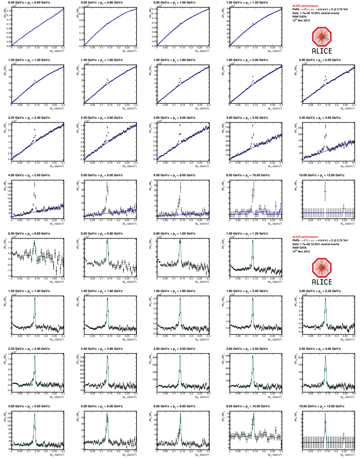
Figure B.17.: Invariant-mass distribution of reconstructed photon pairs M_{\gamma\gamma} around the neutral pion mass in p_T slices in 10-20 % Pb–Pb collisions at \sqrt{s_{NN}} = 2.76 TeV before (upper plot) and after subtraction (lower plot). The black histograms in the upper plot show the combined signal and background distribution and the blue histograms show the calculated and normalized mixed event background. After the subtraction the invariant mass distributions are fitted with Equation 6.3, which is shown in green in the lower plot.
