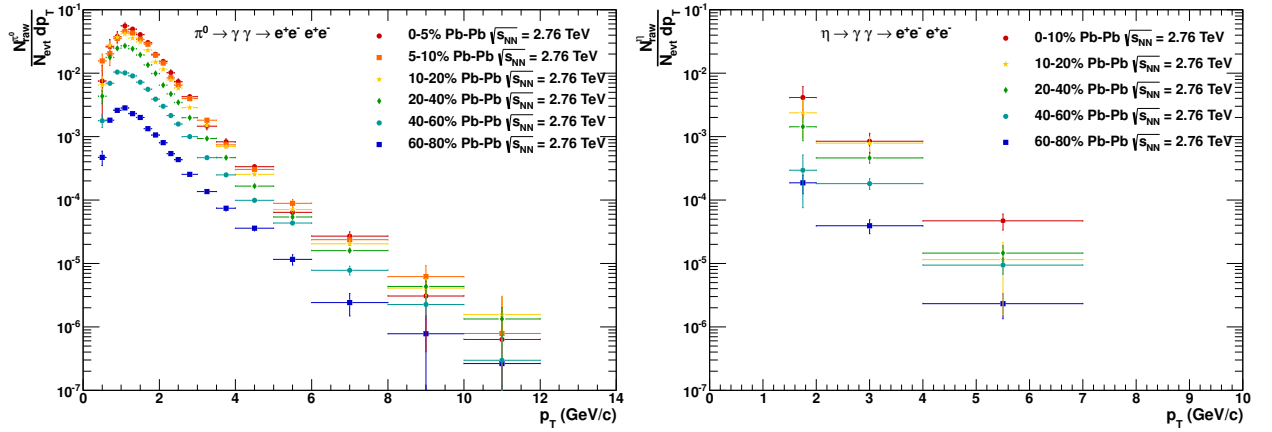
Figure 6.6.: Raw yield of the \pi^0 (left) and \eta (right) meson in Pb-Pb collisions at \sqrt{s} = 2.76 TeV. The yield is normalized to the number of events N_{evt} , according to Table 4.4 and the spectra are divided by the bin width in p_T .
