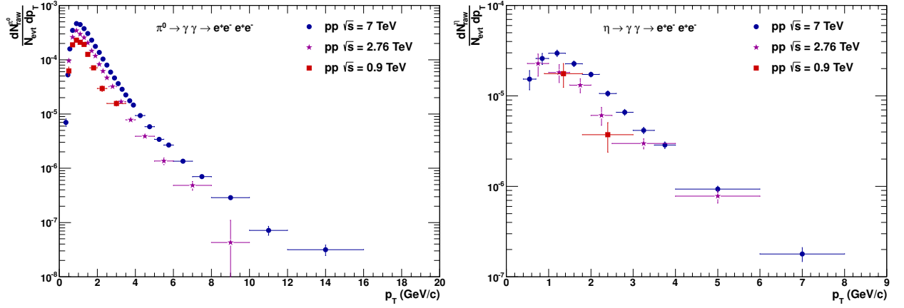
Figure 6.5.: Raw yield of the \pi^0 (left) and \eta (right) meson in pp collisions at \sqrt{s} = 0.9 (red), 2.76 (magenta) and 7 TeV (blue) as function of the transverse momentum. The yield is normalized to the number of events N_{evt} , according to Table 4.2 and the spectra are divided by the bin width in p_T .
