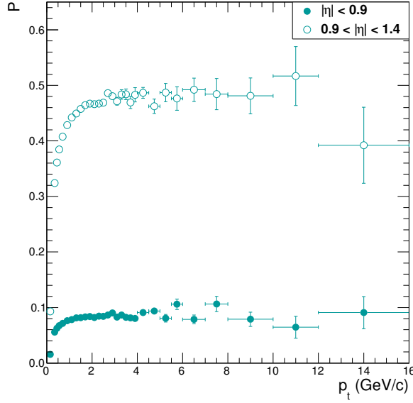
Figure 5.2.: Conversion probability for different regions in \eta .
