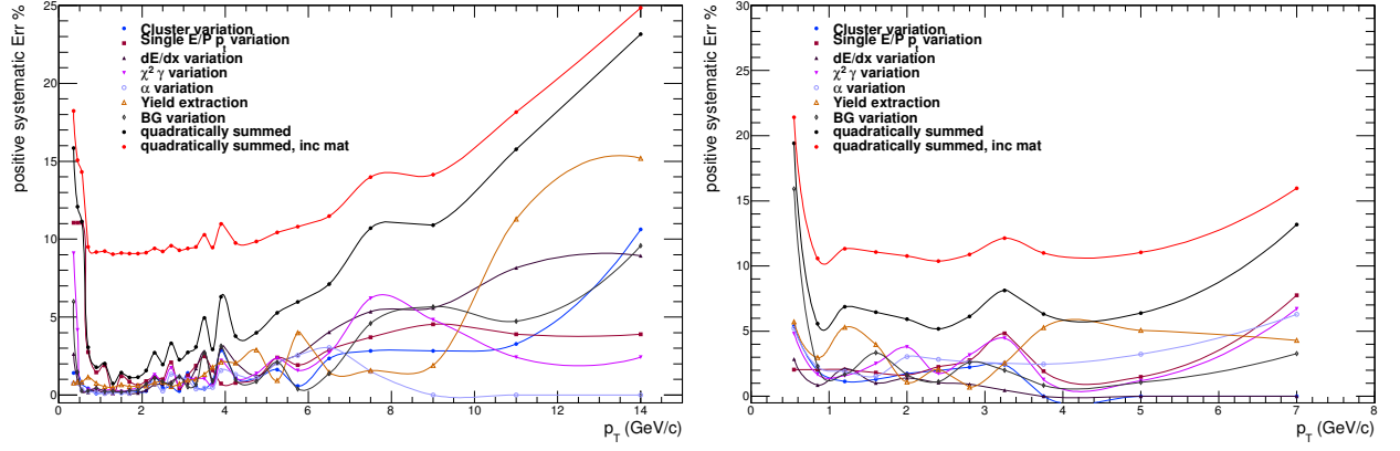
Figure B.9.: Visualization of the systematic errors for pp collisions at \sqrt{s} = 7 TeV. The colored points represent the individual error sources, while the red points represent the final systematic error for the \pi^0 (left) and \eta (right) meson spectra.
