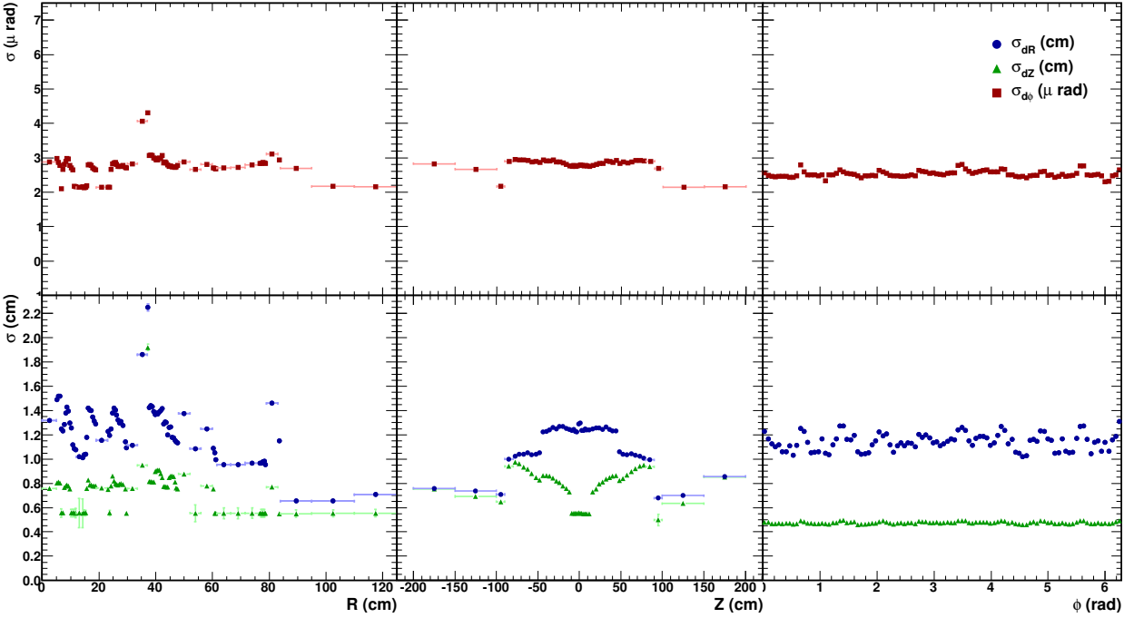
Figure 5.6.: Resolution of the reconstructed coordinates, \phi (top), R and Z (bottom), of the conversion point versus R (left), Z (middle) and \phi (right) for |\eta| < 0.9 . The resolutions are calculated fitting a Gaussian distribution to the dX = X_{\text{rec}} - X_{\text{MC}} ( X = R, Z, \Phi ), identifying the \sigma of the Gaussian distribution with the resolution in the corresponding coordinate.
