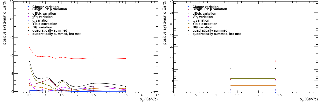
Figure B.4.: Visualization of the systematic errors for pp collisions at \sqrt{s} = 7 TeV. The colored points represent the individual error sources, while the red points represent the final systematic error for the \pi^0 (left) and \eta (right) meson spectra.
