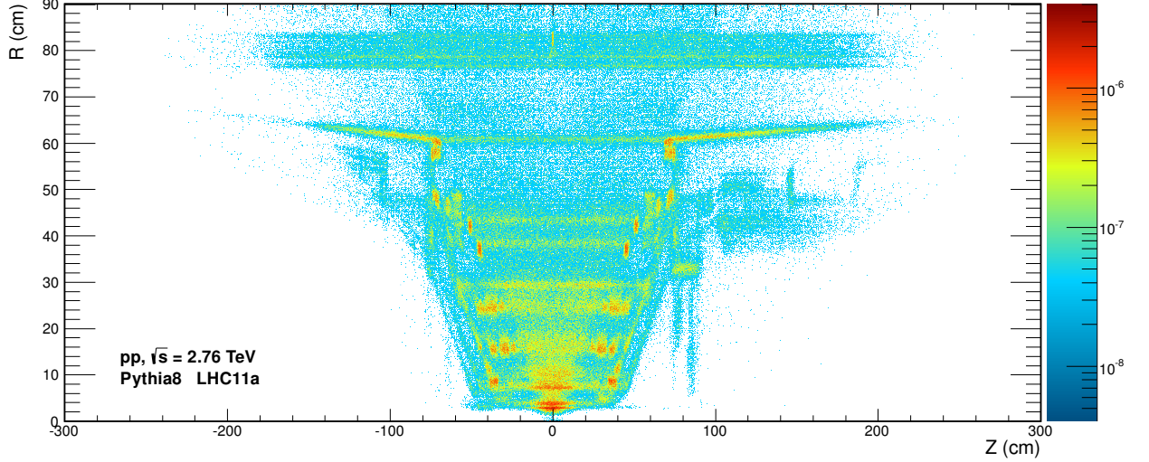
Figure 5.15.: Distribution of the secondary hadronic vertices normalized to the number of events in the ZR -plane for the full pseudo-rapidity range accessible by the SHIM reconstructed in Pythia 8 simulations for pp collisions at \sqrt{s} = 2.76 TeV.
