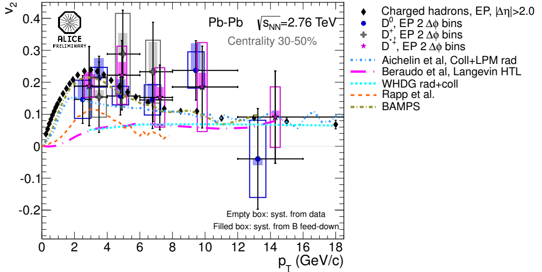
Figure 2.9.: v_2 as a function of transverse momentum for various D-mesons [73] together with the charged particle v_2 [68] and theoretical calculations [74–79].
