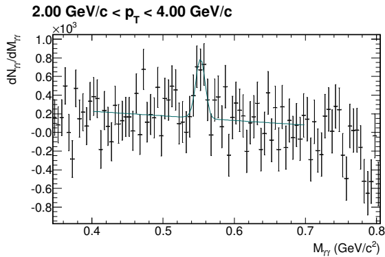
Figure B.14.: Invariant-mass distribution of reconstructed photon pairs M_{\gamma\gamma} around the eta meson mass in p_T slices in 0-10 Pb-Pb collisions at \sqrt{s_{NN}} = 2.76 TeV before (upper plot) and after subtraction (lower plot). The black histograms in the upper plot show the combined signal and background distribution and the blue histograms show the calculated and normalized mixed event background. After the subtraction the invariant mass distributions are fitted with Equation 6.3, which is shown in green in the lower plot.
