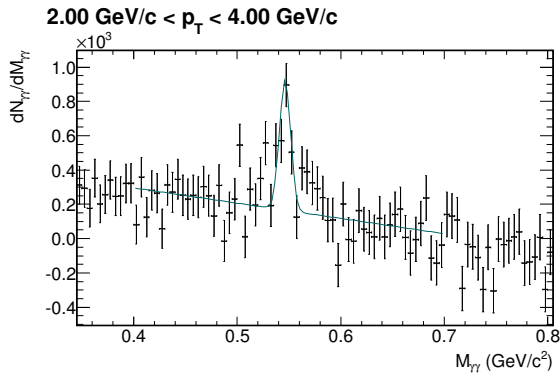
Figure B.18.: Invariant-mass distribution of reconstructed photon pairs M_{\gamma\gamma} around the eta meson mass in p_T slices in 20-40 Pb–Pb collisions at \sqrt{s_{NN}} = 2.76 TeV before (upper plot) and after subtraction (lower plot). The black histograms in the upper plot show the combined signal and background distribution and the blue histograms show the calculated and normalized mixed event background. After the subtraction the invariant mass distributions are fitted with Equation 6.3, which is shown in green in the lower plot.
