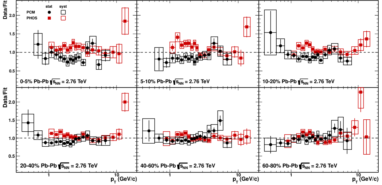
Figure 6.19.: Ratio of the fully corrected \pi^0 spectra in Pb-Pb collisions at \sqrt{s_{NN}} = 2.76 TeV in six centrality bins measured with the PHOS and PCM methods to the fits to the combined result in each bin. The vertical lines represent the statistical errors, while the boxes indicate the individual systematic errors, the error of the fit it not included in the errors.
