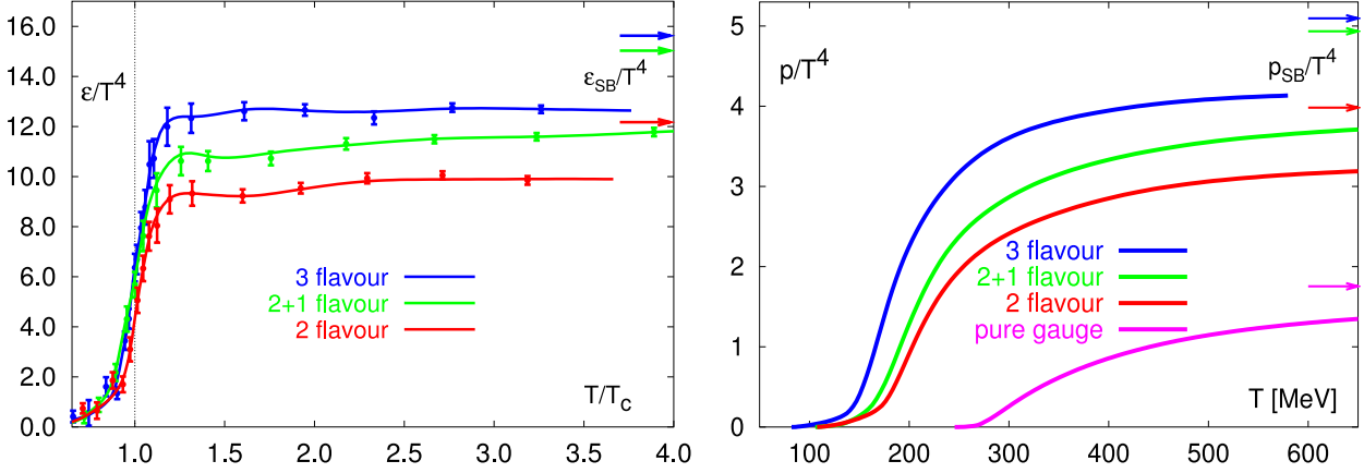
Figure 2.2.: Left: Energy density as a function of the temperature calculated with lattice QCD for different compositions of quark flavors. The critical temperature is around 174 MeV. Right: The pressure in QCD with different number of degrees of freedom as a function of temperature calculated with LQCD. The curves labeled (2 + 1)-flavour corresponds to a calculation with two light and a four times heavier strange quark mass. Taken from [30].
