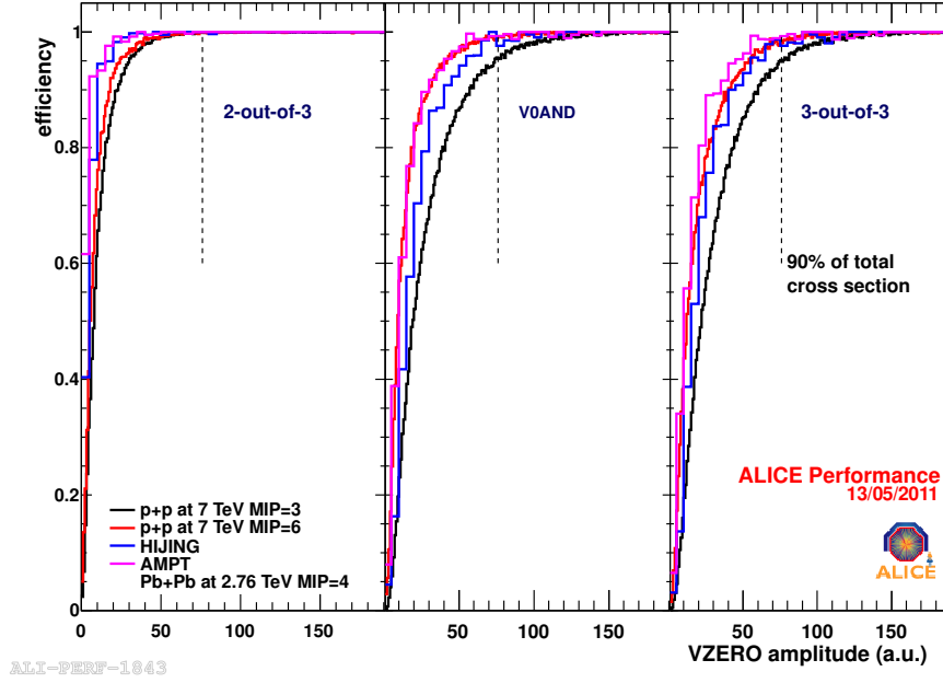
Figure 3.8.: Trigger efficiency for pp and Pb–Pb collisions under the detector conditions for data taken in 2010 (ALI-PERF-1843). The three different triggers use the VZERO and the SPD as inputs. For the left figure a coincidence of 2 out of the 3 detectors has to be present. This trigger measures the largest fraction of the total cross section. The central plot is a coincidence of V0-A and V0-C ( MB_{AND} ), which comes closest to the having NSD events. The last class is the coincidence of all 3 detectors this measures the smallest fraction of the total cross section. All of these classes have very similar efficiencies for heavy-ion collisions and pp collisions as seen by different histograms shown in the figures.
