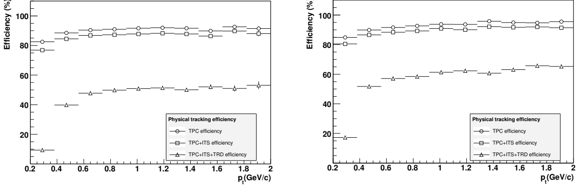
Figure 3.9.: Track finding efficiency for different combinations of tracking detector for central Pb–Pb collisions at dN_{ch}/d\eta = 6000 and pp collisions (right) [159].
