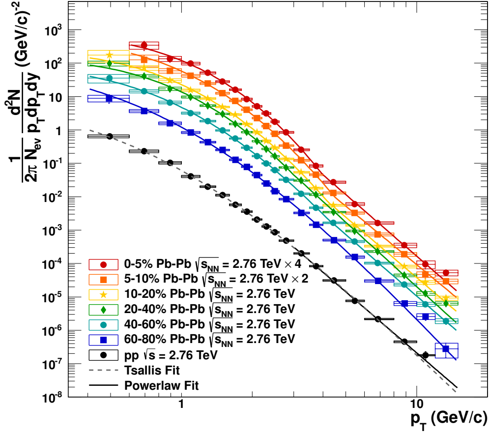
Figure 6.18.: \pi^0 meson differential invariant yield for different centrality classes in Pb–Pb collisions at \sqrt{s_{NN}} = 2.76 TeV and for pp collisions at \sqrt{s} = 2.76 TeV. The pp result was fitted with a pure power law (solid black line, Equation 6.8) and a Tsallis function (dashed gray line, Equation 6.7). For Pb–Pb collisions the spectra have been fitted with a combination of a power law at high momentum and a Tsallis function at low momentum. The resulting fit for each centrality is displayed in the corresponding color.
