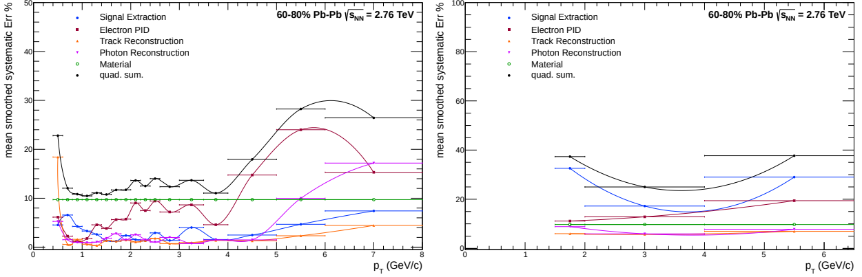
Figure 6.11.: Visualization of the systematic errors for 60-80% Pb–Pb collisions at \sqrt{s_{NN}} = 2.76 TeV. The colored points represent the individual error sources, while the black points represent the final systematic error for the \pi^0 (left) and \eta (right) meson spectra.
