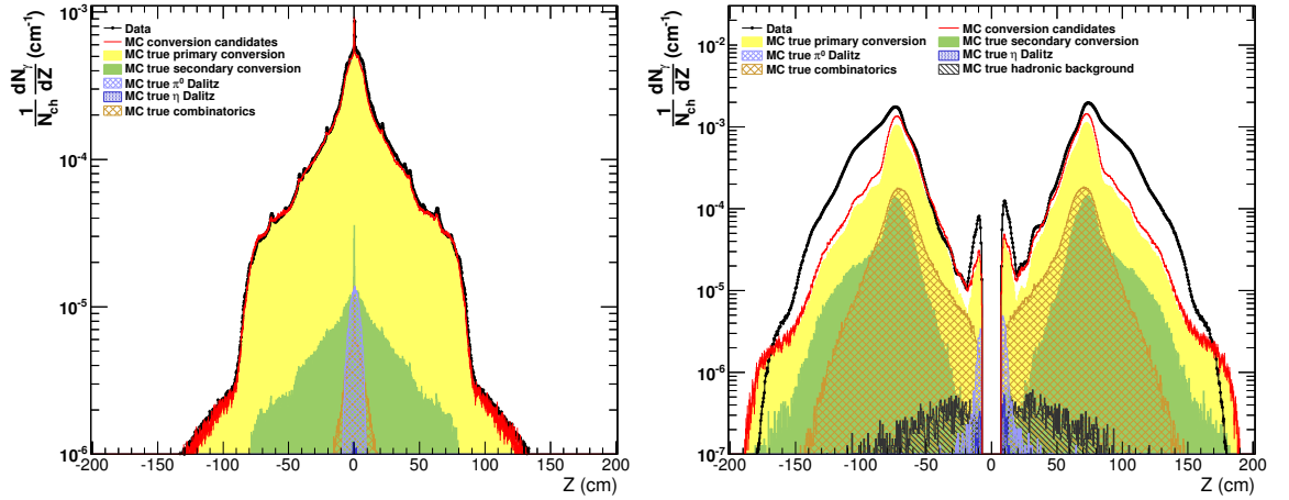
Figure 5.10.: Z distribution of the reconstructed conversion points (black) for |\eta| < 0.9 (left) and 0.9 < |\eta| < 1.4 (right) compared to Monte Carlo simulations done with Pythia 6 tune Perugia 0 (red). The distribution for true primary (secondary) converted photons is shown in yellow (green), while the physics contamination from true \pi^0 and \eta Dalitz decays is shown in blue dashed. The true random combinatorial background is shown in brown, while the hadronic background (contamination from e.g. K_s^0 , \Lambda , \bar{\Lambda} ) is shown in black.
