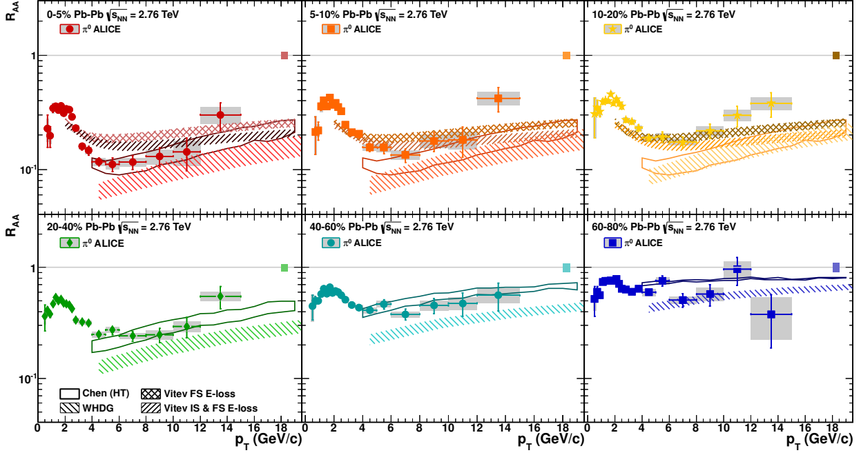
Figure 6.23.: Comparison of the measured R_{AA} to predictions from the WHDG model [190,191] and the higher-twist calculations by Chen et al. [192]. For the first three centrality classes only the WHDG model predictions are available for each centrality bin, thus the comparison has been done to the higher-twist calculations in the 0-20% central events. Moreover, these three centrality classes are compared to the calculations by I. Vitev et al. with and without initial state (IS) parton energy loss in addition to final state (FS) energy loss for the 0-20% most events [193,194].
