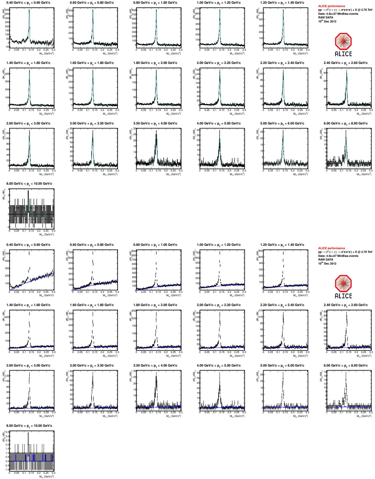
Figure B.3.: Invariant-mass distribution of reconstructed photon pairs M_{\gamma\gamma} around the neutral pion mass in p_T slices in pp collisions at \sqrt{s} = 2.76 TeV before (upper plot) and after subtraction (lower plot). The black histograms in the upper plot show the combined signal and background distribution and the blue histograms show the calculated and normalized mixed event background. After the subtraction the invariant mass distributions are fitted with Equation 6.3, which is shown in green in the lower plot.
