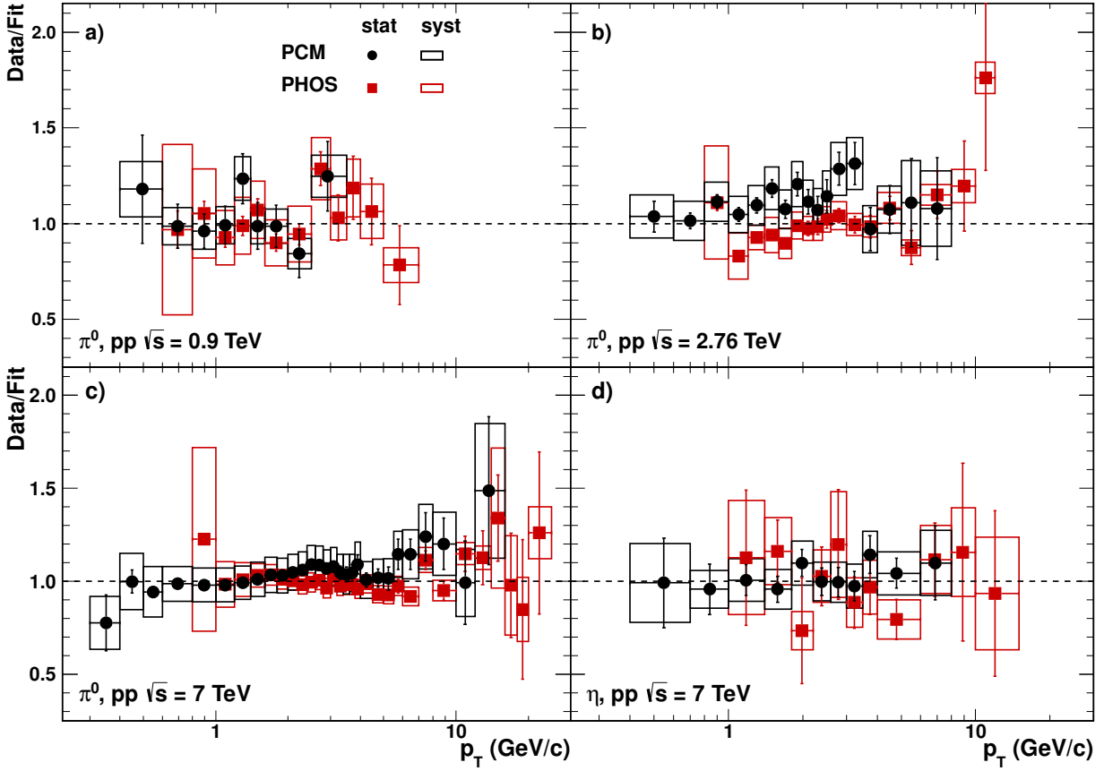
Figure 6.14.: Ratio of the two independent \pi^0 meson measurements in pp collisions at \sqrt{s} = 0.9, 2.76 and 7 TeV (a-c) to the fit of the combined normalized invariant production cross section at the corresponding energies. Moreover, the comparison for the \eta meson at \sqrt{s} = 7 TeV (d) is shown.
