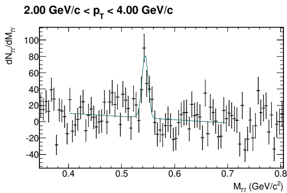
Figure B.22.: Invariant-mass distribution of reconstructed photon pairs M_{\gamma\gamma} around the eta meson mass in p_T slices in 60-80 Pb–Pb collisions at \sqrt{s_{NN}} = 2.76 TeV before (upper plot) and after subtraction (lower plot). The black histograms in the upper plot show the combined signal and background distribution and the blue histograms show the calculated and normalized mixed event background. After the subtraction the invariant mass distributions are fitted with Equation 6.3, which is shown in green in the lower plot.
