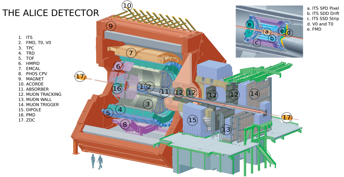
Figure 3.2.: Layout of the ALICE detector system with an insert zooming into the detectors closest to the beam pipe [136].
