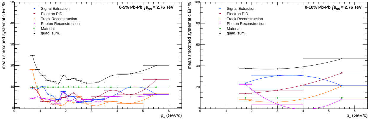
Figure 6.12.: Visualization of the systematic errors for the \pi^0 (left) and \eta (right) meson for 0-5%(0-10%) Pb–Pb collisions at \sqrt{s_{NN}} = 2.76 TeV. The colored points represent the individual error sources, while the black points represent the final systematic error of the spectra.
