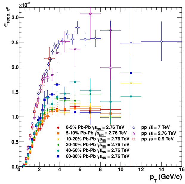
Figure B.1.: Neutral pion reconstruction efficiency obtained from Monte Carlo simulations for pp collisions at \sqrt{s} = 0.9, 2.76 and 7 TeV as well as Pb–Pb collisions in different centrality bins.
