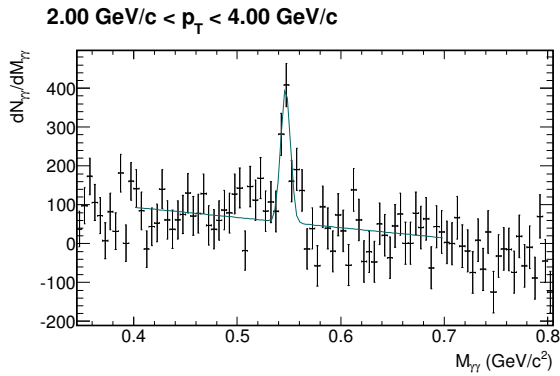
Figure B.20.: Invariant-mass distribution of reconstructed photon pairs M_{\gamma\gamma} around the eta meson mass in p_T slices in 40-60 Pb-Pb collisions at \sqrt{s_{NN}} = 2.76 TeV before (upper plot) and after subtraction (lower plot). The black histograms in the upper plot show the combined signal and background distribution and the blue histograms show the calculated and normalized mixed event background. After the subtraction the invariant mass distributions are fitted with Equation 6.3, which is shown in green in the lower plot.
