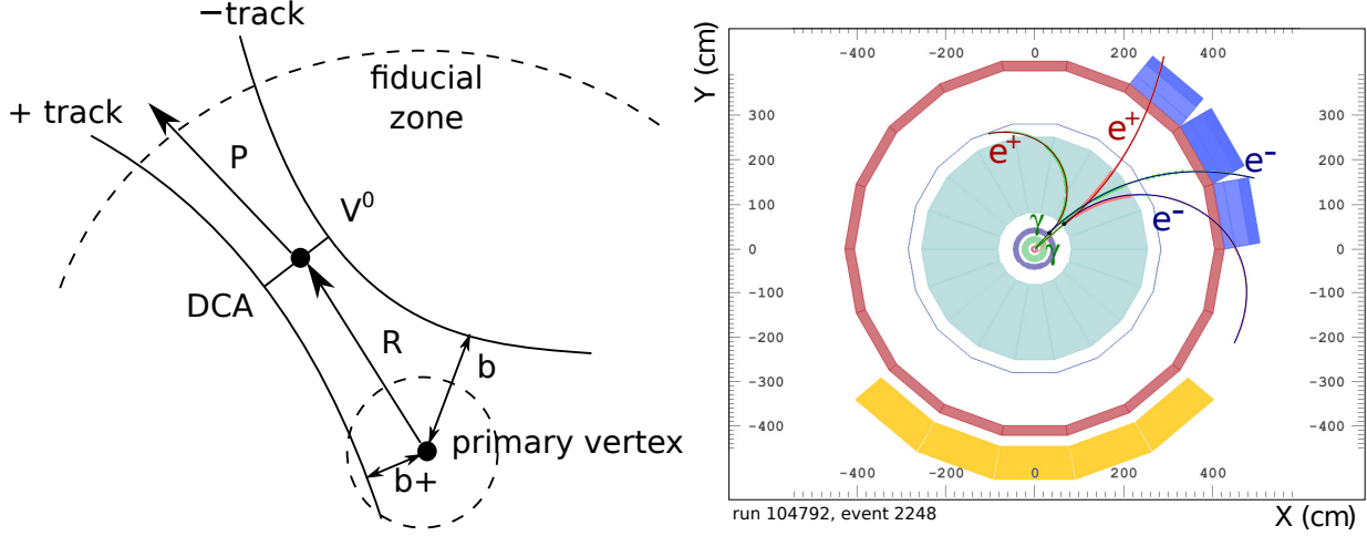
Figure 3.12.: Sketch of the reconstruction of a generic secondary vertex (left) [159] and a reconstructed \pi^0 candidate from 2009 data taking campaign at \sqrt{s} = 900 GeV (right). The reconstructed event shows a \pi^0 meson candidate from 2 reconstructed photon conversions using the V^0 method.
