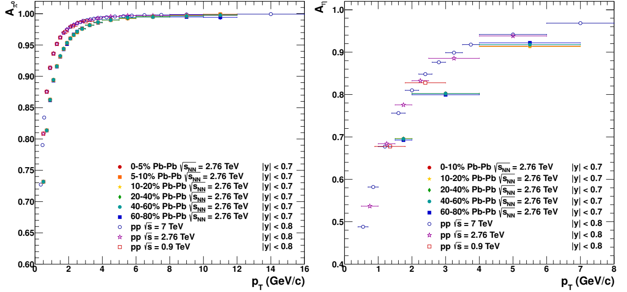
Figure 6.8.: Geometrical acceptance of the \pi^0 (left) and \eta (right) meson in pp collisions at \sqrt{s} = 0.9, 2.76 and 7 TeV, as well as Pb–Pb collisions in all centrality bins considered in this analysis.
