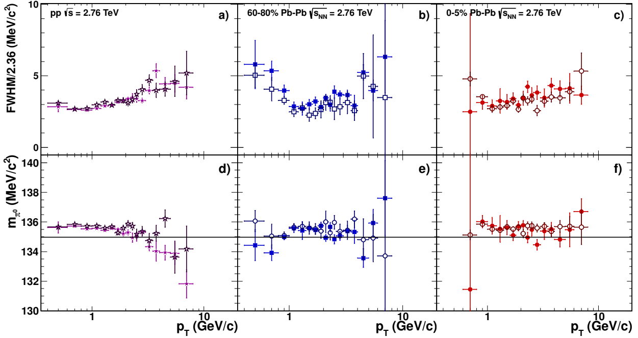
Figure 6.3.: Reconstructed mass resolution (a-c) and mass (d-f) for the \pi^0 meson as function of transverse momentum for pp collisions at \sqrt{s} = 2.76 TeV (a,d) as well as 60-80% (b,e) and 0-5% central Pb-Pb collisions (c,f). The parameters are extracted using the fit described in Equation 6.3. The simulated data is represented by the open symbols, while the real data are shown with filled symbols. Moreover, the nominal mass position according to [130] is indicated by the black line. The resolution is given as the full width at half maximum (FWHM) divided by 2.36 in order to show the corresponding width of the peak in terms of \sigma of a pure Gaussian distribution.
