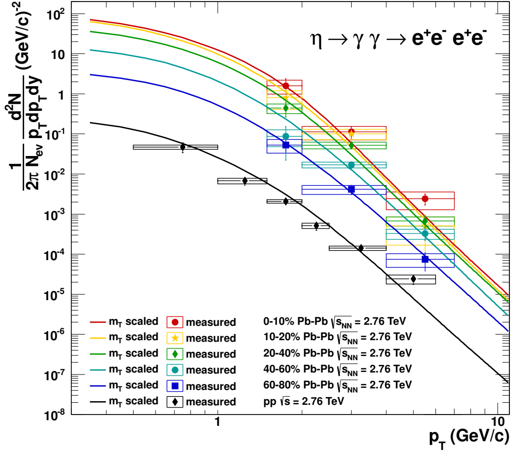
Figure 6.21.: \eta differential invariant yield for different centrality classes in Pb–Pb collisions at \sqrt{s_{\text{NN}}} = 2.76 TeV and for pp collisions at \sqrt{s} = 2.76 TeV. The spectra expected from m_T scaling of the neutral pions are shown as colored lines for the respective centrality classes and collision systems. For the spectra in Pb–Pb collisions no bin width correction (Section 6.1.2) has been applied.
