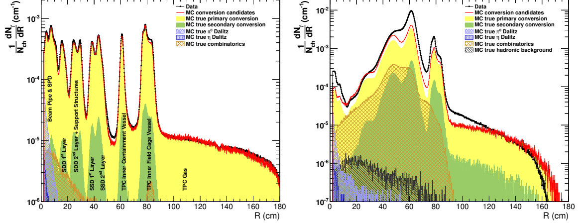
Figure 5.9.: R distribution of the reconstructed conversion points (black) for |\eta| < 0.9 (left) and 0.9 < |\eta| < 1.4 (right) compared to Monte Carlo simulations done with Pythia 6 tune Perugia 0 (red). The distribution for true primary (secondary) converted photons is shown in yellow (green), while the physics contamination from true \pi^0 and \eta Dalitz decays is shown in blue dashed. The true random combinatorial background is shown in brown, while the hadronic background (contamination from e.g. K_s^0 , \Lambda , \bar{\Lambda} ) is shown in black.
