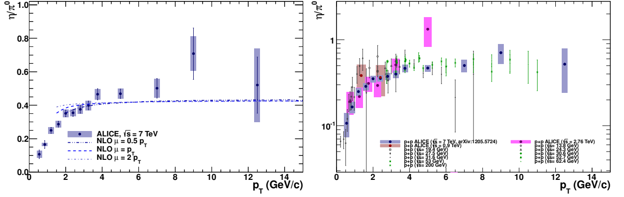
Figure 6.17.: Left: Measured \eta/\pi^0 ratio at \sqrt{s} = 7 TeV as a function of transverse momentum compared to theory [127]. Right: Measured \eta/\pi^0 ratio at \sqrt{s} = 0.9 (red), 2.76 (purple) and 7 TeV (blue) as a function of transverse momentum and previous measurements at lower energies [205]. While the boxes in the left plot reflect the systematic uncertainties and the error bars show the statistical error, the boxes in the right plot indicate the quadratically summed statistical and systematic error as the error bars for the lower energy data.
