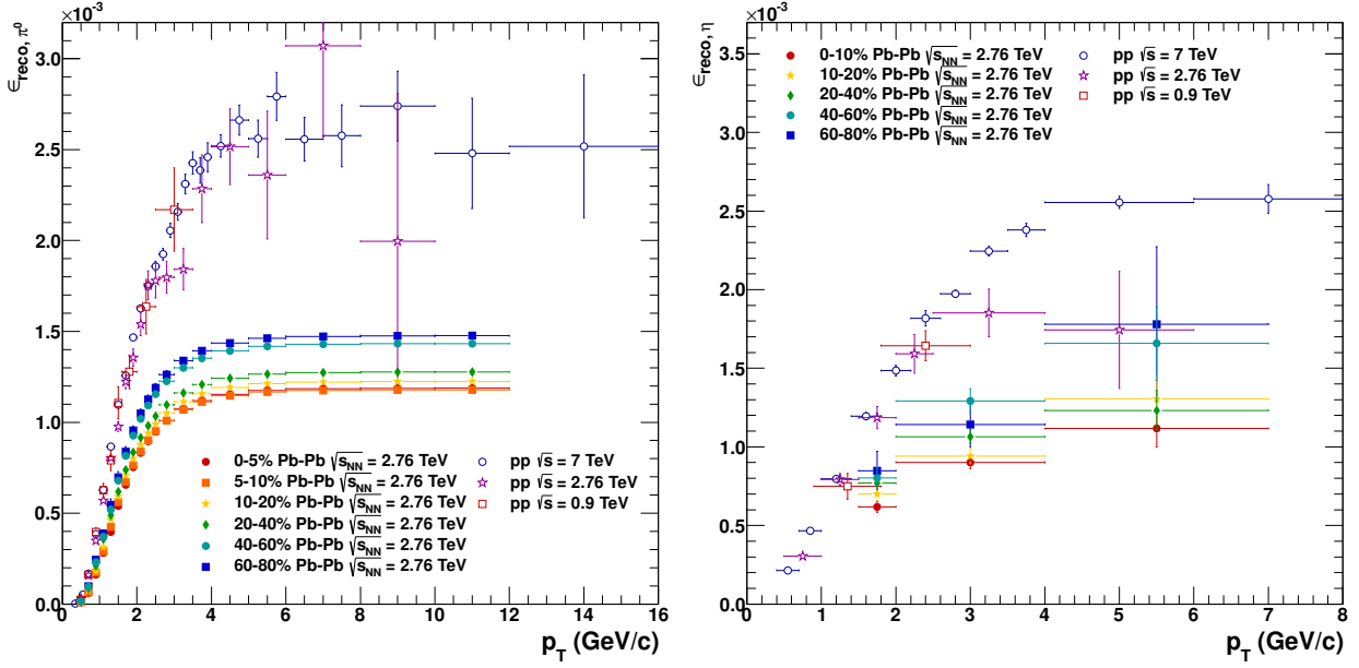
Figure 6.9.: Reconstruction efficiency for \pi^0 (left) and \eta (right) mesons in pp collisions at \sqrt{s} = 0.9, 2.76 and 7 TeV as well as for Pb-Pb collisions at \sqrt{s_{NN}} = 2.76 TeV. For the neutral pion efficiency in Pb-Pb collisions the efficiencies obtained from the Monte Carlo simulations were fitted using Equation 6.6 above 1.2 GeV/c. The original efficiencies can be found in Figure B.1.
