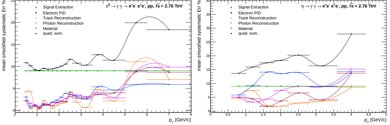
Figure 6.10.: Visualization of the systematic errors for pp collisions at \sqrt{s} = 2.76 TeV. The colored points represent the individual error sources, while the black points represent the final systematic error for the \pi^0 (left) and \eta (right) meson spectra.
