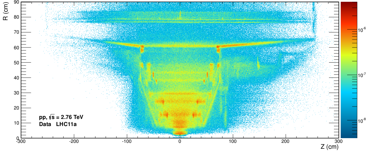
Figure 5.14.: Distribution of the secondary hadronic vertices normalized to the number of events in the ZR -plane for the full pseudo-rapidity range accessible by the SHIM measured in data for pp collisions at \sqrt{s} = 2.76 TeV.
