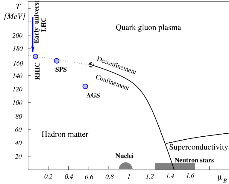
Figure 2.3.: Schematic QCD phase diagram in the T - \mu_B plane, taken from [34]. At low T and \mu_B nuclear matter shows confinement and hadrons determine the number of degrees of freedom. On the other hand, at higher T a phase transition to a deconfined quark-gluon plasma with restored chiral symmetry is predicted by lattice QCD. The phase diagram might exhibit a critical point at about \mu_B \sim 700 MeV. At higher densities more exotic phases can be reached, e.g. states in very dense neutron stars. In this figure the chemical freeze-out conditions for RHIC, SPS and AGS are indicated as well. The LHC will contribute to measurements at low \mu_B , but very high temperatures. The blue arrow illustrates how matter is supposed to have evolved after the Big Bang and before chemical freeze-out at LHC.
