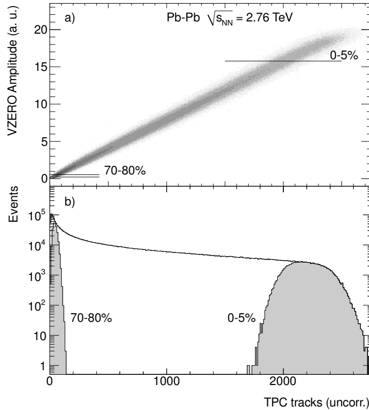
Figure 4.3.: a) Correlation between VZERO amplitude and the Time Projection Chamber (TPC) track multiplicity measured by the ALICE collaboration. b) Minimum bias distribution of the TPC track multiplicity with indicated bins for 70-80% and 0-5% centrality of the Pb-Pb collision at \sqrt{s_{NN}} = 2.76 TeV. [?]
