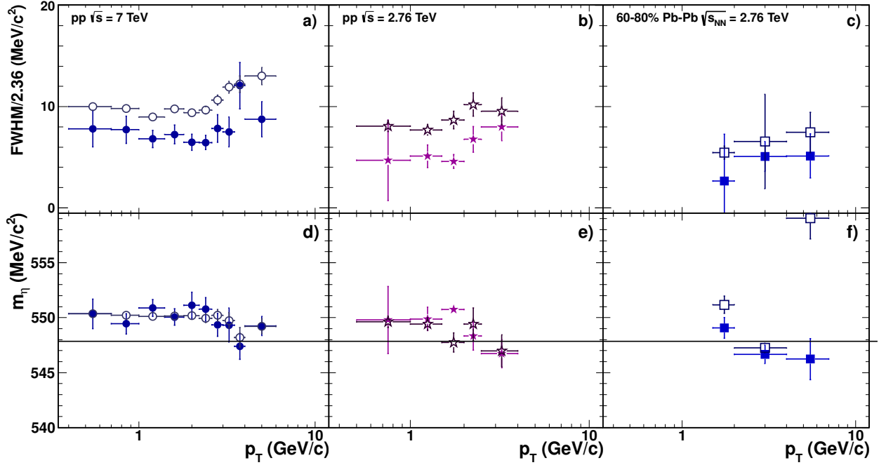
Figure 6.4.: Reconstructed mass resolution (a-c) and mass (d-f) for the \eta meson as function of transverse momentum for pp collisions at \sqrt{s} = 7 TeV (a,d) and 2.76 TeV (b,e) as well as 60-80% Pb-Pb collisions (c,f). The parameters are extracted using the fit described in Equation 6.3. The simulated data is represented by the open symbols, while the real data are shown with filled symbols. Moreover, the nominal mass position according to [130] is indicated by the black line. The resolution is given as the full width at half maximum (FWHM) divided by 2.36 in order to show the corresponding width of the peak in terms of \sigma of a pure Gaussian distribution.
