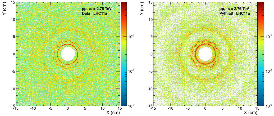
Figure 5.17.: Enlarged view of the distribution of the secondary hadronic vertices in the XY -plane for the \eta < 0.9 measured in data (left) and Pythia 8 (right) for pp collisions at \sqrt{s} = 2.76 TeV. Each distribution is normalized to the total number of events in the corresponding data sample.
