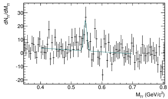
Figure B.20.: Invariant-mass distribution of reconstructed photon pairs M_{\gamma\gamma} around the eta meson mass in p_T slices in 40-60 Pb-Pb collisions at \sqrt{s_{NN}} = 2.76 TeV before (upper plot) and after subtraction (lower plot). The black histograms in the upper plot show the combined signal and background distribution and the blue histograms show the calculated and normalized mixed event background. After the subtraction the invariant mass distributions are fitted with Equation 6.3, which is shown in green in the lower plot.
