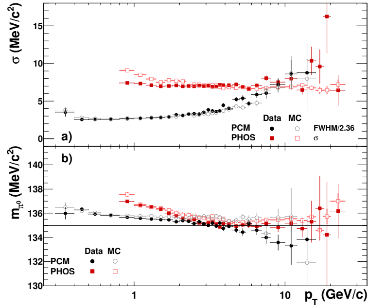
Figure 6.13.: Reconstructed \pi^0 meson invariant mass resolution (a) and peak position (b) as a function of p_T in pp collisions at \sqrt{s} = 7 TeV. Both measurements are compared to the corresponding analysis in Monte Carlo simulations and the nominal \pi^0 mass is indicated by the horizontal black line in (b).
