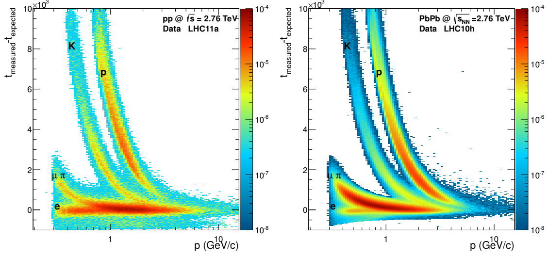
Figure 4.8.: Distribution of the TOF time difference for all electron candidates, after a 5\sigma_e cut in the TPC, versus momentum for pp (left) and Pb–Pb collisions (right).
