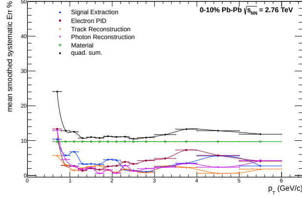
Figure B.26.: Visualization of the systematic errors for the \pi^0 meson for 0-10% Pb–Pb collisions at \sqrt{s_{\text{NN}}} = 2.76 TeV. The colored points represent the individual error sources, while the black points represent the final systematic error of the spectra.
