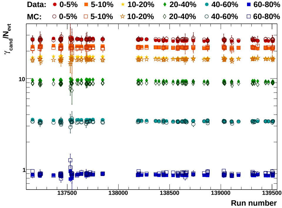
Figure 4.5.: Fraction of photons candidates in Pb-Pb events normalized to the number of events in the corresponding centrality class.
