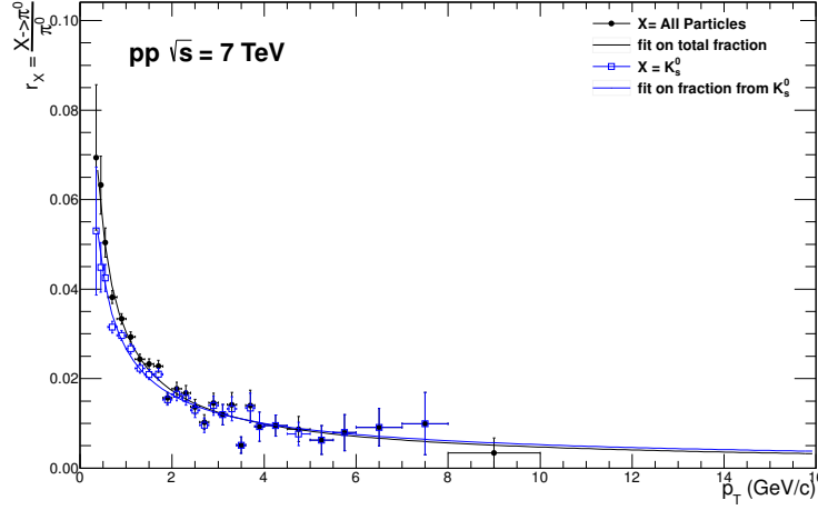
Figure 6.7.: Ratio r_X of reconstructed secondary \pi^0 mesons from K_s^0 mesons (blue squares) or all secondary \pi^0 mesons (black dots) to reconstructed neutral pions. The blue and black line represent the fit to the corresponding fractions with f(x) = \frac{a}{x^b} .
