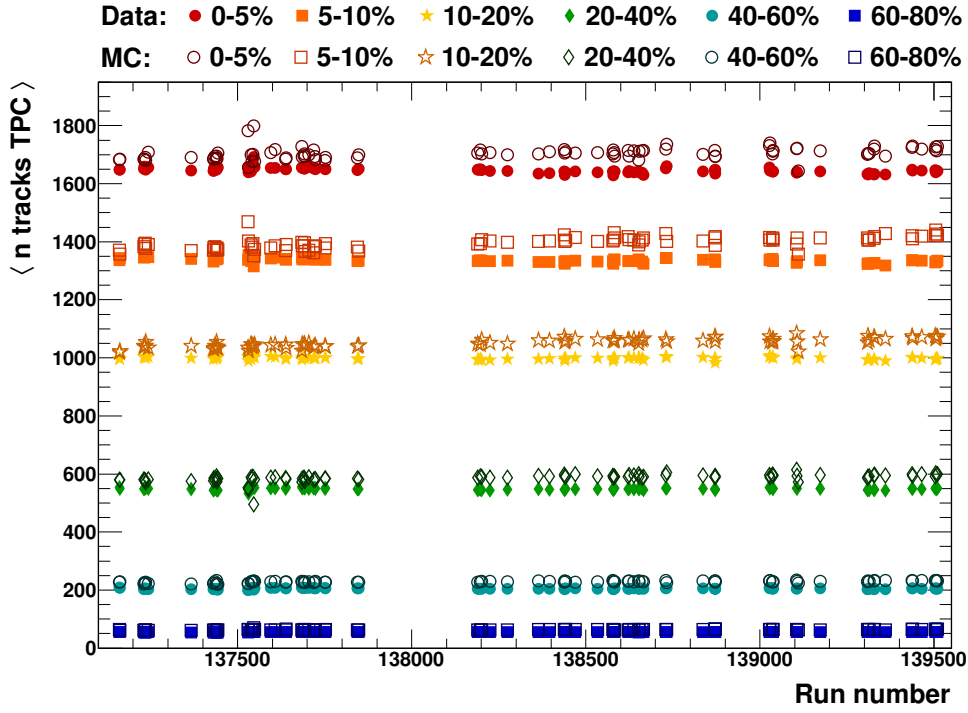
Figure 4.4.: Mean number of primary tracks measured in the TPC ( |\eta| < 0.8 ) compared to minimum bias Monte Carlo simulations (LHC11a10a_bis) for the different centrality classes.
