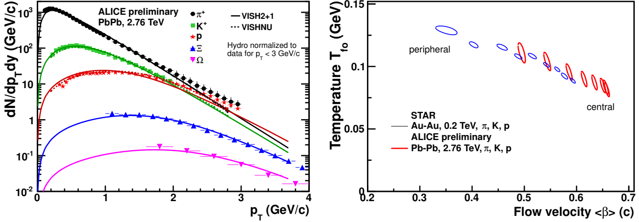
Figure 2.5.: Left: Comparison of the preliminary results on identified transverse-momentum spectra for central Pb–Pb collision at \sqrt{s_{NN}} = 2.76 TeV measured by the ALICE collaboration and scaled results from a boost-invariant hydrodynamic model with (VISHNU, dashed lines) and without (VISH2+1, full lines) rescattering in the hadronic phase. Right: Results from a simultaneous “blastwave”-fit to the identified spectra ( \pi , K , p ) at LHC (Pb–Pb) and RHIC (Au–Au) for different centralities.
