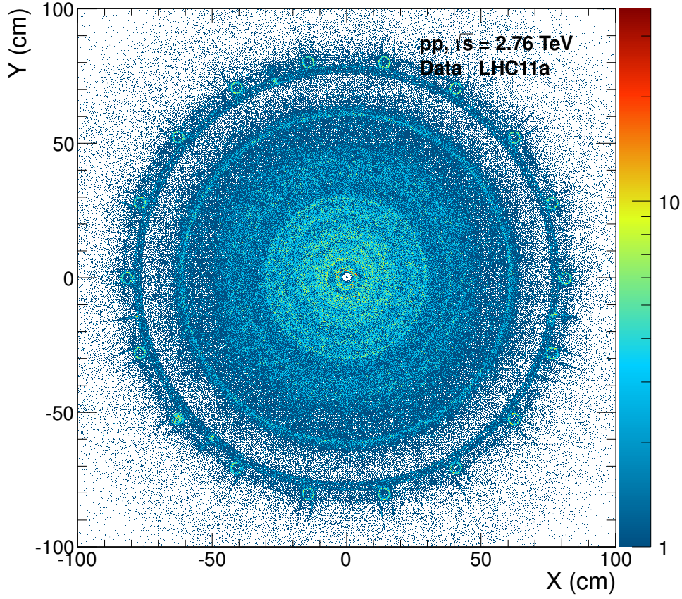
Figure 5.16.: Distribution of the secondary hadronic vertices in the XY -plane for the \eta < 0.9 measured in data for pp collisions at \sqrt{s} = 2.76 TeV.
