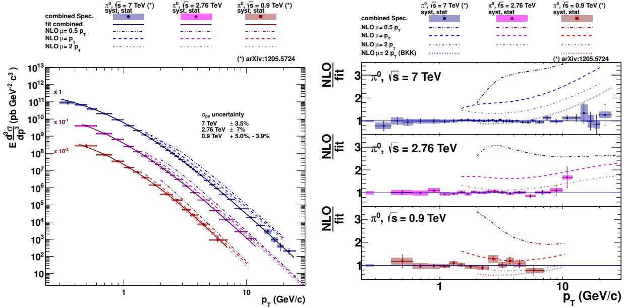
Figure 6.15.: Differential invariant cross section of the \pi^0 meson production (left) in pp at \sqrt{s} = 0.9 (red squares), 2.76 TeV (purple stars) and 7 TeV (blue dots). The shaded boxes indicate the systematic error, while the error bars show the statistical error. The solid lines represent the Tsallis fit the the combined spectrum. Ratio of the data and next to leading order calculation using CTEQ6M5 PDF and the DSS (BKK) fragmentation functions for three scales \mu = 0.5p_T, p_T and 2p_T (right).
