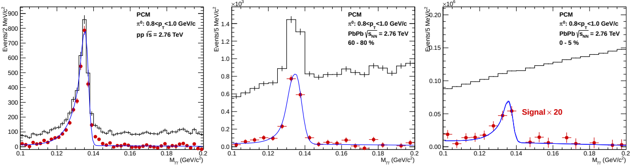
Figure 6.1.: Invariant-mass distribution of reconstructed photon pairs M_{\gamma\gamma} around the neutral pion mass ( 0.135 \text{ GeV}/c^2 ) in selected p_T slices in pp collisions at \sqrt{s} = 2.76 \text{ TeV} (left) and in peripheral (middle) and central (right) Pb–Pb collisions at \sqrt{s_{NN}} = 2.76 \text{ TeV} . The black histogram and the red bullets show the data before and after background subtraction, respectively. The blue curve is a fit to the invariant mass spectrum after background subtraction.
