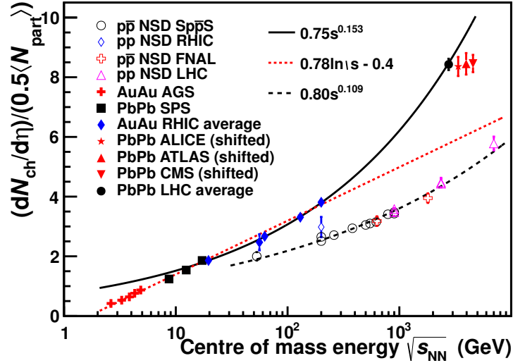
Figure 2.4.: Charged particle pseudo-rapidity density per participant pair as a function of \sqrt{s_{NN}} for central A+A and pp collisions [37].
