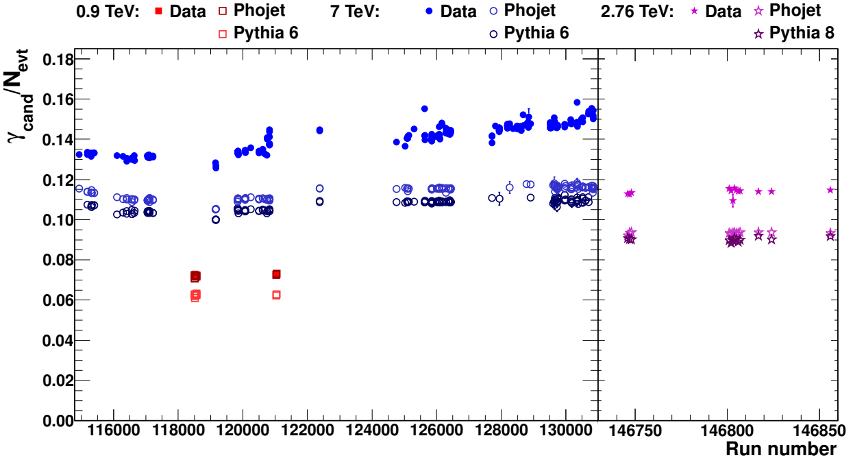
Figure 4.2.: Fraction of photon candidates in pp events normalized to the number of events, which fulfill our event selection criteria (full symbols). The points with open symbols represent the same quantity for the corresponding Monte Carlo simulations.
