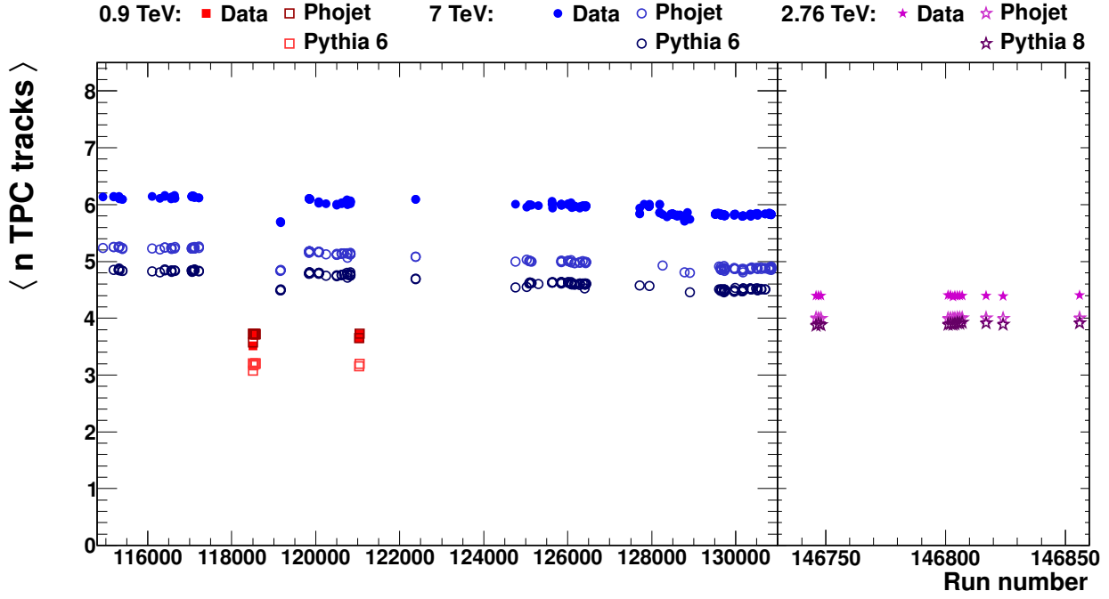
Figure 4.1.: Mean number of primary tracks reaching the TPC versus run number for the different pp data samples and the corresponding Monte Carlo simulations.
