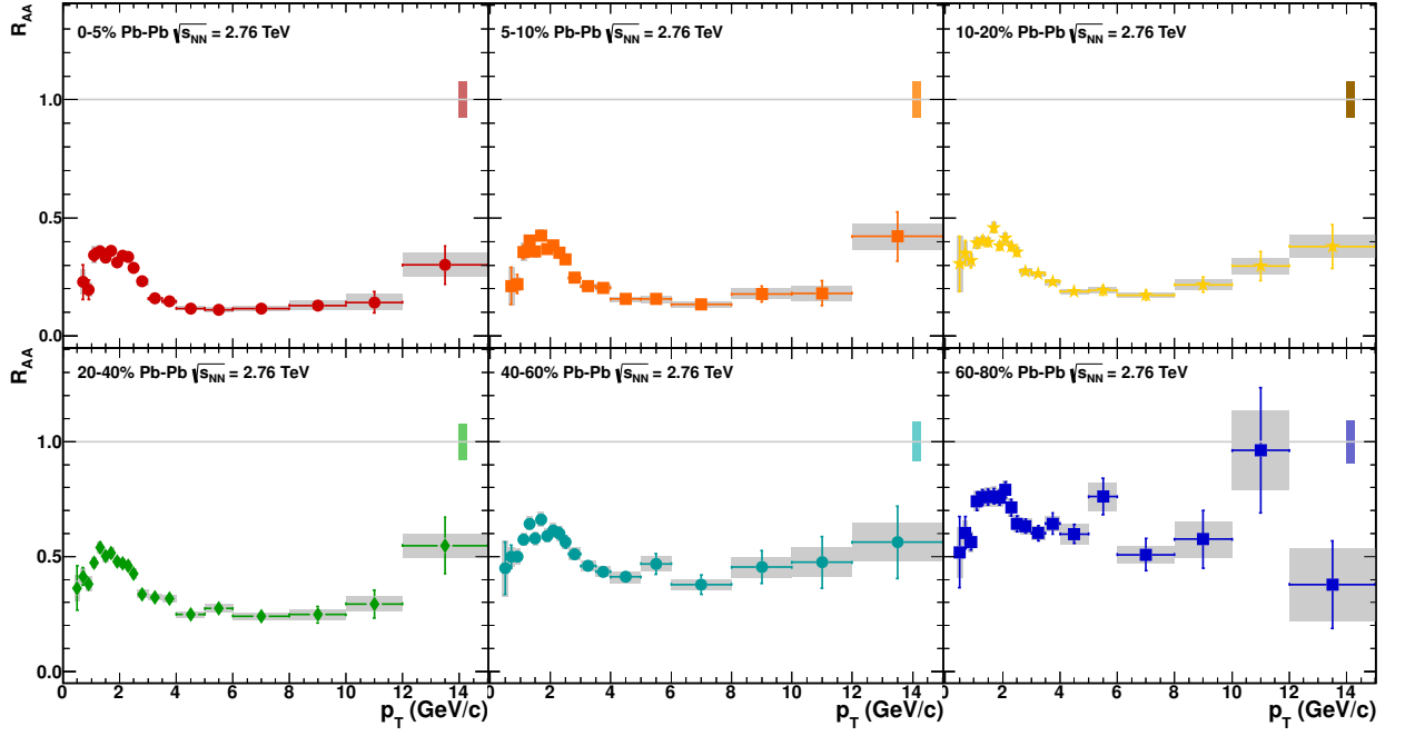
Figure 6.22.: Combined nuclear modification factor, R_{AA} , from individual measurements using PHOS and PCM in Pb–Pb collisions at \sqrt{s_{NN}} = 2.76 TeV for six centrality classes, 0-5 %, 5-10 %, 10-20%, 20-40%, 40-60% and 60-80%. Vertical lines represent the statistical error while the boxes reflect the systematic uncertainty. The boxes around unity reflect the uncertainties of the average nuclear overlap function ( T_{AA} ) and the normalization uncertainty in the pp added in quadrature.
