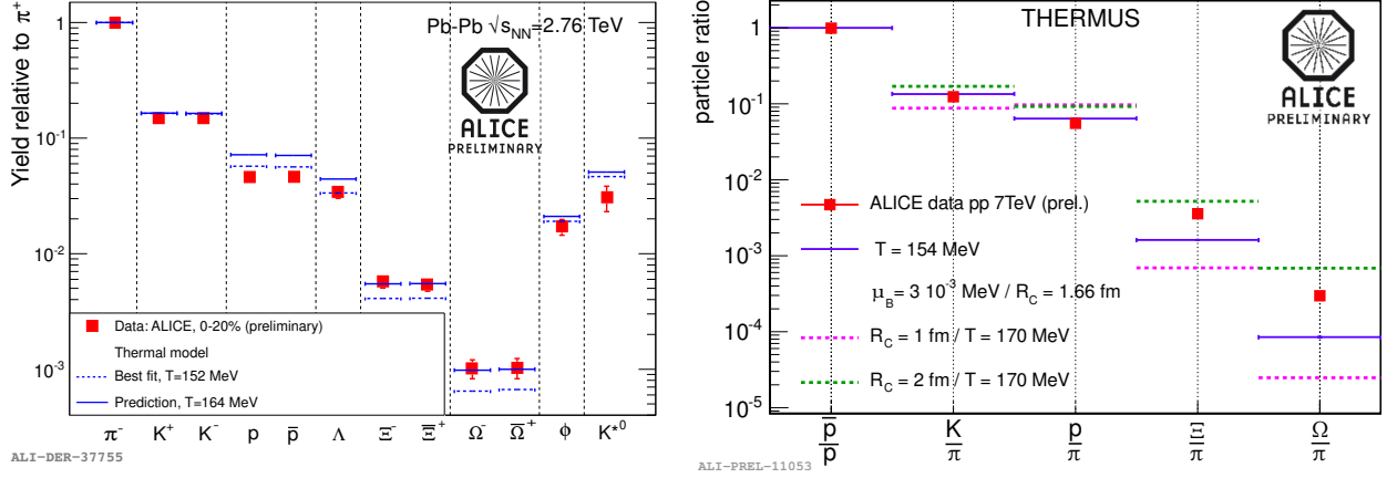
Figure 2.6.: Left: Particle ratios in 0-20% central Pb-Pb collisions at \sqrt{s_{NN}} = 2.76 TeV measured by ALICE together with a thermal model prediction [48] (solid line) and the fit to the data (dashed line). Right: Particle Ratios in pp collisions at \sqrt{s} = 7 TeV together with THERMUS model predictions (dashed lines) for different R_c [60] and a thermal model fit to the data (solid line).
