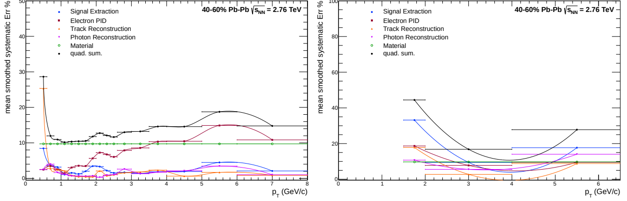
Figure B.35.: Visualization of the systematic errors for the \pi^0 (left) and \eta meson (right) for 40-60% Pb-Pb collisions at \sqrt{s_{NN}} = 2.76 TeV. The colored points represent the individual error sources, while the black points represent the final systematic error of the spectra.
