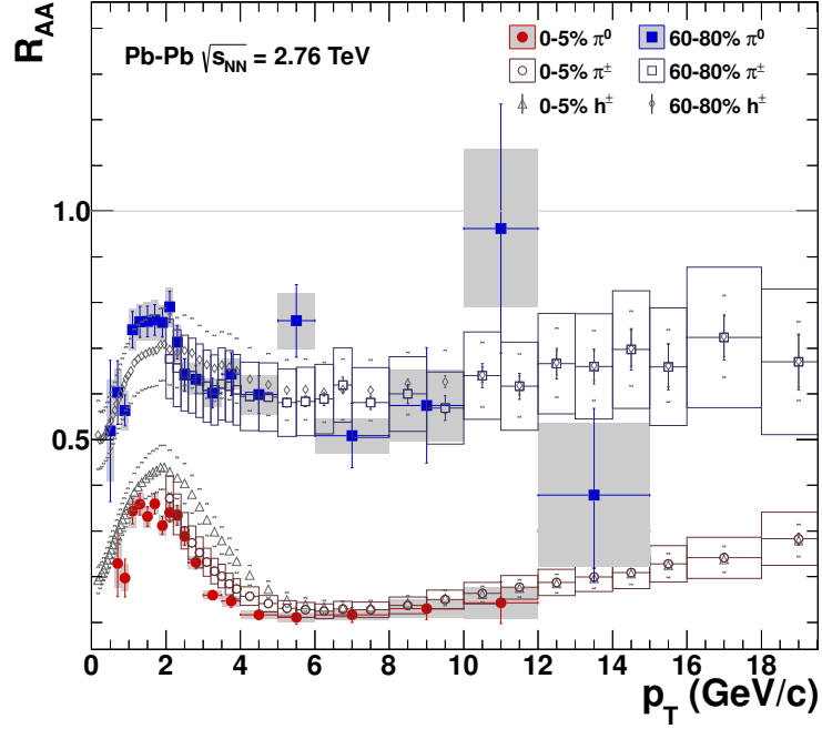
Figure 6.24.: Comparison of the neutral pion R_{AA} in most central (0-5%) and peripheral (60-80%) Pb–Pb collisions to the measurement for unidentified charged hadrons [95] and for charged pions [186] in the same centrality classes.
