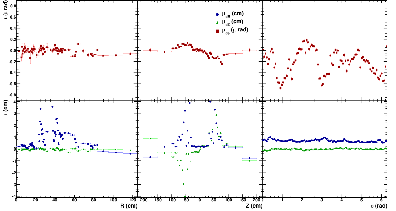
Figure 5.7.: Mean shift of the reconstructed \varphi (top), R and Z (bottom) coordinates versus R (left), Z (middle) and \varphi (right) for 0.9 < |\eta| < 1.4 . The shifts are calculated fitting a Gaussian distribution to the dX = X_{\text{rec}} - X_{\text{MC}} ( X = R, Z, \Phi ), identifying the \mu of the Gaussian distribution with the mean shift in the corresponding coordinate.
