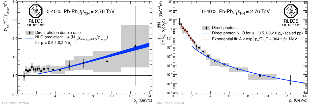
Figure 2.12.: The left plot shows the direct-photon double ratio and the right plot the direct-photon invariant yield in Pb-Pb collisions at \sqrt{s_{NN}} = 2.76 TeV for 0-40% centrality with NLO pQCD predictions, the latter contains an additional exponential fit ( p_T < 2 GeV/c) to the data [124].
