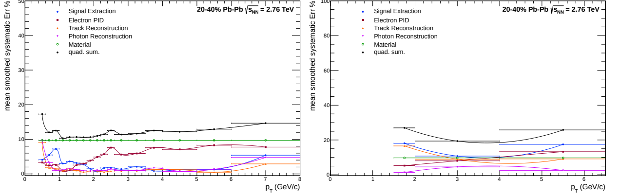
Figure B.32.: Visualization of the systematic errors for the \pi^0 (left) and \eta meson (right) for 20-40% Pb–Pb collisions at \sqrt{s_{NN}} = 2.76 TeV. The colored points represent the individual error sources, while the black points represent the final systematic error of the spectra.
