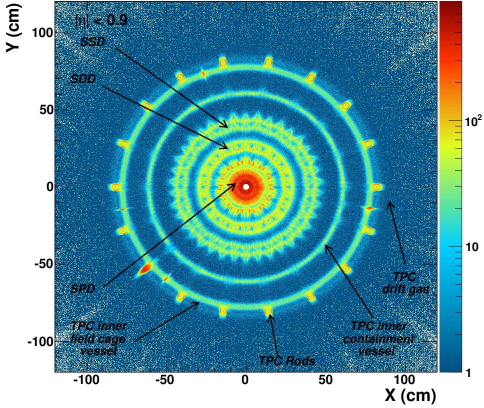
Figure 5.3.: Distribution of the conversion points in the XY -plane for the fiducial acceptance |\eta| < 0.9 measured for pp collisions at \sqrt{s} = 7 TeV. The detector geometry of the inner detectors is clearly visible as well as their \varphi distribution.
