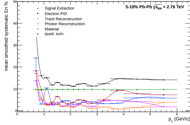
Figure B.24.: Visualization of the systematic errors for the \pi^0 meson for 5-10% Pb-Pb collisions at \sqrt{s_{NN}} = 2.76 TeV. The colored points represent the individual error sources, while the black points represent the final systematic error of the spectra.
