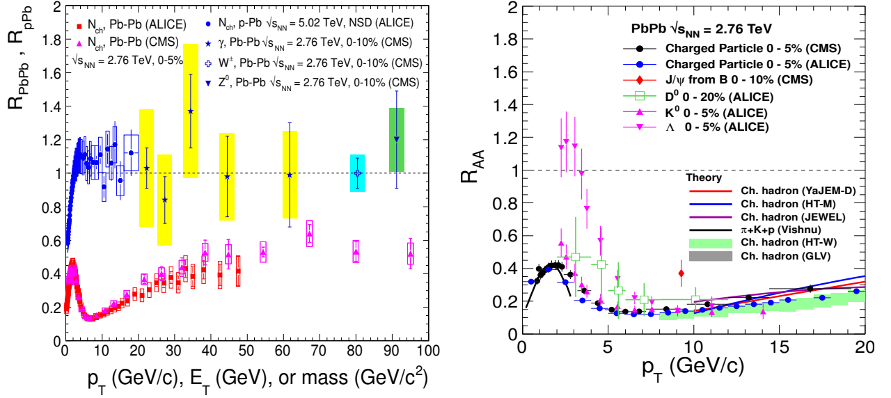
Figure 2.10.: Left: Comparison of the charged hadron nuclear modification factor R_{AA} ( R_{pA} ) for Pb–Pb collisions at \sqrt{s_{NN}} = 2.76 TeV [95,96] and p–Pb collisions at \sqrt{s_{NN}} = 5.02 TeV [97]. In addition the nuclear modification factors for isolated photons [98,99], the Z^0 [100] and the W^\pm [101,102] are shown. Plot taken from [103]. Right: Nuclear modification factor R_{AA} as a function of p_T for a variety of particle species together with theoretical predictions [104–107]. The error bars of the experimental points correspond to the total error (systematic and statistical errors added in quadrature). a) Low momentum ( p_T < 20 GeV) R_{AA} for unidentified charged particles (blue and black points), J/\Psi from B (red points), D^0 -mesons (green rectangles) and strange particles (blue triangles). Plot taken from [37].
