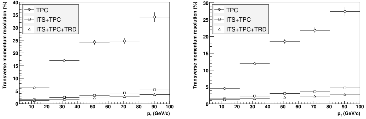
Figure 3.10.: Transverse momentum resolution for different combinations of tracking detectors for central Pb–Pb collisions at dN_{ch}/d\eta = 6000 and pp collision (right) [159].
