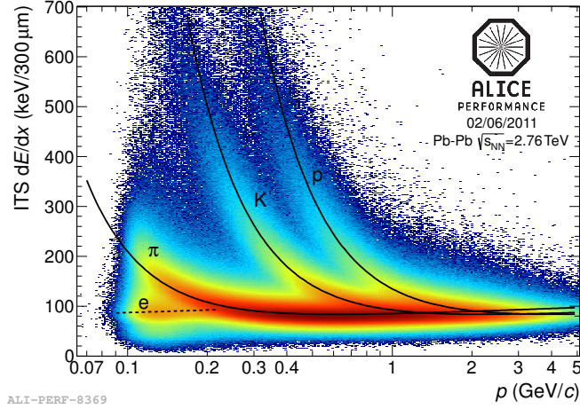
Figure 3.4.: Performance plot (ALI-PERF-8369) of the energy loss measurement ( dE/dx ) performed in the outer layers of the ALICE ITS versus momentum measured by the combined tracking of ITS and TPC. The separation of the different particles species (electrons, pions, kaons, protons) can be clearly seen, the black line indicates the theoretical Bethe-Bloch-curves Equation 3.1.
