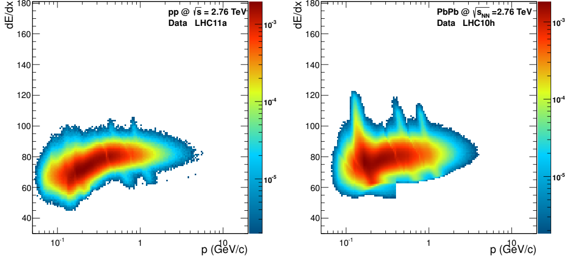
Figure 4.7.: dE/dx distribution for positrons for pp (left) and central (0-5%) Pb–Pb collisions (right) after all electron and photon selection cuts.
