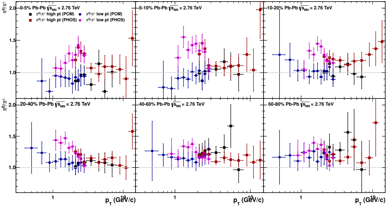
Figure 6.20.: Comparison of the individual measurements of the neutral pion to the low momentum charged pions measured via a combined ITS, TPC and TOF analysis [57] and the high momentum charged pions measured via the particle fractions in the relativistic rise of the dE/dx of the TPC [186]. The error bars reflect the quadratically summed systematic and statistical uncertainties of the measurements. The measurements of the charged pions have been averaged between the two charges to be able to directly compare the \pi^0 and \pi^\pm measurements.
