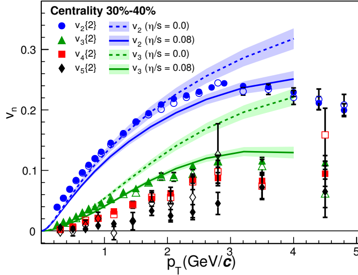
Figure 2.7.: \nu_2 , \nu_3 , \nu_4 , \nu_5 as a function of transverse momentum for 30-40% central Pb–Pb events at LHC measured by ALICE compared to hydrodynamical calculations with different shear viscosities ( \eta/s ) [68]. The full and open symbols are for \Delta\eta > 0.2 and \Delta\eta > 1.0 , respectively.
