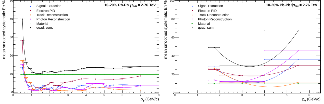
Figure B.29.: Visualization of the systematic errors for the \pi^0 (left) and \eta meson (right) for 10-20% Pb-Pb collisions at \sqrt{s_{NN}} = 2.76 TeV. The colored points represent the individual error sources, while the black points represent the final systematic error of the spectra.
