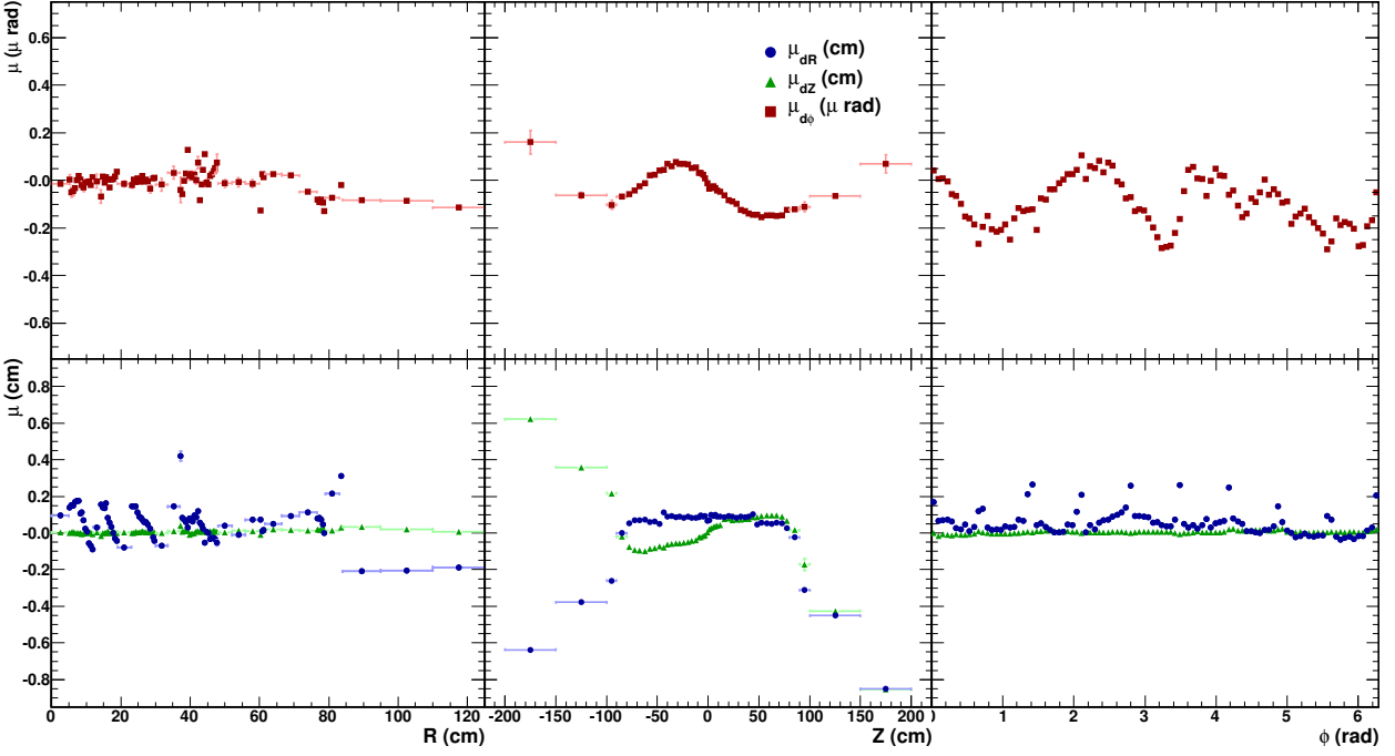
Figure 5.5.: Mean shift of the reconstructed \phi (top), R and Z (bottom) coordinates versus R (left), Z (middle) and \phi (right) for |\eta| < 0.9 . The shifts are calculated fitting a Gaussian distribution to the dX = X_{\text{rec}} - X_{\text{MC}} ( X = R, Z, \Phi ), identifying the \mu of the Gaussian distribution with the mean shift in the corresponding coordinate.
