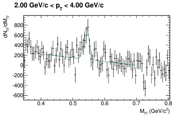
Figure B.16.: Invariant-mass distribution of reconstructed photon pairs M_{\gamma\gamma} around the eta meson mass in p_T slices in 10-20 Pb–Pb collisions at \sqrt{s_{NN}} = 2.76 TeV before (upper plot) and after subtraction (lower plot). The black histograms in the upper plot show the combined signal and background distribution and the blue histograms show the calculated and normalized mixed event background. After the subtraction the invariant mass distributions are fitted with Equation 6.3, which is shown in green in the lower plot.
