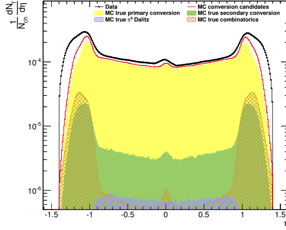
Figure 5.11.: \eta distribution of the reconstructed conversion points (black) for |\eta| < 1.4 compared to Monte Carlo simulations done with Pythia 6 tune Perugia 0 (red). The distribution for true primary (secondary) converted photons is shown in yellow (green), while the physics contamination from true \pi^0 and \eta Dalitz decays is shown in blue dashed. The true random combinatorial background is shown in brown, while the hadronic background (contamination from e.g. K_s^0 , \Lambda , \bar{\Lambda} ) is shown in black.
