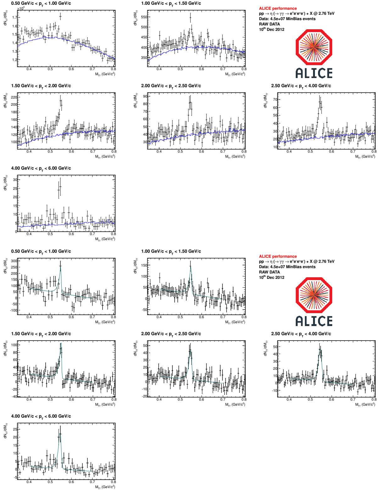
Figure B.2.: Invariant-mass distribution of reconstructed photon pairs M_{\gamma\gamma} around the eta meson mass in p_T slices in pp collisions at \sqrt{s} = 2.76 TeV before (upper plot) and after subtraction (lower plot). The black histograms in the upper plot show the combined signal and background distribution and the blue histograms show the calculated and normalized mixed event background. After the subtraction the invariant mass distributions are fitted with Equation 6.3, which is shown in green in the lower plot.
