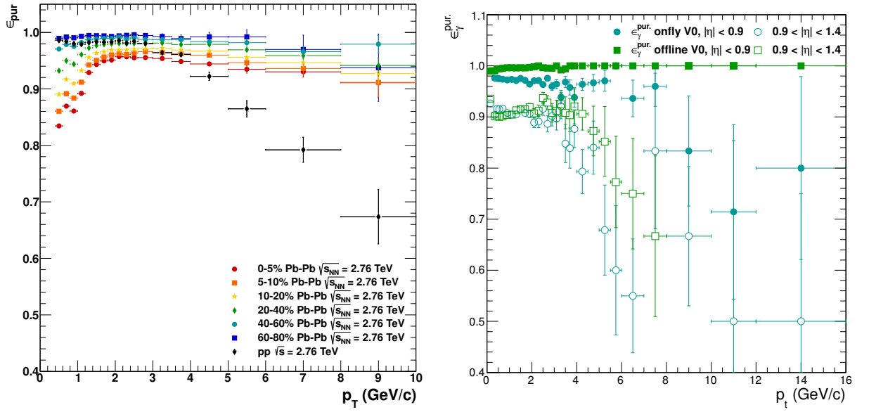
Figure 4.12.: Purity of the photon candidates surviving all cuts for the meson analysis for pp and Pb-Pb collisions (left) and for the material cuts for pp collisions (right). The right plot shows the purity for the two different V0-finders, On-The-Fly (blue) and Offline (green), in addition the two different \eta regions are shown, |\eta| < 0.9 (full symbols) and 0.9 < |\eta| < 1.4 (open symbols).
