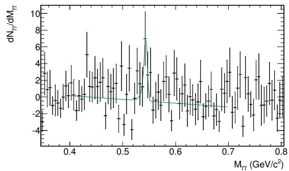
Figure B.22.: Invariant-mass distribution of reconstructed photon pairs M_{\gamma\gamma} around the eta meson mass in p_T slices in 60-80 Pb–Pb collisions at \sqrt{s_{NN}} = 2.76 TeV before (upper plot) and after subtraction (lower plot). The black histograms in the upper plot show the combined signal and background distribution and the blue histograms show the calculated and normalized mixed event background. After the subtraction the invariant mass distributions are fitted with Equation 6.3, which is shown in green in the lower plot.
