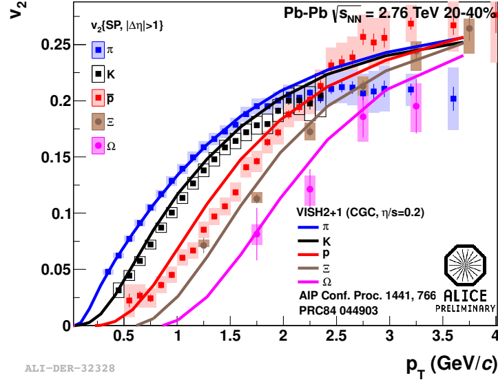
Figure 2.8.: v_2 as a function of transverse momentum for low-momentum \pi , K , \bar{p} , \Xi and \Omega together with the corresponding hydrodynamical calculation [70–72].
