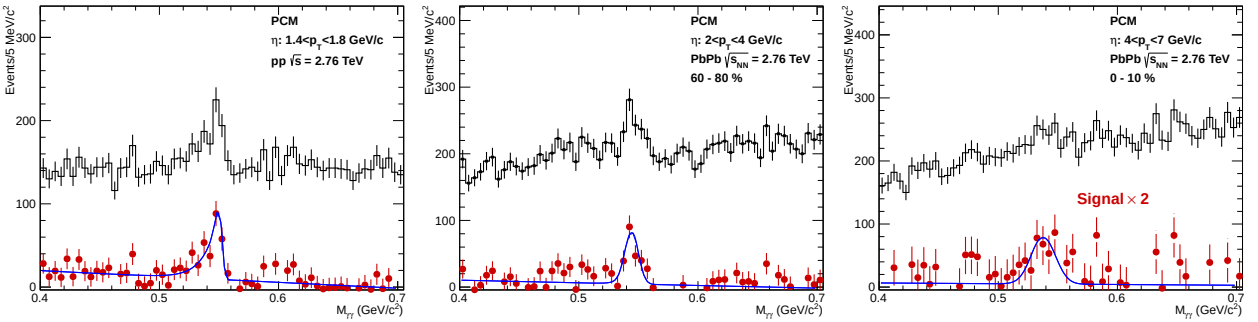
Figure 6.2.: Invariant-mass distribution of reconstructed photon pairs M_{\gamma\gamma} around the mass of the \eta meson ( 0.548 \text{ GeV}/c^2 ) in selected p_T slices in pp collisions at \sqrt{s} = 2.76 \text{ TeV} (left) and in peripheral (middle) and central (right) Pb–Pb collisions at \sqrt{s_{NN}} = 2.76 \text{ TeV} . The black histogram and the red bullets show the data before and after background subtraction, respectively. The blue curve is a fit to the invariant mass spectrum after background subtraction.
