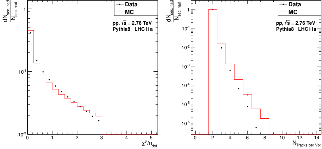
Figure 5.13.: Comparison of the distribution of the \chi^2/N_{\text{dof}} for the secondary vertices obtained from the extrapolation of the tracks to the secondary vertex (left) and the number of tracks per secondary vertex (right) for Monte Carlo simulation (Pythia 8) and the data in pp collisions at \sqrt{s} = 2.76 TeV. Each distribution is normalized to its integral to enable the comparison regardless of the statistics in each data sample.
