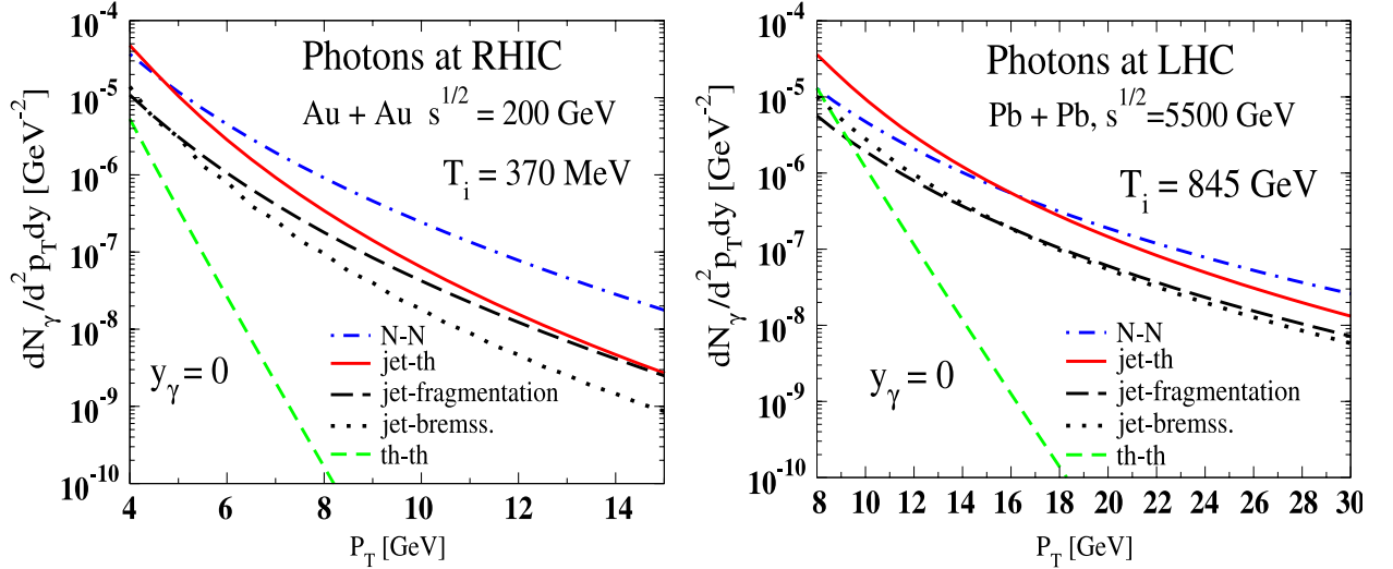
Figure 2.11.: Sources of high p_T photons at midrapidity in central Au-Au collisions at RHIC (left) and for Pb-Pb collisions at LHC (right). The different contributions are (red solid line) Jet-photon conversions in the plasma, (black dotted line) bremsstrahlung from jets in the plasma; (green dashed line) thermal induced production of photons, (black dashed line) fragmentation of jets outside the plasma, (blue dot-dashed line) direct contribution from primordial hard scattering [120].
