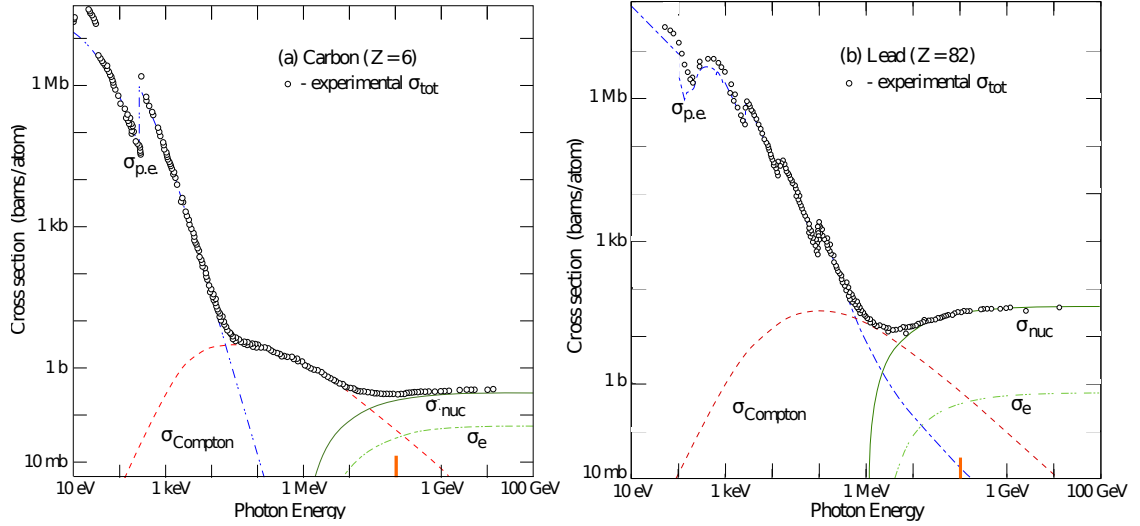
Figure 2.13.: Photon cross section as a function of energy in a) carbon and b) lead. The different cross sections shown are:
