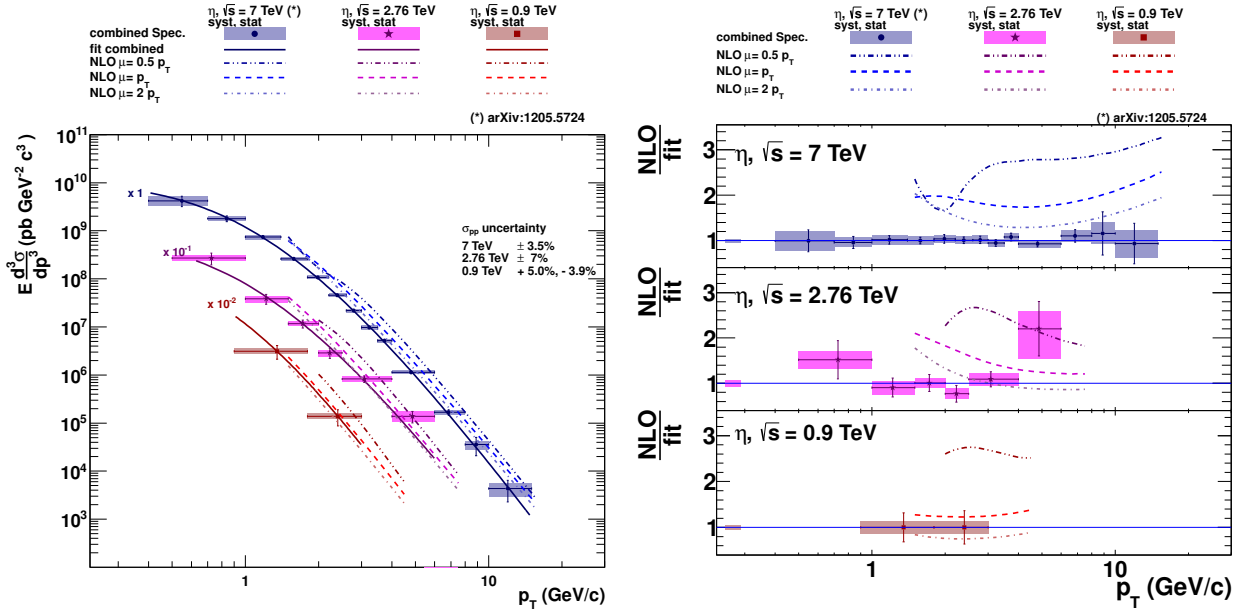
Figure 6.16.: Differential invariant cross section of the \eta meson production (left) in pp at \sqrt{s} = 0.9 (red squares), 2.76 TeV (purple stars) and 7 TeV (blue dots). The shaded boxes indicate the systematic error, while the error bars show the statistical error. The solid lines represent the Tsallis fit the the combined spectrum. Ratio of the data and next to leading order calculation using CTEQ6M5 PDF and the AES fragmentation functions for three scales \mu = 0.5 p_T, p_T and 2p_T (right).
