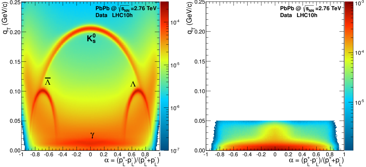
Figure 4.11.: Armenteros-Podolanski-Plot of all V0 candidates after the basic track and V0 cuts, mentioned in Section 4.2.1, for the Pb–Pb minimum bias events (left). On the right the remaining photon candidates after all cuts are shown in the same representation for the 0-5% central Pb–Pb collisions.
