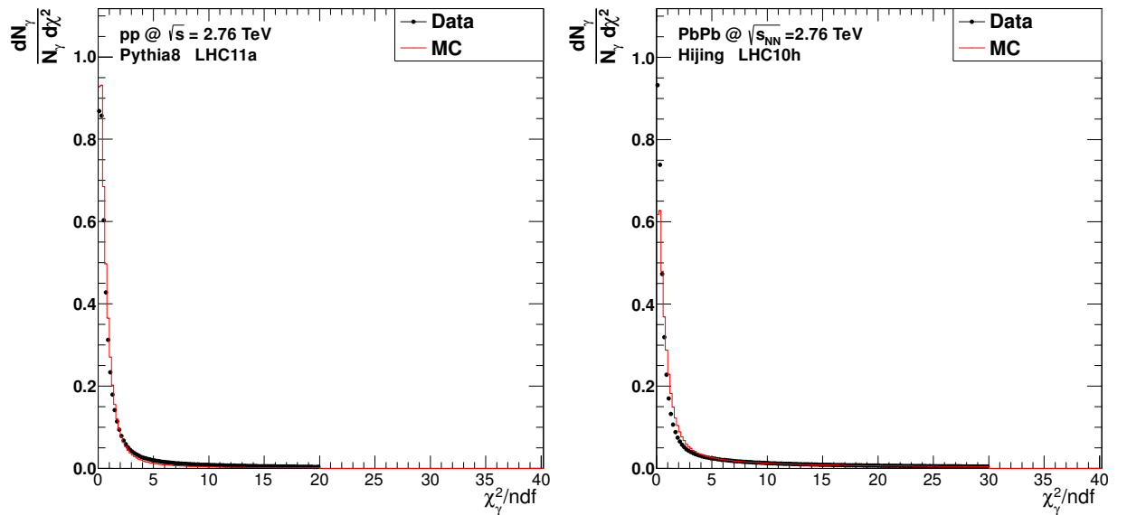
Figure 4.10.: Comparison of the distribution of the \chi^2/\text{ndf} of the photon candidates in data and Monte Carlo for pp (left) and central Pb–Pb collisions (right).
