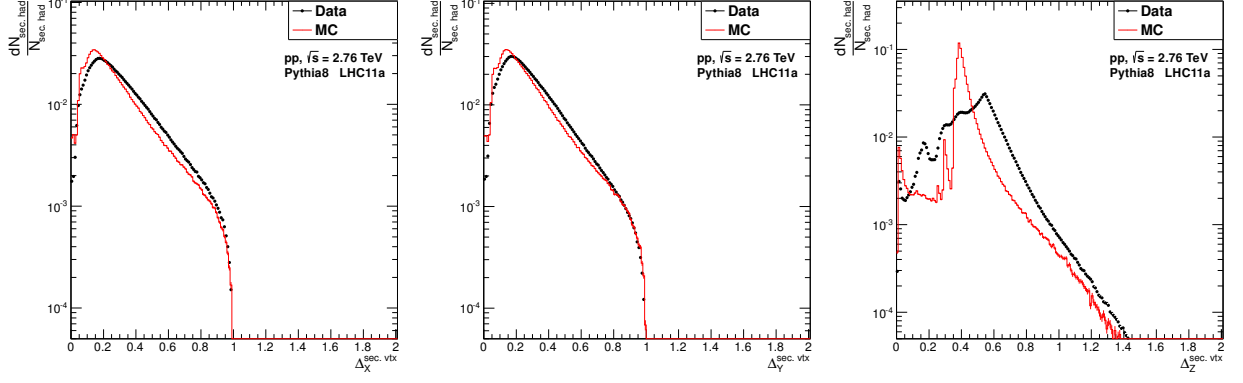
Figure 5.12.: Error estimates on the coordinates of the secondary hadronic vertices in X_{\text{sec}} (left), Y_{\text{sec}} (middle) and Z_{\text{sec}} (right) for data (black dots) and the Pythia 8 Monte Carlo simulation (red histogram) in pp collisions at \sqrt{s} = 2.76 TeV. Each distribution is normalized to its integral to enable the comparison for samples with different statistics.
