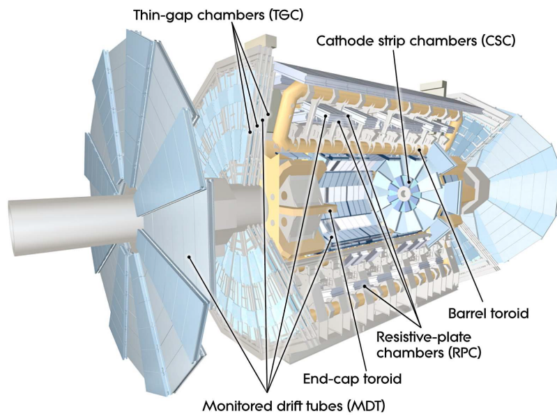
Figure 2.10: ATLAS muon system [19].
