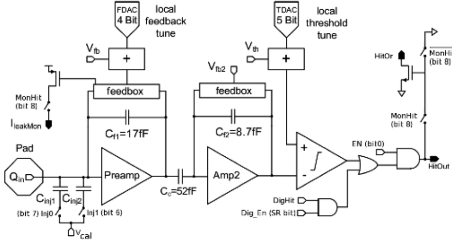
Figure 3.7: Analog Pixel schematic diagram of FE-I4 [27].
