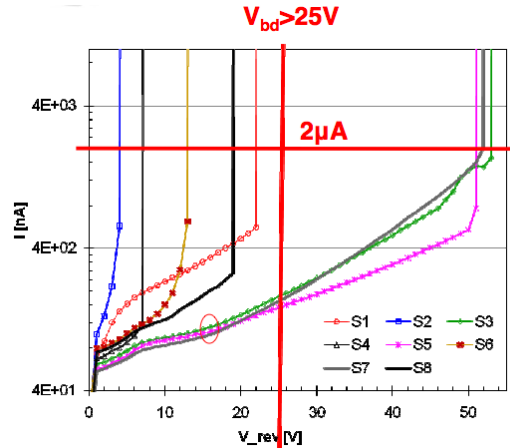
Figure 4.18: Example of IV measurement on the temporary metal directly on the wafer. Sensors 3, 5, 7 satisfy the IBL 3D specifications, while sensors 1, 2, 4, 6, 8 do not satisfy the specifications. Measurement done in Trento by the FBK [48].
