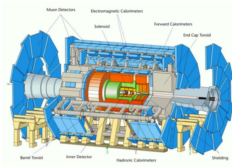
Figure 2.4: Schematic view of the ATLAS detector. The innermost part is the tracker, and an eletromagnetic and a hadron calorimeters follow. The outermost part is made by muon chambers embedded in a large Toroidal magnet.
