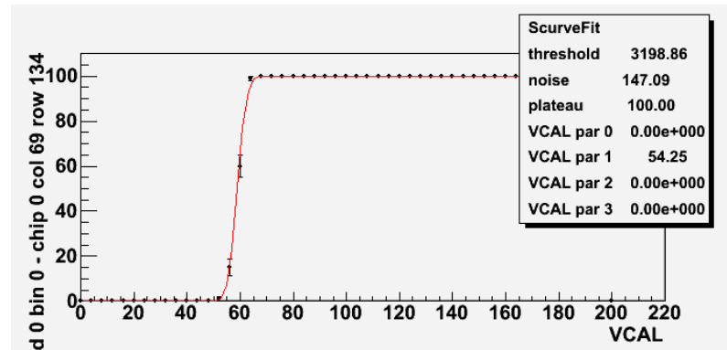
Figure 5.12: Example of a S-curve fit for one pixel: column 69, row 134 at targets values of 3200 electrons, eight TOT for deposited charge of 20000 electrons before irradiation. The S-curve fit belongs to the tuning shown in Figure 5.14.
