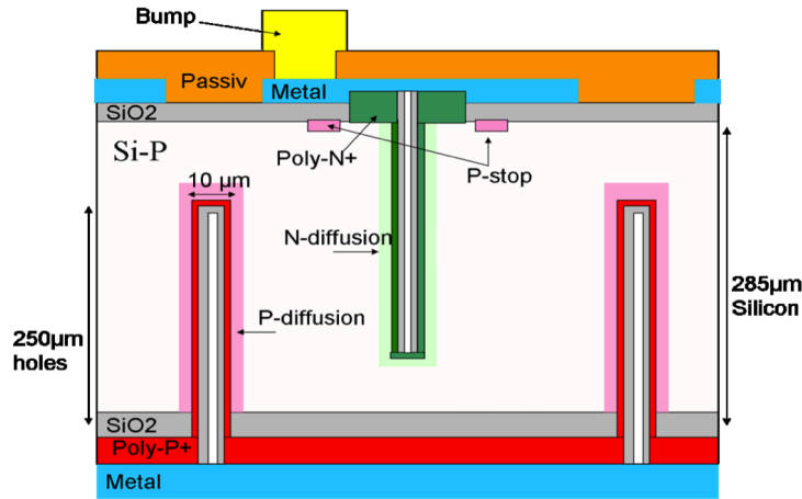
Figure 4.14: Layout proposed for the double sided 3D-CNM detectors [74].
