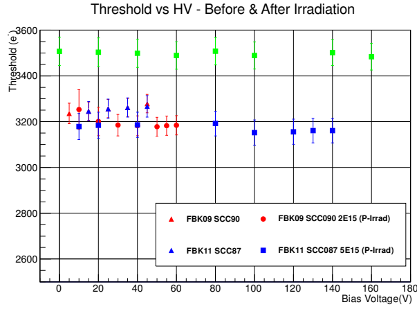
Figure 5.17: Threshold as a function of the applied power supply: comparison before and after proton irradiation for FBK09 ( 2 \times 10^{15} \text{ n}_{eq}/\text{cm}^2 ) and FKB11 ( 5 \times 10^{15} \text{ n}_{eq}/\text{cm}^2 ).
