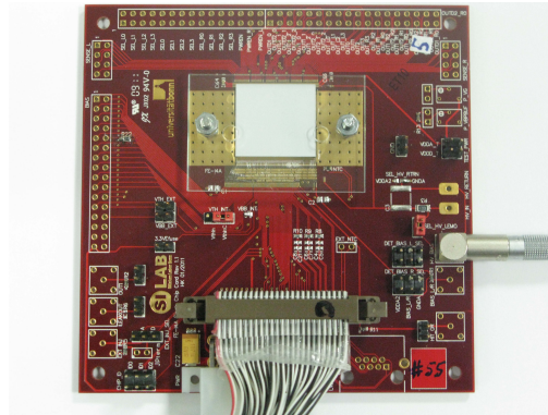
Figure 5.2: SCC board with the FE-I4 and a 3D-FBK sensor wire bonded on it.
