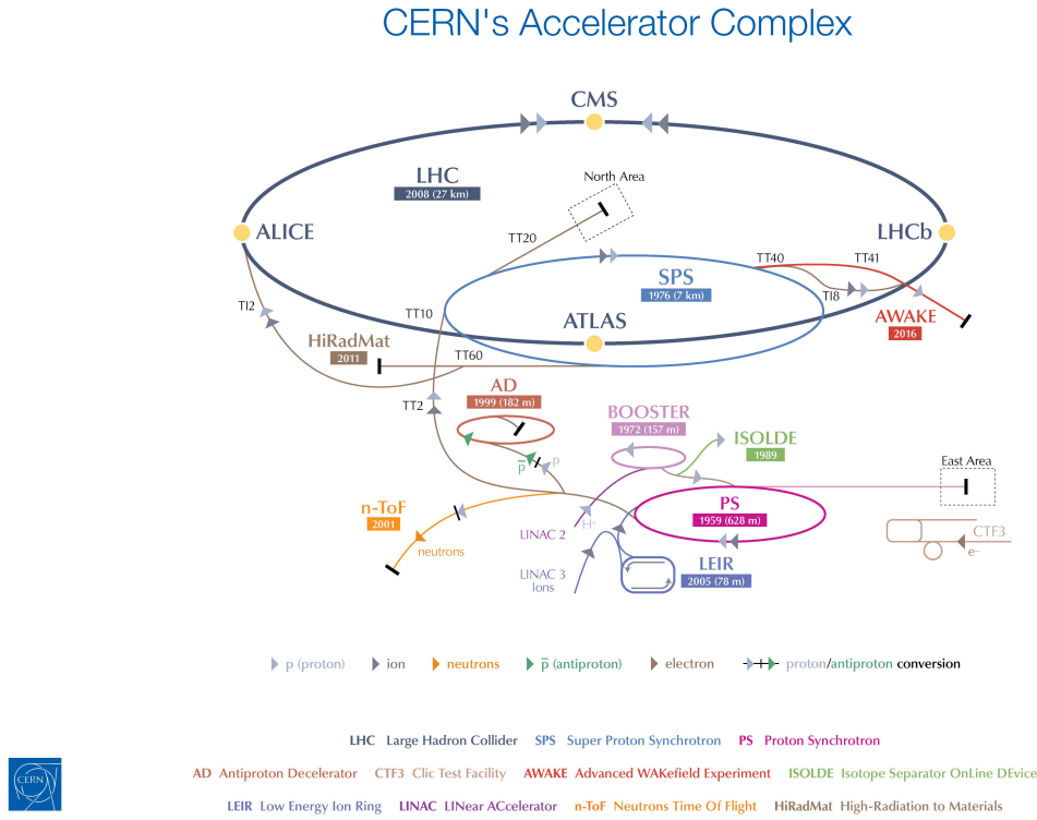
Figure 4.1: A schematic of the CERN LHC accelerator complex [9].
