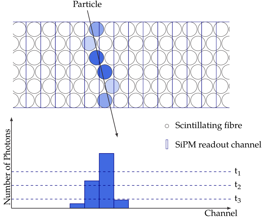
Fig. 4.2.: SciFi clustering procedure. A crossing particle typically creates photons in more than one channel. The signal gets discriminated by three different thresholds ( t_1 , t_2 , t_3 ). Channels which exceed the seed threshold t_2 are selected. If the sum of neighbouring channels above the neighbour threshold t_3 is higher than the sum threshold t_1 these channels are forming a cluster. The actual hit position is calculated as the weighted mean of all channels inside this cluster.
