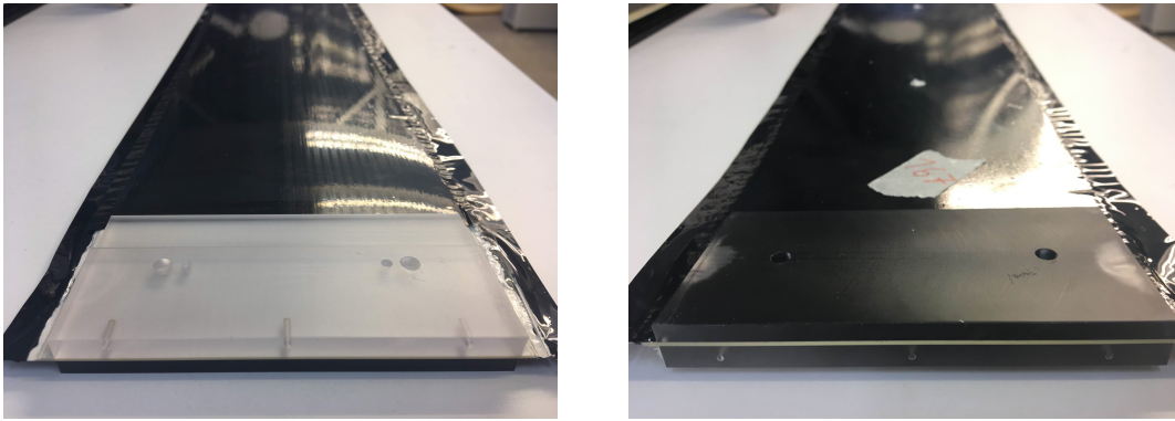
Fig. 4.9.: Laminated fibre mat with end pieces from both sides.
