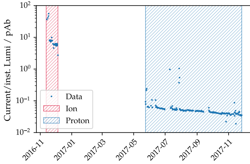
Fig. 6.34.: Normalized signal at the SiPM as a function of time. A clear decrease is visible. Times where ion runs were taking place are hatched red, while proton runs are hatched blue.
