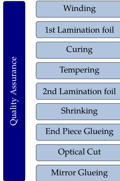
Fig. 5.2.: Necessary steps to produce a fibre mat. These steps are done in the Winding Centres, before the fibre mats get shipped to the Module Centres, where the side cuts are performed before assembling the detector module.
