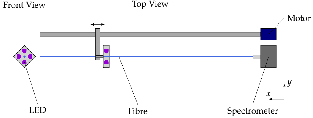
Fig. 6.7.: Setup to measure the attenuation of a single scintillating fibre: the LED housing contains 4 LEDs surrounding the fibre and exciting it. With the help of the x -axis, the position along the fibre axis can be changed.
