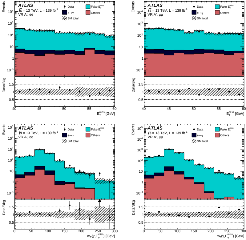
Figure 9.22: Comparison between data and total expected background of the E_T^{\text{miss}} (top) and m_T(E_T^{\text{miss}}, \gamma) (bottom) in the VR. The results are shown in ee (left) and \mu\mu (right) channel.
