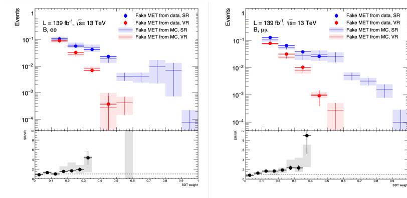
Figure B.13: BDT score distributions in the ee (left) and \mu\mu (right) channel, normalised to unit area, of the fake E_T^{\text{miss}} background in 30 < E_T^{\text{miss}} < 40 GeV (red) and in 40 < E_T^{\text{miss}} < 60 GeV (blue) from data with other background subtracted (dots) up to \text{BDT}=0.5 and from MC in the full BDT range. The data uncertainties are statistical, while MC error bands include both the statistical and the systematic uncertainties arising from the data-driven method for fake E_T^{\text{miss}} estimation.
