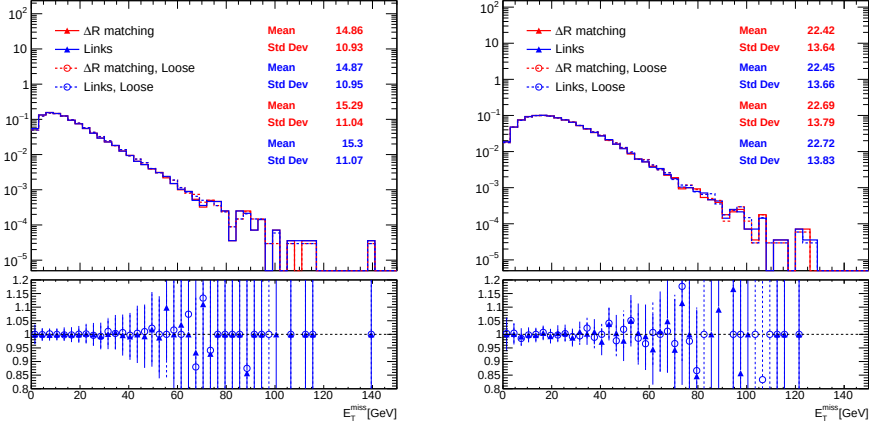
Figure 5.5: Distribution comparison, for Z \rightarrow ee events, of E_T^{\text{miss}} with the Run-2 PFlow reconstruction strategy (red) and the links-based one (blue) using the TST (left plots) and the CST (right plots) E_T^{\text{miss}} , for Looser and Tighter selection criteria. The first two mean and standard deviation values in top right box are associated to Tighter selections, the last two to Looser ones. The error bars include statistical uncertainties only.
