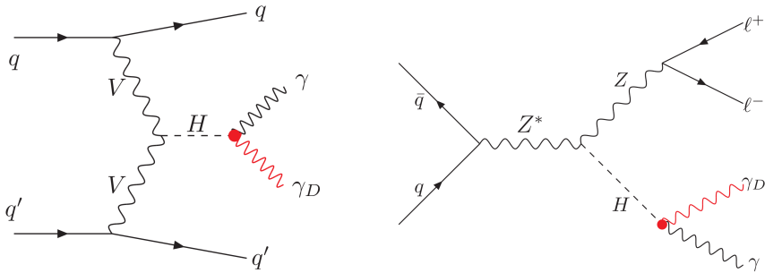
Figure 6.6: Feynman diagrams for the Higgs production via VBF (left), and ZH (right) channels at the LHC.
