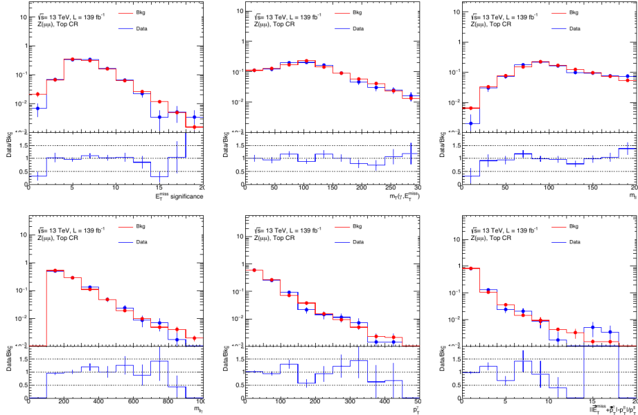
Figure 9.20: Shape comparison of the BDT input variables distributions between data and MC, in the \mu\mu channel of the top CR. The error includes only the statistical uncertainty.
