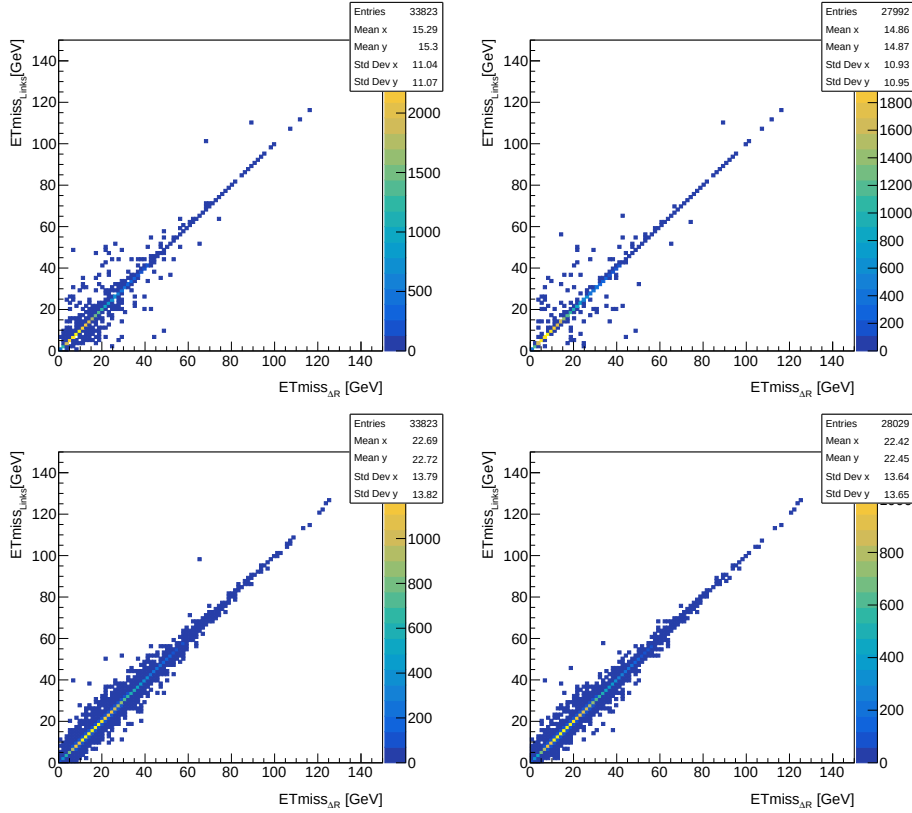
Figure 5.6: Event-by-Event comparison, for Z \rightarrow ee events, of E_T^{\text{miss}} with the Run-2 PFlow strategy (x axis) and the links-based one (y axis) using the TST Soft Term (top plots) and the CST one (bottom plots), for Looser (left plots) and Tighter (right plots) selection criteria.
