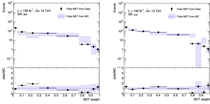
Figure B.11: Results of the extrapolation with a linear fit of the SR/VR ratio from data, for the ee channel (left) and \mu\mu channel.
