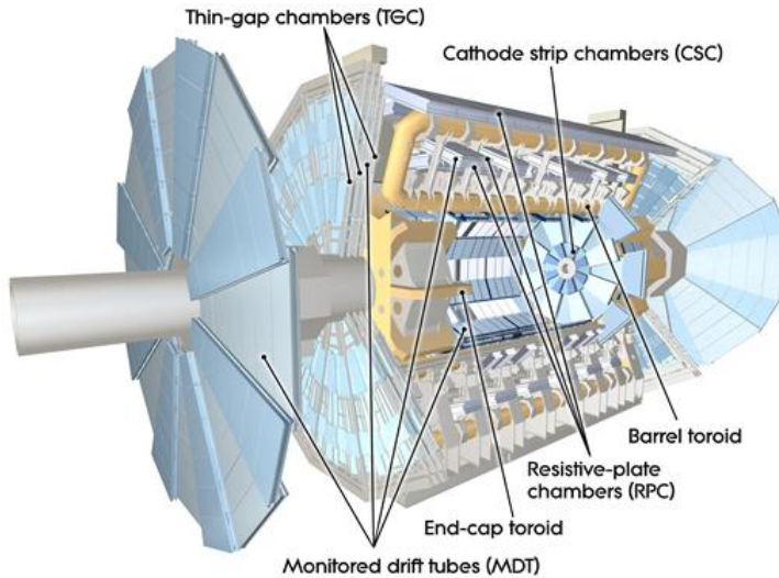
Figure 3.17: Sketch of the ATLAS Muon Spectrometer system [100].
