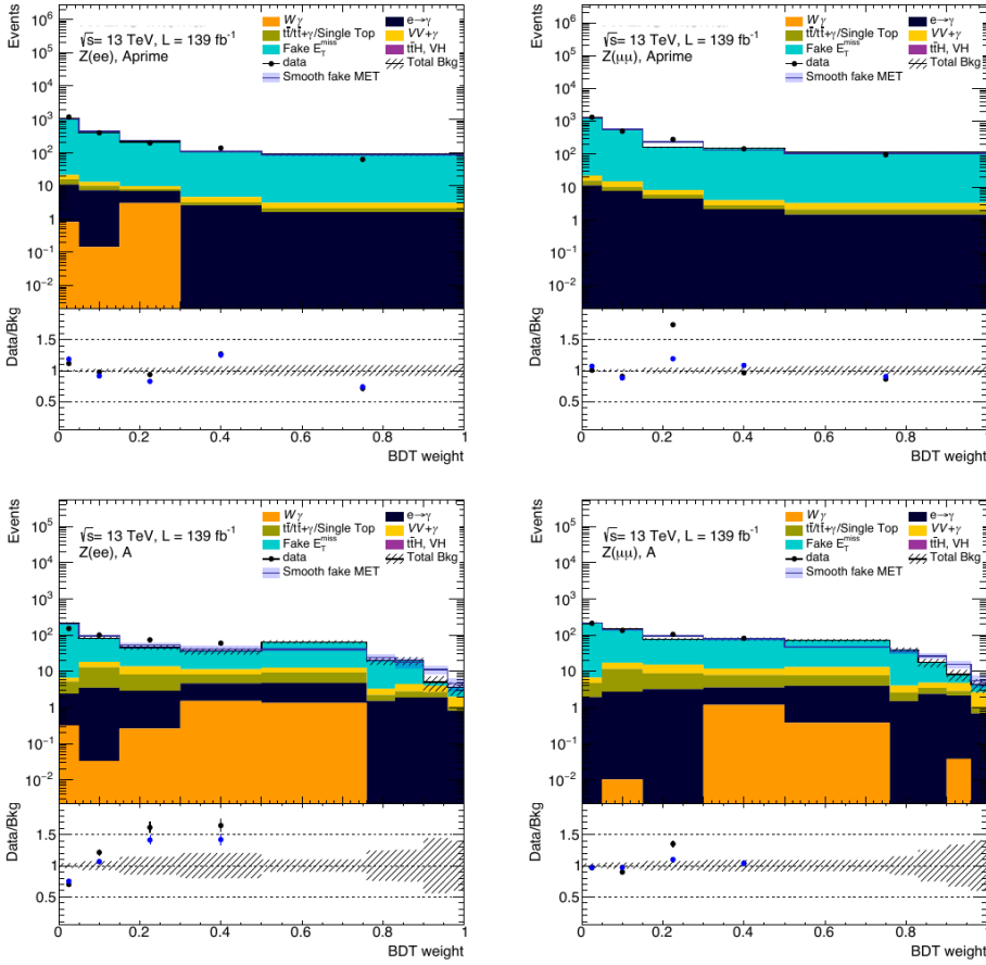
Figure 9.25: Comparison between BDT distributions with and without Z + \text{jets} smoothing, in the VR (top plots) and SR (bottom plots). The blue lines and blue point correspond to the total background with Z + \text{jets} events smoothed, and the error bands include only the statistical uncertainty.
