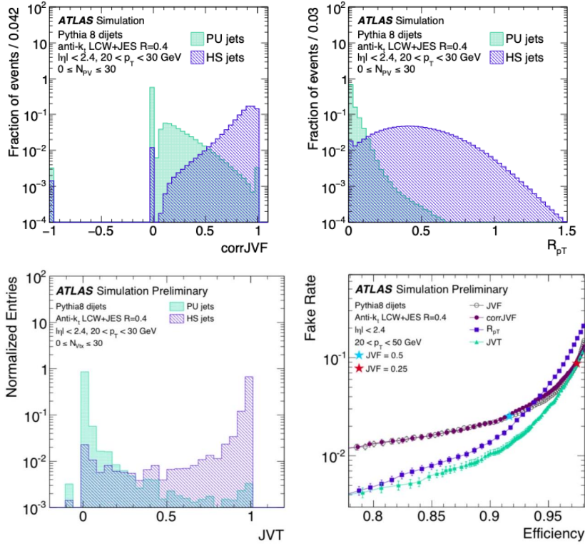
Figure 4.21: Distribution of the corrJVF (top left), R_{p_T} (top right) and JVT variables (bottom left) for pile-up (PU) and hard-scatter (HS) jets at the LC scale, with 20 < p_T < 30 GeV. In the bottom right plot, fake rate, at LC scale, from pile-up jets versus hard-scatter jet efficiency curves for JVF, corrJVF, R_{p_T} , and JVT [129].
