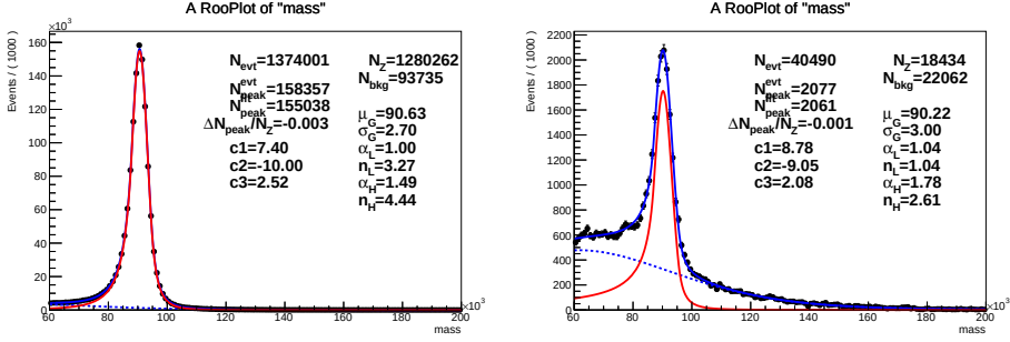
Figure 9.12: Fits for the distributions m_{ee} (left) and m_{e\gamma} (right) in MeV, using data, for \eta \in [0, 0.8] and p_T \in [25, 35] GeV. The signal and the background are represented respectively by the red line and the dotted blue line. The global trend of the fit is represented by the blue line.
