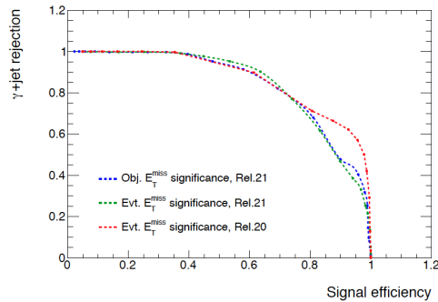
Figure 8.6: The \gamma + \text{jets} rejection as a function of the signal efficiency, varying the \mathcal{S} selection value. The results obtained with the previous Rel. 20 and with the event-based definition are compared with the ones from Rel. 21 with both the event-based and the object-based \mathcal{S} . The signal corresponds to a model with m_\chi = 10 GeV and M_{med} = 200 GeV
