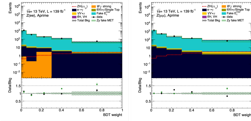
Figure B.15: Comparison between BDT shape in the VR ( 40 < E_T^{\text{miss}} < 60 GeV) obtained using the MC simulations including Z strong process to describe the shape of the fake E_T^{\text{miss}} background, and the ones obtained using only Z\gamma strong. The errors include only statistical uncertainties. In the bottom panel, the green dots correspond to the data/background using the extrapolation, while the black dots describe the data/background using pure MC.
