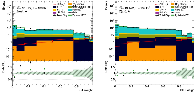
Figure B.16: Comparison between BDT shape in the SR obtained using the MC simulations including Z strong process to describe the shape of the fake E_T^{\text{miss}} background, and the ones obtained using only Z\gamma strong. The errors include only statistical uncertainties. In the bottom panel, the green dots correspond to the data/background using the extrapolation, while the black dots describe the data/background using pure MC.
