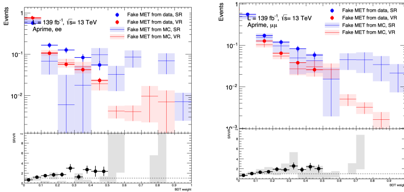
Figure B.6: BDT score distributions in the ee (left) and \mu\mu (right) channel, normalised to unit area, of the fake E_T^{\text{miss}} background in VR (red) and SR (blue) from data with other background subtracted (dots) up to BDT=0.5 and from MC in the full BDT range. The data uncertainties are statistical, while MC error bands include both the statistical and the systematic uncertainties arising from the data-driven method for fake E_T^{\text{miss}} estimation.
