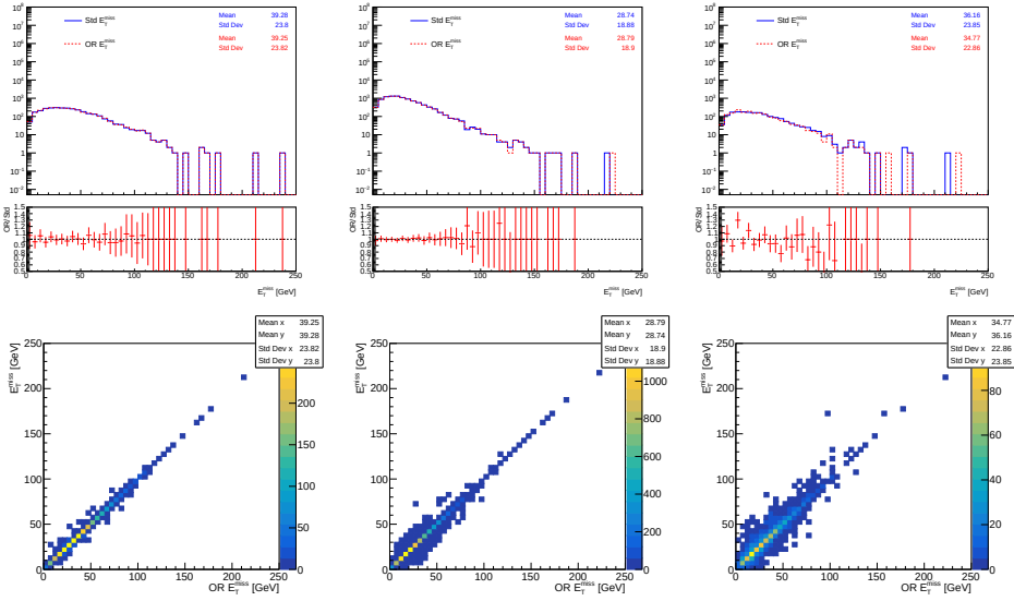
Figure 5.26: Comparison of E_T^{miss} reconstruction with “OR” Jet Term and standard one, in \gamma +jets events. The global E_T^{miss} distributions are compared, as well as the event-by-event values, for events with no overlap (left), with exact overlap (center), and with partial overlap (right) between jets and other physics objects, both considering the TST E_T^{miss} .
