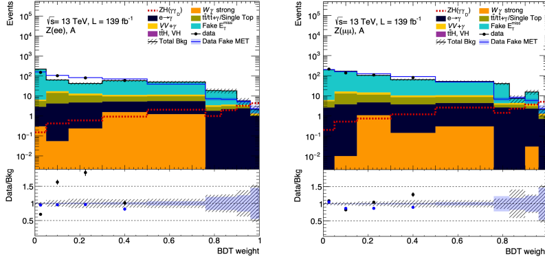
Figure B.12: Comparison between BDT shape in the SR obtained using the MC simulations to describe the shape of the fake E_T^{\text{miss}} background, and the ones obtained using the extrapolation method. The errors include only statistical uncertainties. In the bottom panel, the blue dots correspond to the data/background using the extrapolation, while the black dots describe the data/background using pure MC.
