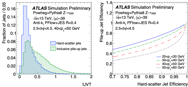
Figure 4.22: Distribution of the fJVT variable for hard-scatter and pile-up forward PFlow jets in the 40 < p_T < 50 GeV range (left), and efficiency for PU forward jets in simulated Z+jets events as a function of the efficiency for hard-scatter jets for different jet p_T ranges [128].
