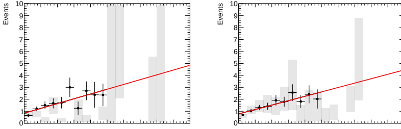
Figure B.8: Linear fit of the SR/VR ratio from data for the ee channel (left) and \mu\mu channel.
