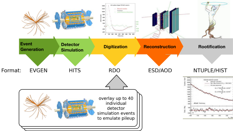
Figure 7.1: Sketch of the ATLAS MC production chain [152].
