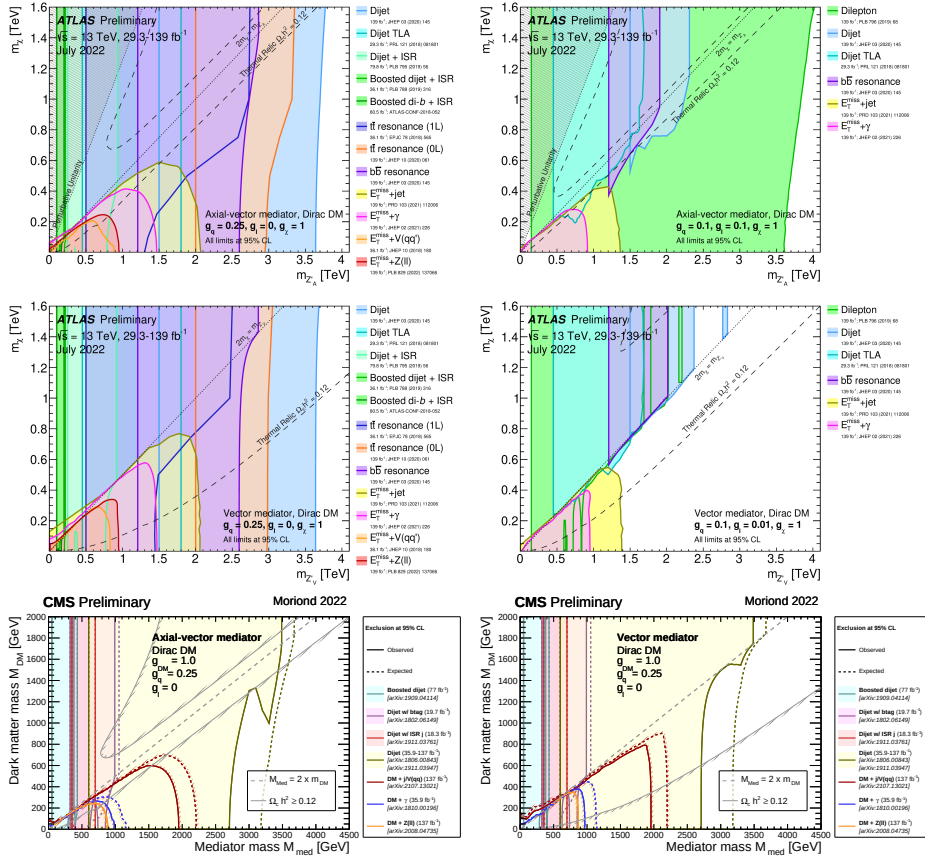
Figure 11.1: Comparison of the limits in M_{med} - m_\chi plane set by Run-2 data analyses carried out, in different channels, by the ATLAS [140] (first two rows) and CMS [229] (last row) collaborations, considering four different signal models.
