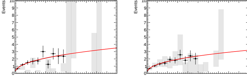
Figure B.7: Power-law fit of the SR/VR ratio from data for the ee channel (left) and \mu\mu channel.
