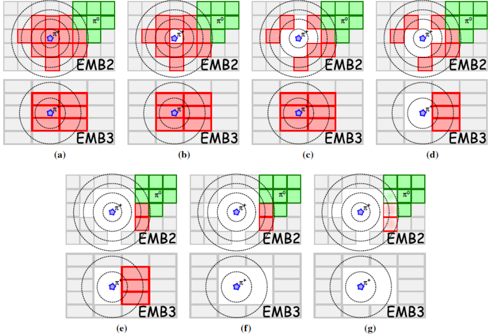
Figure 4.18: An idealised example of how the cell-by-cell subtraction works. Cells in two adjacent calorimeter layers (EMB2 and EMB3) are shown in grey if they are not in clusters, red and green if they belong to a \pi^+ cluster and a \pi^0 meson respectively. The stars represent the extrapolated tracks, and the steps of the ring-based removal procedure are illustrated in the different subfigures. The final ring contains more energy than the expected energy, hence this is only partially subtracted (g), indicated by a lighter shading
