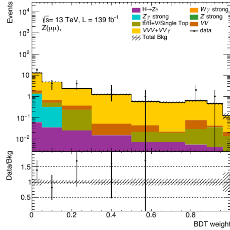
Figure 9.17: BDT weight distribution for data and background in the VV\gamma CR with 3 muons and no E_T^{\text{miss}} and \Delta\phi(\vec{E}_T^{\text{miss}}, p_T^l) selections. The error shown corresponds to the statistical uncertainty.
