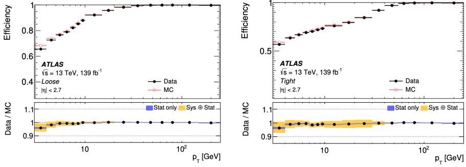
Figure 4.13: Muon isolation efficiency measured in Z \rightarrow \mu\mu events for the Loose (left plot) and Tight (right plot) WP, as a function of p_T . The statistical uncertainty in the efficiency measurement is smaller than the size of the markers, and thus not displayed. The panel at the bottom shows the ratio of the measured to predicted efficiencies, with statistical and systematic uncertainties [116].
