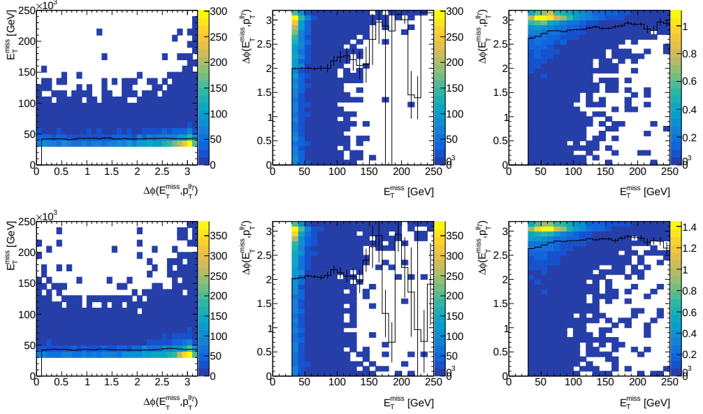
Figure 9.5: 2D plots, in the ee (top) and \mu\mu (bottom) channel, of E_T^{\text{miss}} VS \Delta\phi(\vec{E}_T^{\text{miss}}, \vec{p}_T^{\text{ll}\gamma}) (left) and \Delta\phi(\vec{E}_T^{\text{miss}}, \vec{p}_T^{\text{ll}\gamma}) VS E_T^{\text{miss}} (center) for the Z\gamma + \text{jets} process. As a comparison, \Delta\phi(\vec{E}_T^{\text{miss}}, \vec{p}_T^{\text{ll}\gamma}) VS E_T^{\text{miss}} is also shown for the signal (right). The histograms in black represent the mean value of E_T^{\text{miss}} in each \Delta\phi(\vec{E}_T^{\text{miss}}, \vec{p}_T^{\text{ll}\gamma}) bin (and viceversa).
