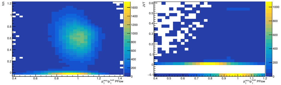
Figure 8.15: Left: f_{ch} versus p_T^{reco}/p_T^{truth} of the leading truth-matched PFlow jet, for preselected events. Right: JVT versus p_T^{reco}/p_T^{truth} of the leading truth-matched PFlow jet, for preselected events with f_{ch} < 0.1
