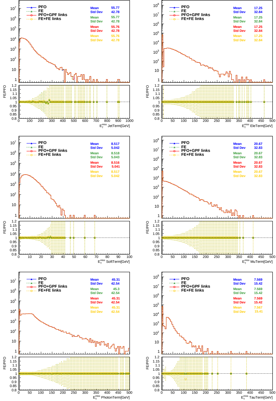
Figure 5.18: Jet, Soft and Photon Term for H \rightarrow \gamma\gamma (left), Electron and Muon Terms for t\bar{t} (right top and central) and Tau Term for Z \rightarrow \tau\tau (right bottom). The error bars include statistical uncertainties only.
