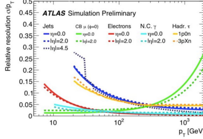
Figure 4.29: Resolution of the objects entering the E_T^{\text{miss}} calculation as a function of p_T and for different values of |\eta| . The label N.C. \gamma indicates unconverted photons and Hadr. \tau hadronically decaying \tau -leptons. 1p0n (3pXn) corresponds to the decay mode with one (three) charged hadron, zero (one or more) neutral hadrons and a non detectable \tau -neutrino.
