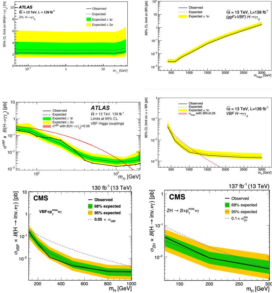
Figure 11.2: In the top plots, exclusion limits at 95% CL on BR(H \rightarrow \gamma\gamma_d) as a function of the Dark Photon mass in the ZH production mode [201](left), and as a function of BSM Higgs mass in the ggF+VBF production mode (right). In the central plots, exclusion limits at 95% CL on \sigma \times BR(H \rightarrow \gamma\gamma_d) as a function of the Higgs mass, in the VBF Higgs production mode, provided by the VBF analysis [147] (left) and mono-photon reinterpretation (right). The red line shows the expected values under the assumption of BR=5\% and theoretical production cross-section reported in [17]. Finally, in the bottom plots, the CMS limits on the \sigma \times BR(H \rightarrow \gamma\gamma_d) , as a function of the Higgs mass in the VBF [149] and ZH [148] production mode. The theoretical expectations are shown in blue dashed line, assuming a 5% and 1% BR.
