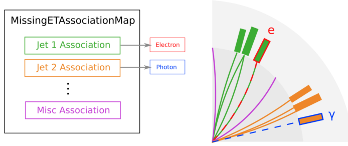
Figure 5.2: Illustration of the structure of the MissingETAssociationMap EDM and the typical detector signals (tracks and calorimeter clusters) corresponding to each element [136]
