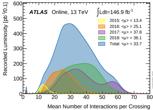
Figure 3.7: Luminosity-weighted distribution of the mean number of interactions per crossing for the full Run-2 pp collision data at \sqrt{s} = 13 TeV [95].
