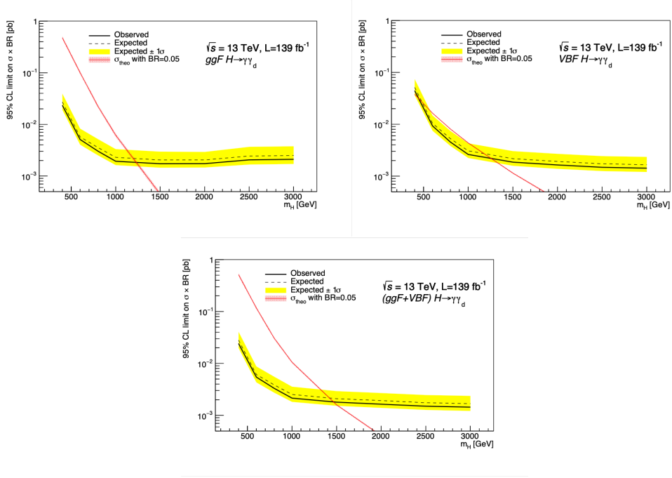
Figure 10.4: Observed and expected exclusion limits at 95% CL on \sigma \times \text{BR}(H \rightarrow \gamma \gamma_d) as function of the BSM Higgs mass, in gluon-gluon Fusion (top left), VBF (top right) and ggF+VBF (bottom) production mode. The yellow band shows the \pm 1\sigma uncertainties. The theoretically predicted cross-section is superimposed assuming the \text{BR}(H \rightarrow \gamma \gamma_d) = 0.05 and the theoretical production cross-section reported in [17].
