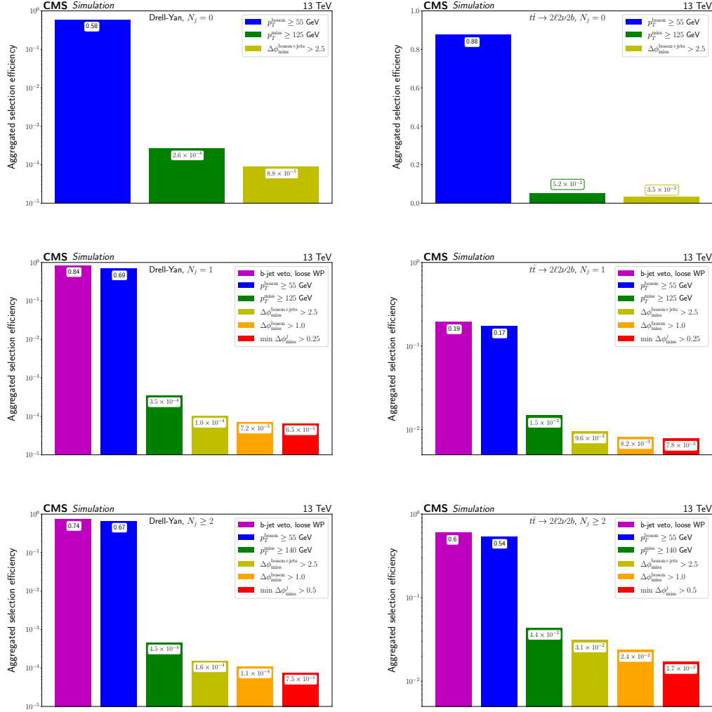
Figure 5.31: Efficiencies of the different selection requirements are shown for the DY (left) and t\bar{t} \rightarrow 2\ell 2\nu 2b processes (right) over the inclusive m_{\text{T}}^{ZZ} range for N_j = 0 (top panels), N_j = 1 (middle panels), or N_j \geq 2 (bottom panels). The efficiencies shown in each bar are after applying the previous set of cuts listed in the legend and also after the set of cuts listed in 5.2 up to |m_{\ell\ell} - 91.2| < 15 \text{ GeV} cut.
