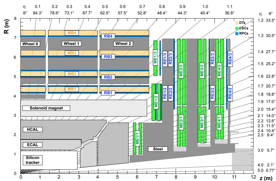
Figure 2.8: One quadrant of the CMS detector in which the DT, CSC and RPC systems are highlighted in yellow, green and blue respectively [25].
