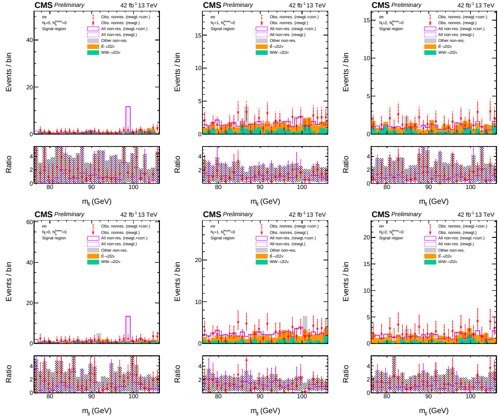
Figure C.2: The m_{\ell\ell} distributions (e e on the top, \mu\mu on the bottom panels) in the signal region are shown for the 2017 data set in each N_j category ( = 0 , = 1 , and \geq 2 from left to right). The red points with error bars show the prediction from the observed data, either with f_{corr}^{\ell\ell} factors applied (filled stars with solid error bars) or without (hollow stars with dashed error bars). The predictions of each simulated non-resonant background component are shown in histograms filled with different colors, stacked on top of each other. The hollow, solid histograms agree with the prediction of the sum of light green (WW continuum production), orange (WW production through the t\bar{t} process), and gray (other small nonresonant contributions) histograms within the statistical uncertainties of the simulation. The statistical uncertainties on the expected and predicted distributions from simulation are not shown in the top event distribution panels to avoid cluttering, but they are shown in the bottom ratio panels, which are shown relative to the stacked histograms.
