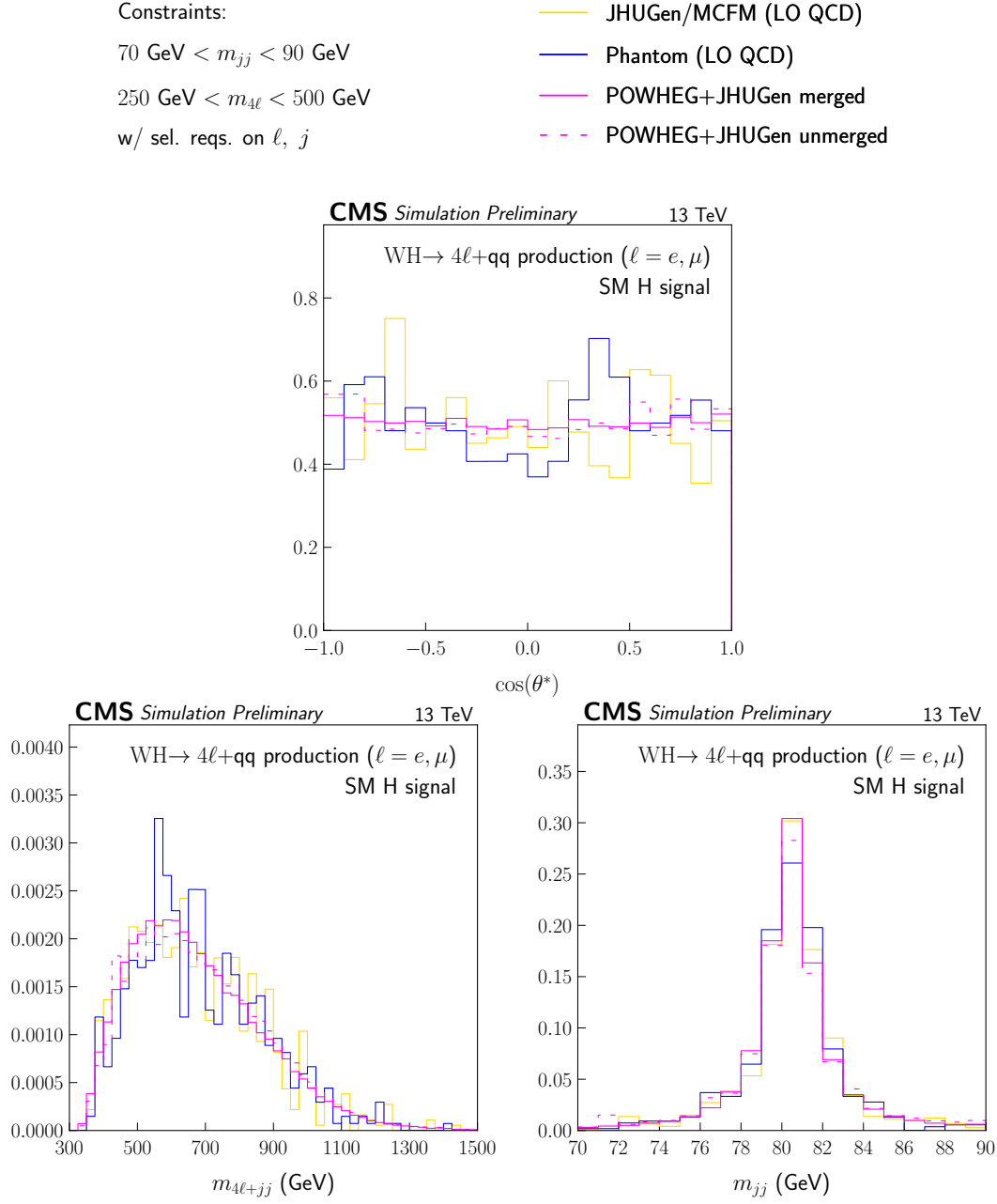
Figure 5.7: The distributions of \cos\theta^* , m_{4\ell+jj} and m_{jj} for off-shell H boson production through the SM EW signal process. The requirement 70 \text{ GeV} < m_{jj} < 90 \text{ GeV} is applied along with requirements on the initial and final state composition to emphasize the WH-like topology. All distributions are normalized to unit area.
