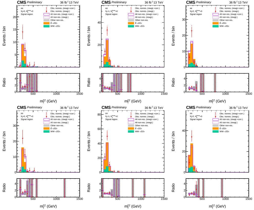
Figure C.6: The m_T^{ZZ} distributions ( ee on the top, \mu\mu on the bottom panels) in the signal region are shown for the 2016 data set in each N_j category ( = 0 , = 1 , and \geq 2 from left to right). The different components and style features shown match those in Fig. C.1.
