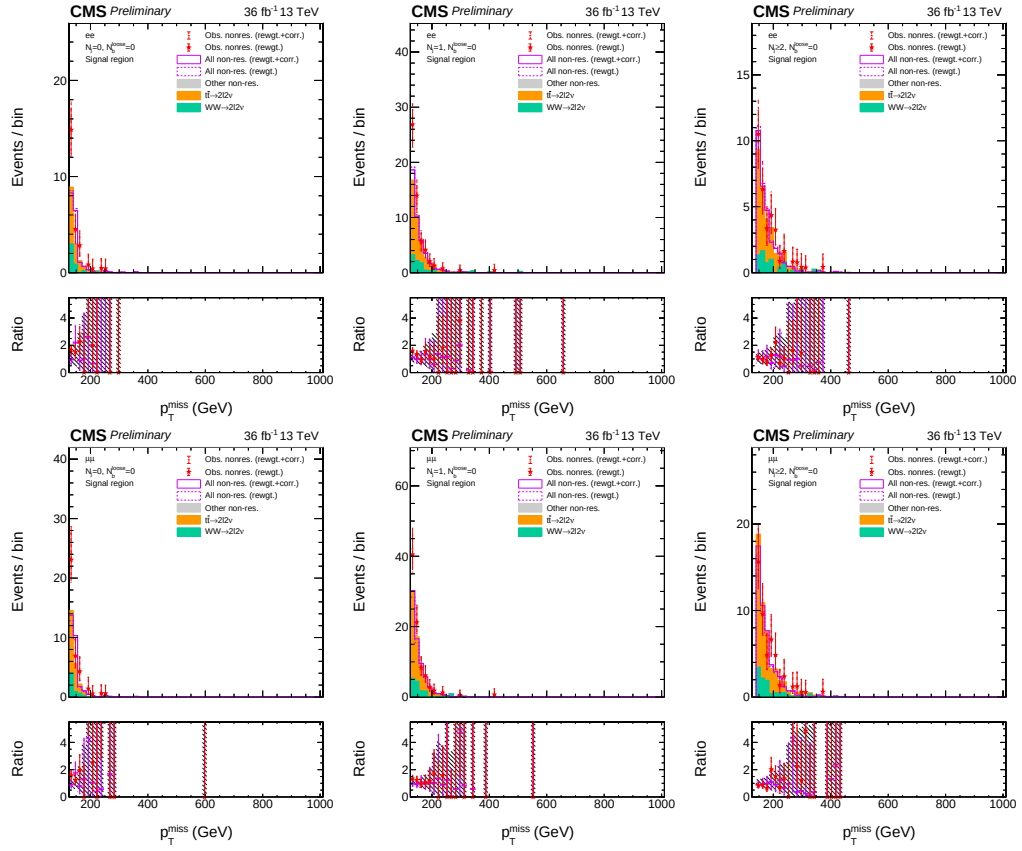
Figure C.4: The p_T^{\text{miss}} distributions ( e e on the top, \mu \mu on the bottom panels) in the signal region are shown for the 2016 data set in each N_j category ( = 0, = 1 , and \geq 2 from left to right). The red points with error bars show the prediction from the observed data, either with f_{\text{corr}}^{\ell\ell} factors applied (filled stars with solid error bars) or without (hollow stars with dashed error bars). The predictions of each simulated non-resonant background component are shown in histograms filled with different colors, stacked on top of each other. The hollow, solid and dashed purple histograms show the prediction from simulated e\mu events, reweighted according to 5.8 with the f_{\text{corr}}^{\ell\ell} factor included or omitted, respectively. The hollow, solid and dashed purple histograms agree with the prediction of the sum of light green (WW continuum production), orange (WW production through the t\bar{t} process), and gray (other small nonresonant contributions) histograms within the statistical uncertainties of the simulation. The statistical uncertainties on the expected and predicted distributions from simulation are not shown in the top event distribution panels to avoid cluttering, but they are shown in the bottom ratio panels, which are shown relative to the stacked histograms.
