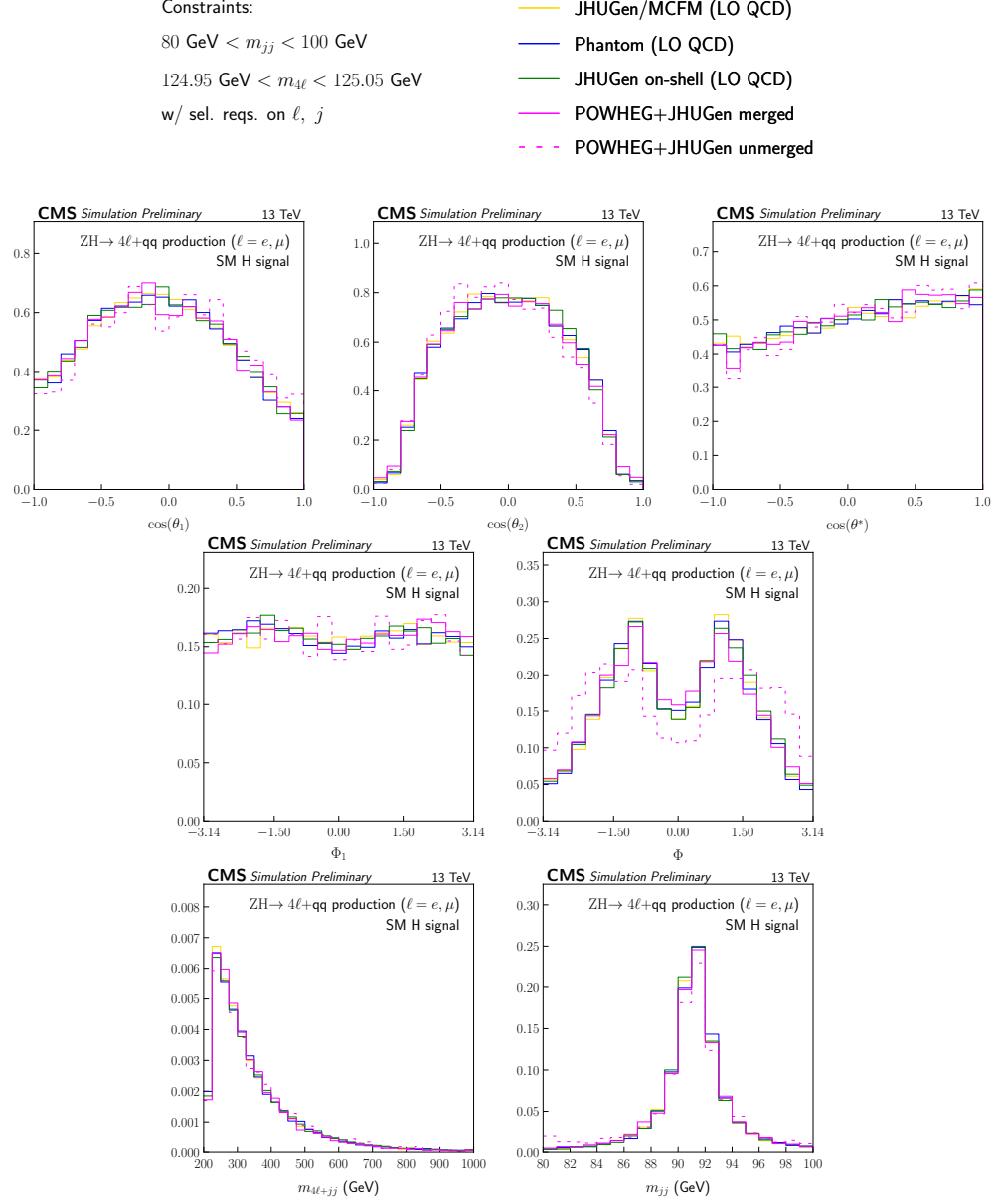
Figure B.2: The distributions of \cos\theta_1 , \cos\theta_2 , \cos\theta^* , \Phi_1 , \Phi , m_{4\ell+jj} and m_{jj} (from top left to bottom right) for on-shell H boson production through the SM EW signal process. The requirement 80 \text{ GeV} < m_{jj} < 100 \text{ GeV} is applied along with requirements on the initial and final state composition to emphasize the ZH-like topology. The different predictions are shown on the legend at the top, and all distributions are normalized to unit area. The unmerged POWHEG scenario uses the two outgoing partons leading in p_T to compute the kinematic quantities.
