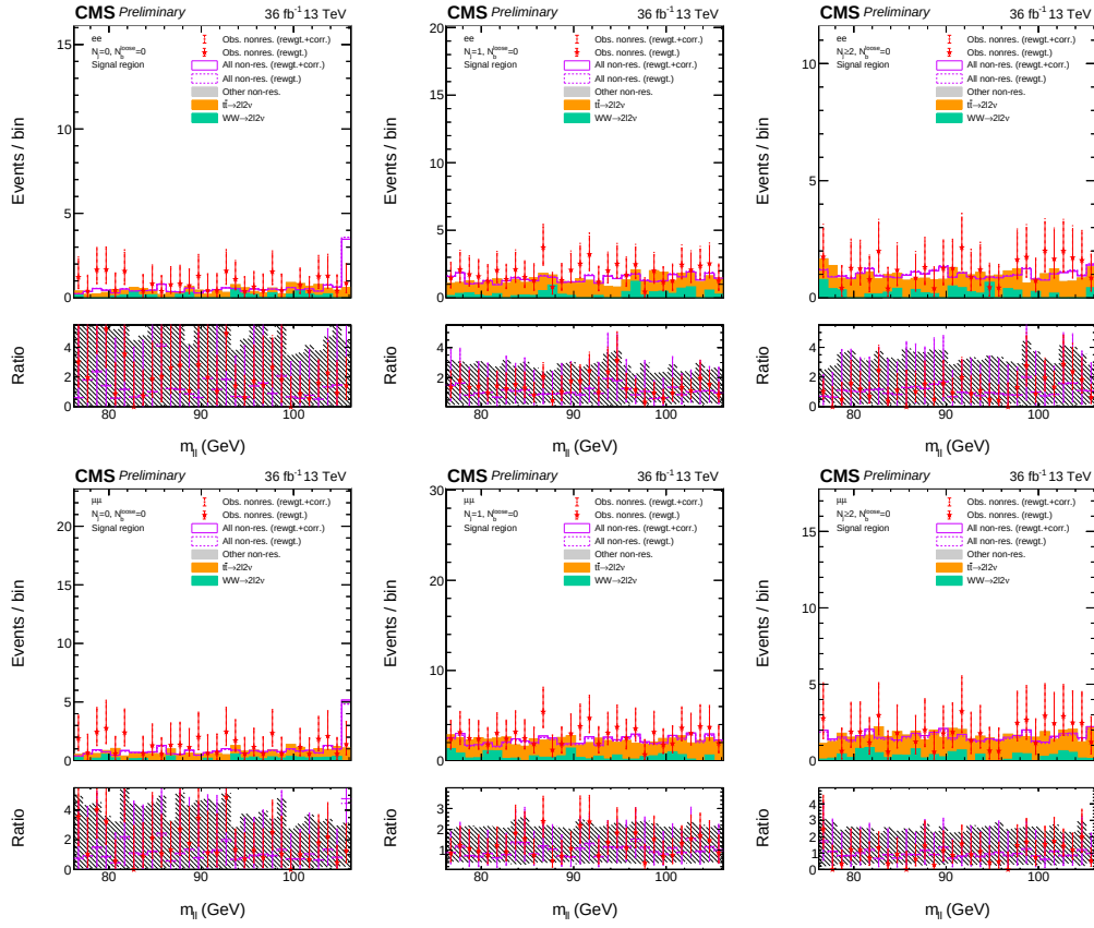
Figure C.1: The m_{\ell\ell} distributions ( e e on the top, \mu\mu on the bottom panels) in the signal region are shown for the 2016 data set in each N_j category ( = 0 , = 1 , and \geq 2 from left to right). The red points with error bars show the prediction from the observed data, either with f_{corr}^{\ell\ell} factors applied (filled stars with solid error bars) or without (hollow stars with dashed error bars). The predictions of each simulated non-resonant background component are shown in histograms filled with different colors, stacked on top of each other. The hollow, solid and dashed purple histograms show the prediction from simulated e\mu events, reweighted according to 5.8 with the f_{corr}^{\ell\ell} factor included or omitted, respectively. The hollow, solid histograms agree with the prediction of the sum of light green (WW continuum production), orange (WW production through the t\bar{t} process), and gray (other small nonresonant contributions) histograms within the statistical uncertainties of the simulation. The statistical uncertainties on the expected and predicted distributions from simulation are not shown in the top event distribution panels to avoid cluttering, but they are shown in the bottom ratio panels, which are shown relative to the stacked histograms.
