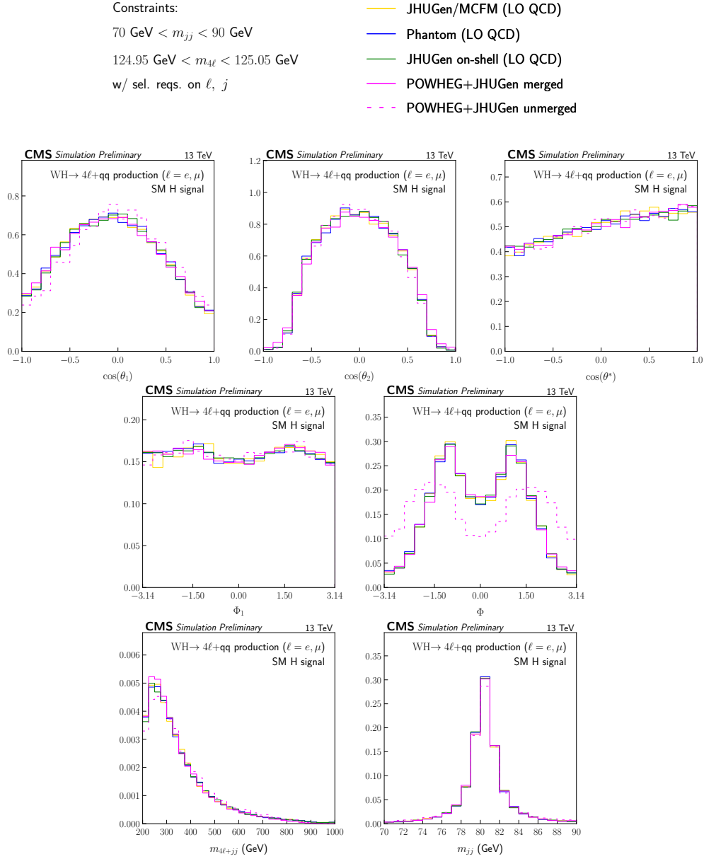
Figure B.3: The distributions of \cos\theta_1 , \cos\theta_2 , \cos\theta^* , \Phi_1 , \Phi , m_{4\ell+jj} and m_{jj} (from top left to bottom right) for on-shell H boson production through the SM EW signal process. The requirement 70 \text{ GeV} < m_{jj} < 90 \text{ GeV} is applied along with requirements on the initial and final state composition to emphasize the WH-like topology. The different predictions are shown on the legend at the top, and all distributions are normalized to unit area. The unmerged POWHEG scenario uses the two outgoing partons leading in p_T to compute the kinematic quantities.
