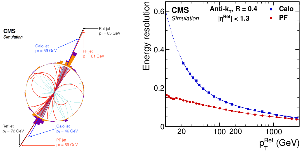
Figure 4.6: Left: an example of jet reconstruction in a simulated dijet event. The p_T of the PF jets are shown in red which can be compared to the p_T of the generated (Ref jet) and the calorimeter (Calo jet) shown in black and blue respectively. Right: comparison of the energy resolutions of the PF jet and Calo jet as a function of Ref jet p_T [69].
