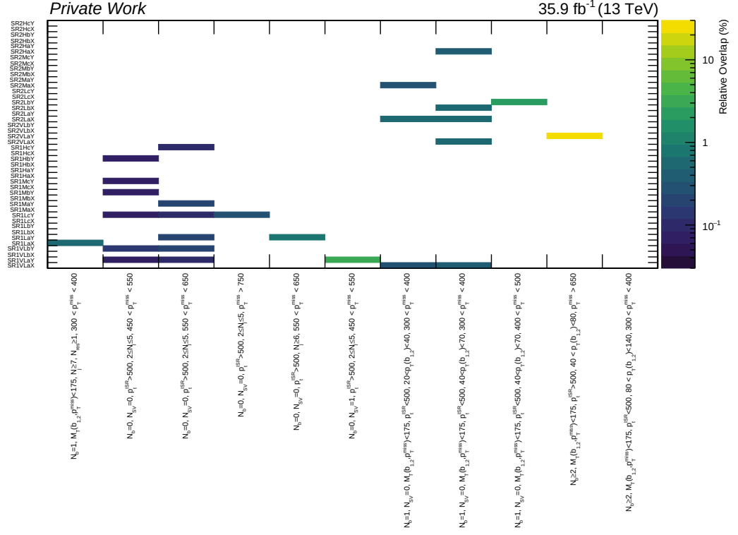
Figure A.7: Relative overlaps, as measured from data events, between the 1\ell SRs and 0\ell SRs normalized to the average sizes of the two regions.
