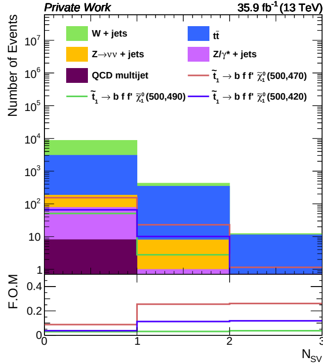
Figure 5.35: The SV multiplicity distribution is shown for the few signal scenarios and the dominant backgrounds. The figure of merit (FOM), shown in the bottom panel, is calculated for each signal scenario based on the methods described in [18].
