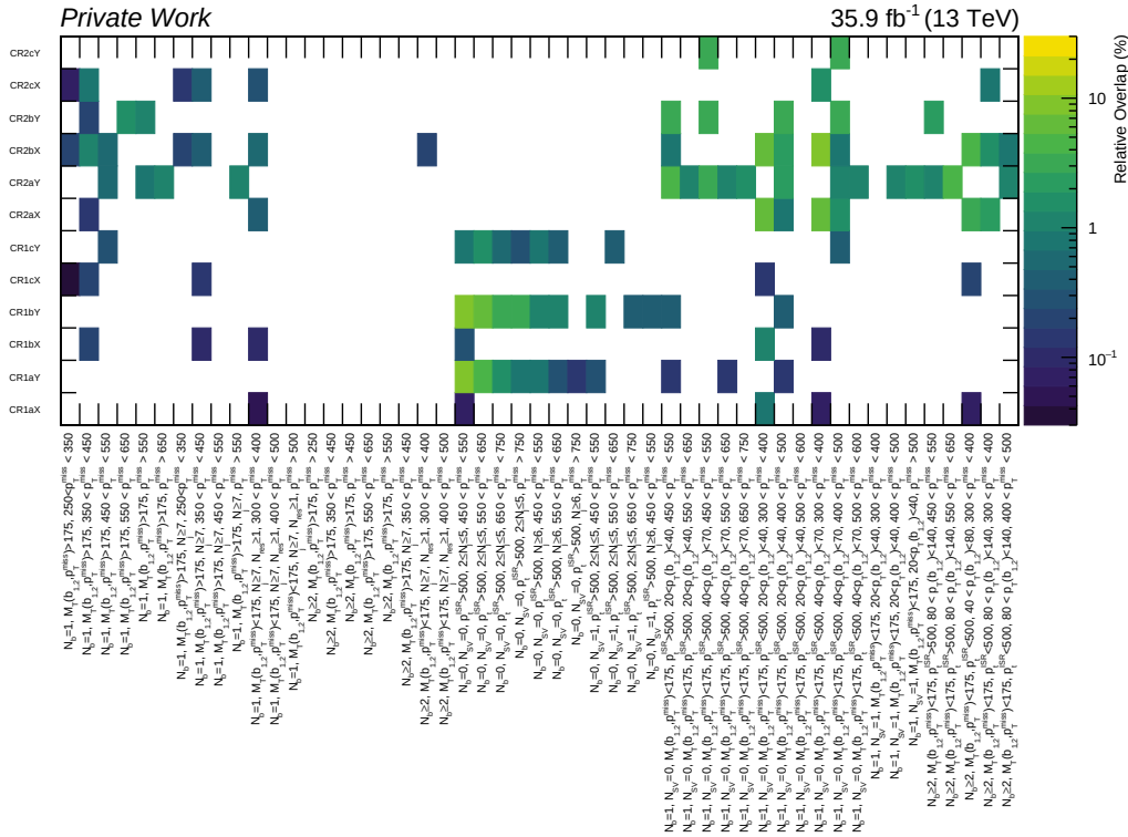
Figure A.6: Relative overlaps, as measured from data events, between the 1\ell CRs and 0\ell CRs normalized to the average sizes of the two regions.
