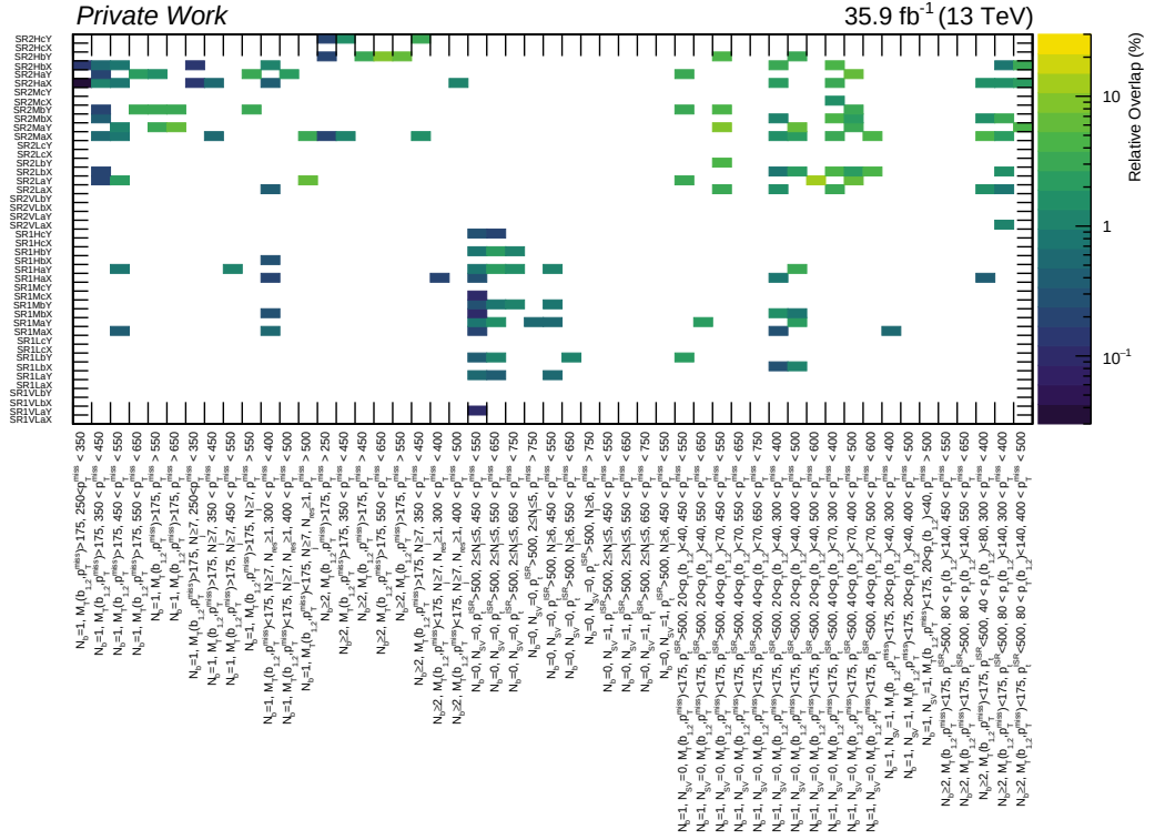
Figure A.5: Relative overlaps, as measured from data events, between the 1\ell SRs and 0\ell CRs normalized to the average sizes of the two regions.
